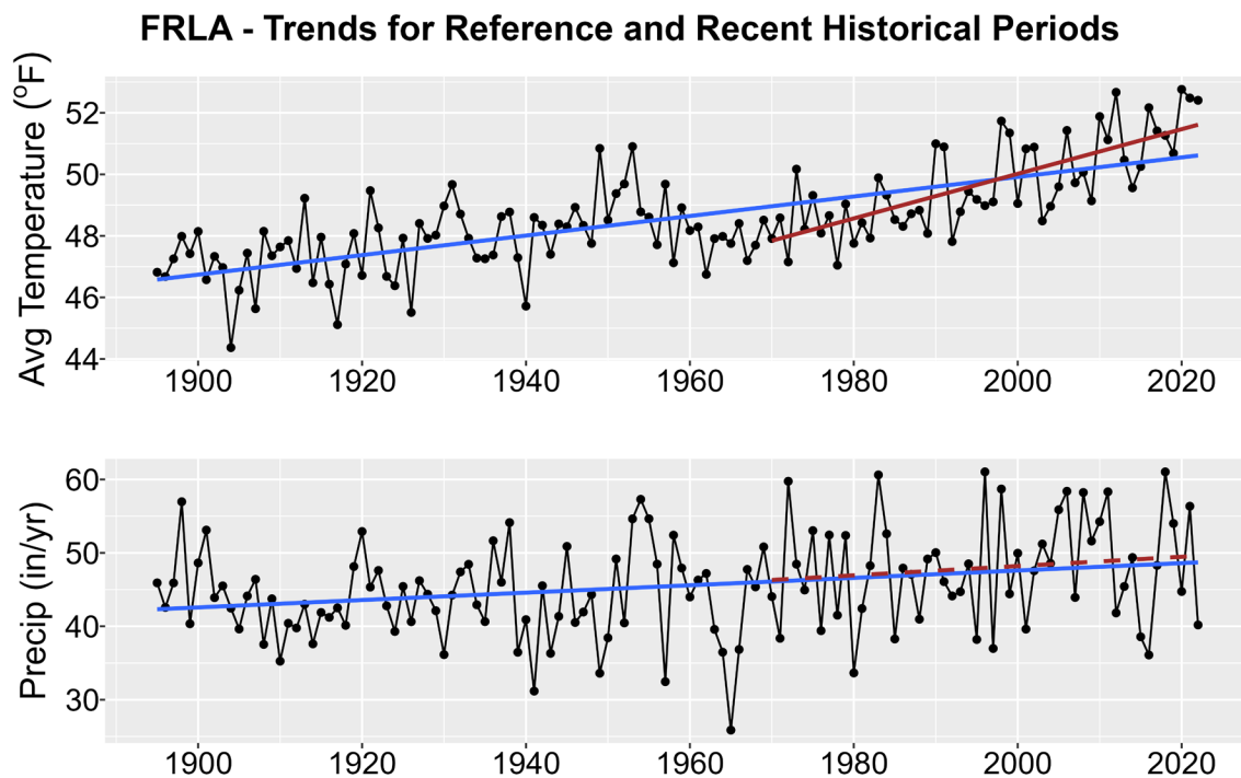
Figure 1. Historical trends in annual average temperature (upper plot) and annual total precipitation (lower plot) for FRLA from 1895-2022. Black points show yearly values while blue lines are linear regressions for the entire period record and red lines for 1970-2022 trends. Solid lines are significant trends (i.e., p < 0.05 ); dashed lines are not statistically significant.
