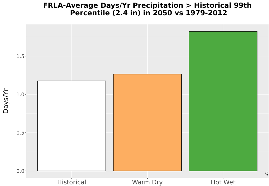
Figure 6. Average number of days annually with precipitation exceeding the 99th percentile (2.4 in.) of precipitation from the historical period 1979-2012 and for each climate future.
