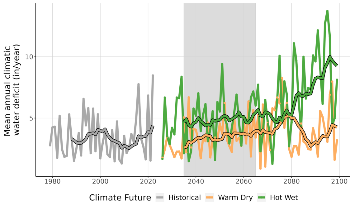
Figure 9. This line graph compares observed climatic water deficit at FRLA (inches/year) (1979-2022) with projected climatic water deficit for the two climate futures over the period 2023-2099. The historical observation data is shown in gray, the Warm Dry climate future in orange, and the Hot Wet climate future in green. The smooth line running through each projection is the 10-year running average for historical observations and future projections. Gray-shaded area represents the time period that was averaged (2035-2065) to summarize future projections for the year 2050.
