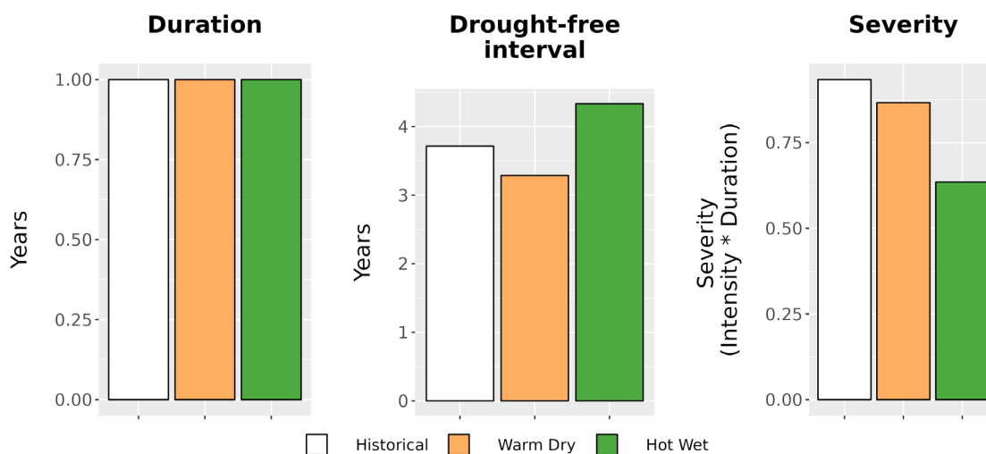
Figure 8. Drought metrics for FRLA. (Left) Average drought duration (years) historically (1979-2012) and under each climate future. (Middle) Average drought return interval (years), indicating the expected amount of time between periods of drought, historically and under each climate future. (Right) Average drought severity, a measure of drought intensity multiplied by duration, historically and under each climate future.
