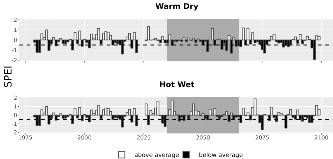
Figure 7. Drought metrics for FRLA. Drought index (SPEI; units = standard deviations from historical) timeseries for each climate future. Below-average SPEI (black bars) indicates dry conditions. The dotted line (SPEI = -0.5) indicates drought conditions.
