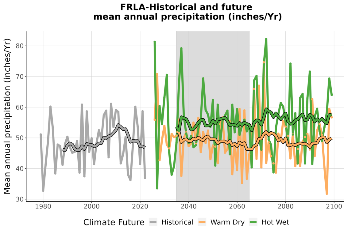
Figure 4. This graph compares observed average annual precipitation at FRLA (inches/year) (1979-2022) with projected average annual precipitation for the two climate futures over the period 2023-2099. The historically observed data is shown in gray, the Warm Dry climate future in orange, and the Hot Wet climate future in green. The smooth line running through each projection is the 10-year running average for historical observations and future projections. The gray-shaded area represents the time period that was averaged (2035-2065) to summarize future projections for the year 2050 (Appendix 1).
