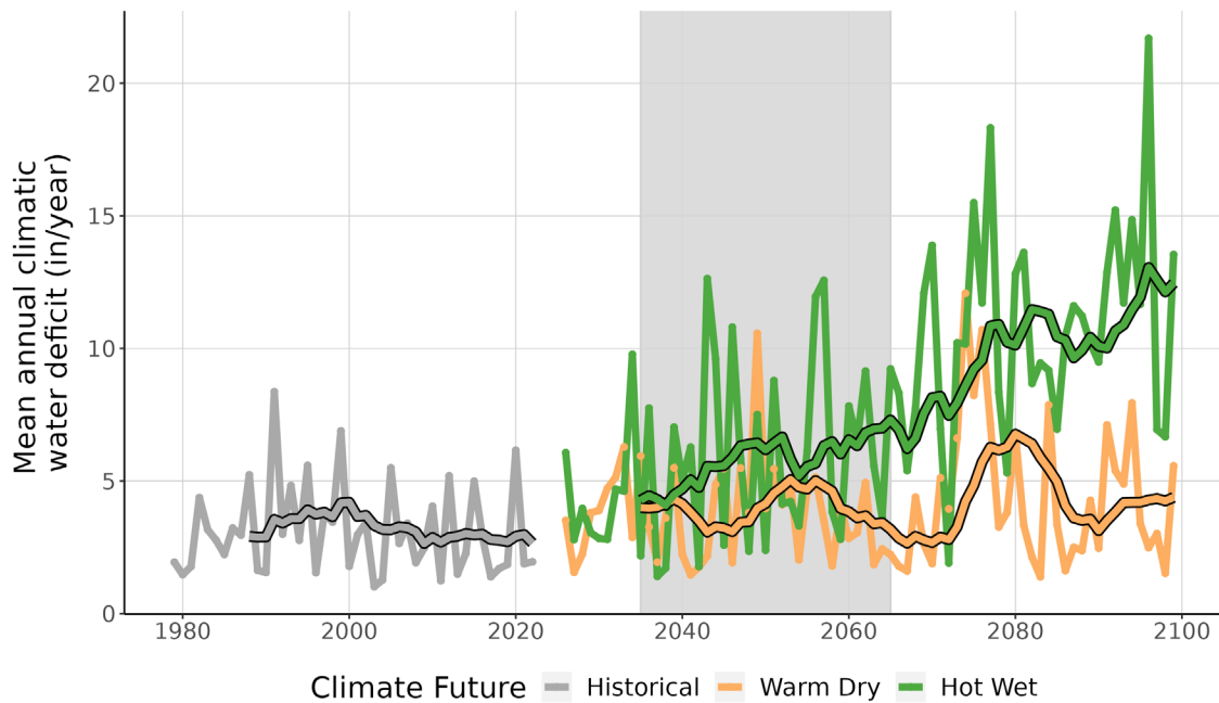
Figure 9. This line graph compares observed climatic water deficit at FRHI (inches/year) (1979-2022) with projected climatic water deficit for the two climate futures over the period 2023-2099. The historical observation data is shown in gray, the Warm Dry climate future in orange, and the Hot Wet climate future in green. The smooth line running through each projection is the 10-year running average for historical observations and future projections. Gray-shaded area represents the time period that was averaged (2035-2065) to summarize future projections for the year 2050.
