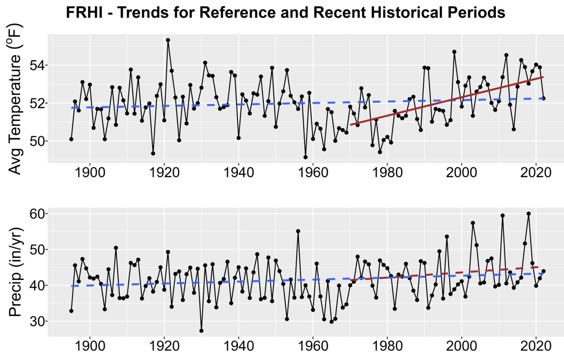
Figure 1. Historical trends in annual average temperature (upper plot) and annual total precipitation (lower plot) for FRHI from 1895-2022. Black points show yearly values while blue lines are linear regressions for the entire period record and red lines for 1970-2022 trends. Solid lines are significant trends (i.e., p < 0.05 ); dashed lines are not statistically significant.
