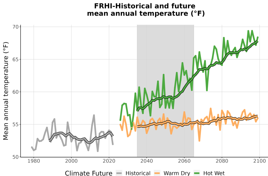
Figure 3. This graph compares observed average annual temperature at FRHI (°F) (1979-2022) with projected average annual temperature for the two climate futures over the period 2023-2099. The historically observed data
