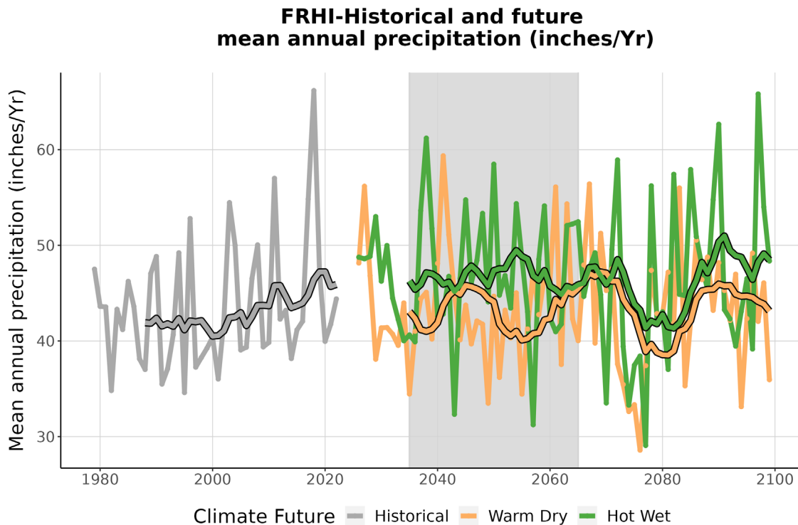
Figure 4. This graph compares observed average annual precipitation at FRHI (inches/year) (1979-2022) with projected average annual precipitation for the two climate futures over the period 2023-2099. The historically observed data is shown in gray, the Warm Dry climate future in orange, and the Hot Wet climate future in green. The smooth line running through each projection is the 10-year running average for historical observations and future projections. The gray-shaded area represents the time period that was averaged (2035-2065) to summarize future projections for the year 2050 (Appendix 1).
