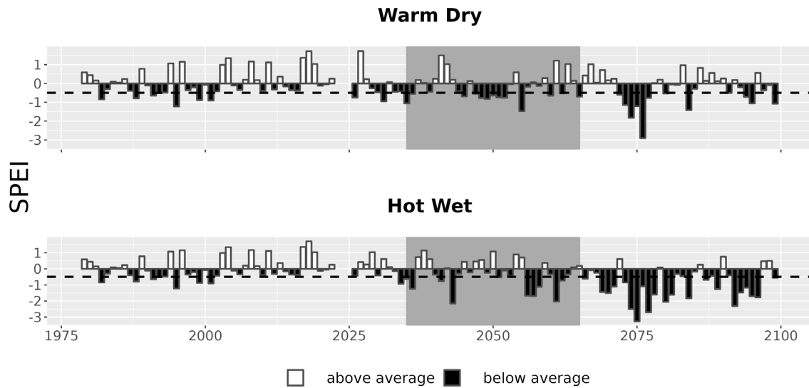
Figure 7. Drought metrics for FRHI. Drought index (SPEI; units = standard deviations from historical) timeseries for each climate future. Below-average SPEI (black bars) indicates dry conditions. The dotted line (SPEI = -0.5) indicates drought conditions.
