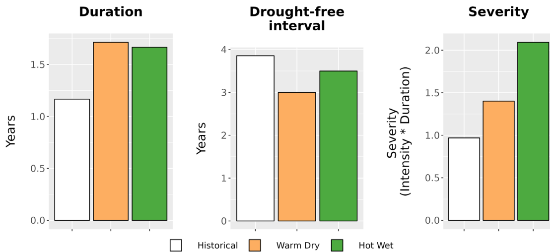
Figure 8. Drought metrics for FRHI. (Left) Average drought duration (years) historically (1979-2012) and under each climate future. (Middle) Average drought return interval (years), indicating the expected amount of time between periods of drought, historically and under each climate future. (Right) Average drought severity, a measure of drought intensity multiplied by duration, historically and under each climate future.
