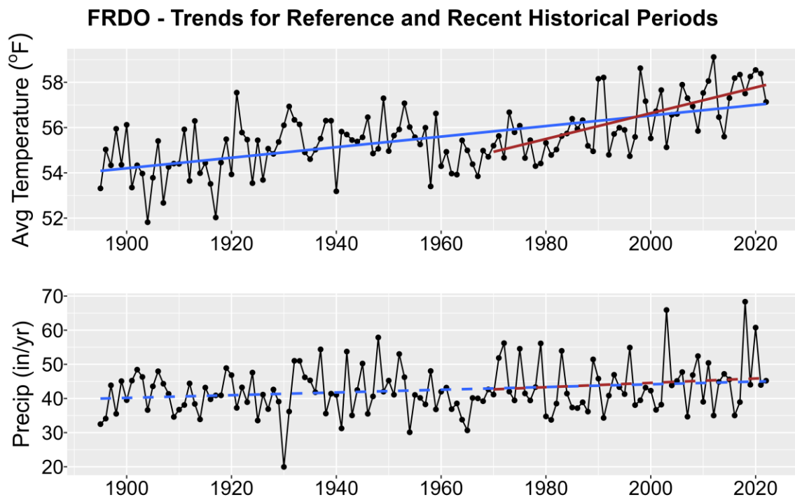
Figure 1. Historical trends in annual average temperature (upper plot) and annual total precipitation (lower plot) for FRDO from 1895-2022. Black points show yearly values while blue lines are linear regressions for the entire period record and red lines for 1970-2022 trends. Solid lines are significant trends (i.e., p < 0.05 ); dashed lines are not statistically significant.
