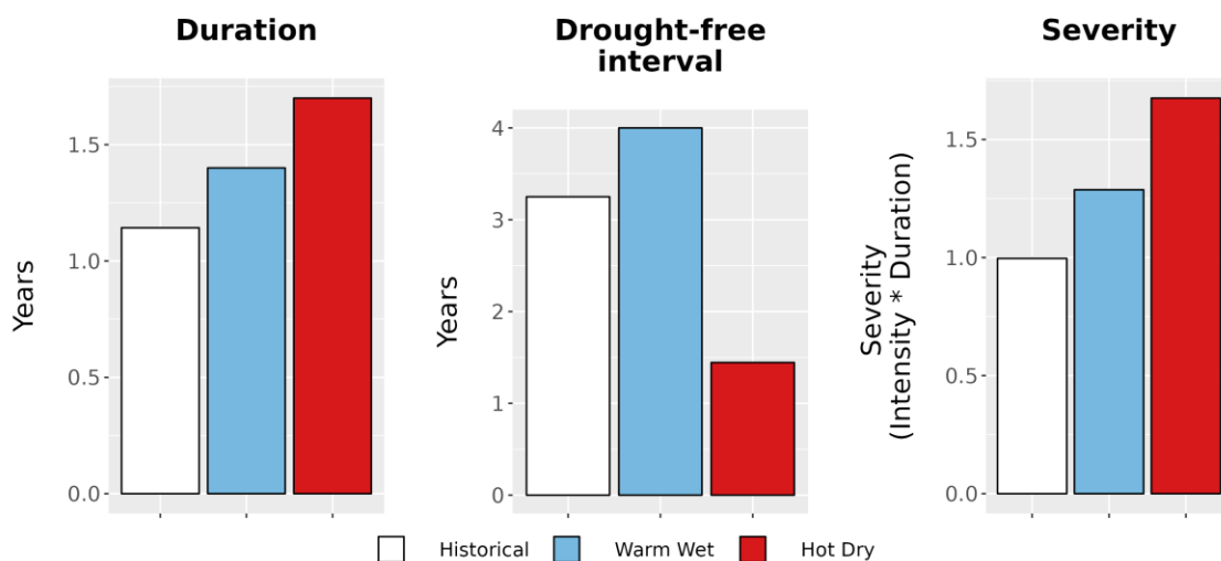
Figure 8. Drought metrics for FRDO. (Left) Average drought duration (years) historically (1979-2012) and under each climate future. (Middle) Average drought return interval (years), indicating the expected amount of time between periods of drought, historically and under each climate future. (Right) Average drought severity, a measure of drought intensity multiplied by duration, historically and under each climate future.
