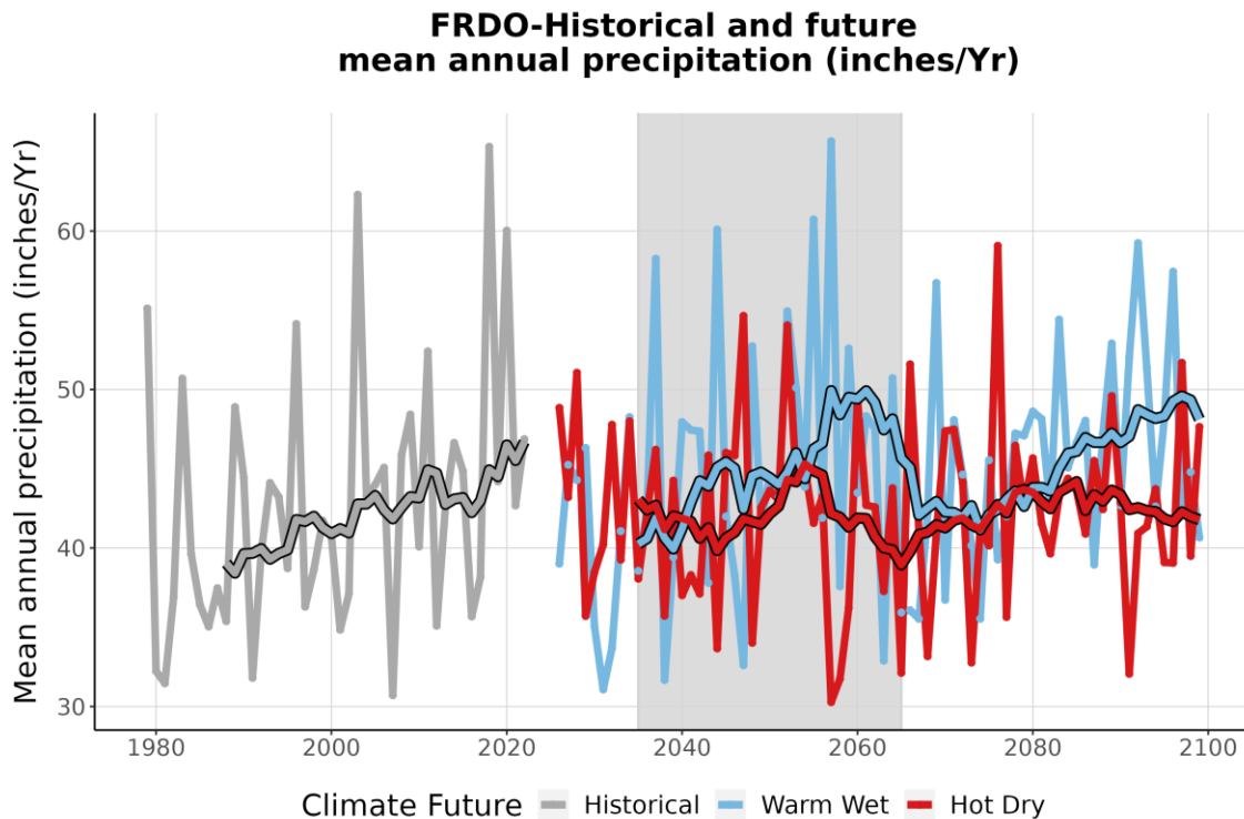
Figure 4. This graph compares observed average annual precipitation at FRDO (inches/year) (1979-2022) with projected average annual precipitation for the two climate futures over the period 2023-2099. The historically observed data is shown in gray, the Warm Wet climate future in blue, and the Hot Dry climate future in red. The smooth line running through each projection is the 10-year running average for historical observations and future projections. The gray-shaded area represents the time period that was averaged (2035-2065) to summarize future projections for the year 2050 (Appendix 1).
