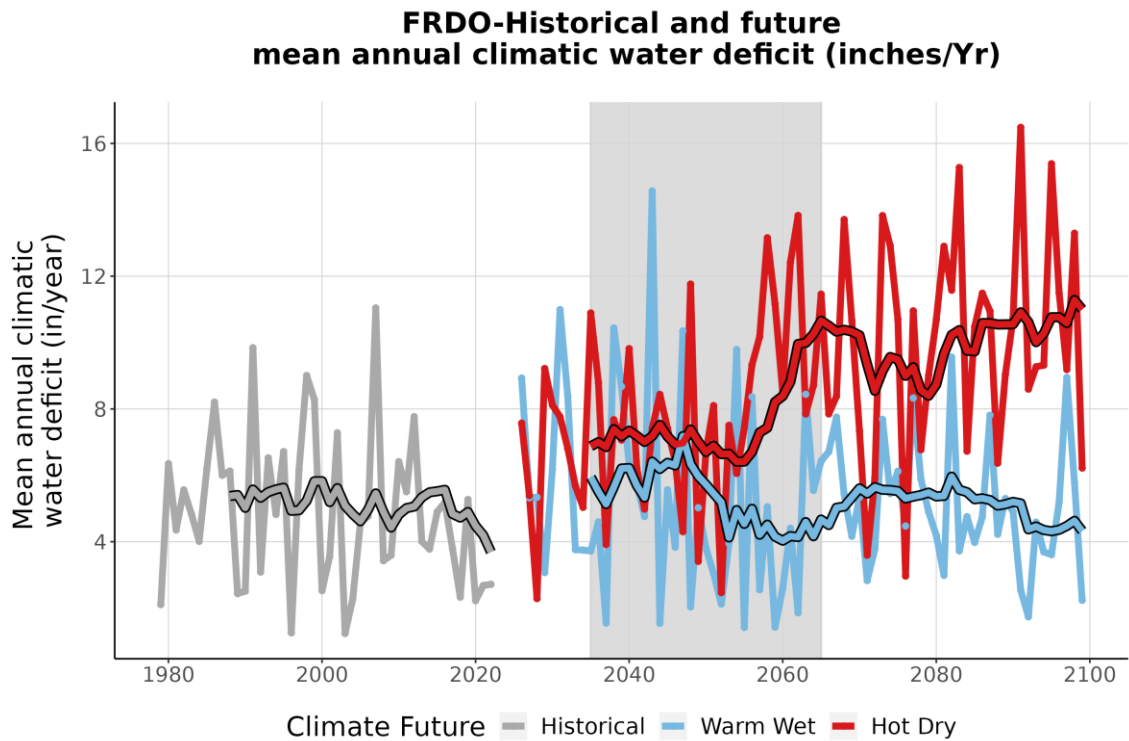
Figure 9. This line graph compares observed climatic water deficit at FRDO (inches/year) (1979-2022) with projected climatic water deficit for the two climate futures over the period 2023-2099. The historical observation data is shown in gray, the Warm Wet climate future in blue, and the Hot Dry climate future in red. The smooth line running through each projection is the 10-year running average for historical observations and future projections. Gray-shaded area represents the time period that was averaged (2035-2065) to summarize future projections for the year 2050.
