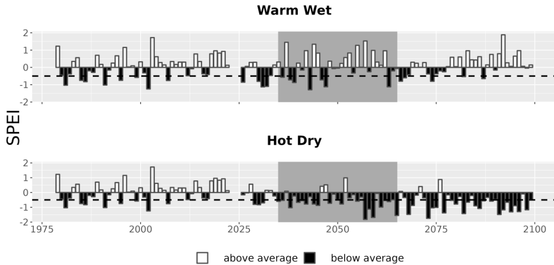
Figure 7. Drought metrics for FRDO. Drought index (SPEI; units = standard deviations from historical) timeseries for each climate future. Below-average SPEI (black bars) indicates dry conditions. The dotted line (SPEI = -0.5) indicates drought conditions.
