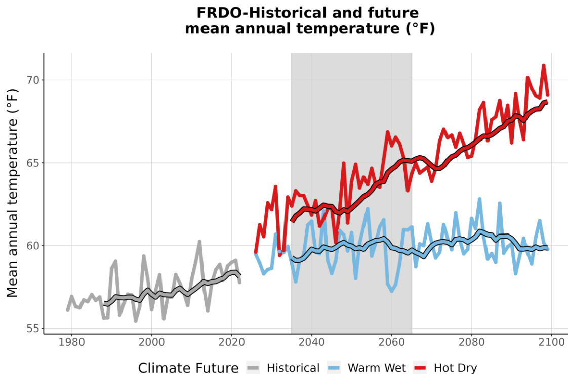
Figure 3. This graph compares observed average annual temperature at FRDO (°F) (1979-2022) with projected average annual temperature for the two climate futures over the period 2023-2099. The historically observed data
