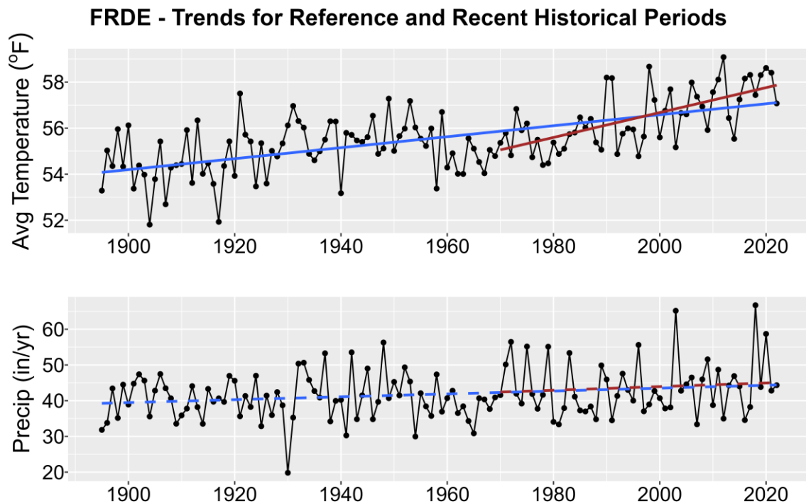
Figure 1. Historical trends in annual average temperature (upper plot) and annual total precipitation (lower plot) for FRDE from 1895-2022. Black points show yearly values while blue lines are linear regressions for the entire period record and red lines for 1970-2022 trends. Solid lines are significant trends (i.e., p < 0.05 ); dashed lines are not statistically significant.
