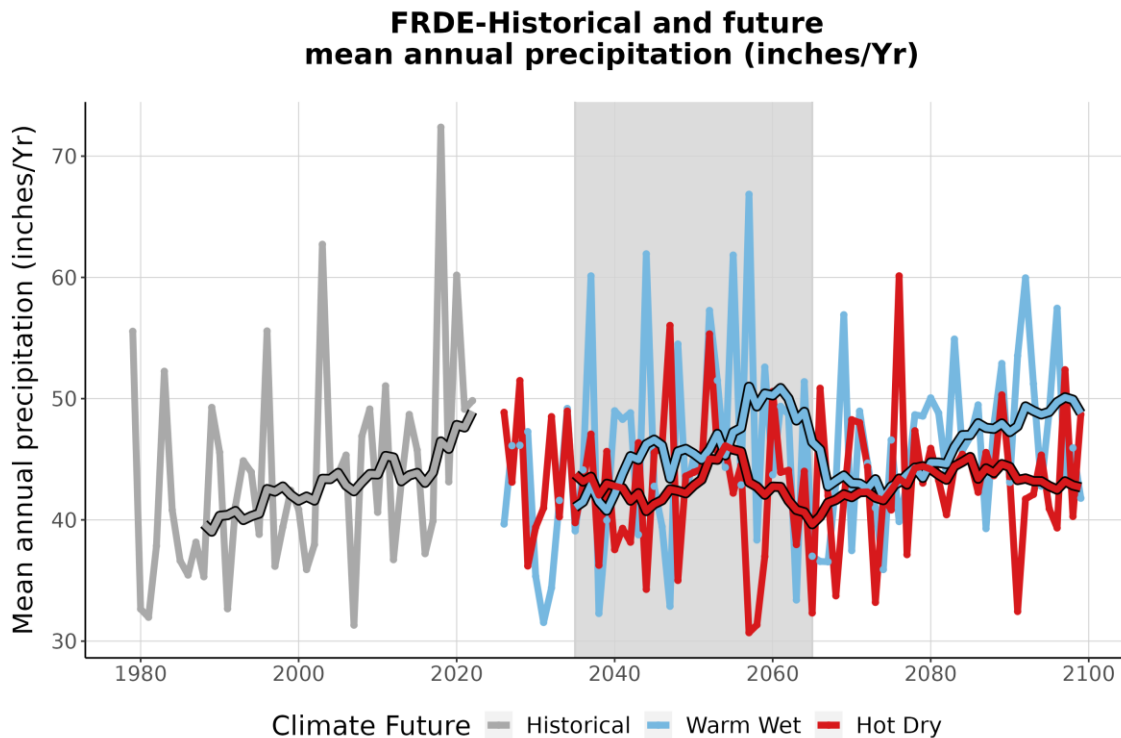
Figure 4. This graph compares observed average annual precipitation at FRDE (inches/year) (1979-2022) with projected average annual precipitation for the two climate futures over the period 2023-2099. The historically observed data is shown in gray, the Warm Wet climate future in blue, and the Hot Dry climate future in red. The smooth line running through each projection is the 10-year running average for historical observations and future projections. The gray-shaded area represents the time period that was averaged (2035-2065) to summarize future projections for the year 2050 (Appendix 1).
