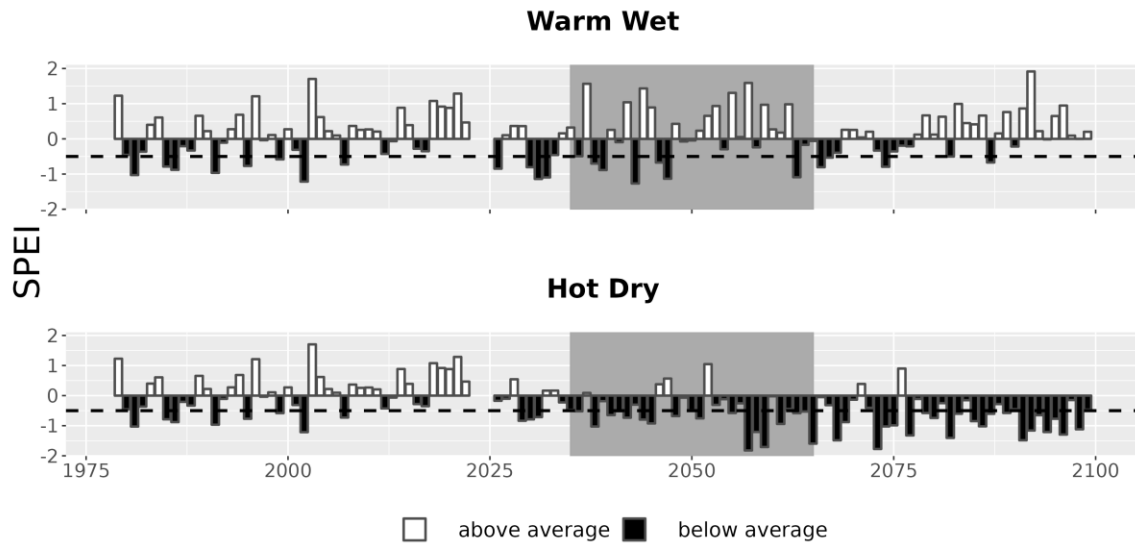
Figure 7. Drought metrics for FRDE. Drought index (SPEI; units = standard deviations from historical) timeseries for each climate future. Below-average SPEI (black bars) indicates dry conditions. The dotted line (SPEI = -0.5) indicates drought conditions.
