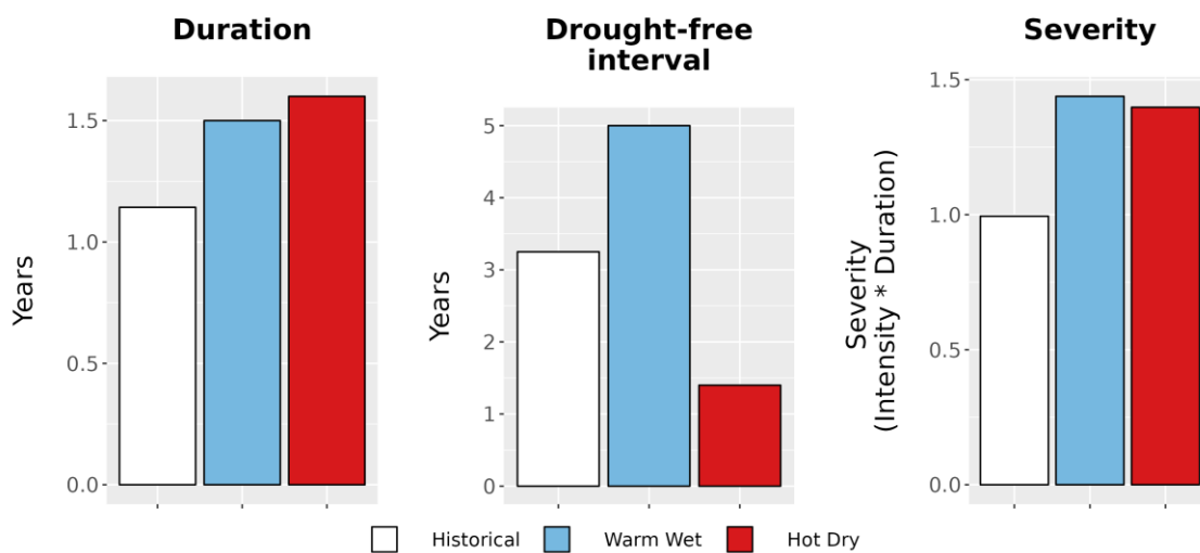
Figure 8. Drought metrics for FRDE. (Left) Average drought duration (years) historically (1979-2012) and under each climate future. (Middle) Average drought return interval (years), indicating the expected amount of time between periods of drought, historically and under each climate future. (Right) Average drought severity, a measure of drought intensity multiplied by duration, historically and under each climate future.
