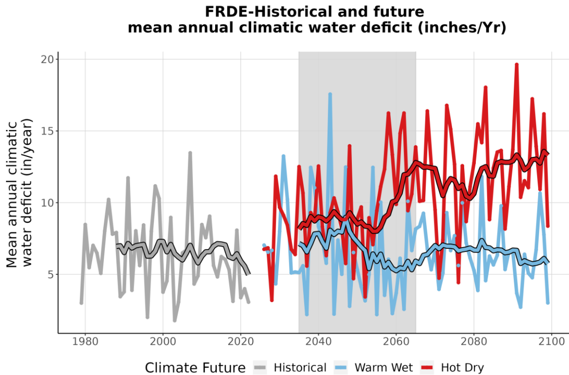
Figure 9. This line graph compares observed climatic water deficit at FRDE (inches/year) (1979-2022) with projected climatic water deficit for the two climate futures over the period 2023-2099. The historical observation data is shown in gray, the Warm Wet climate future in blue, and the Hot Dry climate future in red. The smooth line running through each projection is the 10-year running average for historical observations and future projections. Gray-shaded area represents the time period that was averaged (2035-2065) to summarize future projections for the year 2050.
