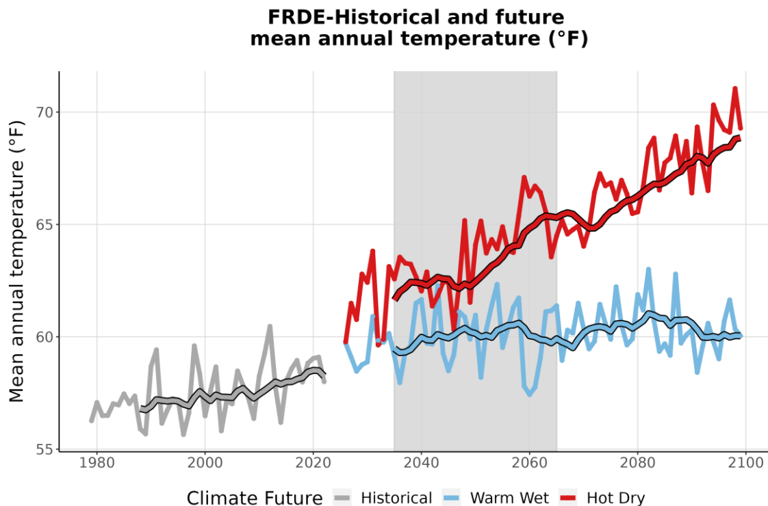
Figure 3. This graph compares observed average annual temperature at FRDE (°F) (1979-2022) with projected average annual temperature for the two climate futures over the period 2023-2099. The historically observed data
