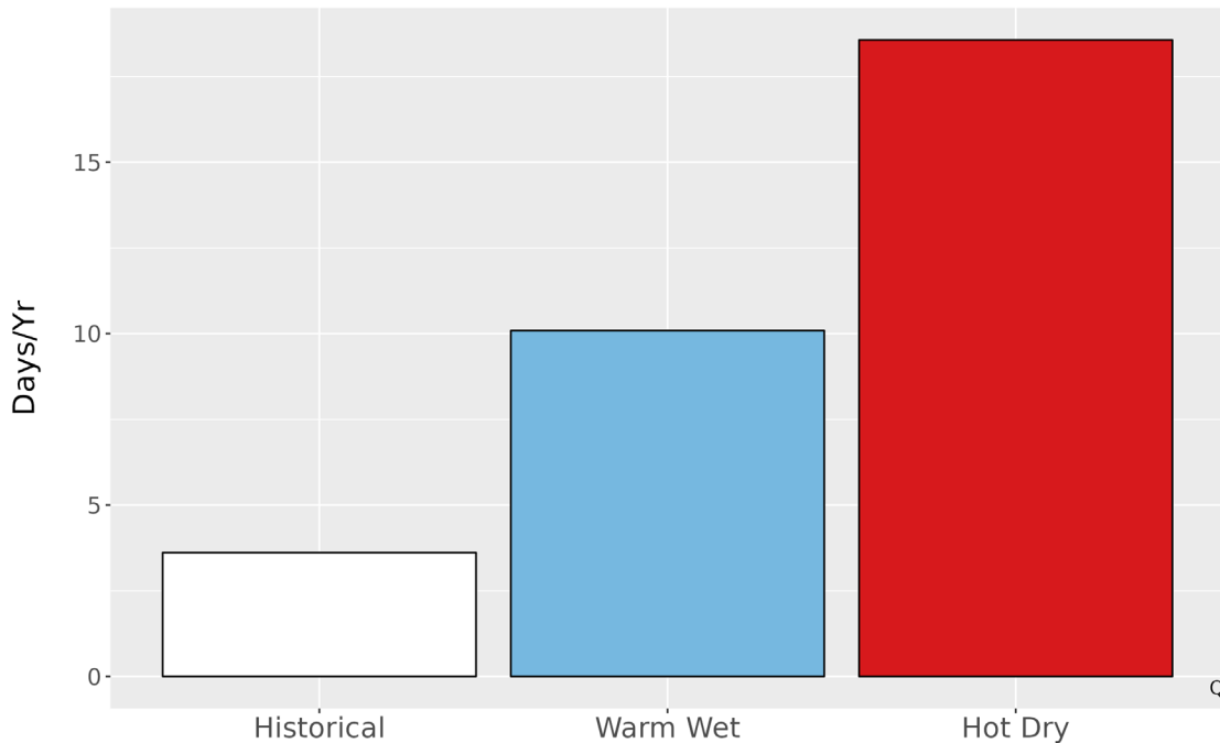
Figure 5. Metrics of extreme temperature at FOVA. The bar graph represents the average number of days annually with temperatures greater than the historical 99th percentile (91.5 °F) historically (1979-2012) and for the two climate futures (2050).
