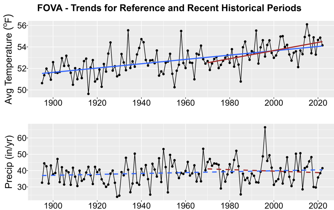
Figure 1. Historical trends in annual average temperature (upper plot) and annual total precipitation (lower plot) for FOVA from 1895-2022. Black points show yearly values while blue lines are linear regressions for the entire period record and red lines for 1970-2022 trends. Solid lines are significant trends (i.e., p < 0.05 ); dashed lines are not statistically significant.
