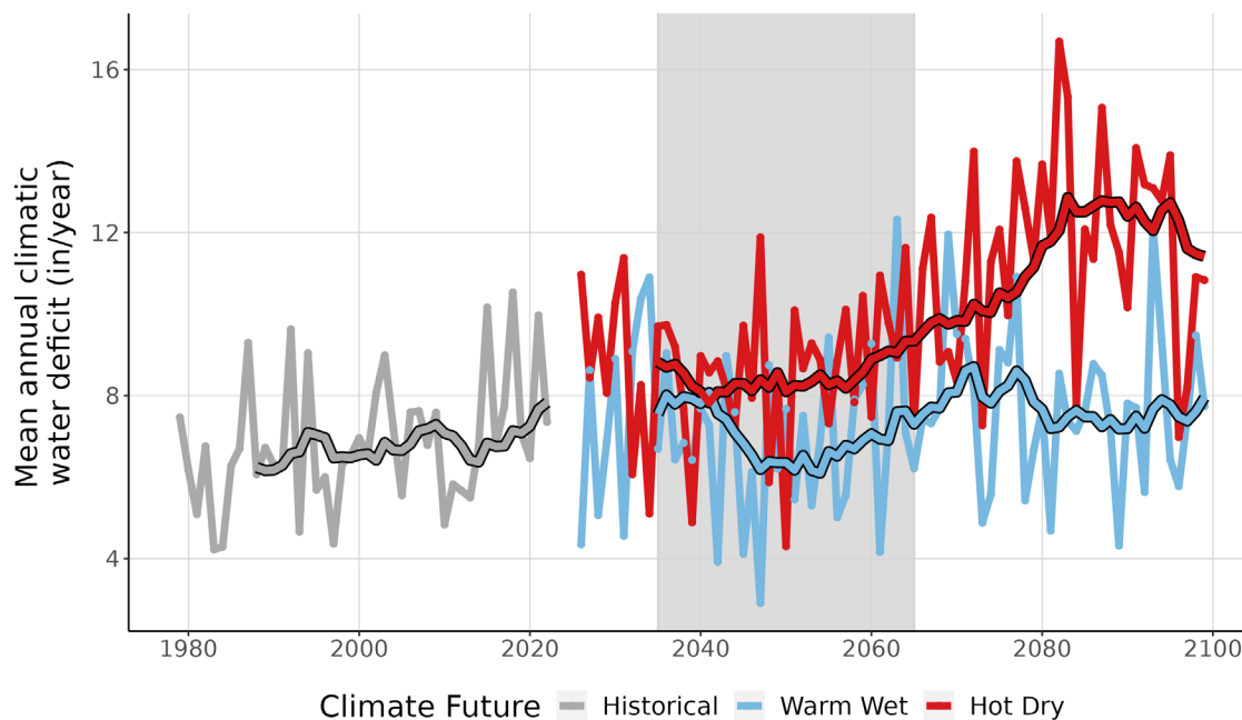
Figure 9. This line graph compares observed climatic water deficit at FOVA (inches/year) (1979-2022) with projected climatic water deficit for the two climate futures over the period 2023-2099. The historical observation data is shown in gray, the Warm Wet climate future in blue, and the Hot Dry climate future in red. The smooth line running through each projection is the 10-year running average for historical observations and future projections. Gray-shaded area represents the time period that was averaged (2035-2065) to summarize future projections for the year 2050.
