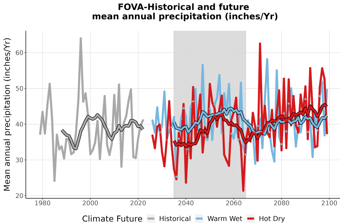
Figure 4. This graph compares observed average annual precipitation at FOVA (inches/year) (1979-2022) with projected average annual precipitation for the two climate futures over the period 2023-2099. The historically observed data is shown in gray, the Warm Wet climate future in blue, and the Hot Dry climate future in red. The smooth line running through each projection is the 10-year running average for historical observations and future projections. The gray-shaded area represents the time period that was averaged (2035-2065) to summarize future projections for the year 2050 (Appendix 1).
