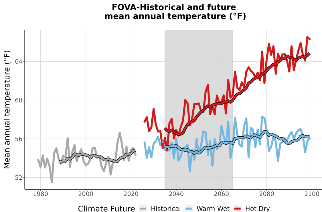
Figure 3. This graph compares observed average annual temperature at FOVA (°F) (1979-2022) with projected average annual temperature for the two climate futures over the period 2023-2099. The historically observed data
