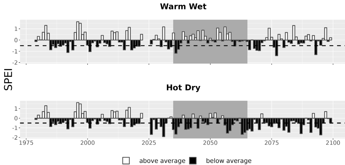
Figure 7. Drought metrics for FOVA. Drought index (SPEI; units = standard deviations from historical) timeseries for each climate future. Below-average SPEI (black bars) indicates dry conditions. The dotted line (SPEI = -0.5) indicates drought conditions.
