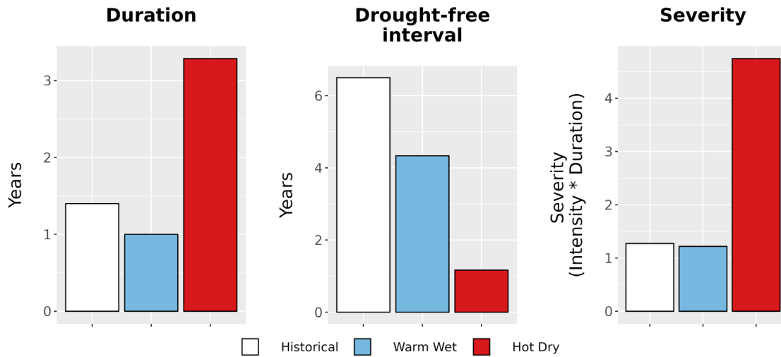
Figure 8. Drought metrics for FOUS. (Left) Average drought duration (years) historically (1979-2012) and under each climate future. (Middle) Average drought return interval (years), indicating the expected amount of time between periods of drought, historically and under each climate future. (Right) Average drought severity, a measure of drought intensity multiplied by duration, historically and under each climate future.
