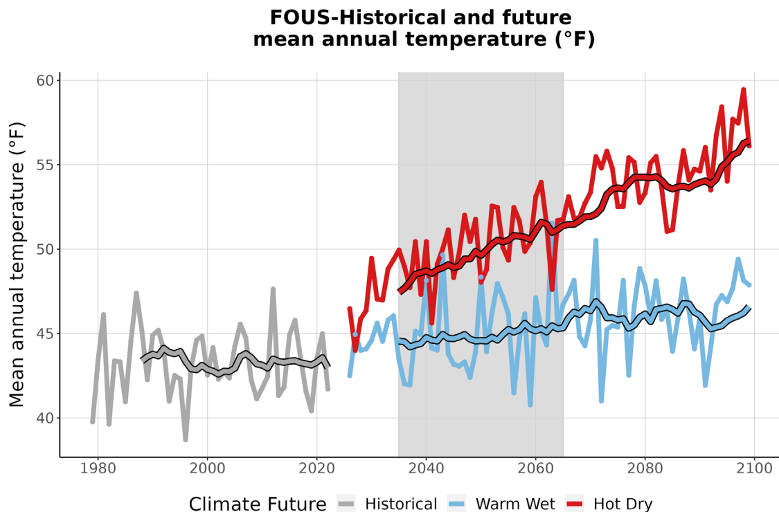
Figure 3. This graph compares observed average annual temperature at FOUS (°F) (1979-2022) with projected average annual temperature for the two climate futures over the period 2023-2099. The historically observed data
