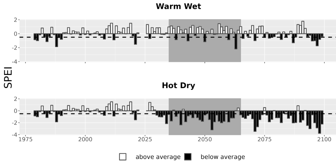
Figure 7. Drought metrics for FOUS. Drought index (SPEI; units = standard deviations from historical) timeseries for each climate future. Below-average SPEI (black bars) indicates dry conditions. The dotted line (SPEI = -0.5) indicates drought conditions.
