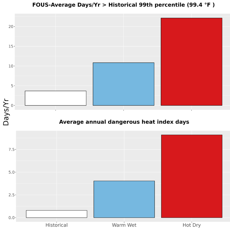
Figure 5. The upper bar graph represents the average number of days annually with temperatures greater than the historical 99th percentile (99.4 °F) historically (1979-2012) and for the two climate futures (2050). The bottom bar graph represents the average annual number of dangerous heat index days historically and for the two climate futures. Dangerous heat index days are days that exceed 105 °F.
