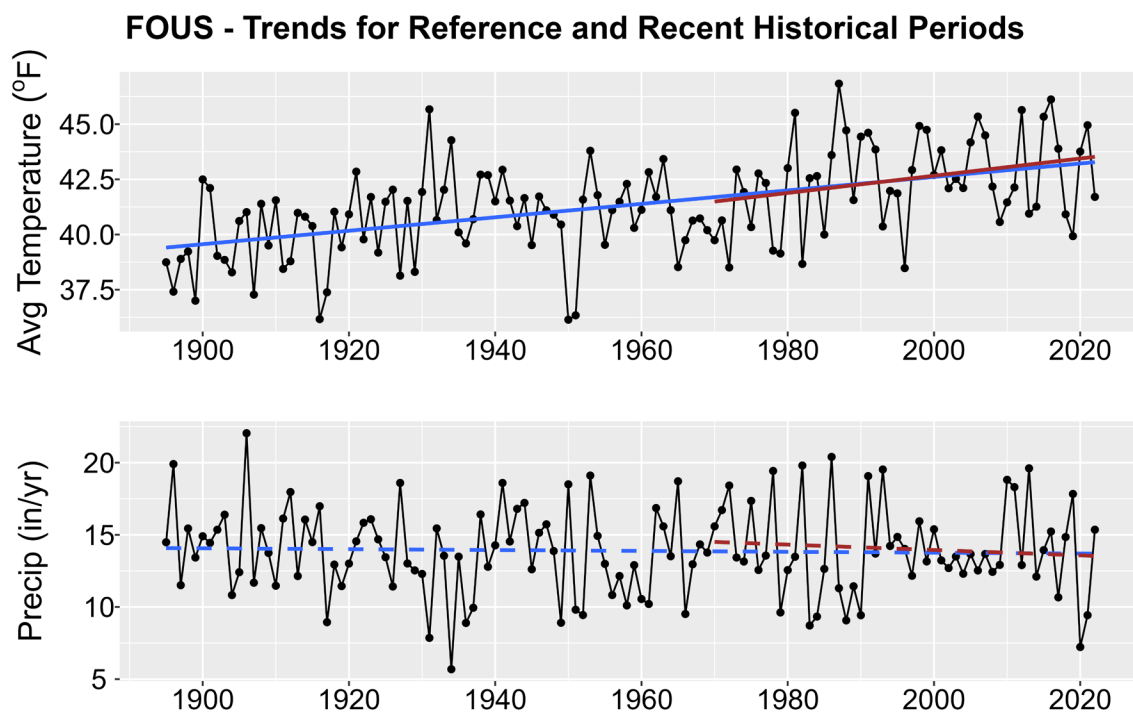
Figure 1. Historical trends in annual average temperature (upper plot) and annual total precipitation (lower plot) for FOUS from 1895-2022. Black points show yearly values while blue lines are linear regressions for the entire period record and red lines for 1970-2022 trends. Solid lines are significant trends (i.e., p < 0.05 ); dashed lines are not statistically significant.
