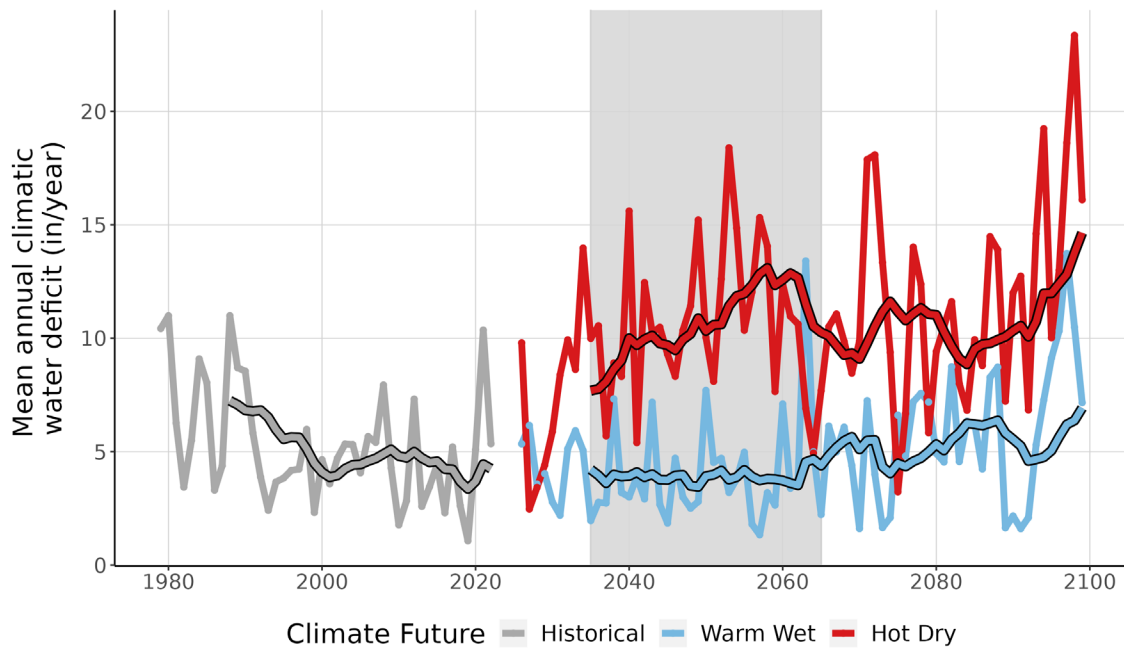
Figure 9. This line graph compares observed climatic water deficit at FOUS (inches/year) (1979-2022) with projected climatic water deficit for the two climate futures over the period 2023-2099. The historical observation data is shown in gray, the Warm Wet climate future in blue, and the Hot Dry climate future in red. The smooth line running through each projection is the 10-year running average for historical observations and future projections. Gray-shaded area represents the time period that was averaged (2035-2065) to summarize future projections for the year 2050.
