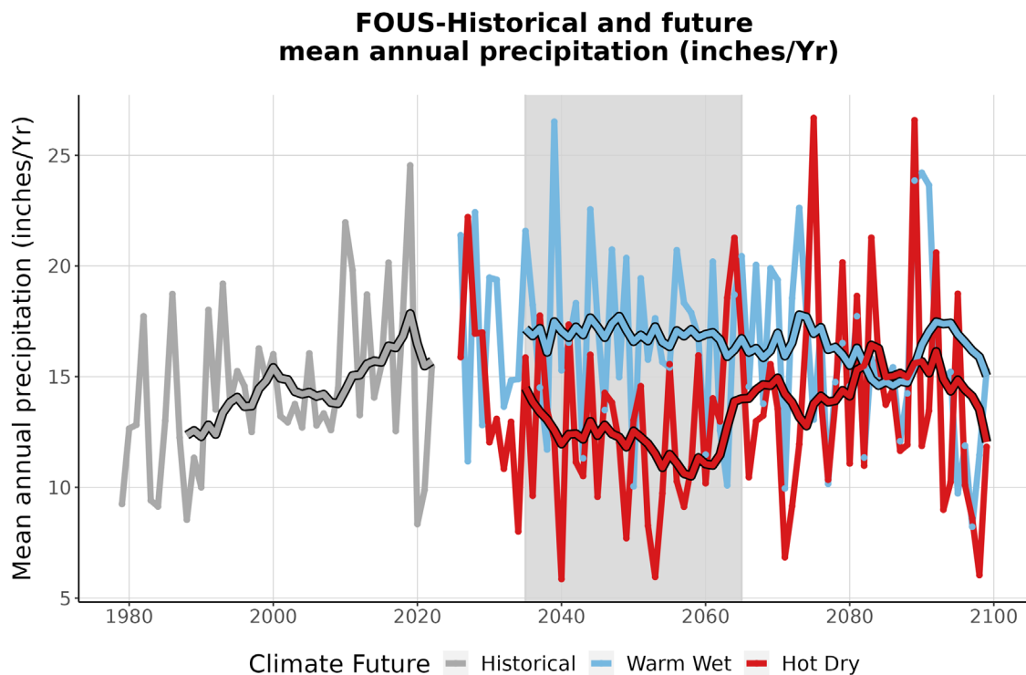
Figure 4. This graph compares observed average annual precipitation at FOUS (inches/year) (1979-2022) with projected average annual precipitation for the two climate futures over the period 2023-2099. The historically observed data is shown in gray, the Warm Wet climate future in blue, and the Hot Dry climate future in red. The smooth line running through each projection is the 10-year running average for historical observations and future projections. The gray-shaded area represents the time period that was averaged (2035-2065) to summarize future projections for the year 2050 (Appendix 1).
