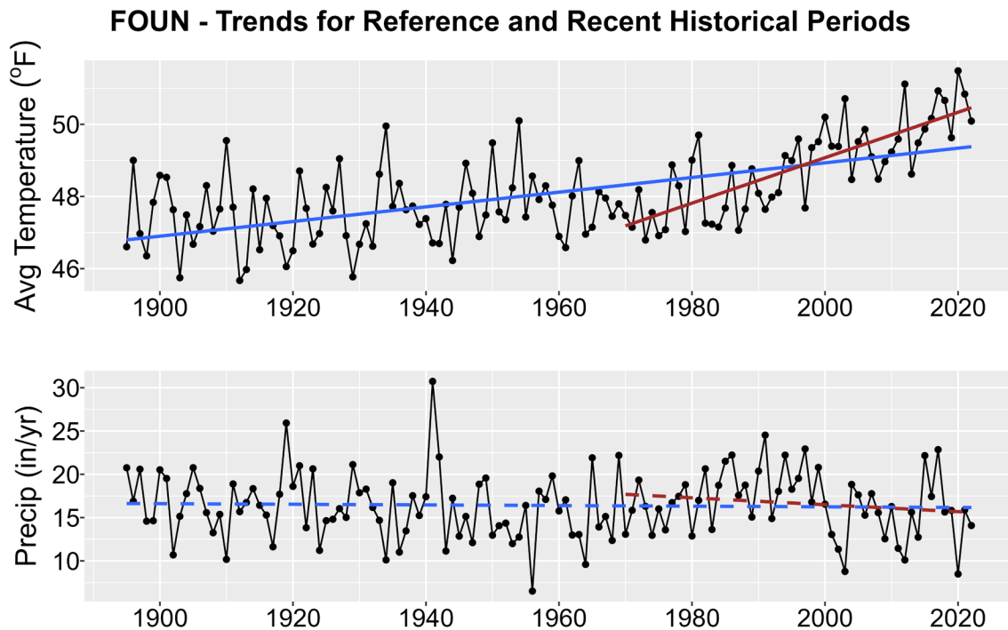
Figure 1. Historical trends in annual average temperature (upper plot) and annual total precipitation (lower plot) for FOUN from 1895-2022. Black points show yearly values while blue lines are linear regressions for the entire period record and red lines for 1970-2022 trends. Solid lines are significant trends (i.e., p < 0.05 ); dashed lines are not statistically significant.
