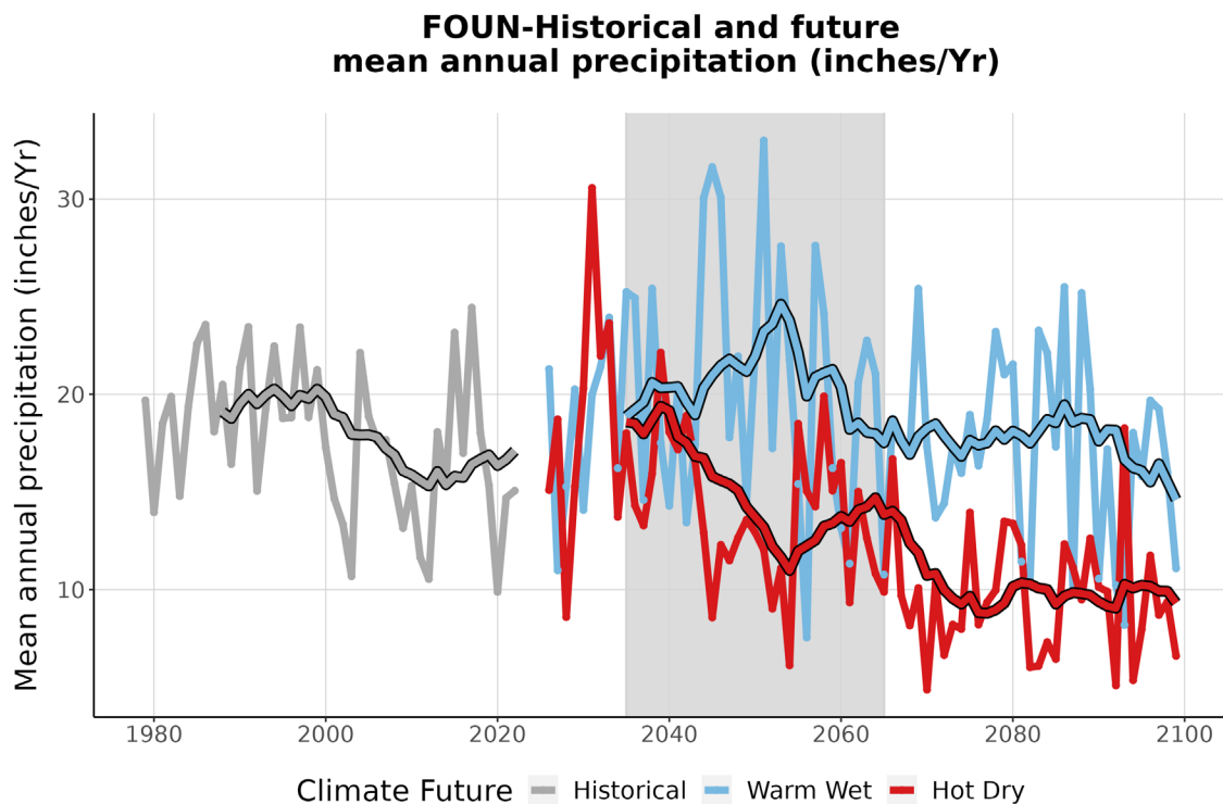
Figure 4. This graph compares observed average annual precipitation at FOUN (inches/year) (1979-2022) with projected average annual precipitation for the two climate futures over the period 2023-2099. The historically observed data is shown in gray, the Warm Wet climate future in blue, and the Hot Dry climate future in red. The smooth line running through each projection is the 10-year running average for historical observations and future projections. The gray-shaded area represents the time period that was averaged (2035-2065) to summarize future projections for the year 2050 (Appendix 1).
