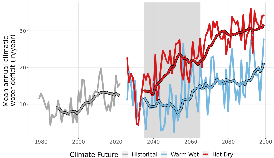
Figure 9. This line graph compares observed climatic water deficit at FOUN (inches/year) (1979-2022) with projected climatic water deficit for the two climate futures over the period 2023-2099. The historical observation data is shown in gray, the Warm Wet climate future in blue, and the Hot Dry climate future in red. The smooth line running through each projection is the 10-year running average for historical observations and future projections. Gray-shaded area represents the time period that was averaged (2035-2065) to summarize future projections for the year 2050.
