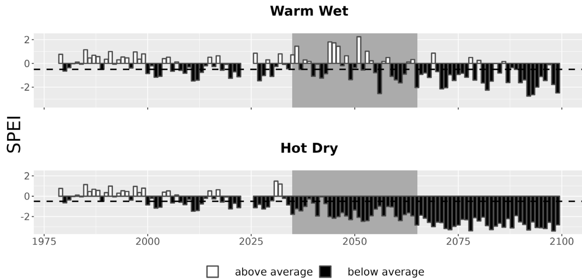
Figure 7. Drought metrics for FOUN. Drought index (SPEI; units = standard deviations from historical) timeseries for each climate future. Below-average SPEI (black bars) indicates dry conditions. The dotted line (SPEI = -0.5) indicates drought conditions.
