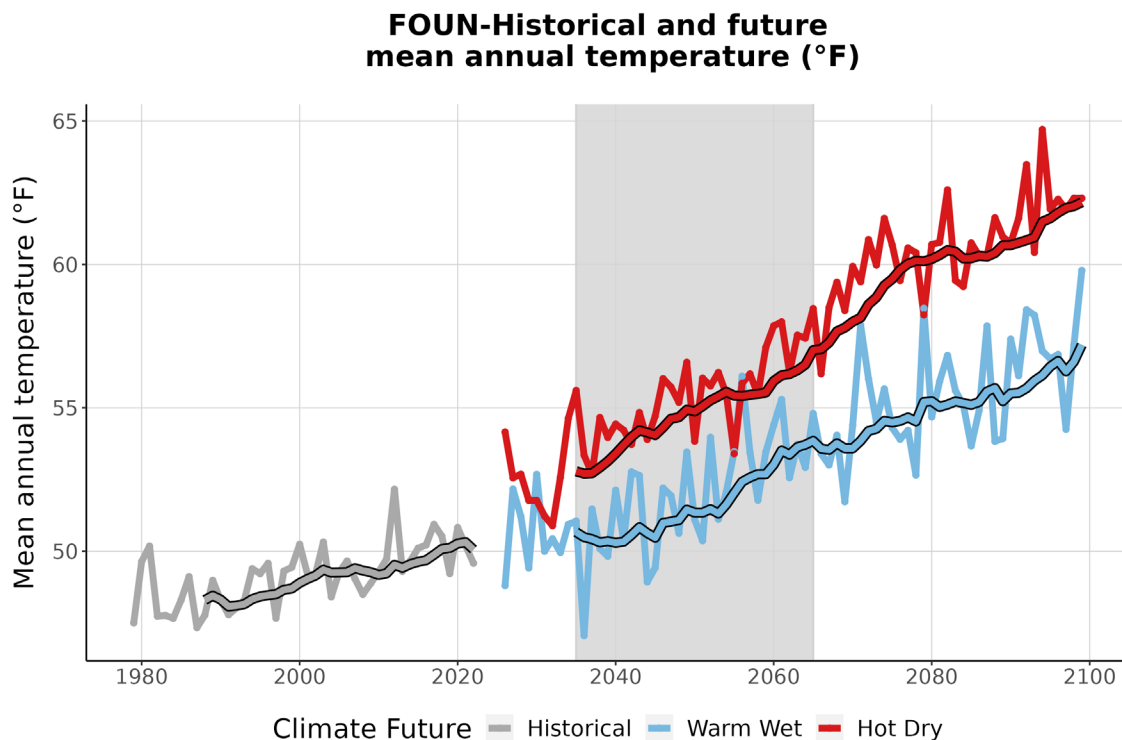
Figure 3. This graph compares observed average annual temperature at FOUN (°F) (1979-2022) with projected average annual temperature for the two climate futures over the period 2023-2099. The historically observed data
