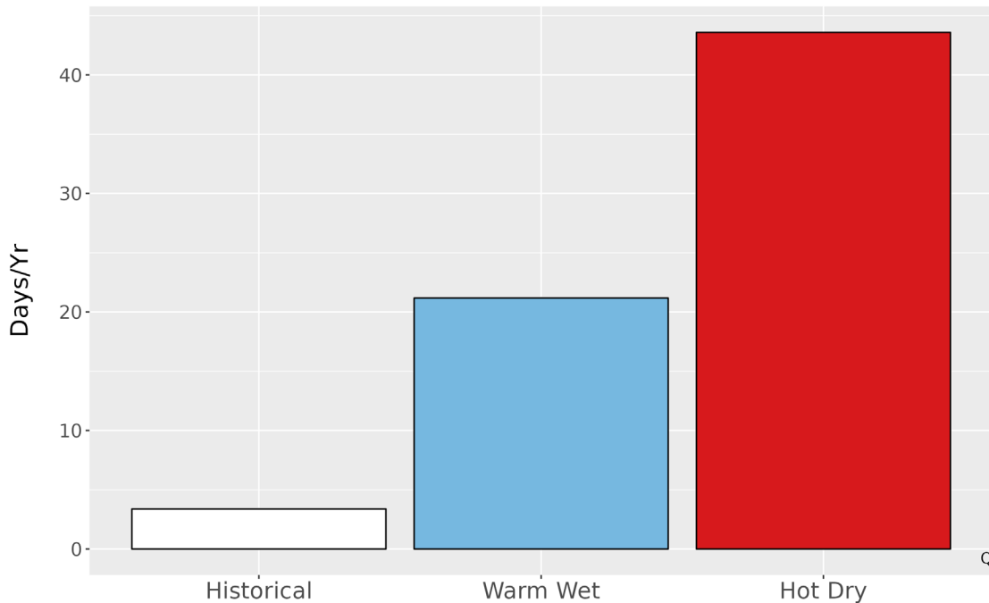
Figure 5. Metrics of extreme temperature at FOUN. The bar graph represents the average number of days annually with temperatures greater than the historical 99th percentile (90.2 °F) historically (1979-2012) and for the two climate futures (2050).
