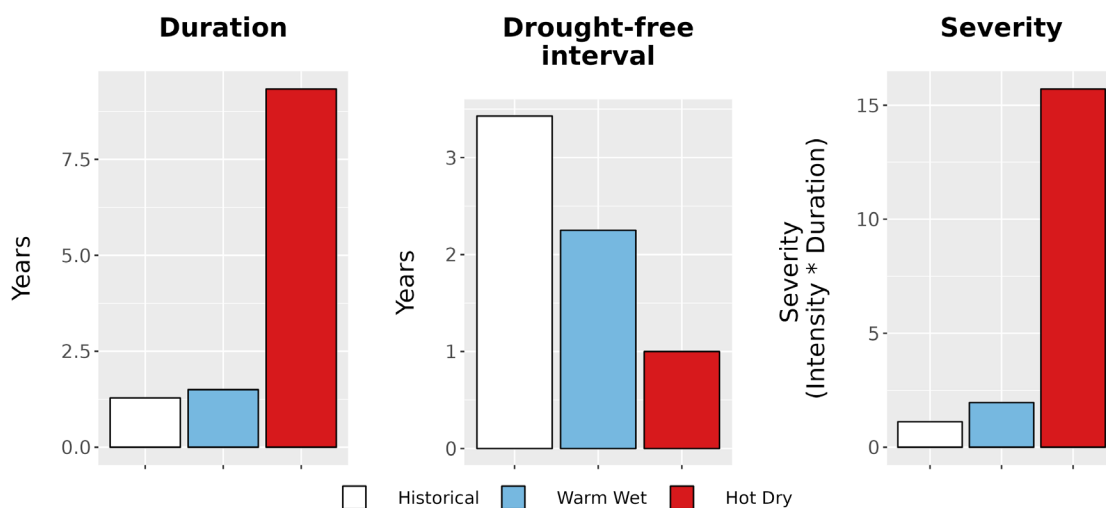
Figure 8. Drought metrics for FOUN. (Left) Average drought duration (years) historically (1979-2012) and under each climate future. (Middle) Average drought return interval (years), indicating the expected amount of time between periods of drought, historically and under each climate future. (Right) Average drought severity, a measure of drought intensity multiplied by duration, historically and under each climate future.
