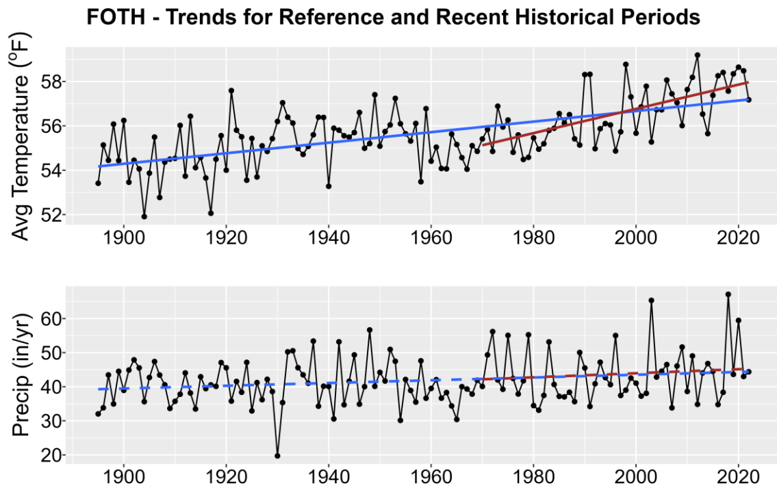
Figure 1. Historical trends in annual average temperature (upper plot) and annual total precipitation (lower plot) for FOTH from 1895-2022. Black points show yearly values while blue lines are linear regressions for the entire period record and red lines for 1970-2022 trends. Solid lines are significant trends (i.e., p < 0.05 ); dashed lines are not statistically significant.
