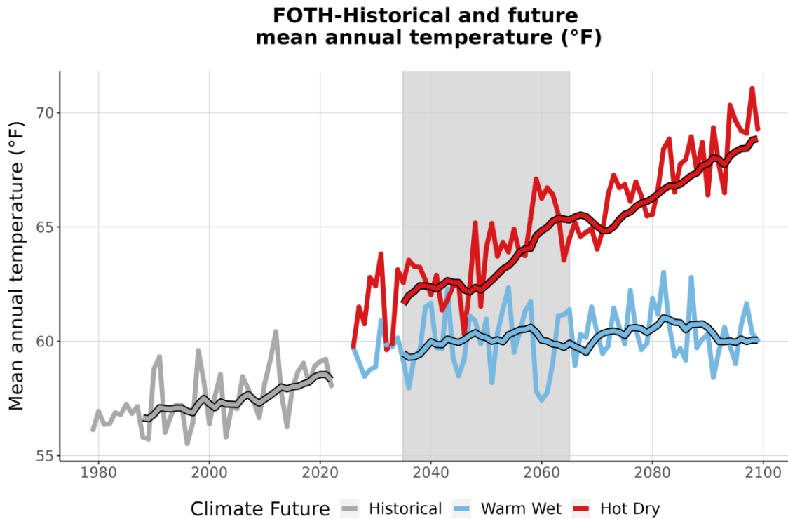
Figure 3. This graph compares observed average annual temperature at FOTH (°F) (1979-2022) with projected average annual temperature for the two climate futures over the period 2023-2099. The historically observed data
