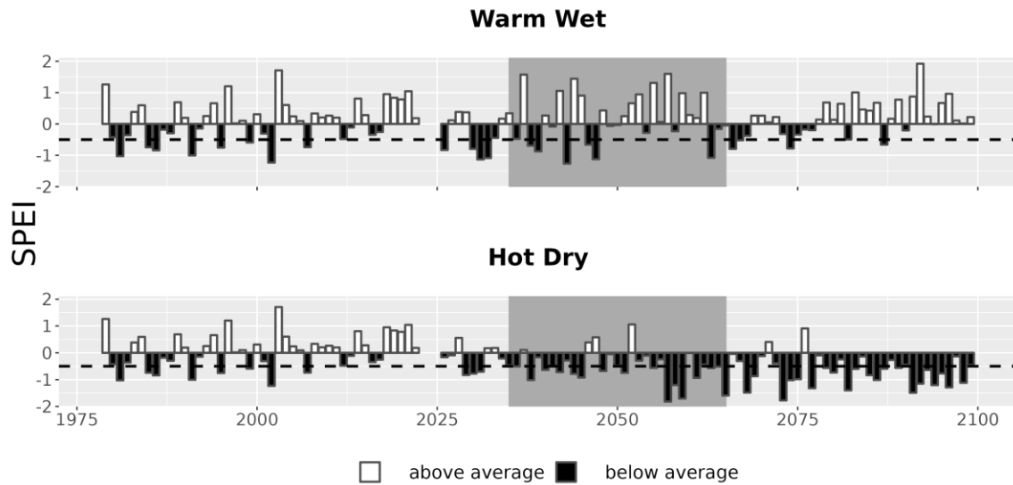
Figure 7. Drought metrics for FOTH. Drought index (SPEI; units = standard deviations from historical) timeseries for each climate future. Below-average SPEI (black bars) indicates dry conditions. The dotted line (SPEI = -0.5) indicates drought conditions.
