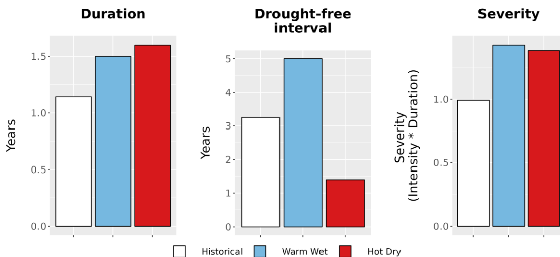
Figure 8. Drought metrics for FOTH. (Left) Average drought duration (years) historically (1979-2012) and under each climate future. (Middle) Average drought return interval (years), indicating the expected amount of time between periods of drought, historically and under each climate future. (Right) Average drought severity, a measure of drought intensity multiplied by duration, historically and under each climate future.
