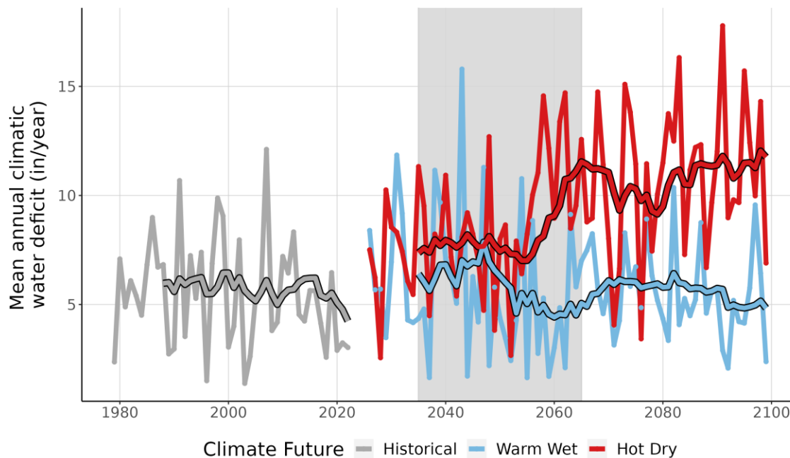
Figure 9. This line graph compares observed climatic water deficit at FOTH (inches/year) (1979-2022) with projected climatic water deficit for the two climate futures over the period 2023-2099. The historical observation data is shown in gray, the Warm Wet climate future in blue, and the Hot Dry climate future in red. The smooth line running through each projection is the 10-year running average for historical observations and future projections. Gray-shaded area represents the time period that was averaged (2035-2065) to summarize future projections for the year 2050.
