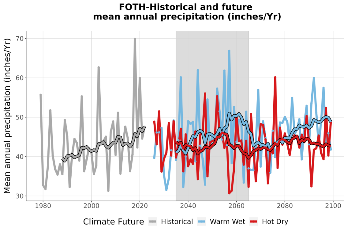
Figure 4. This graph compares observed average annual precipitation at FOTH (inches/year) (1979-2022) with projected average annual precipitation for the two climate futures over the period 2023-2099. The historically observed data is shown in gray, the Warm Wet climate future in blue, and the Hot Dry climate future in red. The smooth line running through each projection is the 10-year running average for historical observations and future projections. The gray-shaded area represents the time period that was averaged (2035-2065) to summarize future projections for the year 2050 (Appendix 1).
