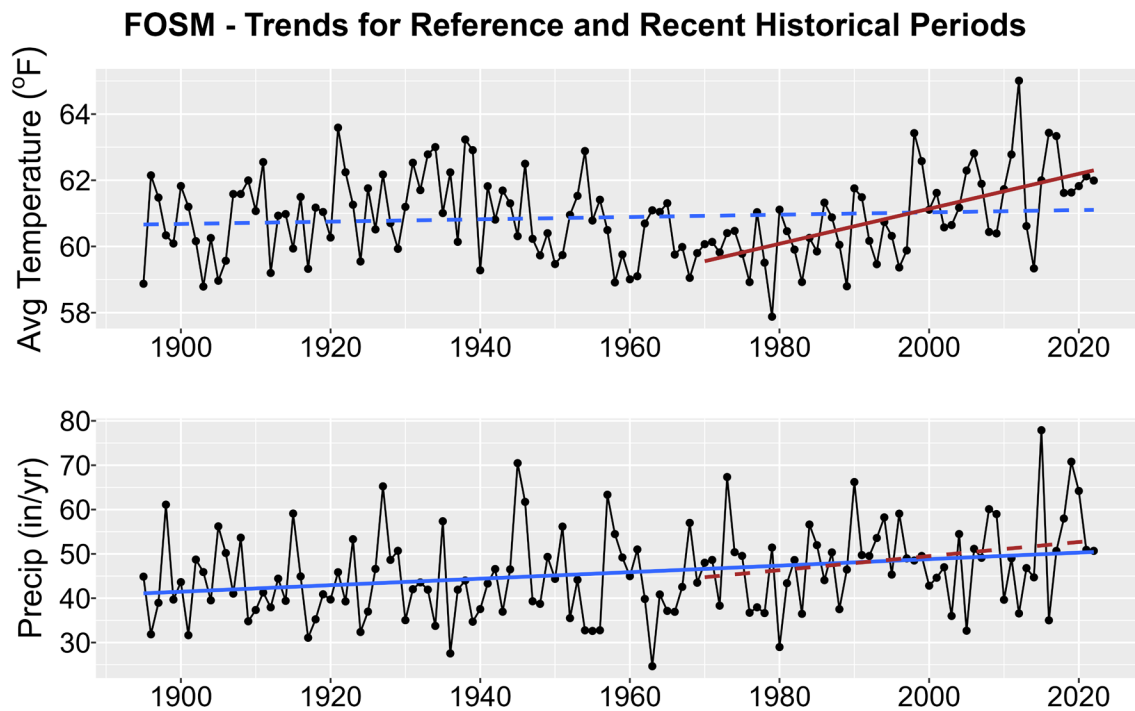
Figure 1. Historical trends in annual average temperature (upper plot) and annual total precipitation (lower plot) for FOSM from 1895-2022. Black points show yearly values while blue lines are linear regressions for the entire period record and red lines for 1970-2022 trends. Solid lines are significant trends (i.e., p < 0.05 ); dashed lines are not statistically significant.
