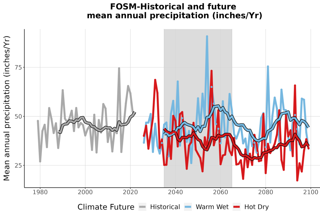
Figure 4. This graph compares observed average annual precipitation at FOSM (inches/year) (1979-2022) with projected average annual precipitation for the two climate futures over the period 2023-2099. The historically observed data is shown in gray, the Warm Wet climate future in blue, and the Hot Dry climate future in red. The smooth line running through each projection is the 10-year running average for historical observations and future projections. The gray-shaded area represents the time period that was averaged (2035-2065) to summarize future projections for the year 2050 (Appendix 1).
