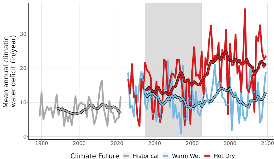
Figure 9. This line graph compares observed climatic water deficit at FOSM (inches/year) (1979-2022) with projected climatic water deficit for the two climate futures over the period 2023-2099. The historical observation data is shown in gray, the Warm Wet climate future in blue, and the Hot Dry climate future in red. The smooth line running through each projection is the 10-year running average for historical observations and future projections. Gray-shaded area represents the time period that was averaged (2035-2065) to summarize future projections for the year 2050.
