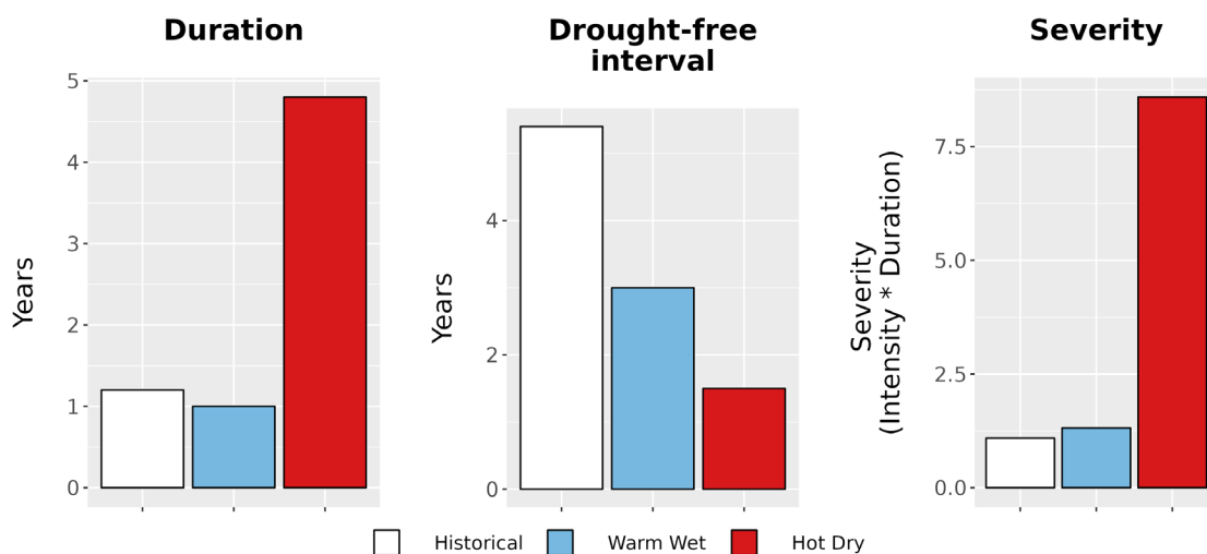
Figure 8. Drought metrics for FOSM. (Left) Average drought duration (years) historically (1979-2012) and under each climate future. (Middle) Average drought return interval (years), indicating the expected amount of time between periods of drought, historically and under each climate future. (Right) Average drought severity, a measure of drought intensity multiplied by duration, historically and under each climate future.
