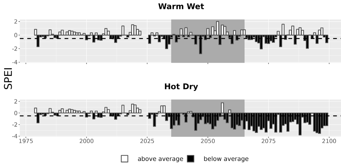
Figure 7. Drought metrics for FOSM. Drought index (SPEI; units = standard deviations from historical) timeseries for each climate future. Below-average SPEI (black bars) indicates dry conditions. The dotted line (SPEI = -0.5) indicates drought conditions.
