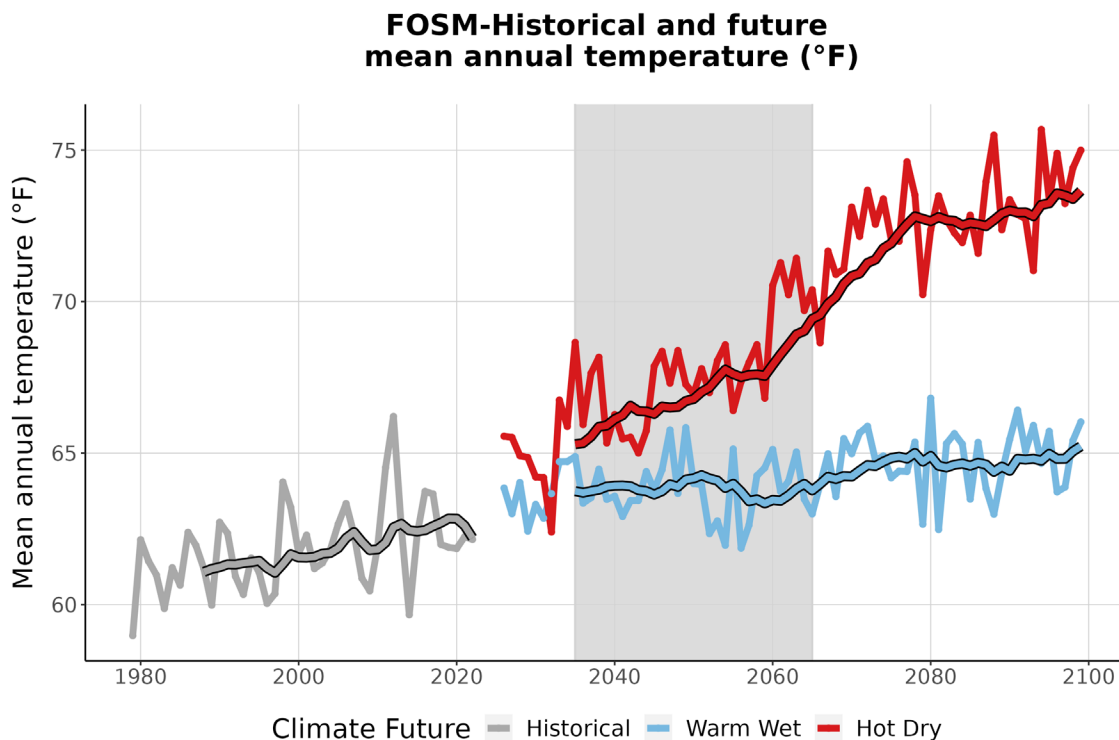
Figure 3. This graph compares observed average annual temperature at FOSM (°F) (1979-2022) with projected average annual temperature for the two climate futures over the period 2023-2099. The historically observed data
