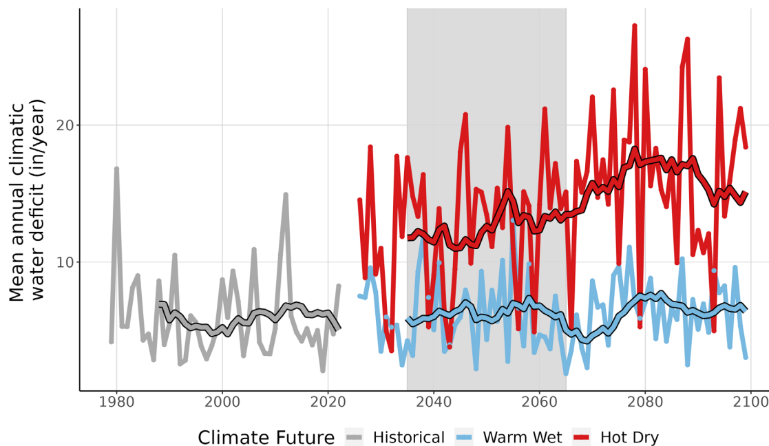
Figure 9. This line graph compares observed climatic water deficit at FOSC (inches/year) (1979-2022) with projected climatic water deficit for the two climate futures over the period 2023-2099. The historical observation data is shown in gray, the Warm Wet climate future in blue, and the Hot Dry climate future in red. The smooth line running through each projection is the 10-year running average for historical observations and future projections. Gray-shaded area represents the time period that was averaged (2035-2065) to summarize future projections for the year 2050.
