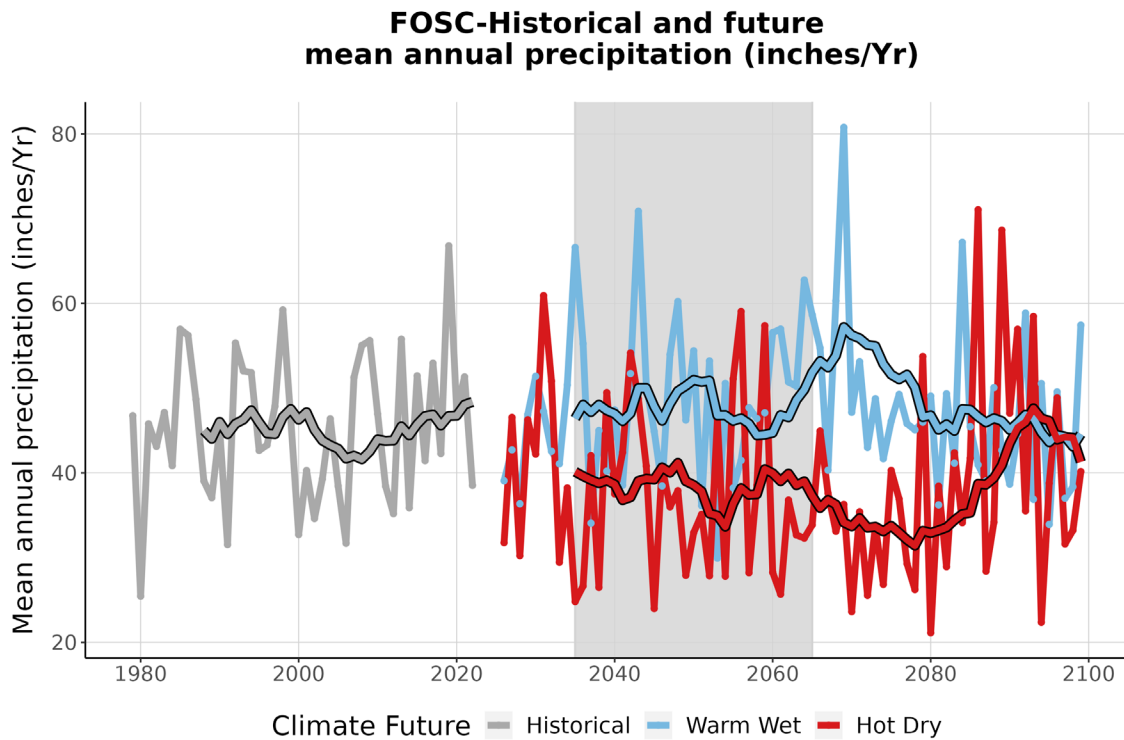
Figure 4. This graph compares observed average annual precipitation at FOSC (inches/year) (1979-2022) with projected average annual precipitation for the two climate futures over the period 2023-2099. The historically observed data is shown in gray, the Warm Wet climate future in blue, and the Hot Dry climate future in red. The smooth line running through each projection is the 10-year running average for historical observations and future projections. The gray-shaded area represents the time period that was averaged (2035-2065) to summarize future projections for the year 2050 (Appendix 1).
