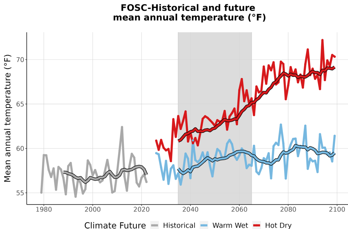
Figure 3. This graph compares observed average annual temperature at FOSC (°F) (1979-2022) with projected average annual temperature for the two climate futures over the period 2023-2099. The historically observed data
