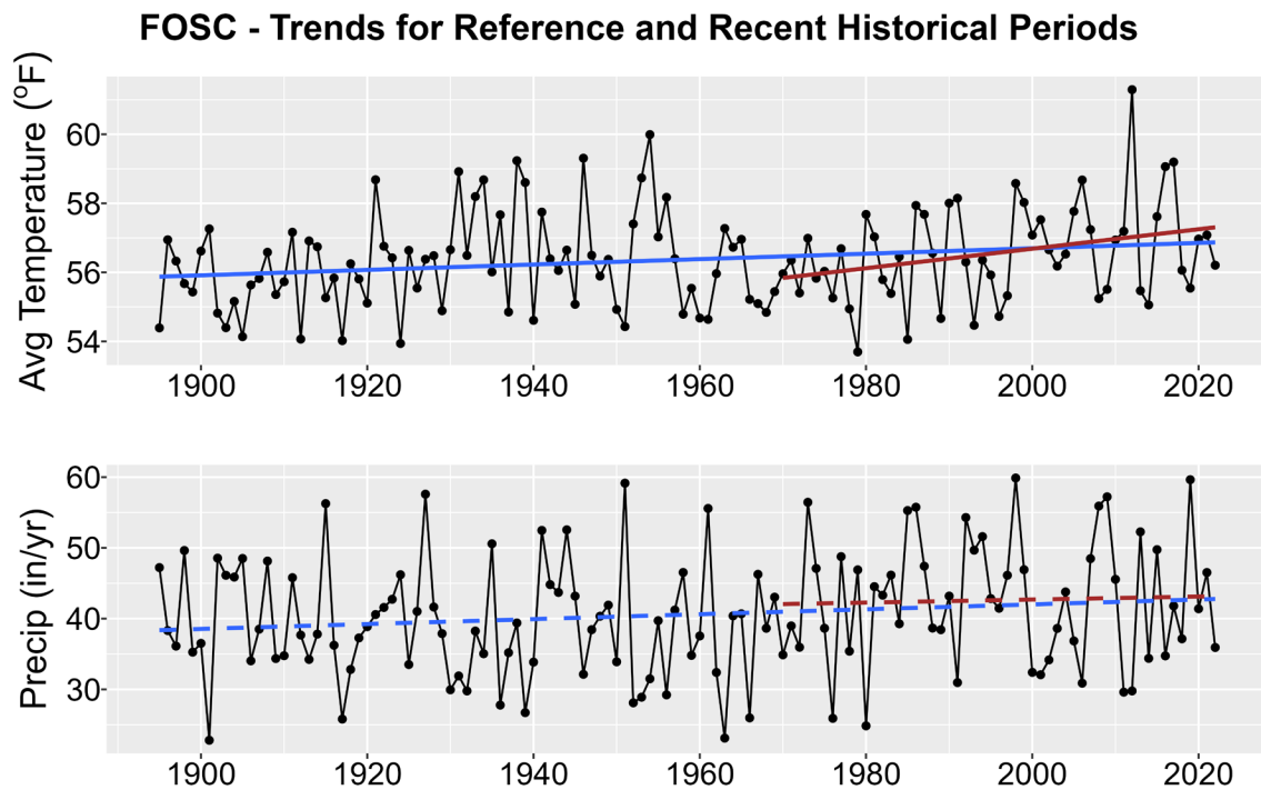
Figure 1. Historical trends in annual average temperature (upper plot) and annual total precipitation (lower plot) for FOSC from 1895-2022. Black points show yearly values while blue lines are linear regressions for the entire period record and red lines for 1970-2022 trends. Solid lines are significant trends (i.e., p < 0.05 ); dashed lines are not statistically significant.
