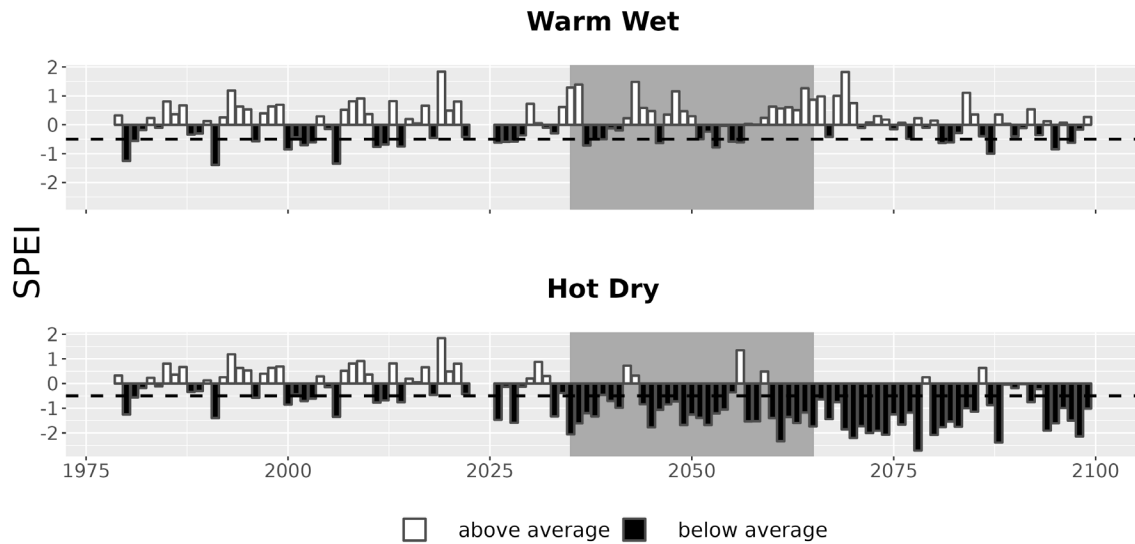
Figure 7. Drought metrics for FOSC. Drought index (SPEI; units = standard deviations from historical) timeseries for each climate future. Below-average SPEI (black bars) indicates dry conditions. The dotted line (SPEI = -0.5) indicates drought conditions.
