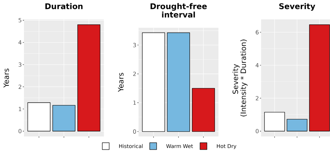
Figure 8. Drought metrics for FOSC. (Left) Average drought duration (years) historically (1979-2012) and under each climate future. (Middle) Average drought return interval (years), indicating the expected amount of time between periods of drought, historically and under each climate future. (Right) Average drought severity, a measure of drought intensity multiplied by duration, historically and under each climate future.
