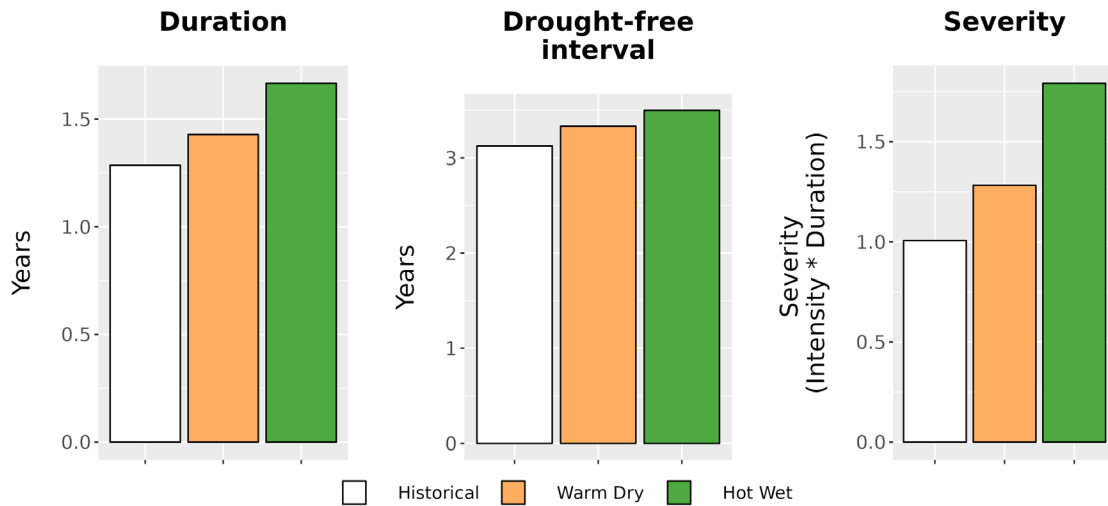
Figure 8. Drought metrics for FONE. (Left) Average drought duration (years) historically (1979-2012) and under each climate future. (Middle) Average drought return interval (years), indicating the expected amount of time between periods of drought, historically and under each climate future. (Right) Average drought severity, a measure of drought intensity multiplied by duration, historically and under each climate future.
