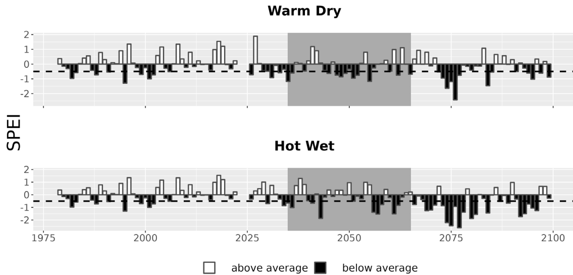
Figure 7. Drought metrics for FONE. Drought index (SPEI; units = standard deviations from historical) timeseries for each climate future. Below-average SPEI (black bars) indicates dry conditions. The dotted line (SPEI = -0.5) indicates drought conditions.
