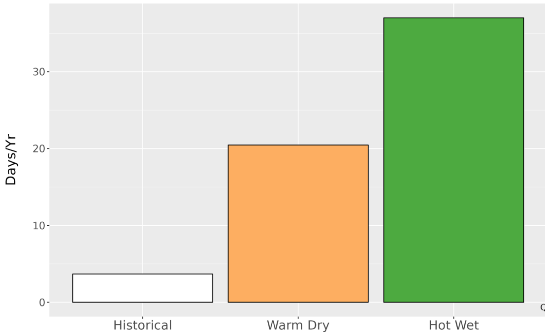
Figure 5. Metrics of extreme temperature at FONE. The bar graph represents the average number of days annually with temperatures greater than the historical 99th percentile (87.1 °F) historically (1979-2012) and for the two climate futures (2050).
