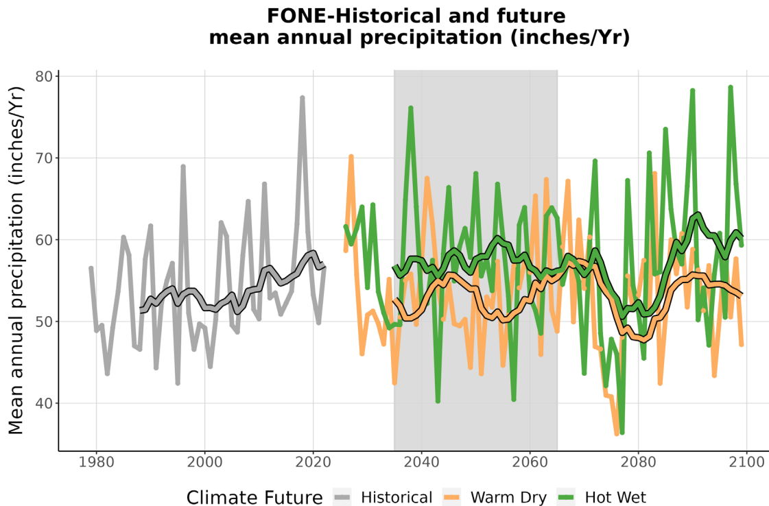
Figure 4. This graph compares observed average annual precipitation at FONE (inches/year) (1979-2022) with projected average annual precipitation for the two climate futures over the period 2023-2099. The historically observed data is shown in gray, the Warm Dry climate future in orange, and the Hot Wet climate future in green. The smooth line running through each projection is the 10-year running average for historical observations and future projections. The gray-shaded area represents the time period that was averaged (2035-2065) to summarize future projections for the year 2050 (Appendix 1).
