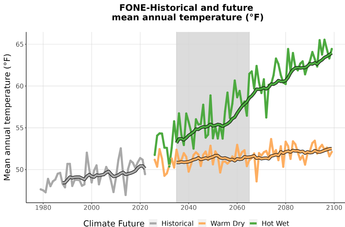
Figure 3. This graph compares observed average annual temperature at FONE (°F) (1979-2022) with projected average annual temperature for the two climate futures over the period 2023-2099. The historically observed data
