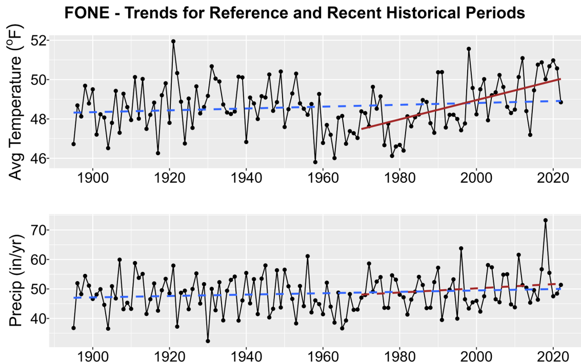
Figure 1. Historical trends in annual average temperature (upper plot) and annual total precipitation (lower plot) for FONE from 1895-2022. Black points show yearly values while blue lines are linear regressions for the entire period record and red lines for 1970-2022 trends. Solid lines are significant trends (i.e., p < 0.05 ); dashed lines are not statistically significant.
