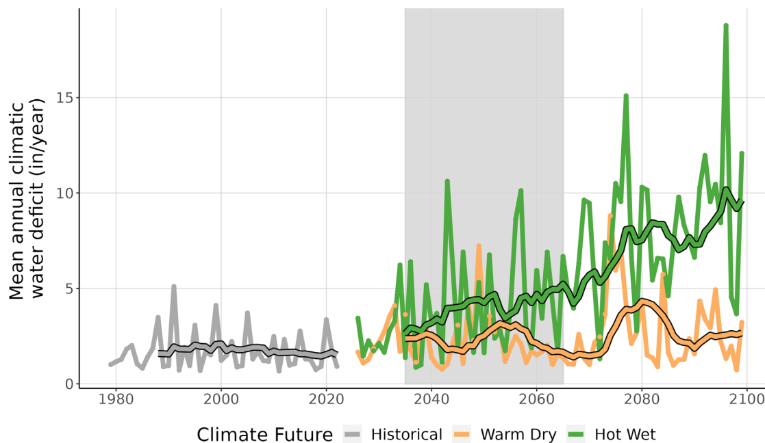
Figure 9. This line graph compares observed climatic water deficit at FONE (inches/year) (1979-2022) with projected climatic water deficit for the two climate futures over the period 2023-2099. The historical observation data is shown in gray, the Warm Dry climate future in orange, and the Hot Wet climate future in green. The smooth line running through each projection is the 10-year running average for historical observations and future projections. Gray-shaded area represents the time period that was averaged (2035-2065) to summarize future projections for the year 2050.
