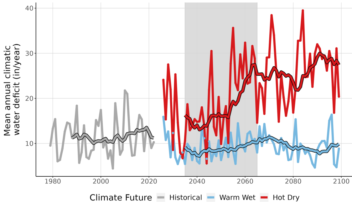
Figure 9. This line graph compares observed climatic water deficit at FOMA (inches/year) (1979-2022) with projected climatic water deficit for the two climate futures over the period 2023-2099. The historical observation data is shown in gray, the Warm Wet climate future in blue, and the Hot Dry climate future in red. The smooth line running through each projection is the 10-year running average for historical observations and future projections. Gray-shaded area represents the time period that was averaged (2035-2065) to summarize future projections for the year 2050.
