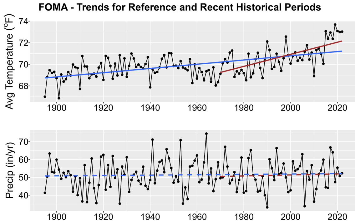
Figure 1. Historical trends in annual average temperature (upper plot) and annual total precipitation (lower plot) for FOMA from 1895-2022. Black points show yearly values while blue lines are linear regressions for the entire period record and red lines for 1970-2022 trends. Solid lines are significant trends (i.e., p < 0.05 ); dashed lines are not statistically significant.
