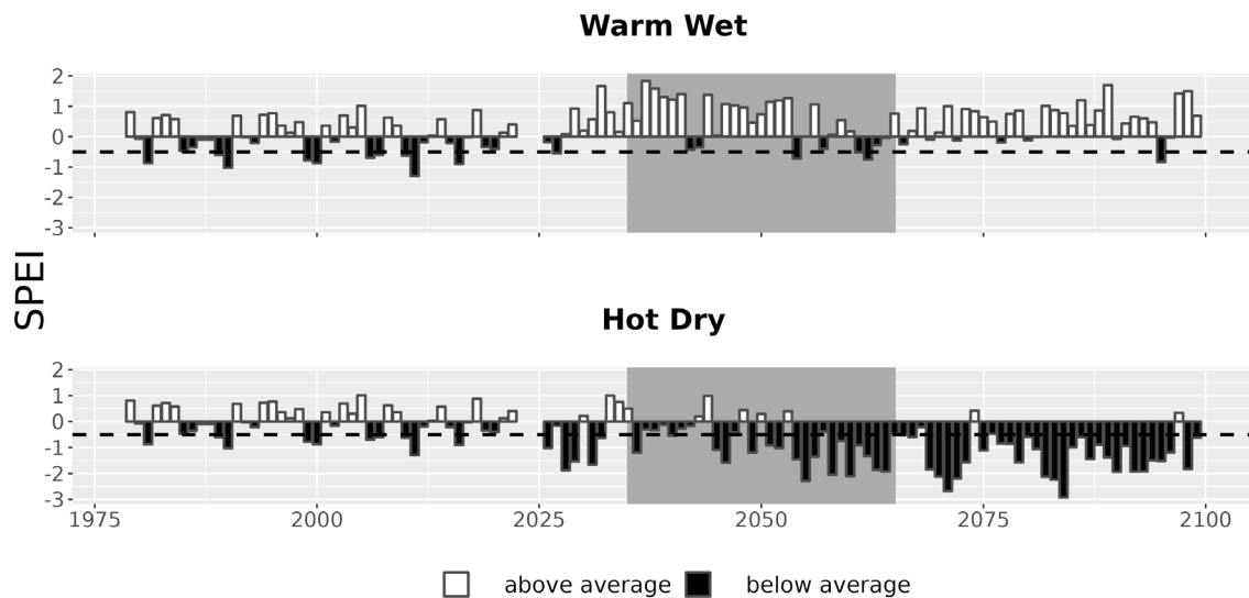
Figure 7. Drought metrics for FOMA. Drought index (SPEI; units = standard deviations from historical) timeseries for each climate future. Below-average SPEI (black bars) indicates dry conditions. The dotted line (SPEI = -0.5) indicates drought conditions.
