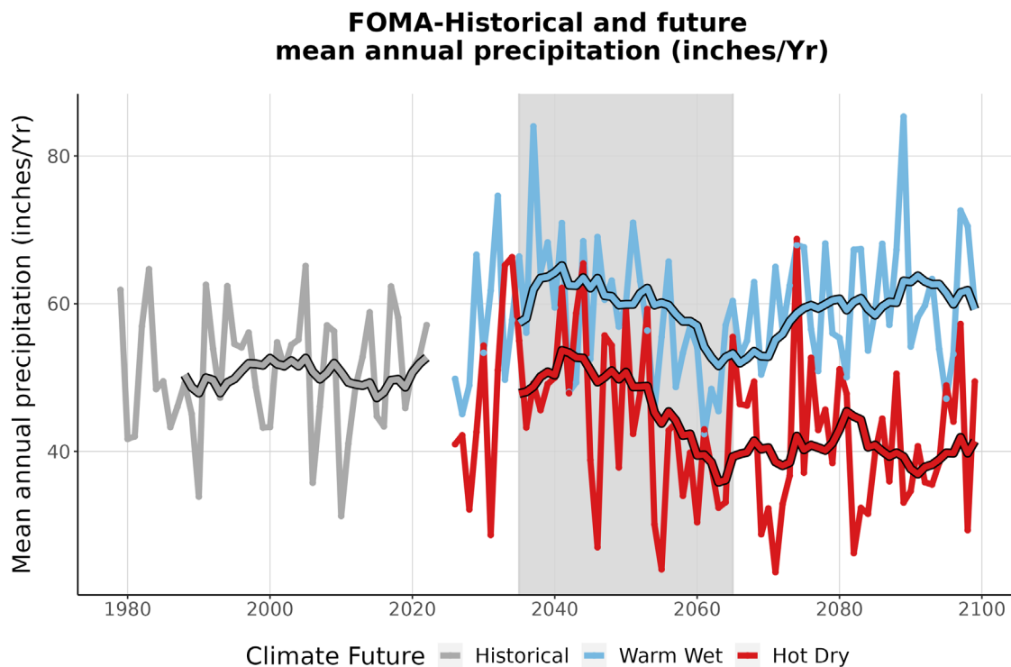
Figure 4. This graph compares observed average annual precipitation at FOMA (inches/year) (1979-2022) with projected average annual precipitation for the two climate futures over the period 2023-2099. The historically observed data is shown in gray, the Warm Wet climate future in blue, and the Hot Dry climate future in red. The smooth line running through each projection is the 10-year running average for historical observations and future projections. The gray-shaded area represents the time period that was averaged (2035-2065) to summarize future projections for the year 2050 (Appendix 1).
