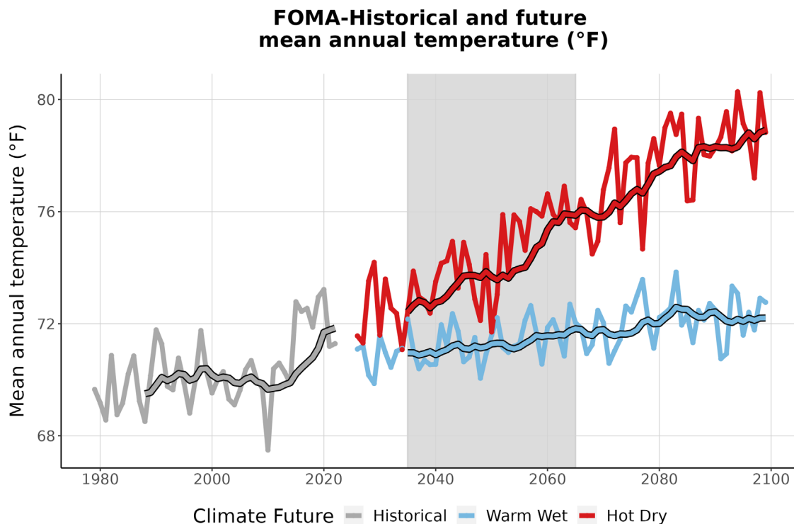
Figure 3. This graph compares observed average annual temperature at FOMA (°F) (1979-2022) with projected average annual temperature for the two climate futures over the period 2023-2099. The historically observed data
