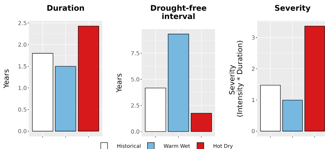
Figure 8. Drought metrics for FOMA. (Left) Average drought duration (years) historically (1979-2012) and under each climate future. (Middle) Average drought return interval (years), indicating the expected amount of time between periods of drought, historically and under each climate future. (Right) Average drought severity, a measure of drought intensity multiplied by duration, historically and under each climate future.
