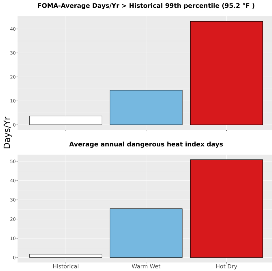
Figure 5. The upper bar graph represents the average number of days annually with temperatures greater than the historical 99th percentile (95.2 °F) historically (1979-2012) and for the two climate futures (2050). The bottom bar graph represents the average annual number of dangerous heat index days historically and for the two climate futures. Dangerous heat index days are days that exceed 105 °F.
