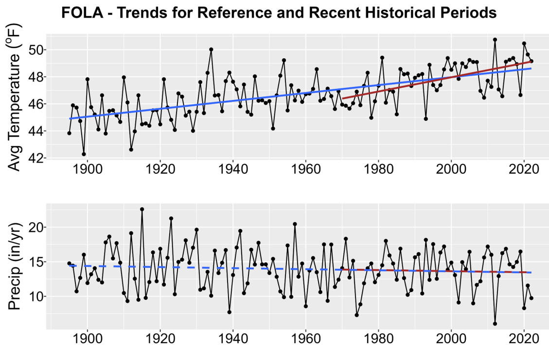
Figure 1. Historical trends in annual average temperature (upper plot) and annual total precipitation (lower plot) for FOLA from 1895-2022. Black points show yearly values while blue lines are linear regressions for the entire period record and red lines for 1970-2022 trends. Solid lines are significant trends (i.e., p < 0.05 ); dashed lines are not statistically significant.
