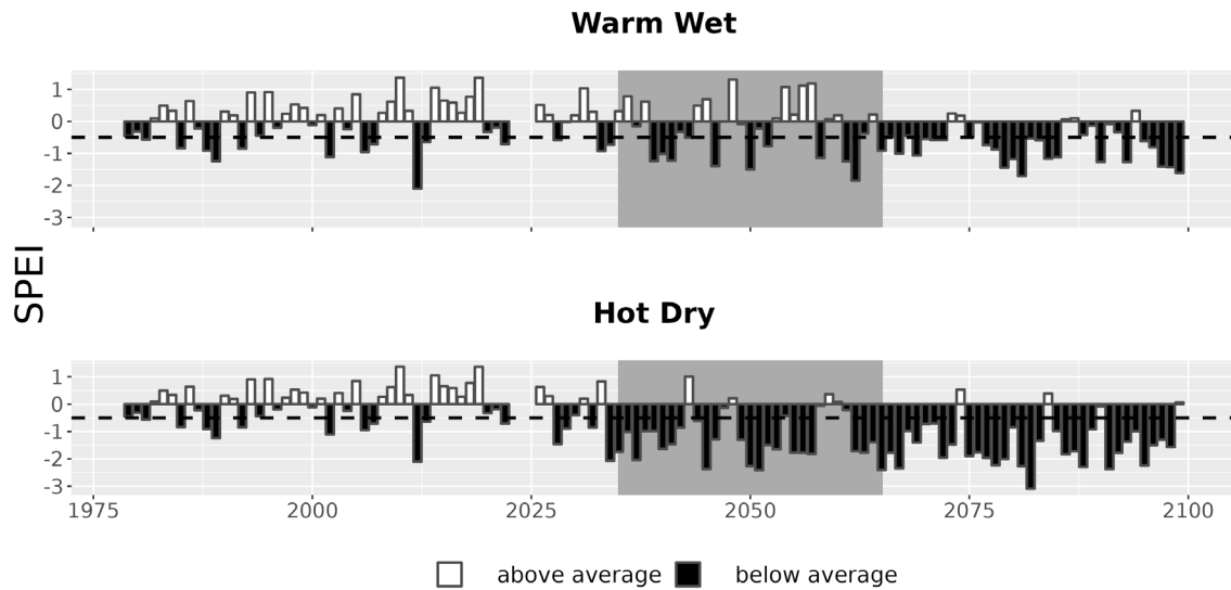
Figure 7. Drought metrics for FOLA. Drought index (SPEI; units = standard deviations from historical) timeseries for each climate future. Below-average SPEI (black bars) indicates dry conditions. The dotted line (SPEI = -0.5) indicates drought conditions.
