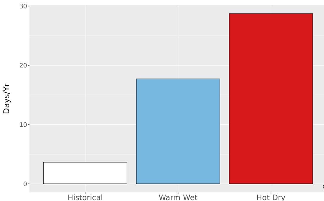
Figure 5. Metrics of extreme temperature at FOLA. The bar graph represents the average number of days annually with temperatures greater than the historical 99th percentile (98.7 °F) historically (1979-2012) and for the two climate futures (2050).
