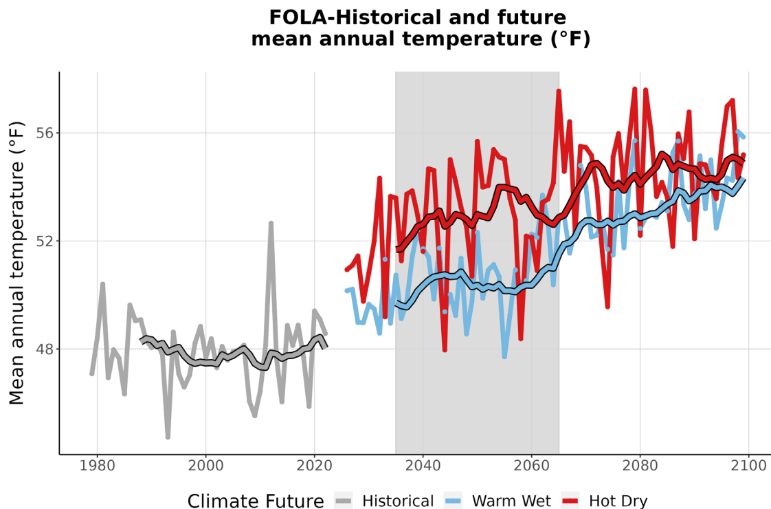
Figure 3. This graph compares observed average annual temperature at FOLA (°F) (1979-2022) with projected average annual temperature for the two climate futures over the period 2023-2099. The historically observed data
