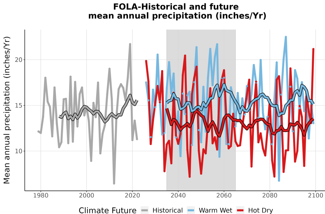
Figure 4. This graph compares observed average annual precipitation at FOLA (inches/year) (1979-2022) with projected average annual precipitation for the two climate futures over the period 2023-2099. The historically observed data is shown in gray, the Warm Wet climate future in blue, and the Hot Dry climate future in red. The smooth line running through each projection is the 10-year running average for historical observations and future projections. The gray-shaded area represents the time period that was averaged (2035-2065) to summarize future projections for the year 2050 (Appendix 1).
