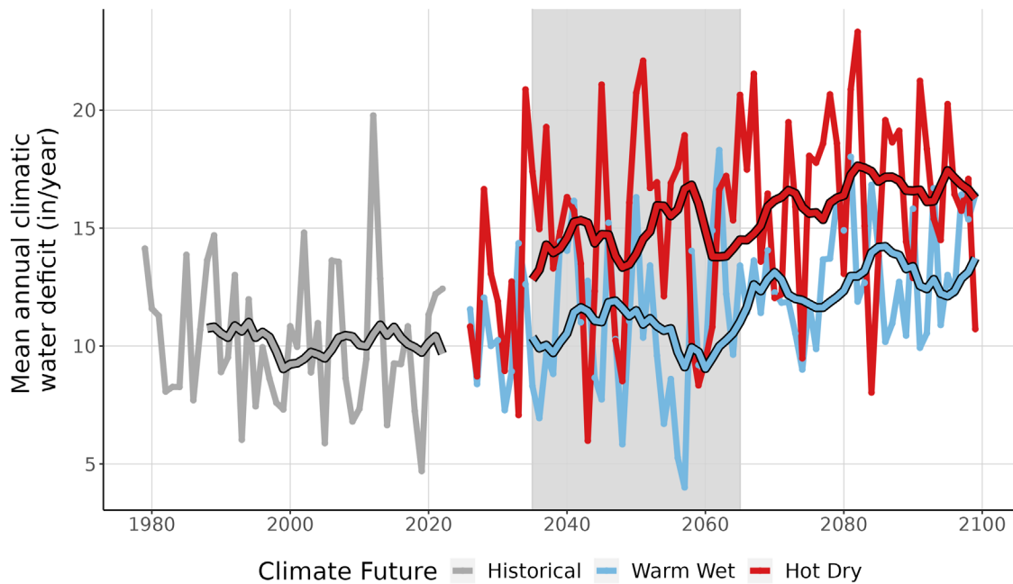
Figure 9. This line graph compares observed climatic water deficit at FOLA (inches/year) (1979-2022) with projected climatic water deficit for the two climate futures over the period 2023-2099. The historical observation data is shown in gray, the Warm Wet climate future in blue, and the Hot Dry climate future in red. The smooth line running through each projection is the 10-year running average for historical observations and future projections. Gray-shaded area represents the time period that was averaged (2035-2065) to summarize future projections for the year 2050.
