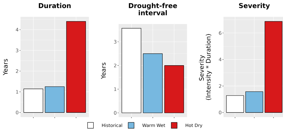
Figure 8. Drought metrics for FOLA. (Left) Average drought duration (years) historically (1979-2012) and under each climate future. (Middle) Average drought return interval (years), indicating the expected amount of time between periods of drought, historically and under each climate future. (Right) Average drought severity, a measure of drought intensity multiplied by duration, historically and under each climate future.
