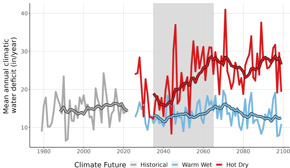
Figure 9. This line graph compares observed climatic water deficit at FOFR (inches/year) (1979-2022) with projected climatic water deficit for the two climate futures over the period 2023-2099. The historical observation data is shown in gray, the Warm Wet climate future in blue, and the Hot Dry climate future in red. The smooth line running through each projection is the 10-year running average for historical observations and future projections. Gray-shaded area represents the time period that was averaged (2035-2065) to summarize future projections for the year 2050.
