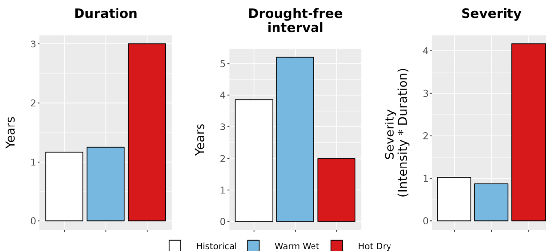
Figure 8. Drought metrics for FOFR. (Left) Average drought duration (years) historically (1979-2012) and under each climate future. (Middle) Average drought return interval (years), indicating the expected amount of time between periods of drought, historically and under each climate future. (Right) Average drought severity, a measure of drought intensity multiplied by duration, historically and under each climate future.
