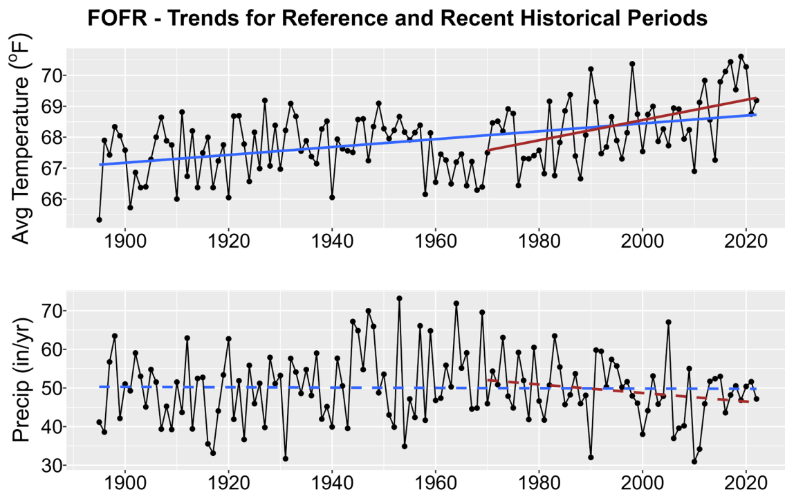
Figure 1. Historical trends in annual average temperature (upper plot) and annual total precipitation (lower plot) for FOFR from 1895-2022. Black points show yearly values while blue lines are linear regressions for the entire period record and red lines for 1970-2022 trends. Solid lines are significant trends (i.e., p < 0.05 ); dashed lines are not statistically significant.
