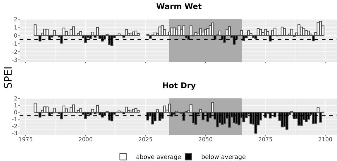
Figure 7. Drought metrics for FOFR. Drought index (SPEI; units = standard deviations from historical) timeseries for each climate future. Below-average SPEI (black bars) indicates dry conditions. The dotted line (SPEI = -0.5) indicates drought conditions.
