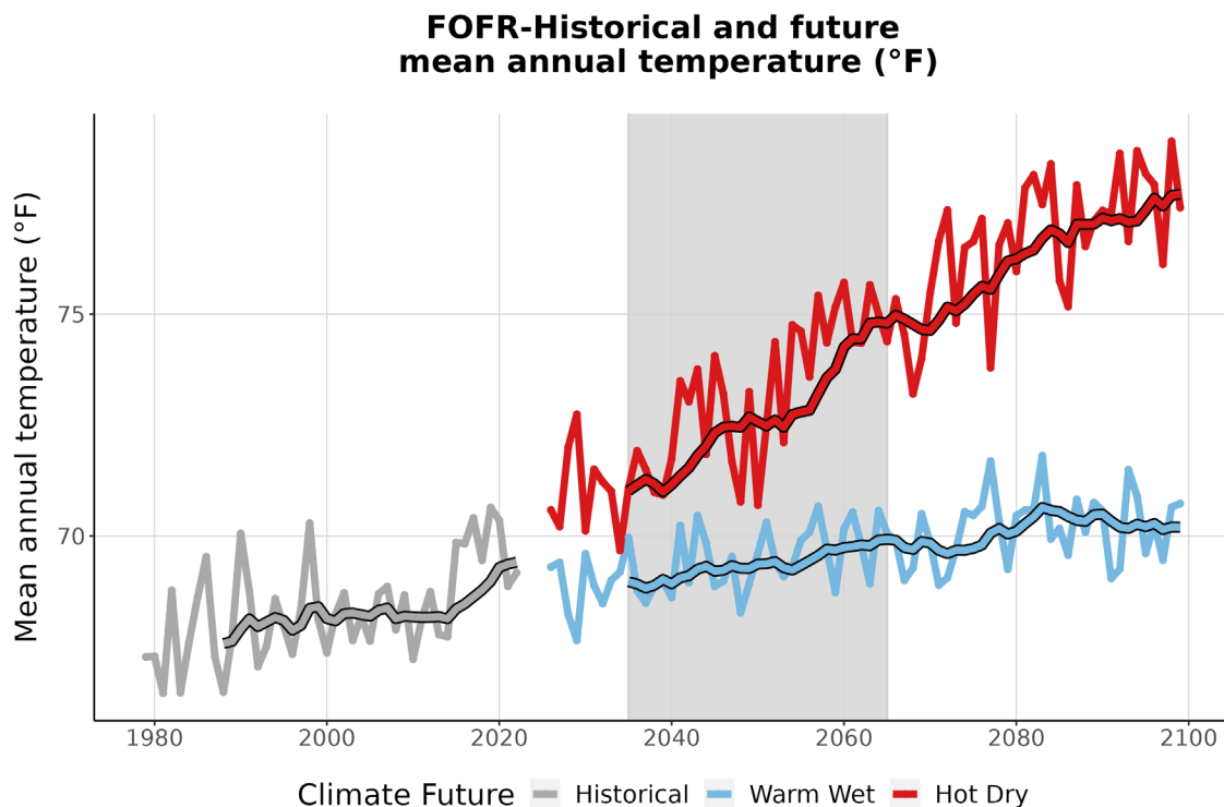
Figure 3. This graph compares observed average annual temperature at FOFR (°F) (1979-2022) with projected average annual temperature for the two climate futures over the period 2023-2099. The historically observed data
