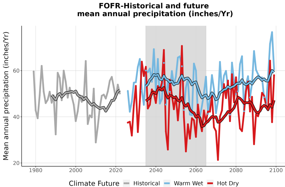
Figure 4. This graph compares observed average annual precipitation at FOFR (inches/year) (1979-2022) with projected average annual precipitation for the two climate futures over the period 2023-2099. The historically observed data is shown in gray, the Warm Wet climate future in blue, and the Hot Dry climate future in red. The smooth line running through each projection is the 10-year running average for historical observations and future projections. The gray-shaded area represents the time period that was averaged (2035-2065) to summarize future projections for the year 2050 (Appendix 1).
