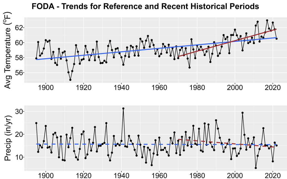
Figure 1. Historical trends in annual average temperature (upper plot) and annual total precipitation (lower plot) for FODA from 1895-2022. Black points show yearly values while blue lines are linear regressions for the entire period record and red lines for 1970-2022 trends. Solid lines are significant trends (i.e., p < 0.05 ); dashed lines are not statistically significant.
