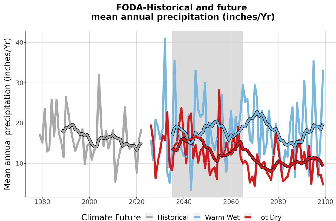
Figure 4. This graph compares observed average annual precipitation at FODA (inches/year) (1979-2022) with projected average annual precipitation for the two climate futures over the period 2023-2099. The historically observed data is shown in gray, the Warm Wet climate future in blue, and the Hot Dry climate future in red. The smooth line running through each projection is the 10-year running average for historical observations and future projections. The gray-shaded area represents the time period that was averaged (2035-2065) to summarize future projections for the year 2050 (Appendix 1).
