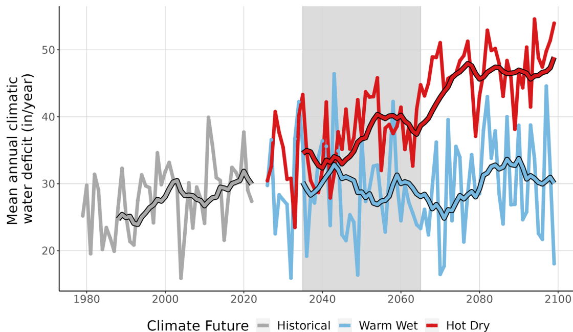
Figure 9. This line graph compares observed climatic water deficit at FODA (inches/year) (1979-2022) with projected climatic water deficit for the two climate futures over the period 2023-2099. The historical observation data is shown in gray, the Warm Wet climate future in blue, and the Hot Dry climate future in red. The smooth line running through each projection is the 10-year running average for historical observations and future projections. Gray-shaded area represents the time period that was averaged (2035-2065) to summarize future projections for the year 2050.
