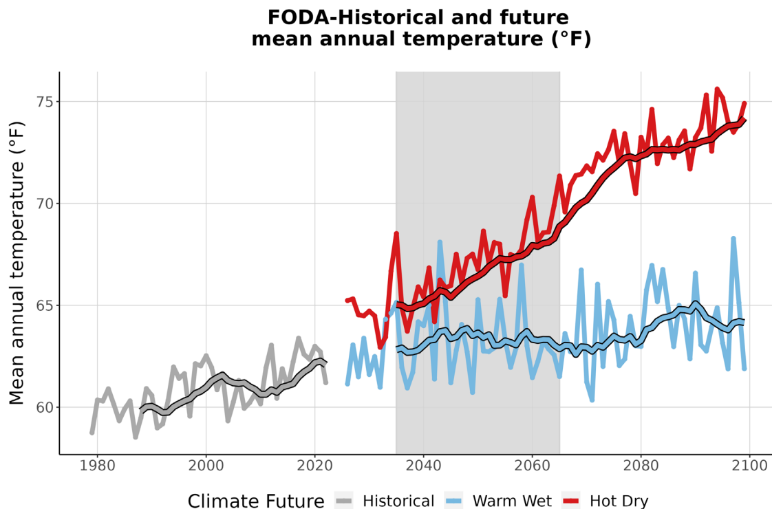
Figure 3. This graph compares observed average annual temperature at FODA (°F) (1979-2022) with projected average annual temperature for the two climate futures over the period 2023-2099. The historically observed data
