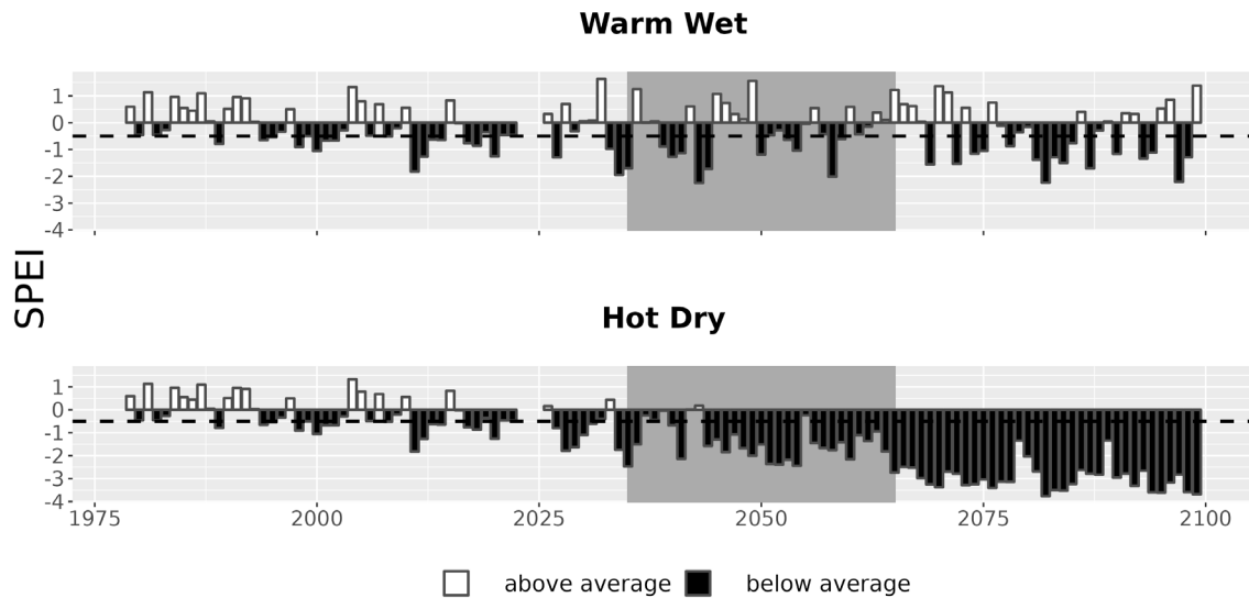
Figure 7. Drought metrics for FODA. Drought index (SPEI; units = standard deviations from historical) timeseries for each climate future. Below-average SPEI (black bars) indicates dry conditions. The dotted line (SPEI = -0.5) indicates drought conditions.
