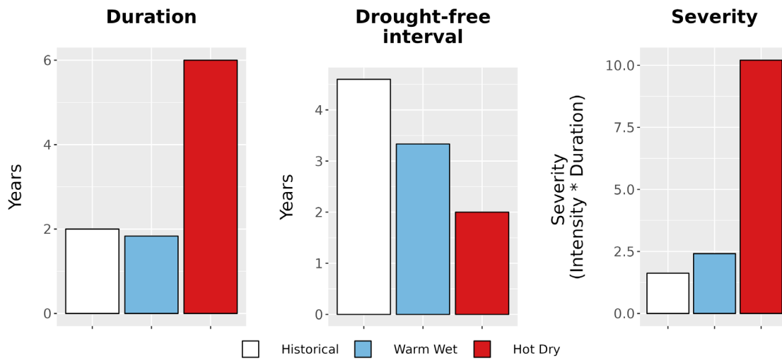
Figure 8. Drought metrics for FODA. (Left) Average drought duration (years) historically (1979-2012) and under each climate future. (Middle) Average drought return interval (years), indicating the expected amount of time between periods of drought, historically and under each climate future. (Right) Average drought severity, a measure of drought intensity multiplied by duration, historically and under each climate future.
