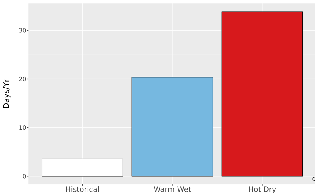
Figure 5. Metrics of extreme temperature at FODA. The bar graph represents the average number of days annually with temperatures greater than the historical 99th percentile (97.1 °F) historically (1979-2012) and for the two climate futures (2050).
