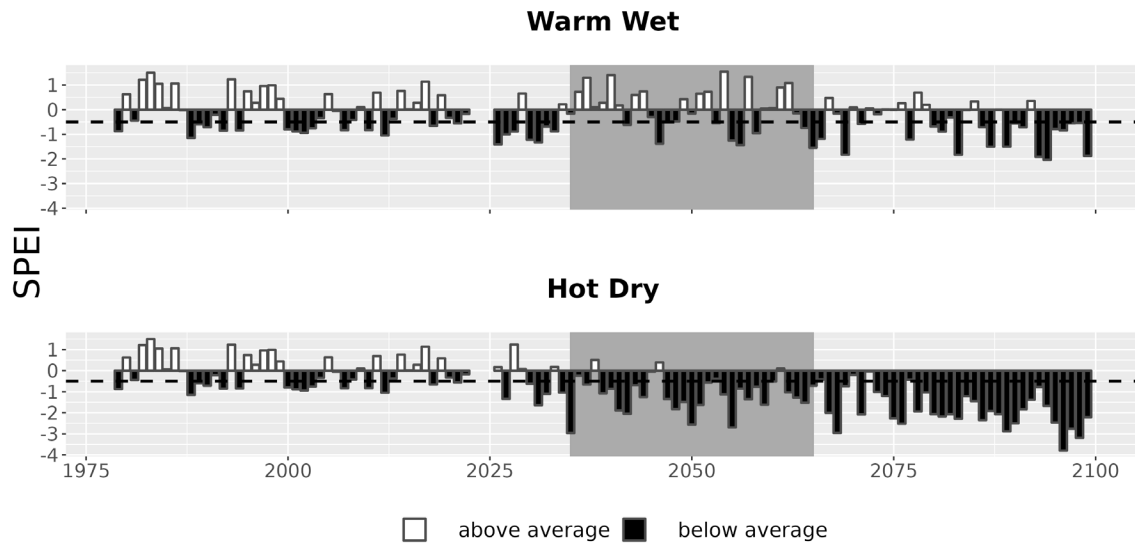
Figure 7. Drought metrics for FOBU. Drought index (SPEI; units = standard deviations from historical) timeseries for each climate future. Below-average SPEI (black bars) indicates dry conditions. The dotted line (SPEI = -0.5) indicates drought conditions.
