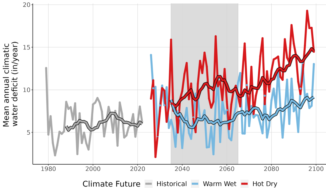
Figure 9. This line graph compares observed climatic water deficit at FOBU (inches/year) (1979-2022) with projected climatic water deficit for the two climate futures over the period 2023-2099. The historical observation data is shown in gray, the Warm Wet climate future in blue, and the Hot Dry climate future in red. The smooth line running through each projection is the 10-year running average for historical observations and future projections. Gray-shaded area represents the time period that was averaged (2035-2065) to summarize future projections for the year 2050.
