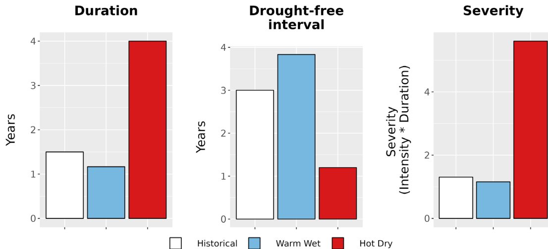
Figure 8. Drought metrics for FOBU. (Left) Average drought duration (years) historically (1979-2012) and under each climate future. (Middle) Average drought return interval (years), indicating the expected amount of time between periods of drought, historically and under each climate future. (Right) Average drought severity, a measure of drought intensity multiplied by duration, historically and under each climate future.
