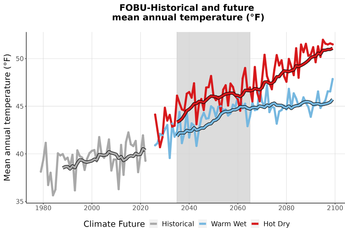
Figure 3. This graph compares observed average annual temperature at FOBU (°F) (1979-2022) with projected average annual temperature for the two climate futures over the period 2023-2099. The historically observed data is shown in gray, the Warm Wet climate future in blue, and the Hot Dry climate future in red. The smooth line
