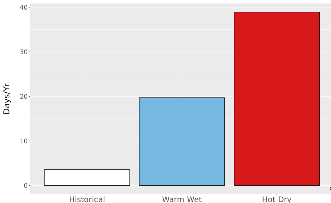
Figure 5. Metrics of extreme temperature at FOBU. The bar graph represents the average number of days annually with temperatures greater than the historical 99th percentile (88.2 °F) historically (1979-2012) and for the two climate futures (2050).
