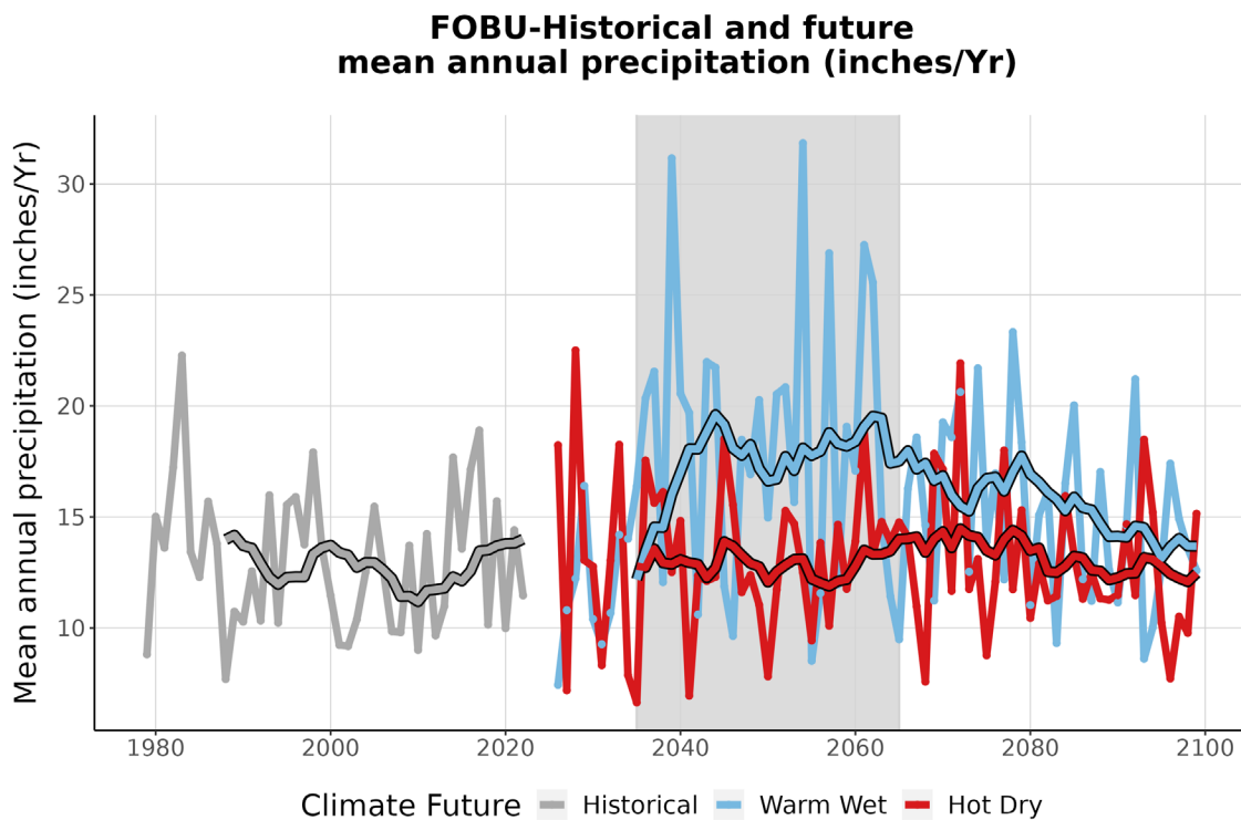
Figure 4. This graph compares observed average annual precipitation at FOBU (inches/year) (1979-2022) with projected average annual precipitation for the two climate futures over the period 2023-2099. The historically observed data is shown in gray, the Warm Wet climate future in blue, and the Hot Dry climate future in red. The smooth line running through each projection is the 10-year running average for historical observations and future projections. The gray-shaded area represents the time period that was averaged (2035-2065) to summarize future projections for the year 2050 (Appendix 1).
