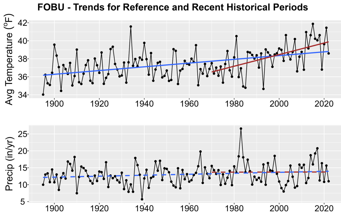
Figure 1. Historical trends in annual average temperature (upper plot) and annual total precipitation (lower plot) for FOBU from 1895-2022. Black points show yearly values while blue lines are linear regressions for the entire period record and red lines for 1970-2022 trends. Solid lines are significant trends (i.e., p < 0.05 ); dashed lines are not statistically significant.
