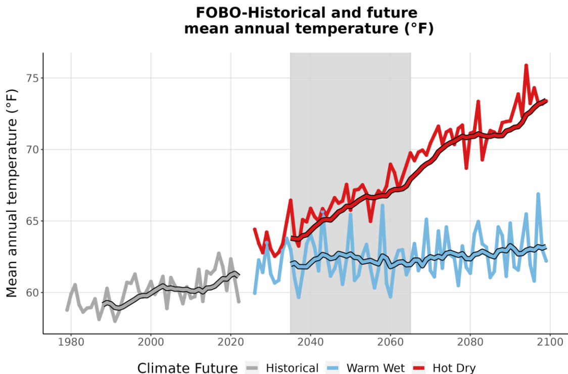
Figure 3. This graph compares observed average annual temperature at FOBO (°F) (1979-2022) with projected average annual temperature for the two climate futures over the period 2023-2099. The historically observed data
