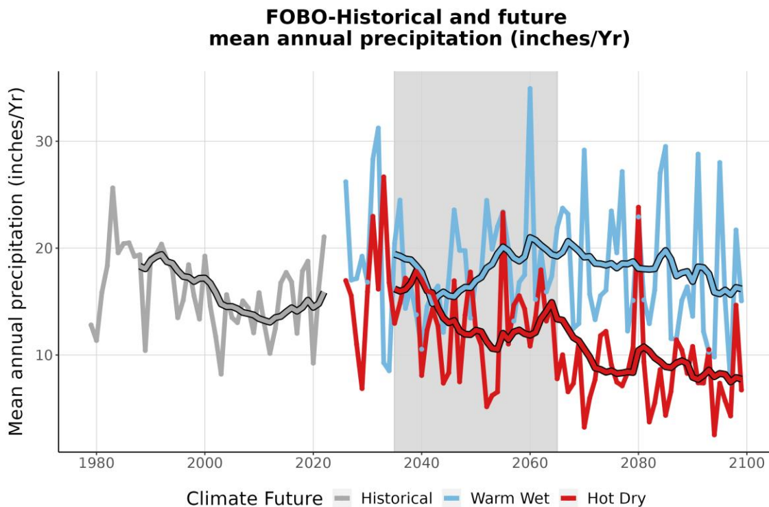
Figure 4. This graph compares observed average annual precipitation at FOBO (inches/year) (1979-2022) with projected average annual precipitation for the two climate futures over the period 2023-2099. The historically observed data is shown in gray, the Warm Wet climate future in blue, and the Hot Dry climate future in red. The smooth line running through each projection is the 10-year running average for historical observations and future projections. The gray-shaded area represents the time period that was averaged (2035-2065) to summarize future projections for the year 2050 (Appendix 1).
