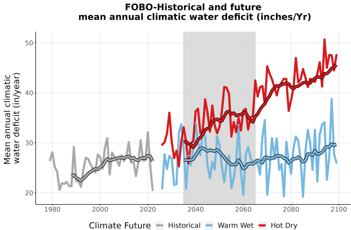
Figure 9. This line graph compares observed climatic water deficit at FOBO (inches/year) (1979-2022) with projected climatic water deficit for the two climate futures over the period 2023-2099. The historical observation data is shown in gray, the Warm Wet climate future in blue, and the Hot Dry climate future in red. The smooth line running through each projection is the 10-year running average for historical observations and future projections. Gray-shaded area represents the time period that was averaged (2035-2065) to summarize future projections for the year 2050.
