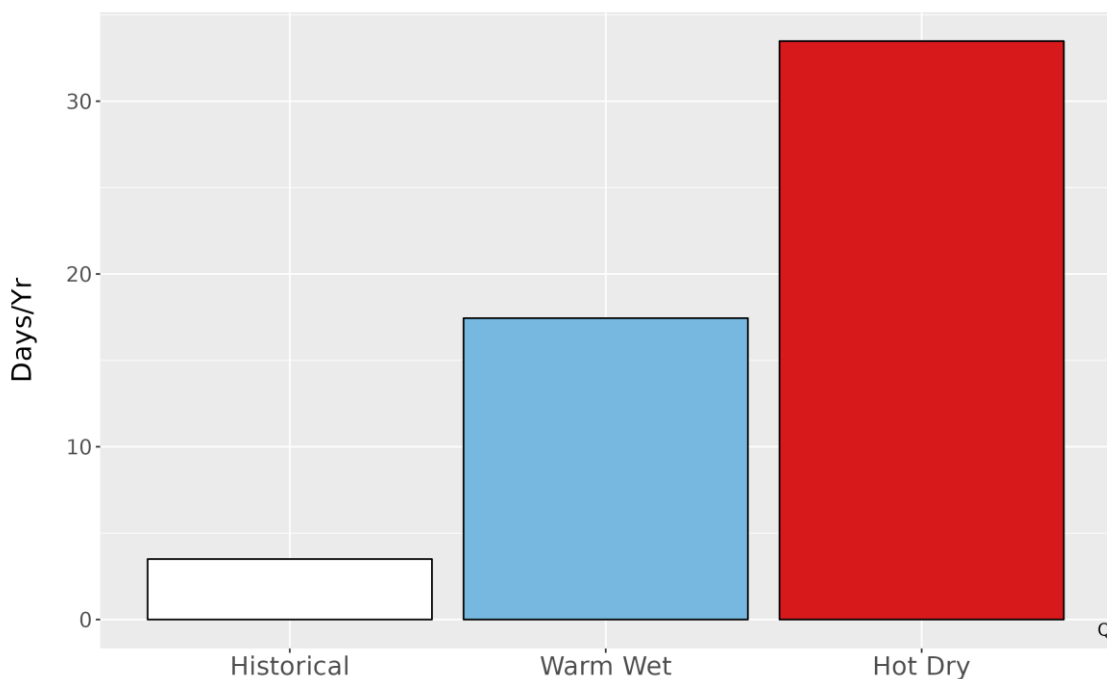
Figure 5. Metrics of extreme temperature at FOBO. The bar graph represents the average number of days annually with temperatures greater than the historical 99th percentile (98.9 °F) historically (1979-2012) and for the two climate futures (2050).
