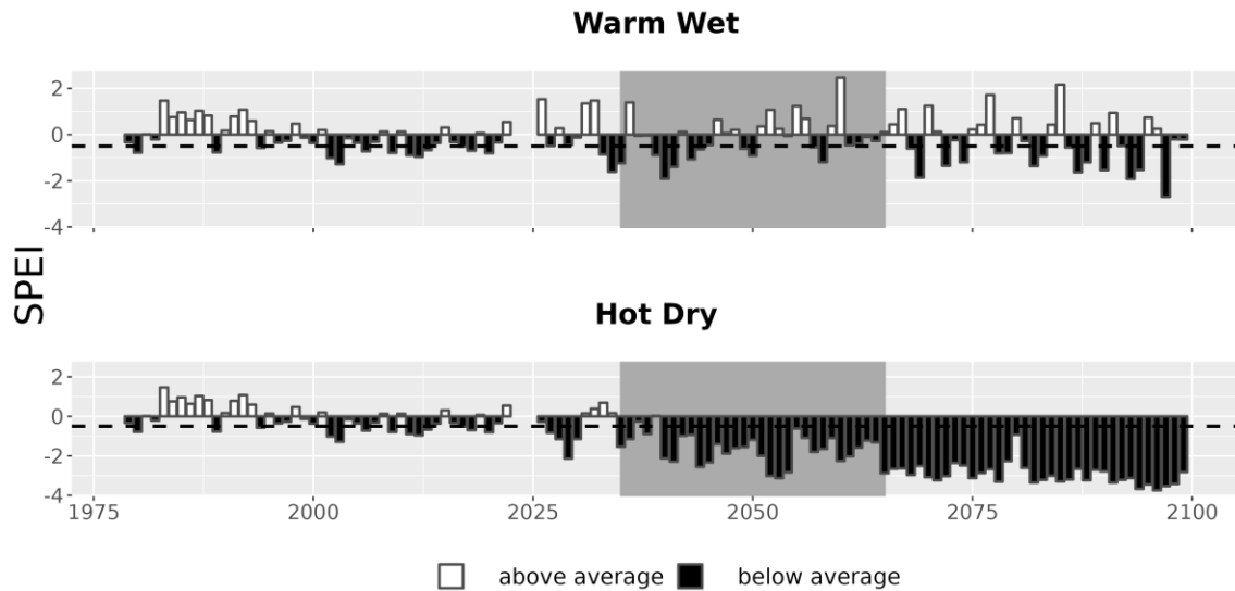
Figure 7. Drought metrics for FOBO. Drought index (SPEI; units = standard deviations from historical) timeseries for each climate future. Below-average SPEI (black bars) indicates dry conditions. The dotted line (SPEI = -0.5) indicates drought conditions.
