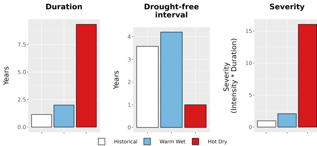
Figure 8. Drought metrics for FOBO. (Left) Average drought duration (years) historically (1979-2012) and under each climate future. (Middle) Average drought return interval (years), indicating the expected amount of time between periods of drought, historically and under each climate future. (Right) Average drought severity, a measure of drought intensity multiplied by duration, historically and under each climate future.
