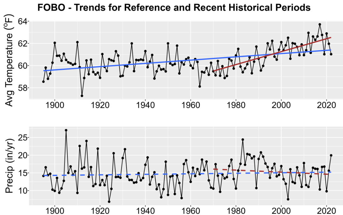
Figure 1. Historical trends in annual average temperature (upper plot) and annual total precipitation (lower plot) for FOBO from 1895-2022. Black points show yearly values while blue lines are linear regressions for the entire period record and red lines for 1970-2022 trends. Solid lines are significant trends (i.e., p < 0.05 ); dashed lines are not statistically significant.
