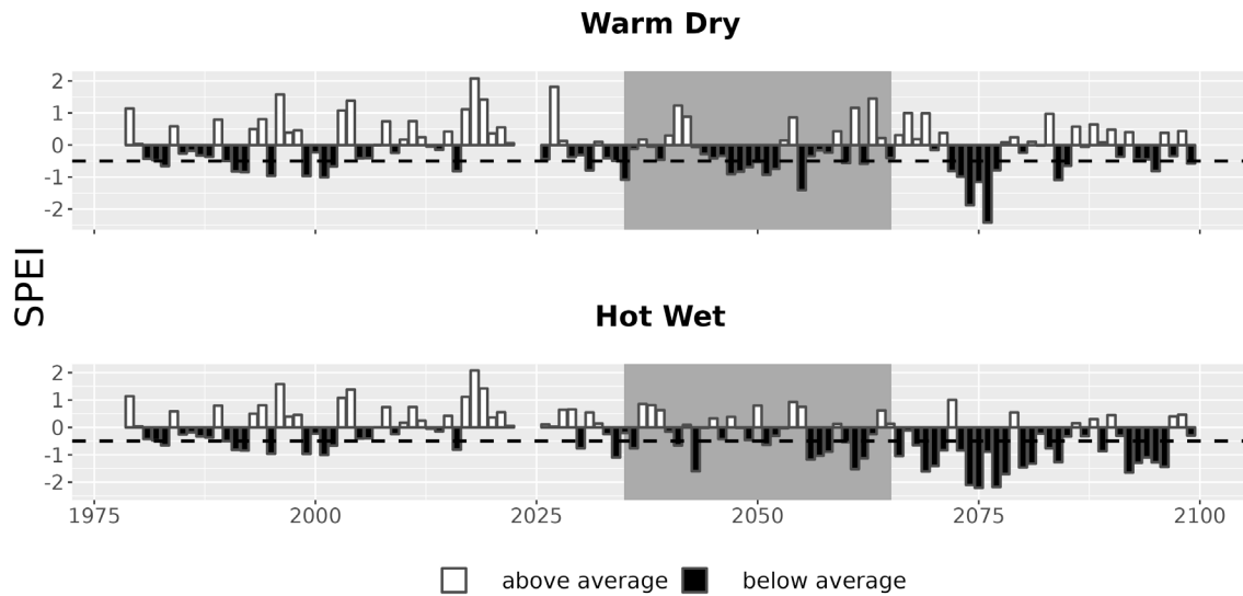
Figure 7. Drought metrics for FLNI. Drought index (SPEI; units = standard deviations from historical) timeseries for each climate future. Below-average SPEI (black bars) indicates dry conditions. The dotted line (SPEI = -0.5) indicates drought conditions.
