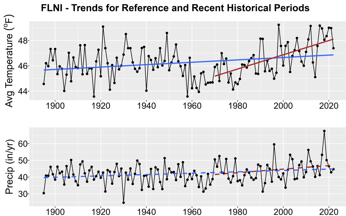
Figure 1. Historical trends in annual average temperature (upper plot) and annual total precipitation (lower plot) for FLNI from 1895-2022. Black points show yearly values while blue lines are linear regressions for the entire period record and red lines for 1970-2022 trends. Solid lines are significant trends (i.e., p < 0.05 ); dashed lines are not statistically significant.
