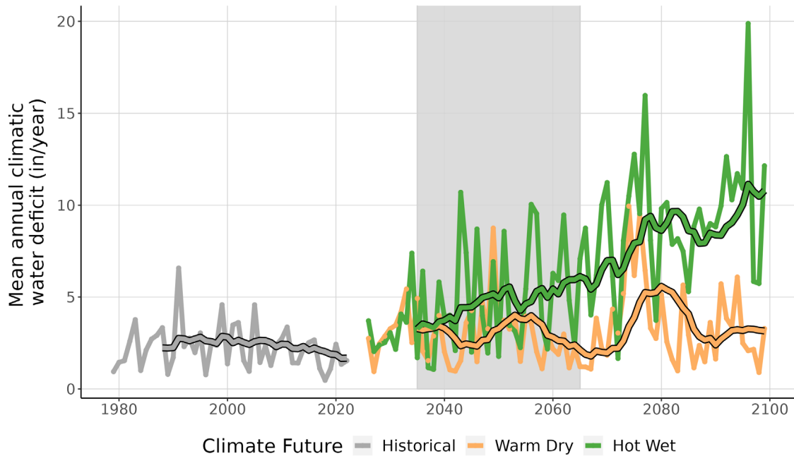
Figure 9. This line graph compares observed climatic water deficit at FLNI (inches/year) (1979-2022) with projected climatic water deficit for the two climate futures over the period 2023-2099. The historical observation data is shown in gray, the Warm Dry climate future in orange, and the Hot Wet climate future in green. The smooth line running through each projection is the 10-year running average for historical observations and future projections. Gray-shaded area represents the time period that was averaged (2035-2065) to summarize future projections for the year 2050.
