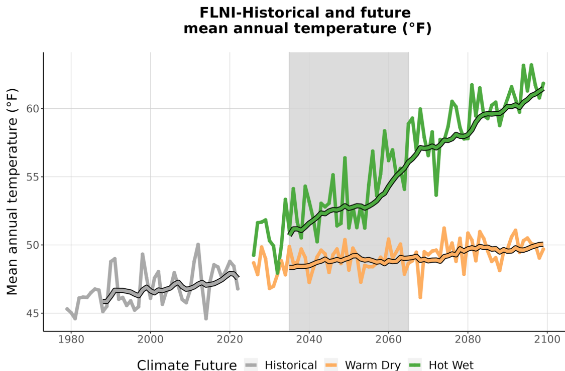
Figure 3. This graph compares observed average annual temperature at FLNI (°F) (1979-2022) with projected average annual temperature for the two climate futures over the period 2023-2099. The historically observed data
