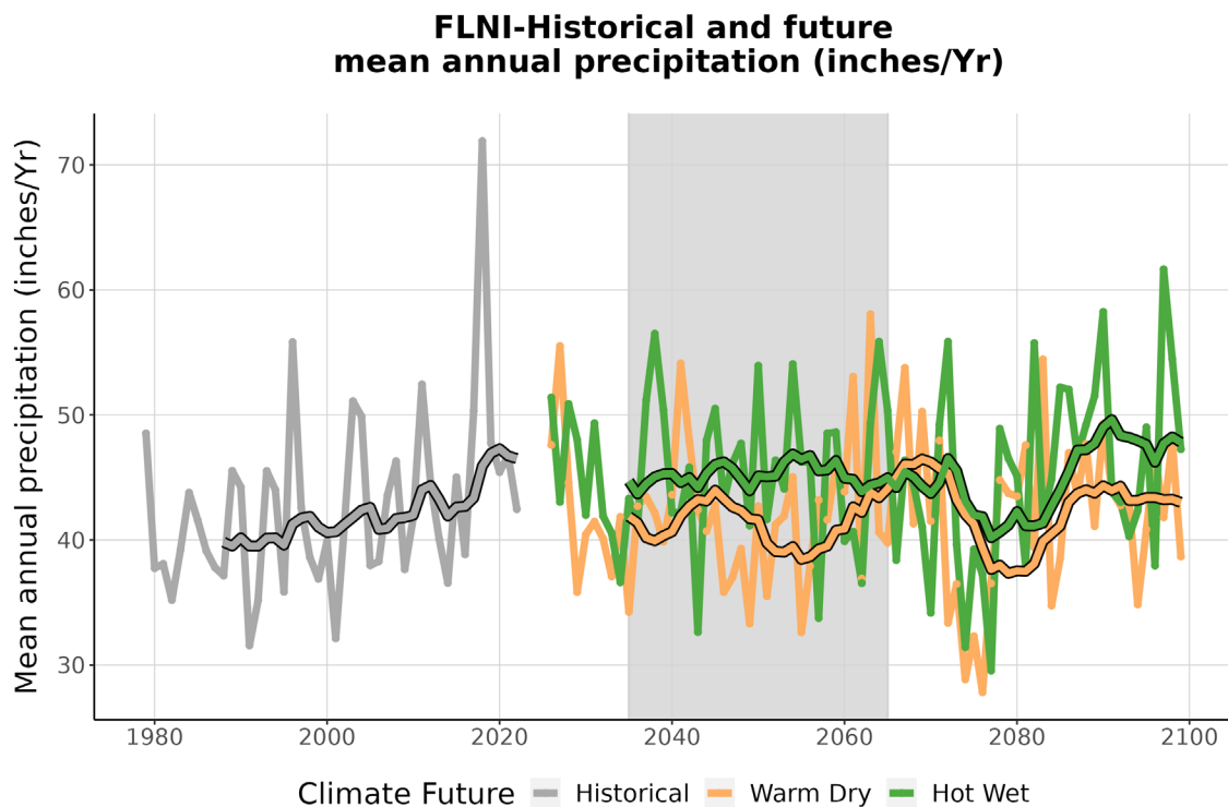
Figure 4. This graph compares observed average annual precipitation at FLNI (inches/year) (1979-2022) with projected average annual precipitation for the two climate futures over the period 2023-2099. The historically observed data is shown in gray, the Warm Dry climate future in orange, and the Hot Wet climate future in green. The smooth line running through each projection is the 10-year running average for historical observations and future projections. The gray-shaded area represents the time period that was averaged (2035-2065) to summarize future projections for the year 2050 (Appendix 1).
