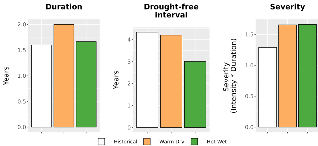
Figure 8. Drought metrics for FLNI. (Left) Average drought duration (years) historically (1979-2012) and under each climate future. (Middle) Average drought return interval (years), indicating the expected amount of time between periods of drought, historically and under each climate future. (Right) Average drought severity, a measure of drought intensity multiplied by duration, historically and under each climate future.
