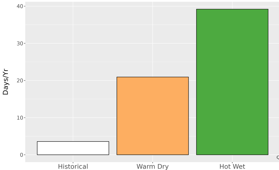
Figure 5. Metrics of extreme temperature at FLNI. The bar graph represents the average number of days annually with temperatures greater than the historical 99th percentile (84.6 °F) historically (1979-2012) and for the two climate futures (2050).
