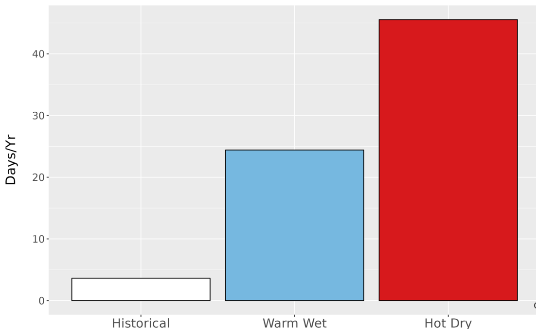
Figure 5. Metrics of extreme temperature at FLFO. The bar graph represents the average number of days annually with temperatures greater than the historical 99th percentile (82.8 °F) historically (1979-2012) and for the two climate futures (2050).
