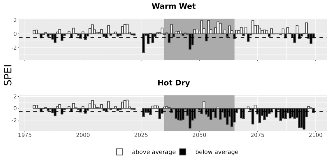
Figure 7. Drought metrics for FILA. Drought index (SPEI; units = standard deviations from historical) timeseries for each climate future. Below-average SPEI (black bars) indicates dry conditions. The dotted line (SPEI = -0.5) indicates drought conditions.
