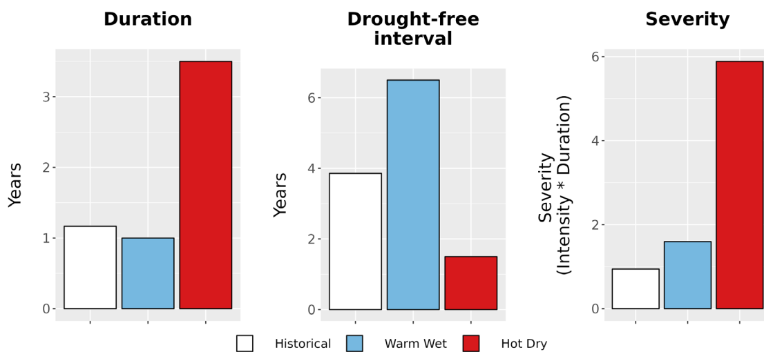
Figure 8. Drought metrics for FILA. (Left) Average drought duration (years) historically (1979-2012) and under each climate future. (Middle) Average drought return interval (years), indicating the expected amount of time between periods of drought, historically and under each climate future. (Right) Average drought severity, a measure of drought intensity multiplied by duration, historically and under each climate future.
