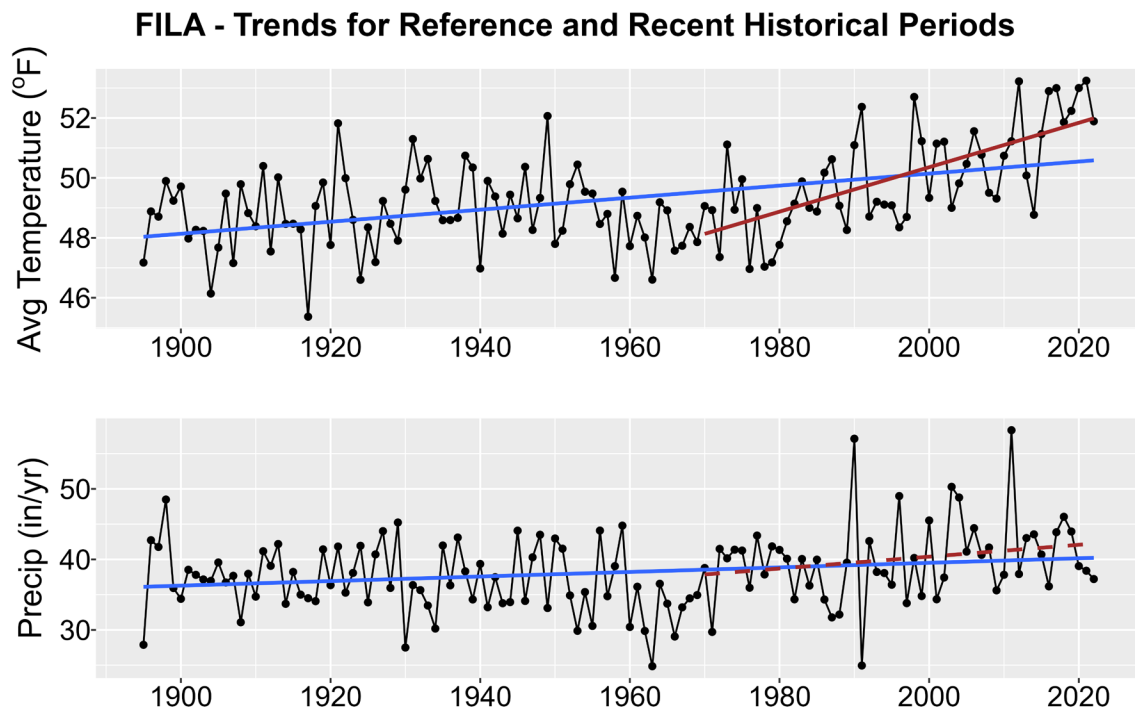
Figure 1. Historical trends in annual average temperature (upper plot) and annual total precipitation (lower plot) for FILA from 1895-2022. Black points show yearly values while blue lines are linear regressions for the entire period record and red lines for 1970-2022 trends. Solid lines are significant trends (i.e., p < 0.05 ); dashed lines are not statistically significant.
