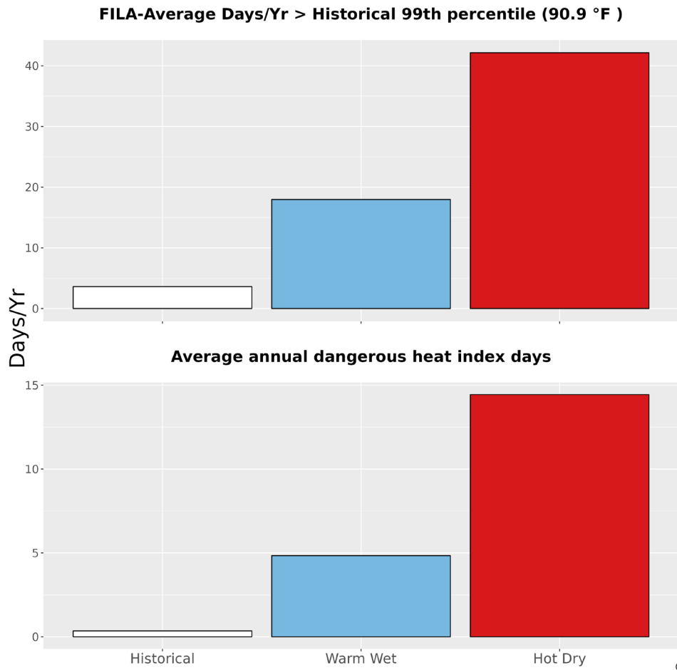
Figure 5. The upper bar graph represents the average number of days annually with temperatures greater than the historical 99th percentile (90.9 °F) historically (1979-2012) and for the two climate futures (2050). The bottom bar graph represents the average annual number of dangerous heat index days historically and for the two climate futures. Dangerous heat index days are days that exceed 105 °F.
