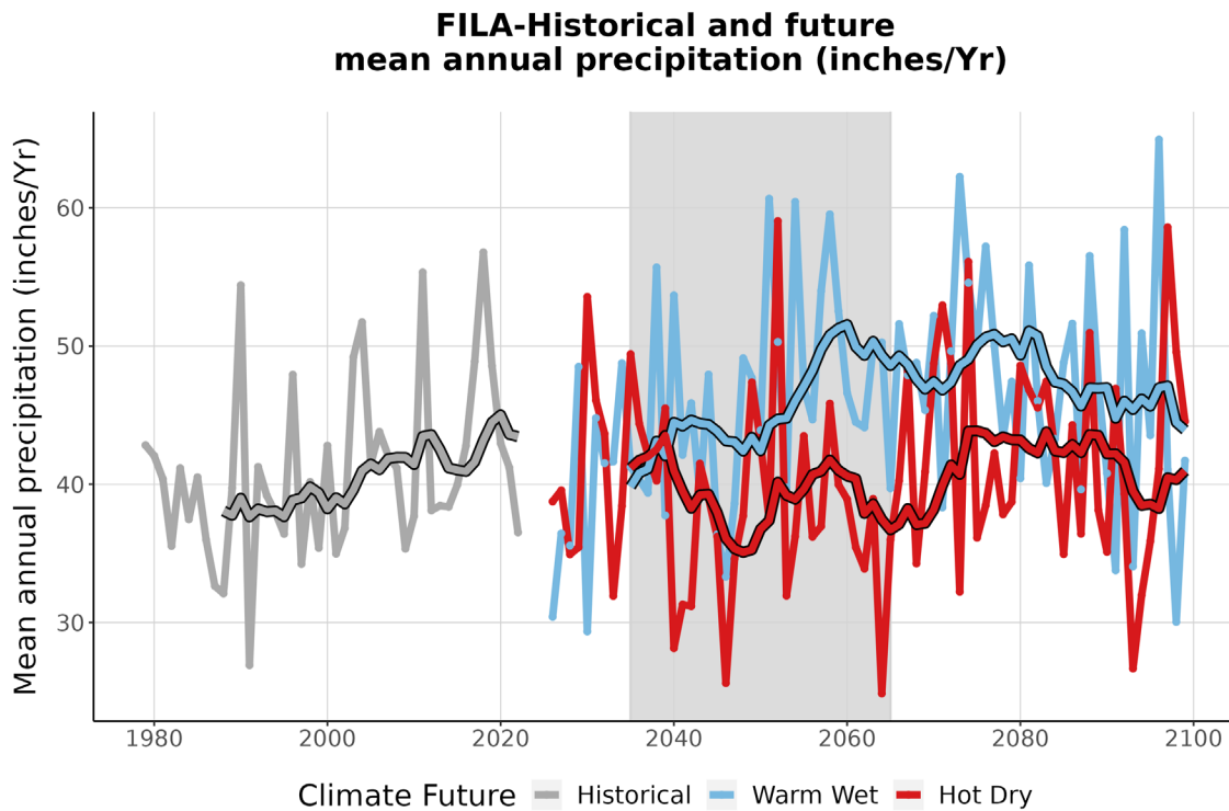
Figure 4. This graph compares observed average annual precipitation at FILA (inches/year) (1979-2022) with projected average annual precipitation for the two climate futures over the period 2023-2099. The historically observed data is shown in gray, the Warm Wet climate future in blue, and the Hot Dry climate future in red. The smooth line running through each projection is the 10-year running average for historical observations and future projections. The gray-shaded area represents the time period that was averaged (2035-2065) to summarize future projections for the year 2050 (Appendix 1).
