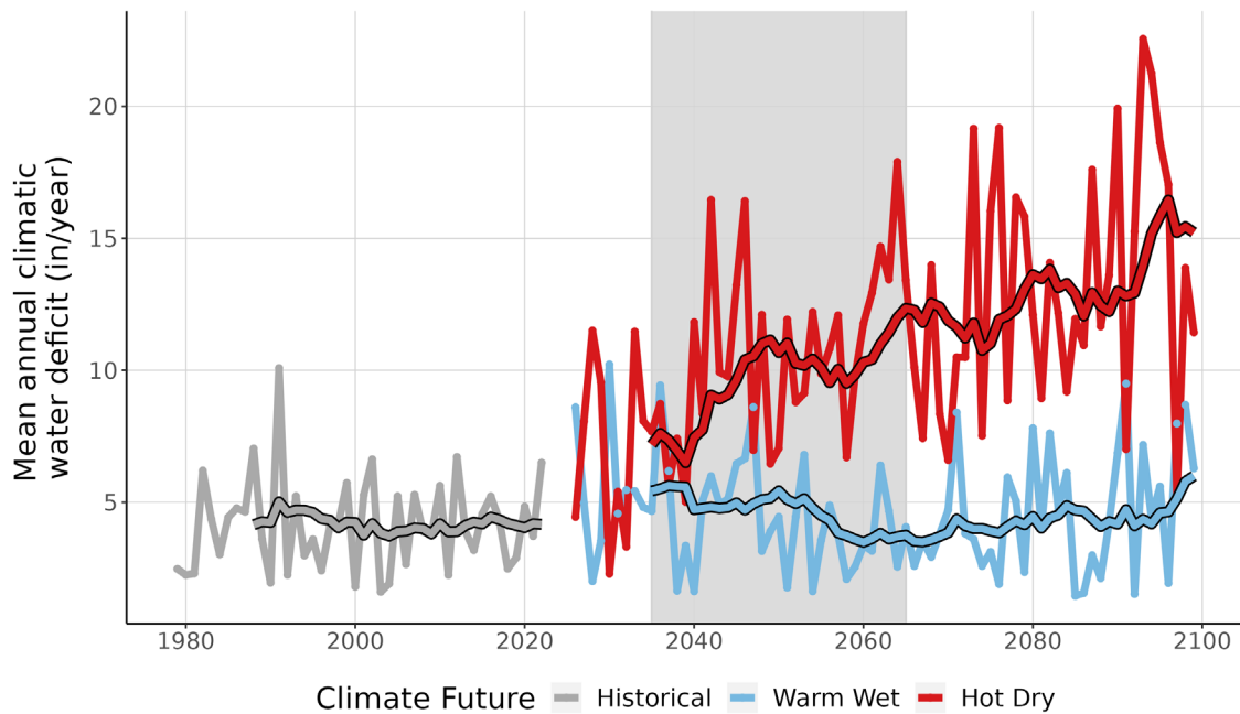
Figure 9. This line graph compares observed climatic water deficit at FILA (inches/year) (1979-2022) with projected climatic water deficit for the two climate futures over the period 2023-2099. The historical observation data is shown in gray, the Warm Wet climate future in blue, and the Hot Dry climate future in red. The smooth line running through each projection is the 10-year running average for historical observations and future projections. Gray-shaded area represents the time period that was averaged (2035-2065) to summarize future projections for the year 2050.
