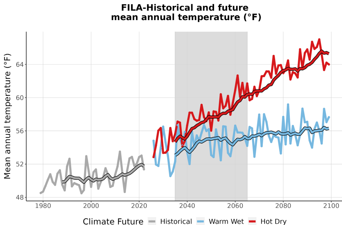
Figure 3. This graph compares observed average annual temperature at FILA (°F) (1979-2022) with projected average annual temperature for the two climate futures over the period 2023-2099. The historically observed data
