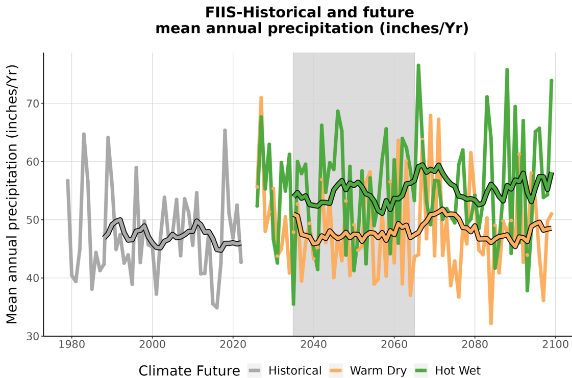
Figure 4. This graph compares observed average annual precipitation at FIIS (inches/year) (1979-2022) with projected average annual precipitation for the two climate futures over the period 2023-2099. The historically observed data is shown in gray, the Warm Dry climate future in orange, and the Hot Wet climate future in green. The smooth line running through each projection is the 10-year running average for historical observations and future projections. The gray-shaded area represents the time period that was averaged (2035-2065) to summarize future projections for the year 2050 (Appendix 1).
