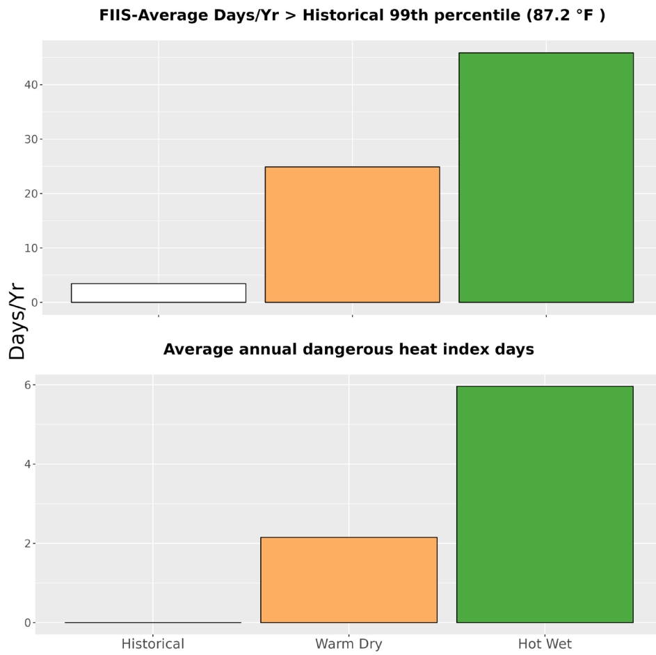
Figure 5. The upper bar graph represents the average number of days annually with temperatures greater than the historical 99th percentile (87.2 °F) historically (1979-2012) and for the two climate futures (2050). The bottom bar graph represents the average annual number of dangerous heat index days historically and for the two climate futures. Dangerous heat index days are days that exceed 105 °F.
