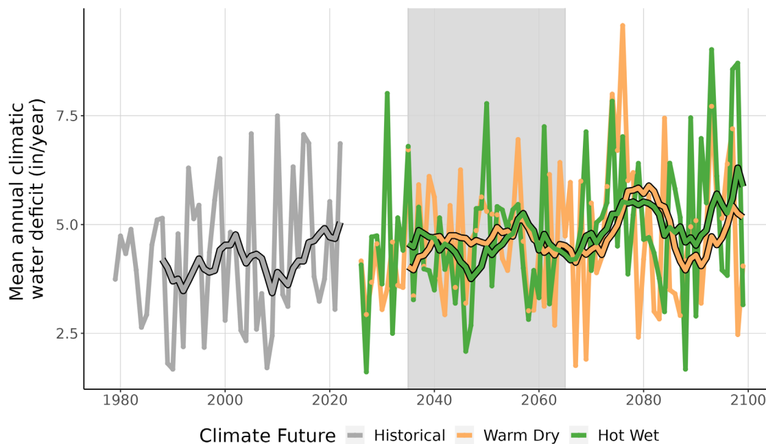
Figure 9. This line graph compares observed climatic water deficit at FIIS (inches/year) (1979-2022) with projected climatic water deficit for the two climate futures over the period 2023-2099. The historical observation data is shown in gray, the Warm Dry climate future in orange, and the Hot Wet climate future in green. The smooth line running through each projection is the 10-year running average for historical observations and future projections. Gray-shaded area represents the time period that was averaged (2035-2065) to summarize future projections for the year 2050.
