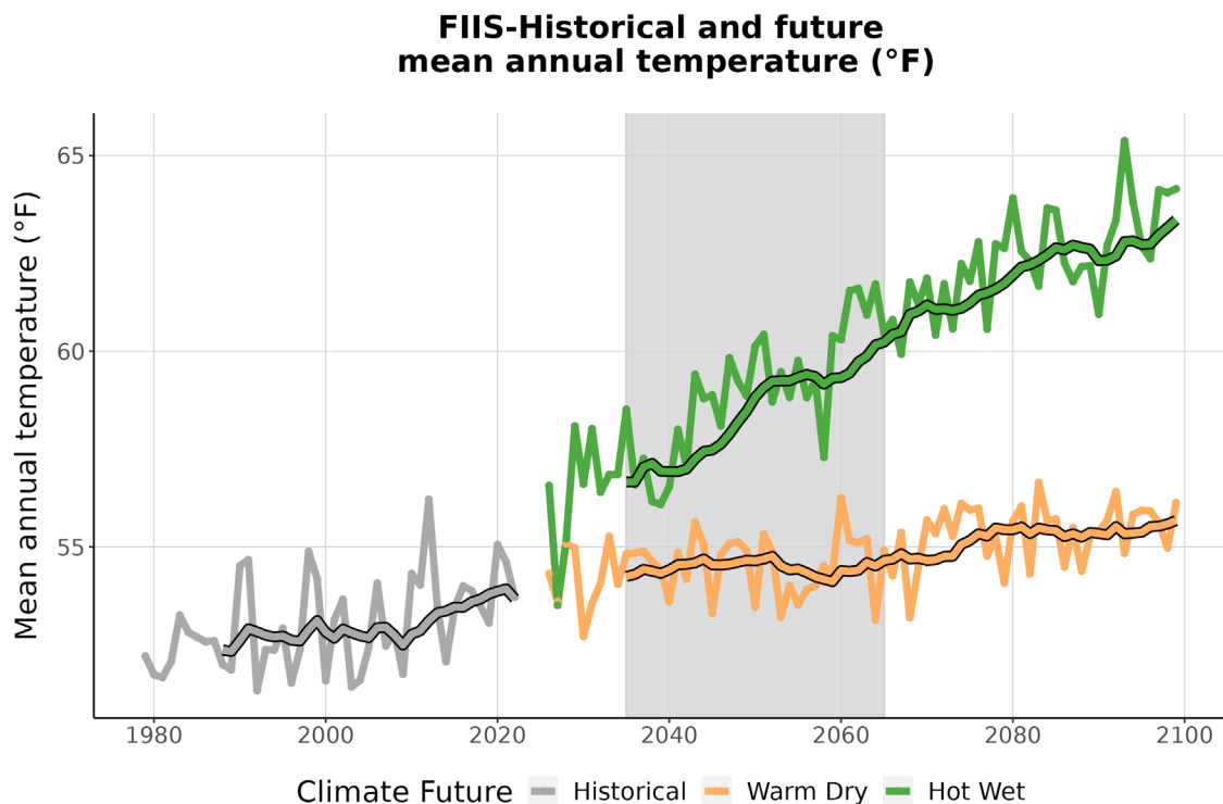
Figure 3. This graph compares observed average annual temperature at FIIS (°F) (1979-2022) with projected average annual temperature for the two climate futures over the period 2023-2099. The historically observed data
