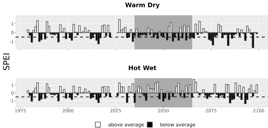
Figure 7. Drought metrics for FIIS. Drought index (SPEI; units = standard deviations from historical) timeseries for each climate future. Below-average SPEI (black bars) indicates dry conditions. The dotted line (SPEI = -0.5) indicates drought conditions.
