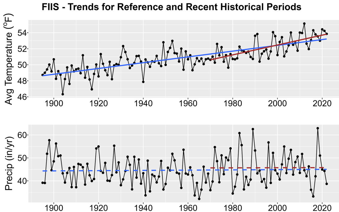
Figure 1. Historical trends in annual average temperature (upper plot) and annual total precipitation (lower plot) for FIIS from 1895-2022. Black points show yearly values while blue lines are linear regressions for the entire period record and red lines for 1970-2022 trends. Solid lines are significant trends (i.e., p < 0.05 ); dashed lines are not statistically significant.
