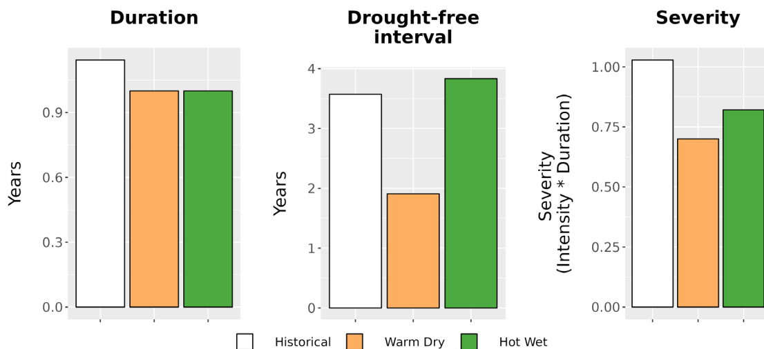
Figure 8. Drought metrics for FIIS. (Left) Average drought duration (years) historically (1979-2012) and under each climate future. (Middle) Average drought return interval (years), indicating the expected amount of time between periods of drought, historically and under each climate future. (Right) Average drought severity, a measure of drought intensity multiplied by duration, historically and under each climate future.
