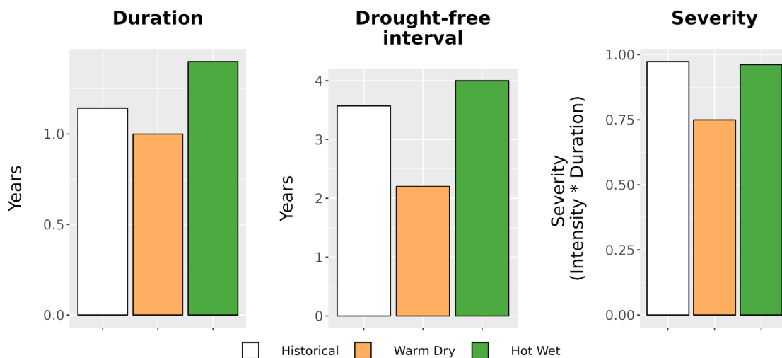
Figure 8. Drought metrics for FEHA. (Left) Average drought duration (years) historically (1979-2012) and under each climate future. (Middle) Average drought return interval (years), indicating the expected amount of time between periods of drought, historically and under each climate future. (Right) Average drought severity, a measure of drought intensity multiplied by duration, historically and under each climate future.
