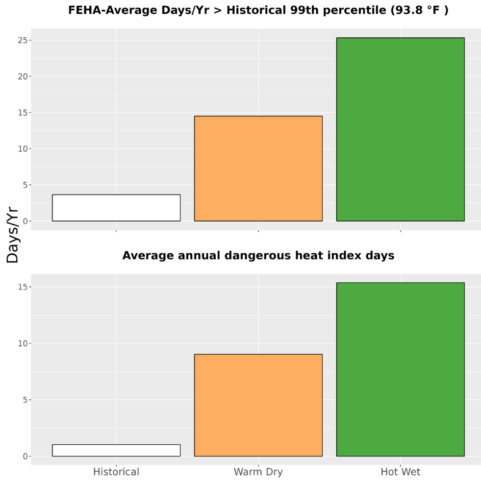
Figure 5. The upper bar graph represents the average number of days annually with temperatures greater than the historical 99th percentile (93.8 °F) historically (1979-2012) and for the two climate futures (2050). The bottom bar graph represents the average annual number of dangerous heat index days historically and for the two climate futures. Dangerous heat index days are days that exceed 105 °F.
