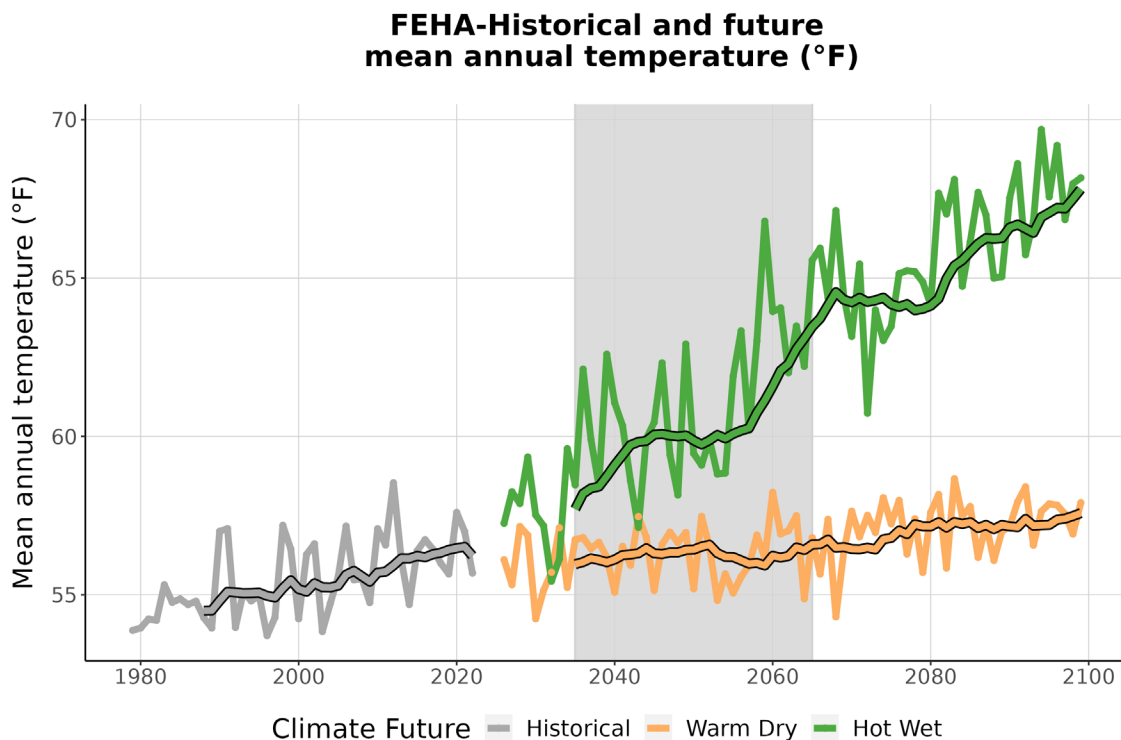
Figure 3. This graph compares observed average annual temperature at FEHA (°F) (1979-2022) with projected average annual temperature for the two climate futures over the period 2023-2099. The historically observed data
