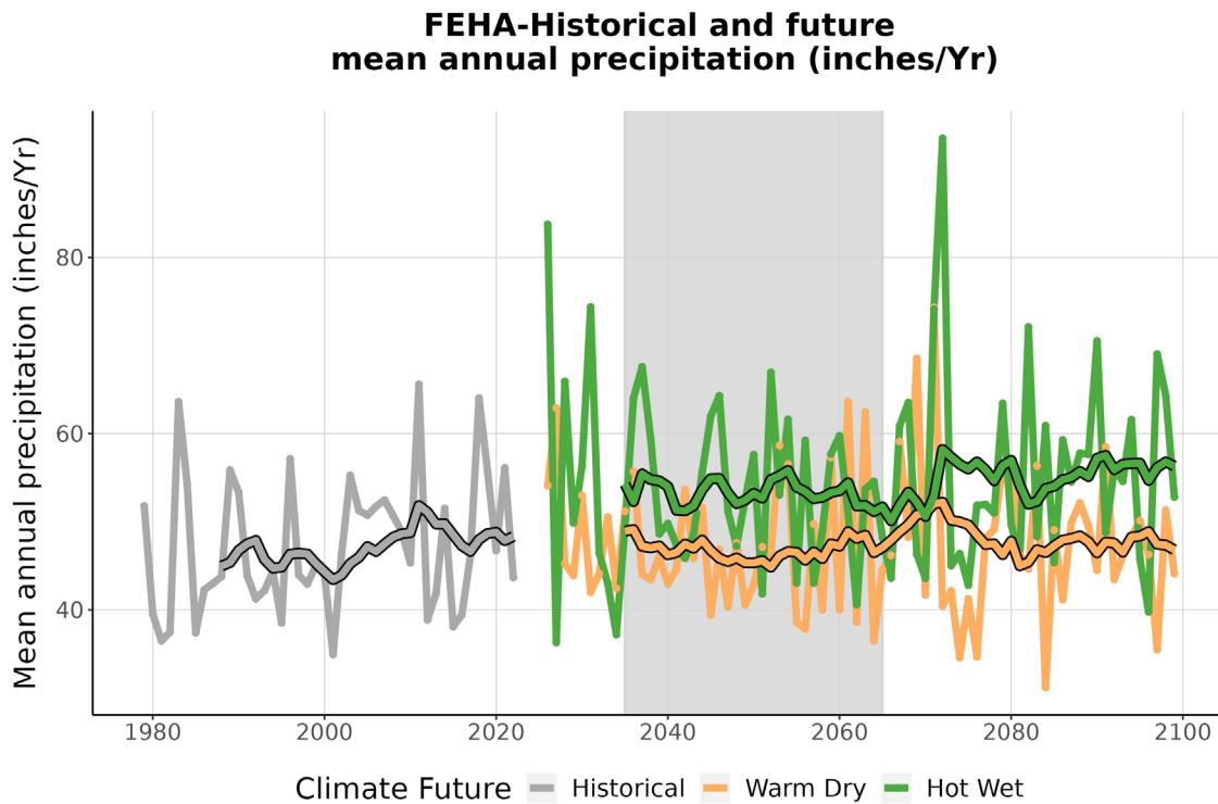
Figure 4. This graph compares observed average annual precipitation at FEHA (inches/year) (1979-2022) with projected average annual precipitation for the two climate futures over the period 2023-2099. The historically observed data is shown in gray, the Warm Dry climate future in orange, and the Hot Wet climate future in green. The smooth line running through each projection is the 10-year running average for historical observations and future projections. The gray-shaded area represents the time period that was averaged (2035-2065) to summarize future projections for the year 2050 (Appendix 1).
