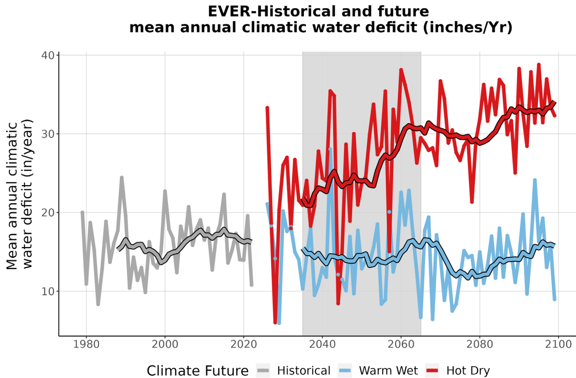
Figure 9. This line graph compares observed climatic water deficit at EVER (inches/year) (1979-2022) with projected climatic water deficit for the two climate futures over the period 2023-2099. The historical observation data is shown in gray, the Warm Wet climate future in blue, and the Hot Dry climate future in red. The smooth line running through each projection is the 10-year running average for historical observations and future projections. Gray-shaded area represents the time period that was averaged (2035-2065) to summarize future projections for the year 2050.
