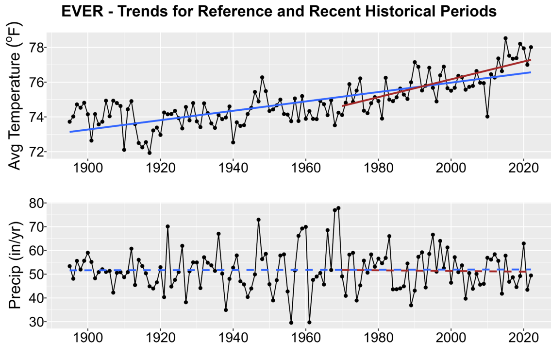
Figure 1. Historical trends in annual average temperature (upper plot) and annual total precipitation (lower plot) for EVER from 1895-2022. Black points show yearly values while blue lines are linear regressions for the entire period record and red lines for 1970-2022 trends. Solid lines are significant trends (i.e., p < 0.05 ); dashed lines are not statistically significant.
