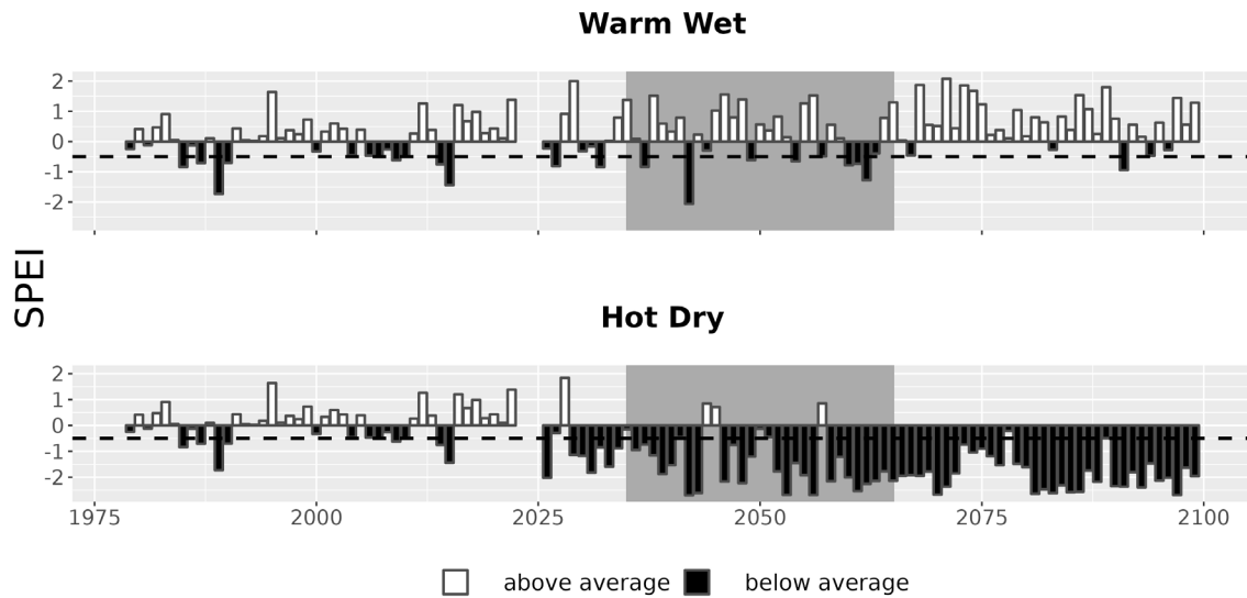
Figure 7. Drought metrics for EVER. Drought index (SPEI; units = standard deviations from historical) timeseries for each climate future. Below-average SPEI (black bars) indicates dry conditions. The dotted line (SPEI = -0.5) indicates drought conditions.
