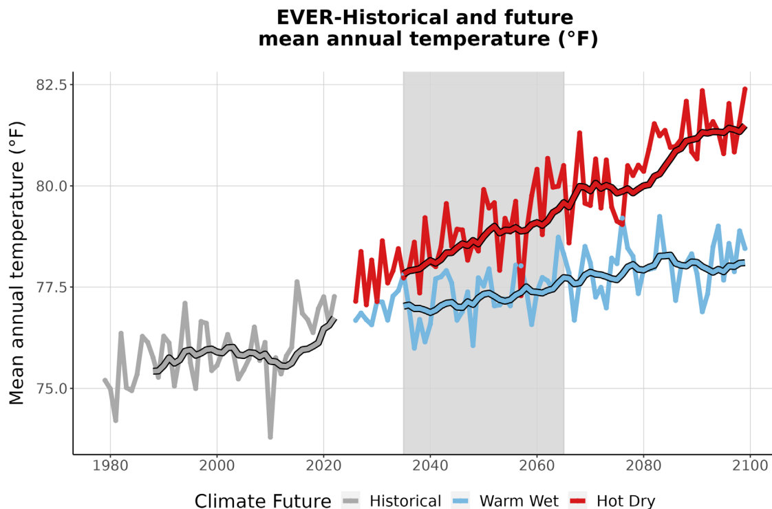
Figure 3. This graph compares observed average annual temperature at EVER (°F) (1979-2022) with projected average annual temperature for the two climate futures over the period 2023-2099. The historically observed data
