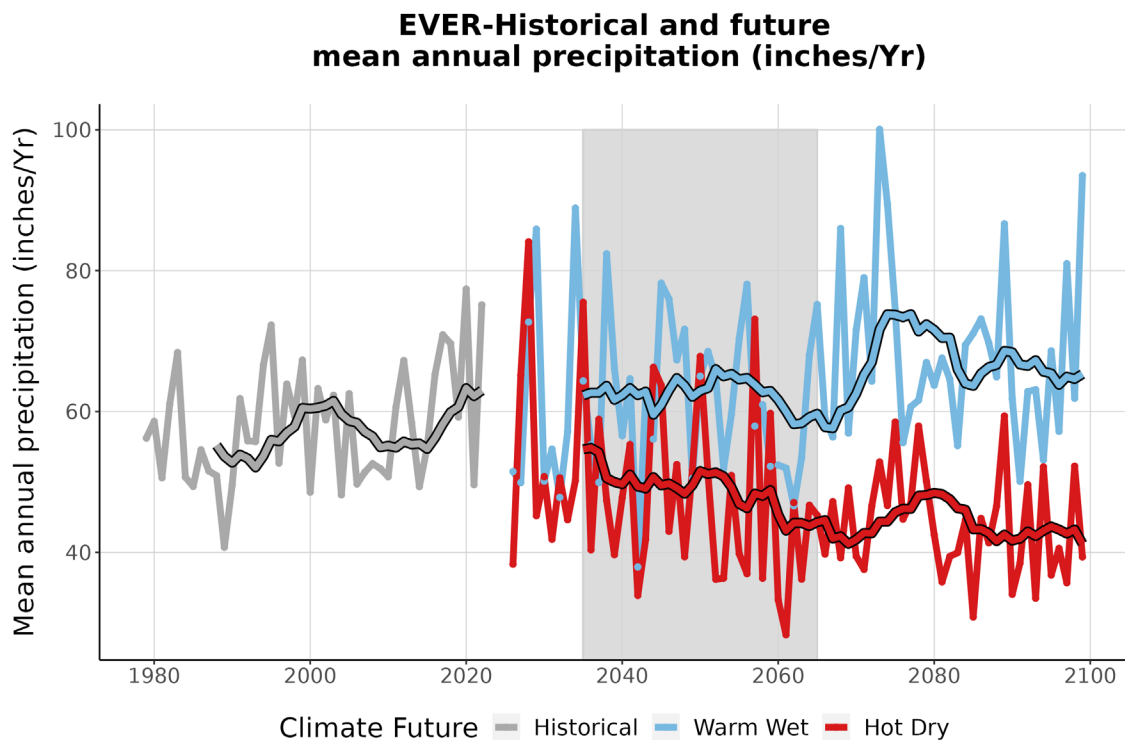
Figure 4. This graph compares observed average annual precipitation at EVER (inches/year) (1979-2022) with projected average annual precipitation for the two climate futures over the period 2023-2099. The historically observed data is shown in gray, the Warm Wet climate future in blue, and the Hot Dry climate future in red. The smooth line running through each projection is the 10-year running average for historical observations and future projections. The gray-shaded area represents the time period that was averaged (2035-2065) to summarize future projections for the year 2050 (Appendix 1).
