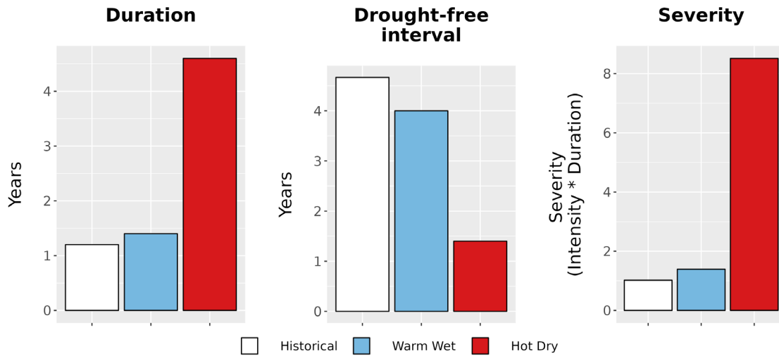
Figure 8. Drought metrics for EVER. (Left) Average drought duration (years) historically (1979-2012) and under each climate future. (Middle) Average drought return interval (years), indicating the expected amount of time between periods of drought, historically and under each climate future. (Right) Average drought severity, a measure of drought intensity multiplied by duration, historically and under each climate future.
