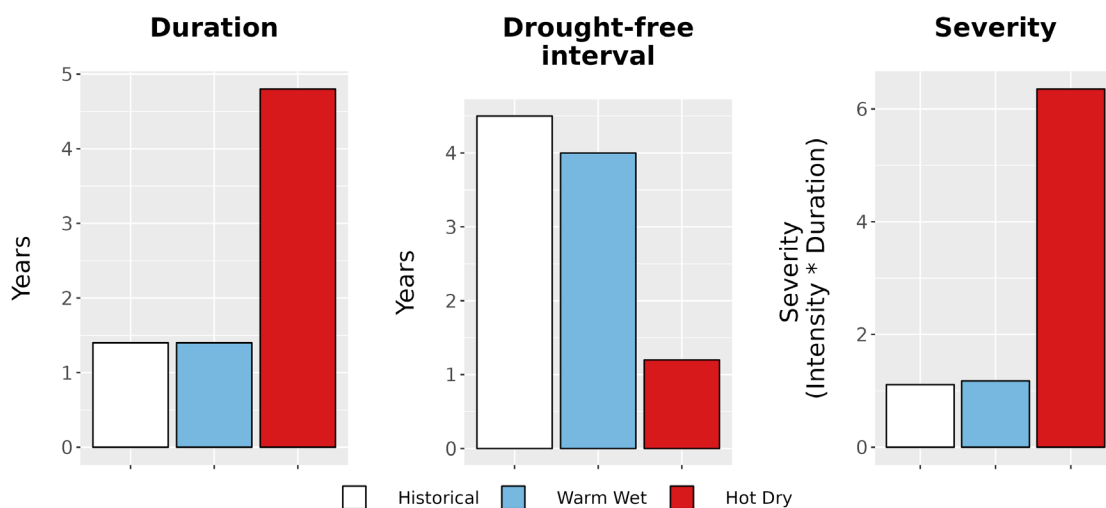
Figure 8. Drought metrics for EUON. (Left) Average drought duration (years) historically (1979-2012) and under each climate future. (Middle) Average drought return interval (years), indicating the expected amount of time between periods of drought, historically and under each climate future. (Right) Average drought severity, a measure of drought intensity multiplied by duration, historically and under each climate future.
