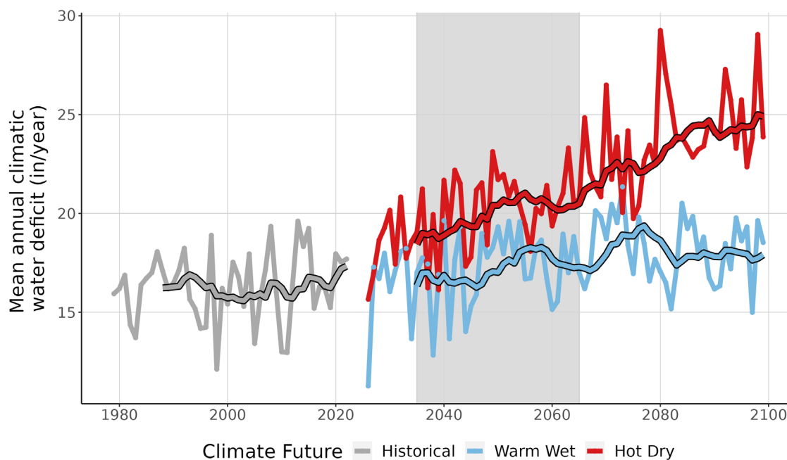
Figure 9. This line graph compares observed climatic water deficit at EUON (inches/year) (1979-2022) with projected climatic water deficit for the two climate futures over the period 2023-2099. The historical observation data is shown in gray, the Warm Wet climate future in blue, and the Hot Dry climate future in red. The smooth line running through each projection is the 10-year running average for historical observations and future projections. Gray-shaded area represents the time period that was averaged (2035-2065) to summarize future projections for the year 2050.
