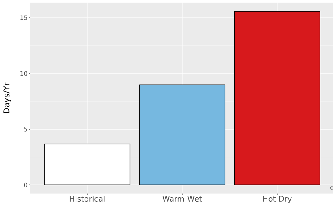
Figure 5. Metrics of extreme temperature at EUON. The bar graph represents the average number of days annually with temperatures greater than the historical 99th percentile (96.7 °F) historically (1979-2012) and for the two climate futures (2050).
