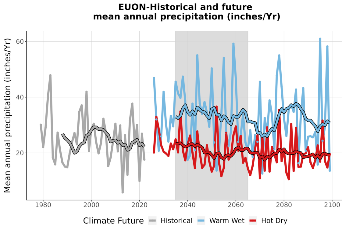
Figure 4. This graph compares observed average annual precipitation at EUON (inches/year) (1979-2022) with projected average annual precipitation for the two climate futures over the period 2023-2099. The historically observed data is shown in gray, the Warm Wet climate future in blue, and the Hot Dry climate future in red. The smooth line running through each projection is the 10-year running average for historical observations and future projections. The gray-shaded area represents the time period that was averaged (2035-2065) to summarize future projections for the year 2050 (Appendix 1).
