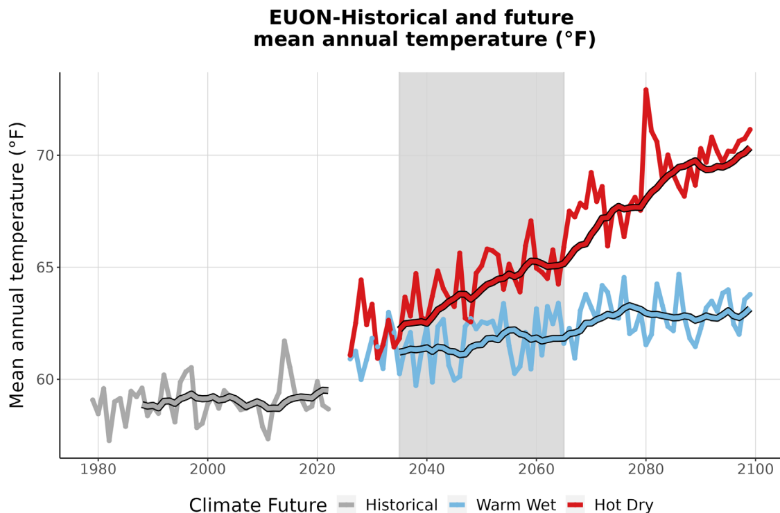
Figure 3. This graph compares observed average annual temperature at EUON (°F) (1979-2022) with projected average annual temperature for the two climate futures over the period 2023-2099. The historically observed data
