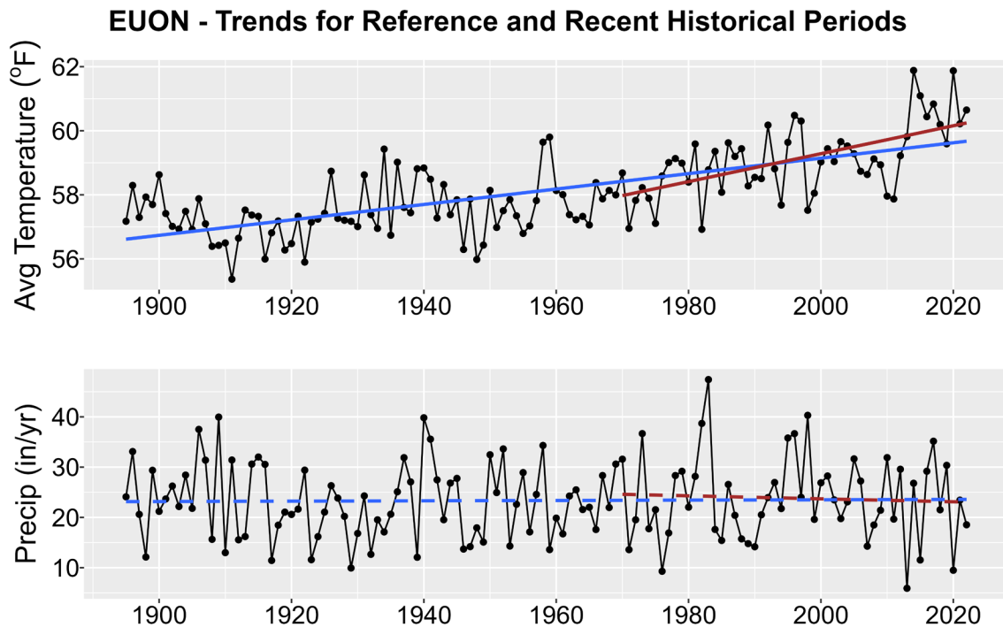
Figure 1. Historical trends in annual average temperature (upper plot) and annual total precipitation (lower plot) for EUON from 1895-2022. Black points show yearly values while blue lines are linear regressions for the entire period record and red lines for 1970-2022 trends. Solid lines are significant trends (i.e., p < 0.05 ); dashed lines are not statistically significant.
