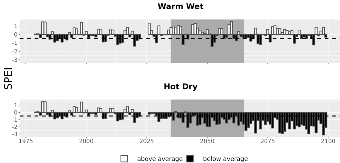
Figure 7. Drought metrics for EUON. Drought index (SPEI; units = standard deviations from historical) timeseries for each climate future. Below-average SPEI (black bars) indicates dry conditions. The dotted line (SPEI = -0.5) indicates drought conditions.
