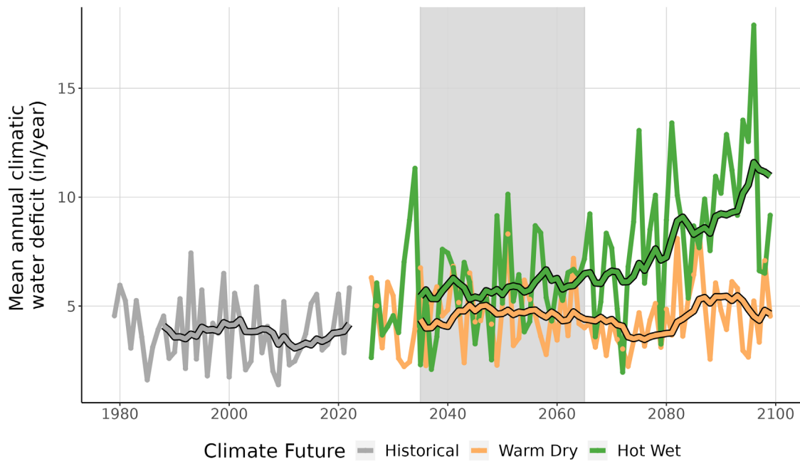
Figure 9. This line graph compares observed climatic water deficit at ELRO (inches/year) (1979-2022) with projected climatic water deficit for the two climate futures over the period 2023-2099. The historical observation data is shown in gray, the Warm Dry climate future in orange, and the Hot Wet climate future in green. The smooth line running through each projection is the 10-year running average for historical observations and future projections. Gray-shaded area represents the time period that was averaged (2035-2065) to summarize future projections for the year 2050.
