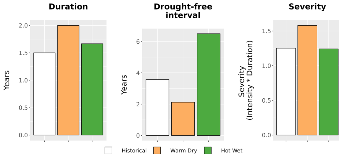
Figure 8. Drought metrics for ELRO. (Left) Average drought duration (years) historically (1979-2012) and under each climate future. (Middle) Average drought return interval (years), indicating the expected amount of time between periods of drought, historically and under each climate future. (Right) Average drought severity, a measure of drought intensity multiplied by duration, historically and under each climate future.
