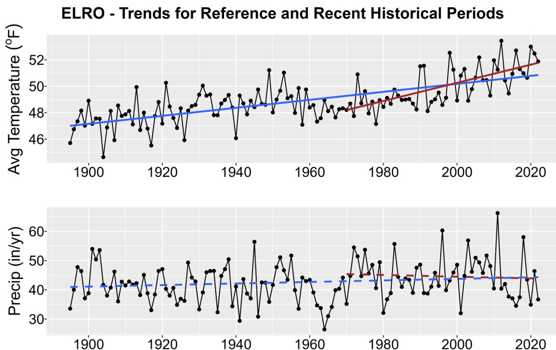
Figure 1. Historical trends in annual average temperature (upper plot) and annual total precipitation (lower plot) for ELRO from 1895-2022. Black points show yearly values while blue lines are linear regressions for the entire period record and red lines for 1970-2022 trends. Solid lines are significant trends (i.e., p < 0.05 ); dashed lines are not statistically significant.
