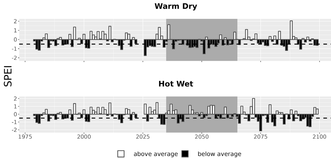
Figure 7. Drought metrics for ELRO. Drought index (SPEI; units = standard deviations from historical) timeseries for each climate future. Below-average SPEI (black bars) indicates dry conditions. The dotted line (SPEI = -0.5) indicates drought conditions.
