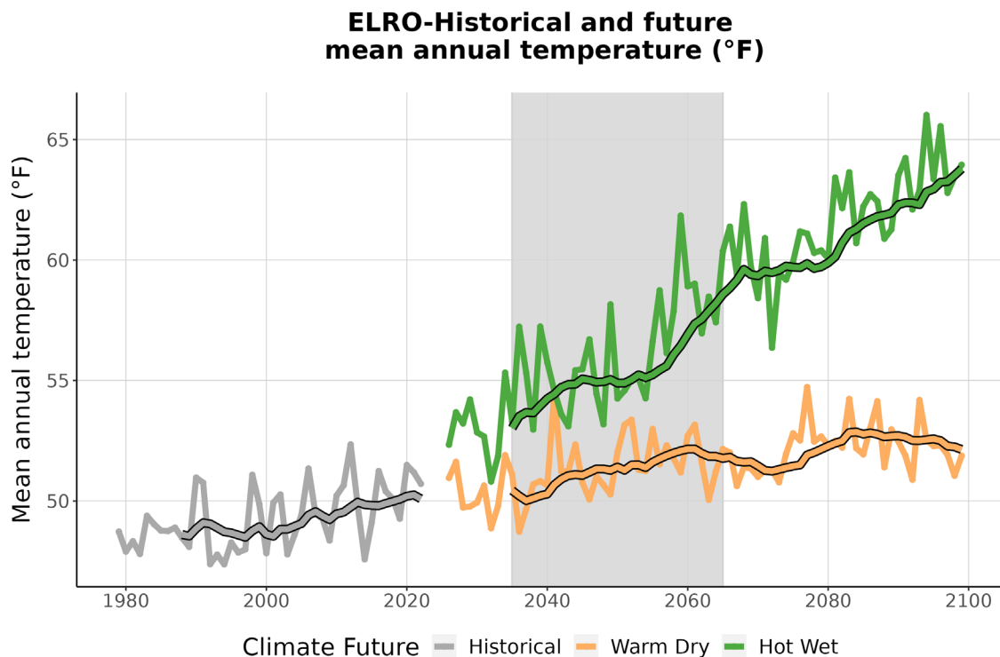
Figure 3. This graph compares observed average annual temperature at ELRO (°F) (1979-2022) with projected average annual temperature for the two climate futures over the period 2023-2099. The historically observed data
