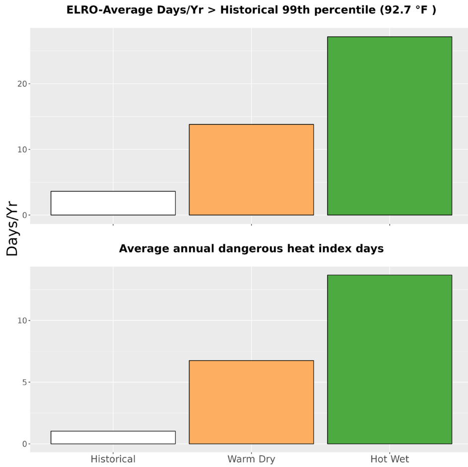
Figure 5. The upper bar graph represents the average number of days annually with temperatures greater than the historical 99th percentile (92.7 °F) historically (1979-2012) and for the two climate futures (2050). The bottom bar graph represents the average annual number of dangerous heat index days historically and for the two climate futures. Dangerous heat index days are days that exceed 105 °F.
