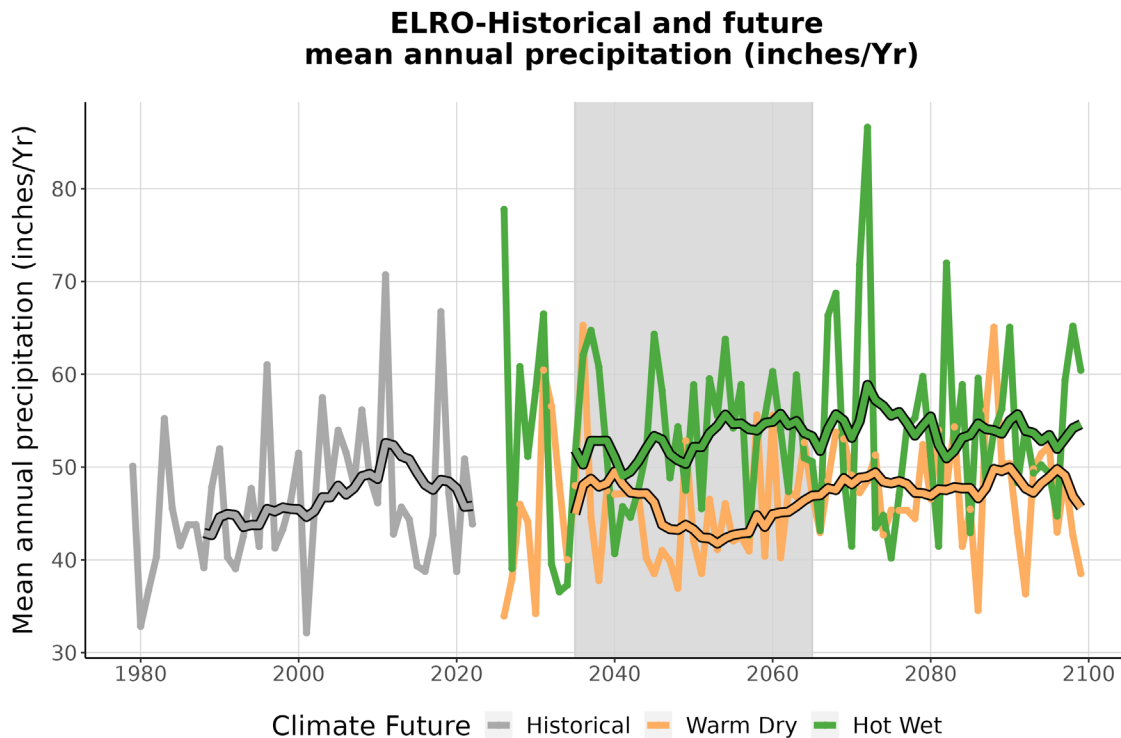
Figure 4. This graph compares observed average annual precipitation at ELRO (inches/year) (1979-2022) with projected average annual precipitation for the two climate futures over the period 2023-2099. The historically observed data is shown in gray, the Warm Dry climate future in orange, and the Hot Wet climate future in green. The smooth line running through each projection is the 10-year running average for historical observations and future projections. The gray-shaded area represents the time period that was averaged (2035-2065) to summarize future projections for the year 2050 (Appendix 1).
