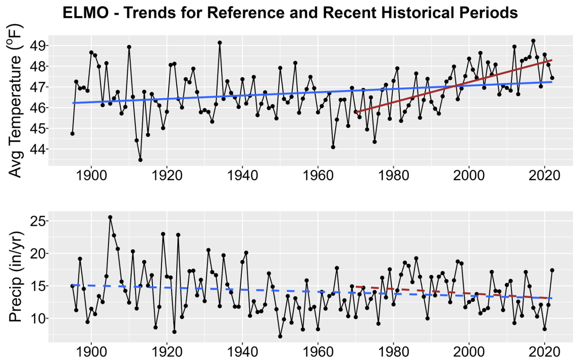
Figure 1. Historical trends in annual average temperature (upper plot) and annual total precipitation (lower plot) for ELMO from 1895-2022. Black points show yearly values while blue lines are linear regressions for the entire period record and red lines for 1970-2022 trends. Solid lines are significant trends (i.e., p < 0.05 ); dashed lines are not statistically significant.
