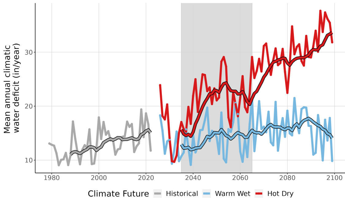
Figure 9. This line graph compares observed climatic water deficit at ELMO (inches/year) (1979-2022) with projected climatic water deficit for the two climate futures over the period 2023-2099. The historical observation data is shown in gray, the Warm Wet climate future in blue, and the Hot Dry climate future in red. The smooth line running through each projection is the 10-year running average for historical observations and future projections. Gray-shaded area represents the time period that was averaged (2035-2065) to summarize future projections for the year 2050.
