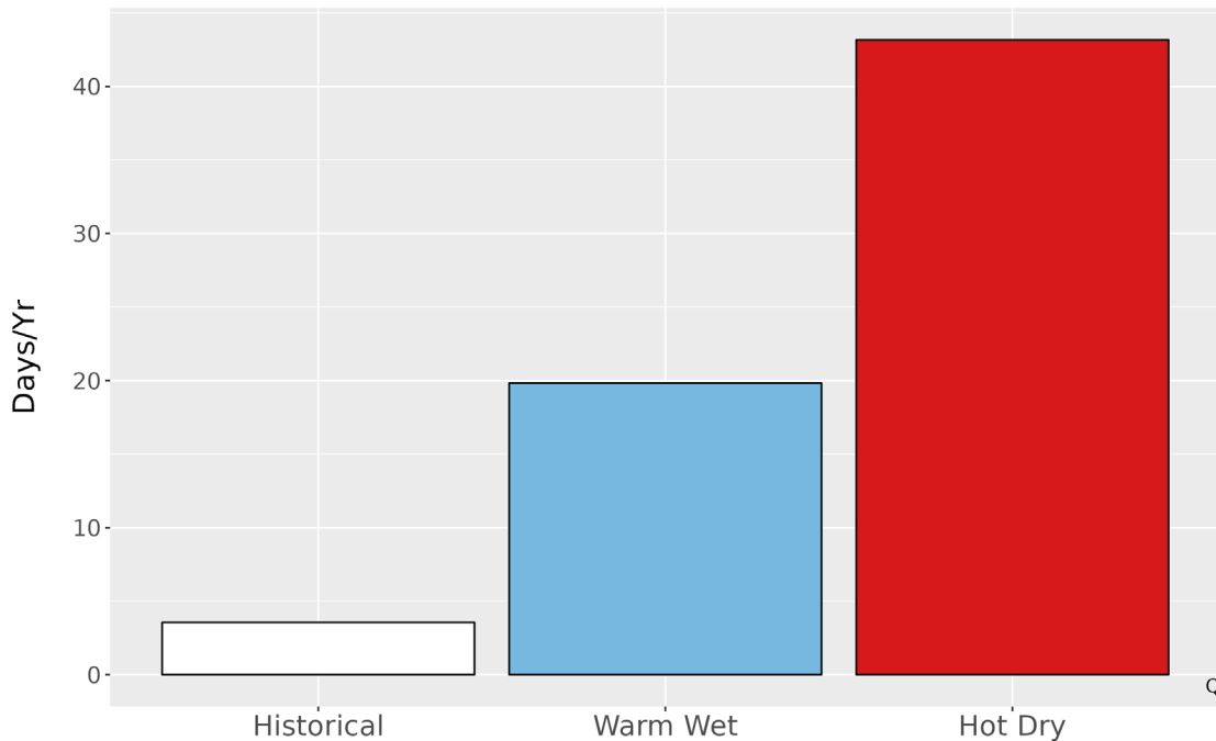
Figure 5. Metrics of extreme temperature at ELMO. The bar graph represents the average number of days annually with temperatures greater than the historical 99th percentile (90.9 °F) historically (1979-2012) and for the two climate futures (2050).
