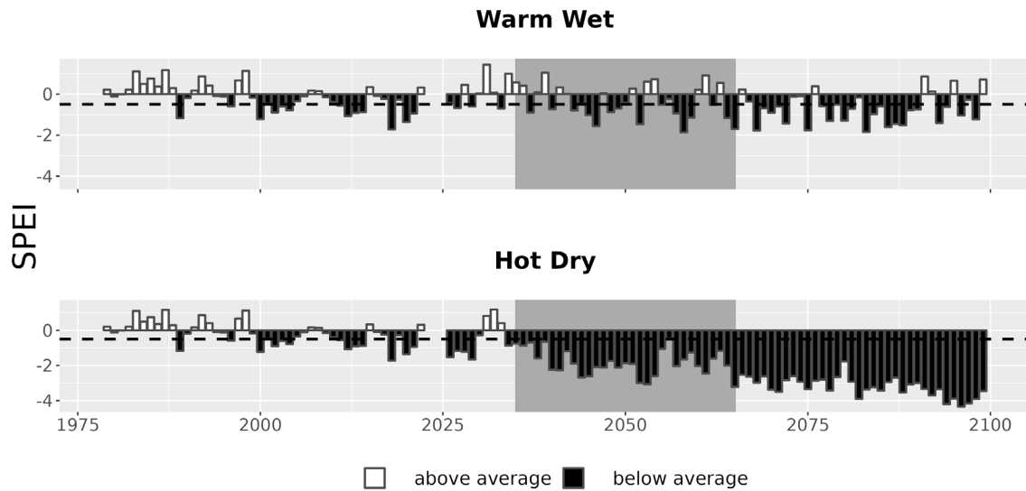
Figure 7. Drought metrics for ELMO. Drought index (SPEI; units = standard deviations from historical) timeseries for each climate future. Below-average SPEI (black bars) indicates dry conditions. The dotted line (SPEI = -0.5) indicates drought conditions.
