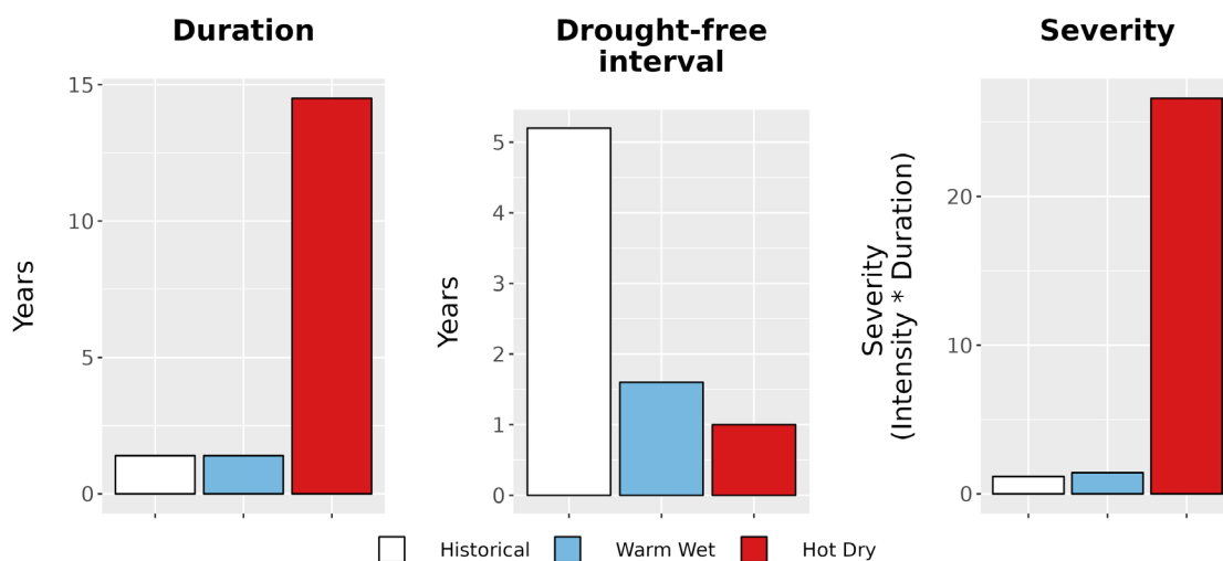
Figure 8. Drought metrics for ELMO. (Left) Average drought duration (years) historically (1979-2012) and under each climate future. (Middle) Average drought return interval (years), indicating the expected amount of time between periods of drought, historically and under each climate future. (Right) Average drought severity, a measure of drought intensity multiplied by duration, historically and under each climate future.
