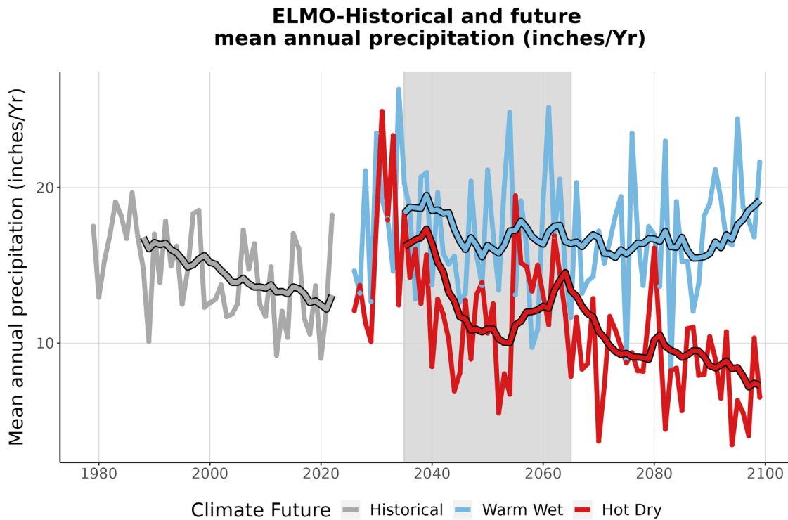
Figure 4. This graph compares observed average annual precipitation at ELMO (inches/year) (1979-2022) with projected average annual precipitation for the two climate futures over the period 2023-2099. The historically observed data is shown in gray, the Warm Wet climate future in blue, and the Hot Dry climate future in red. The smooth line running through each projection is the 10-year running average for historical observations and future projections. The gray-shaded area represents the time period that was averaged (2035-2065) to summarize future projections for the year 2050 (Appendix 1).
