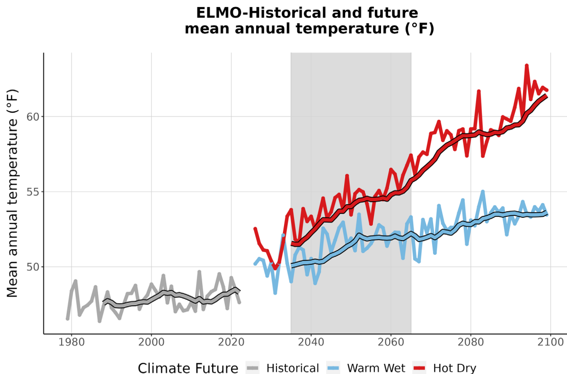
Figure 3. This graph compares observed average annual temperature at ELMO (°F) (1979-2022) with projected average annual temperature for the two climate futures over the period 2023-2099. The historically observed data
