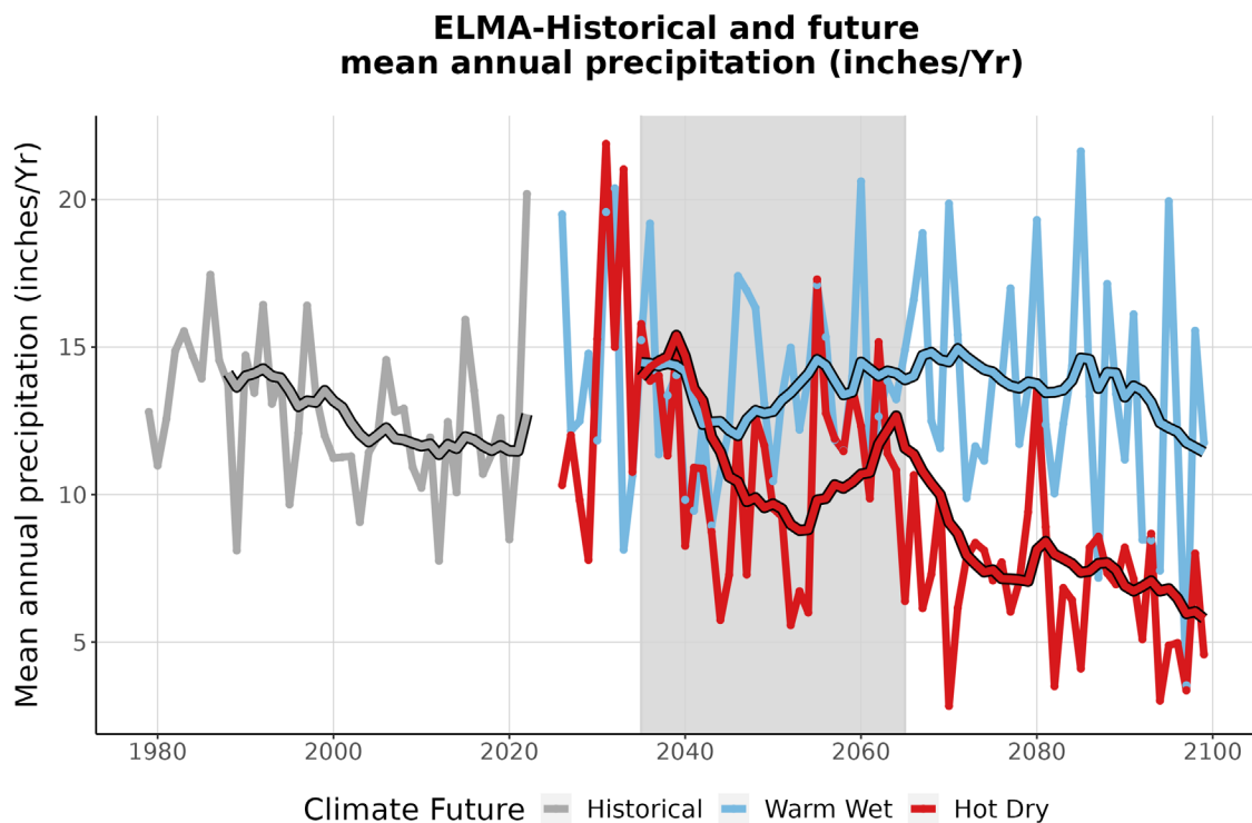
Figure 4. This graph compares observed average annual precipitation at ELMA (inches/year) (1979-2022) with projected average annual precipitation for the two climate futures over the period 2023-2099. The historically observed data is shown in gray, the Warm Wet climate future in blue, and the Hot Dry climate future in red. The smooth line running through each projection is the 10-year running average for historical observations and future projections. The gray-shaded area represents the time period that was averaged (2035-2065) to summarize future projections for the year 2050 (Appendix 1).
