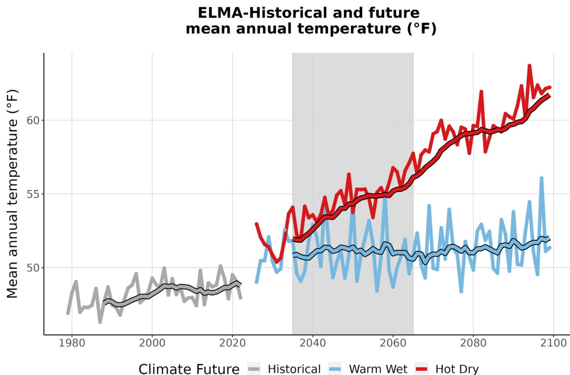
Figure 3. This graph compares observed average annual temperature at ELMA (°F) (1979-2022) with projected average annual temperature for the two climate futures over the period 2023-2099. The historically observed data
