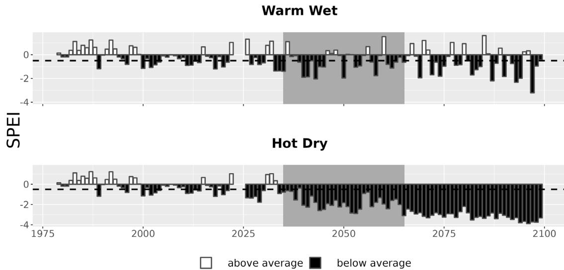
Figure 7. Drought metrics for ELMA. Drought index (SPEI; units = standard deviations from historical) timeseries for each climate future. Below-average SPEI (black bars) indicates dry conditions. The dotted line (SPEI = -0.5) indicates drought conditions.
