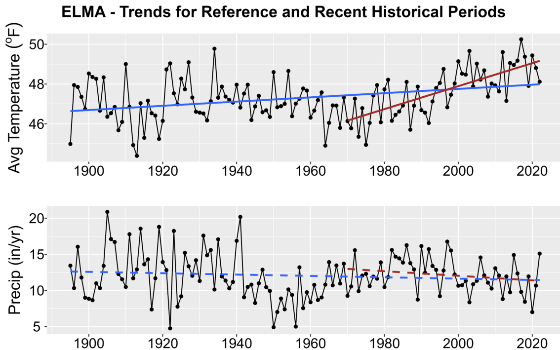
Figure 1. Historical trends in annual average temperature (upper plot) and annual total precipitation (lower plot) for ELMA from 1895-2022. Black points show yearly values while blue lines are linear regressions for the entire period record and red lines for 1970-2022 trends. Solid lines are significant trends (i.e., p < 0.05 ); dashed lines are not statistically significant.
