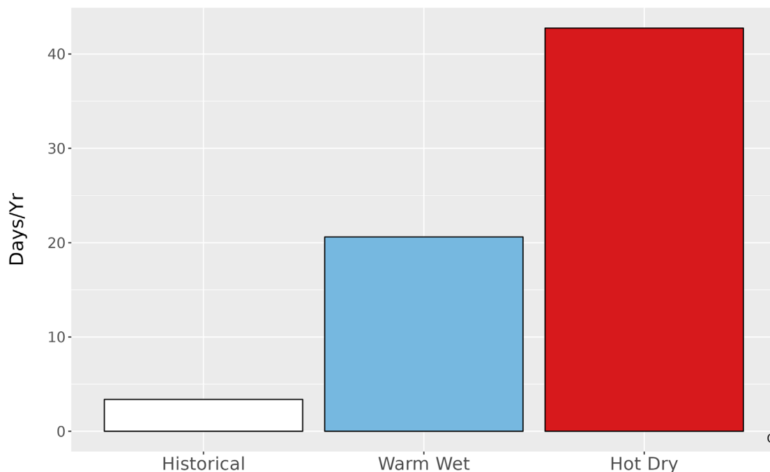
Figure 5. Metrics of extreme temperature at ELMA. The bar graph represents the average number of days annually with temperatures greater than the historical 99th percentile (90.8 °F) historically (1979-2012) and for the two climate futures (2050).
