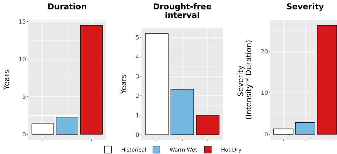
Figure 8. Drought metrics for ELMA. (Left) Average drought duration (years) historically (1979-2012) and under each climate future. (Middle) Average drought return interval (years), indicating the expected amount of time between periods of drought, historically and under each climate future. (Right) Average drought severity, a measure of drought intensity multiplied by duration, historically and under each climate future.
