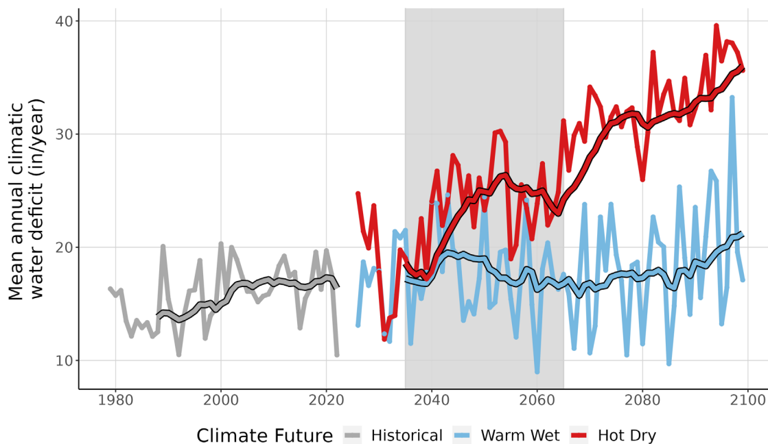
Figure 9. This line graph compares observed climatic water deficit at ELMA (inches/year) (1979-2022) with projected climatic water deficit for the two climate futures over the period 2023-2099. The historical observation data is shown in gray, the Warm Wet climate future in blue, and the Hot Dry climate future in red. The smooth line running through each projection is the 10-year running average for historical observations and future projections. Gray-shaded area represents the time period that was averaged (2035-2065) to summarize future projections for the year 2050.
