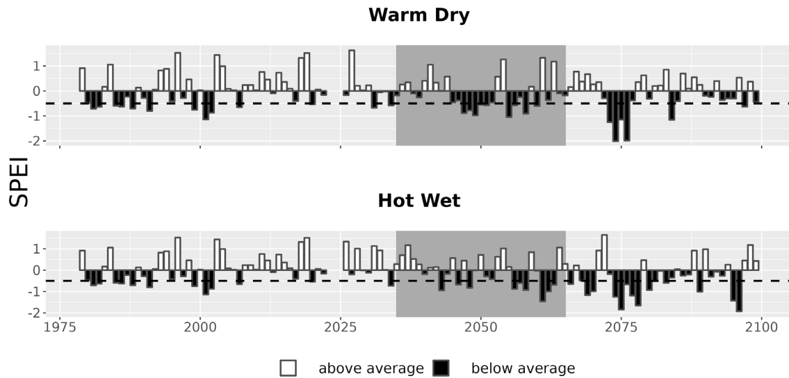
Figure 7. Drought metrics for EISE. Drought index (SPEI; units = standard deviations from historical) timeseries for each climate future. Below-average SPEI (black bars) indicates dry conditions. The dotted line (SPEI = -0.5) indicates drought conditions.
