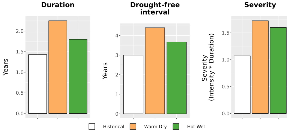
Figure 8. Drought metrics for EISE. (Left) Average drought duration (years) historically (1979-2012) and under each climate future. (Middle) Average drought return interval (years), indicating the expected amount of time between periods of drought, historically and under each climate future. (Right) Average drought severity, a measure of drought intensity multiplied by duration, historically and under each climate future.
