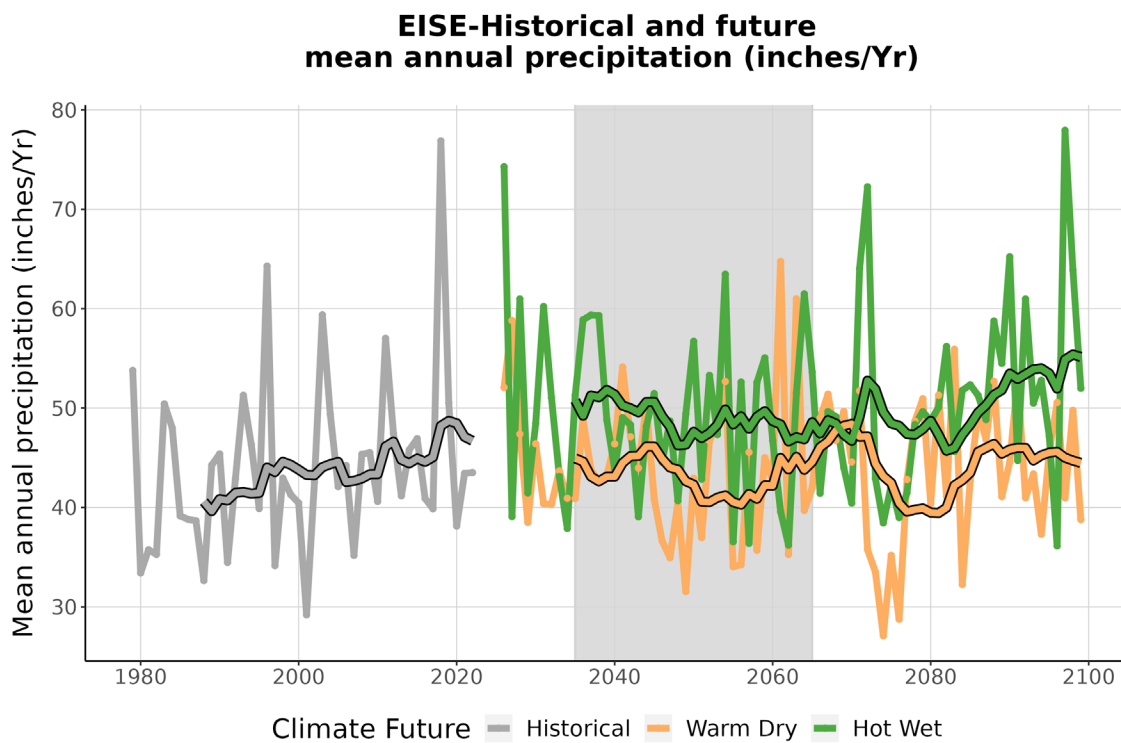
Figure 4. This graph compares observed average annual precipitation at EISE (inches/year) (1979-2022) with projected average annual precipitation for the two climate futures over the period 2023-2099. The historically observed data is shown in gray, the Warm Dry climate future in orange, and the Hot Wet climate future in green. The smooth line running through each projection is the 10-year running average for historical observations and future projections. The gray-shaded area represents the time period that was averaged (2035-2065) to summarize future projections for the year 2050 (Appendix 1).
