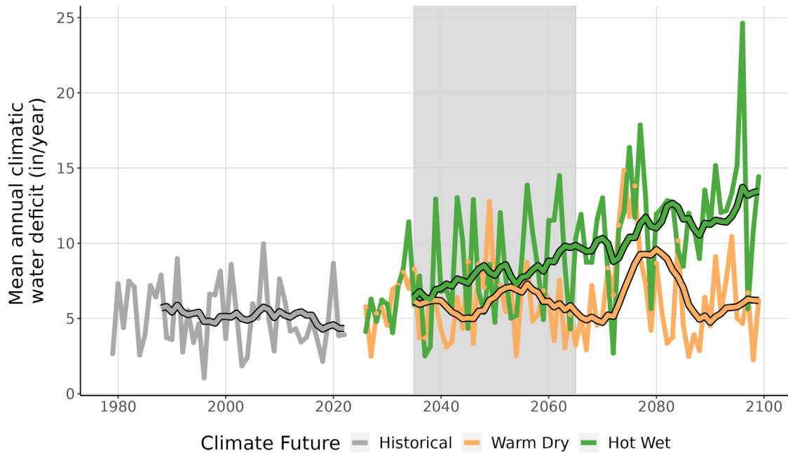
Figure 9. This line graph compares observed climatic water deficit at EISE (inches/year) (1979-2022) with projected climatic water deficit for the two climate futures over the period 2023-2099. The historical observation data is shown in gray, the Warm Dry climate future in orange, and the Hot Wet climate future in green. The smooth line running through each projection is the 10-year running average for historical observations and future projections. Gray-shaded area represents the time period that was averaged (2035-2065) to summarize future projections for the year 2050.
