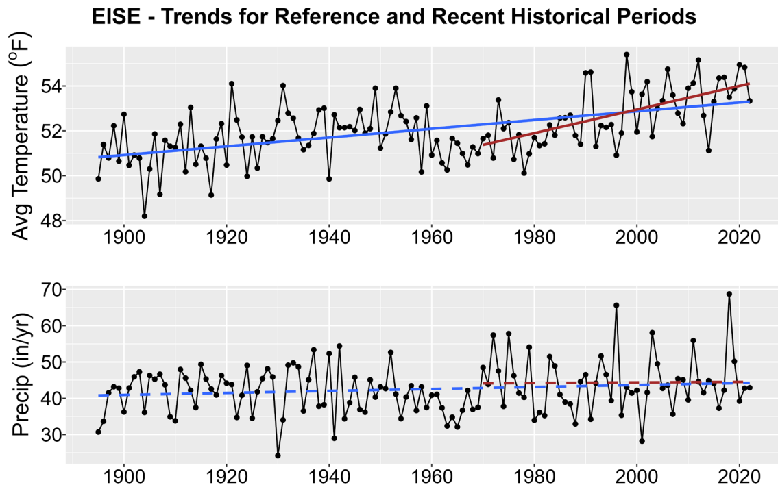
Figure 1. Historical trends in annual average temperature (upper plot) and annual total precipitation (lower plot) for EISE from 1895-2022. Black points show yearly values while blue lines are linear regressions for the entire period record and red lines for 1970-2022 trends. Solid lines are significant trends (i.e., p < 0.05 ); dashed lines are not statistically significant.
