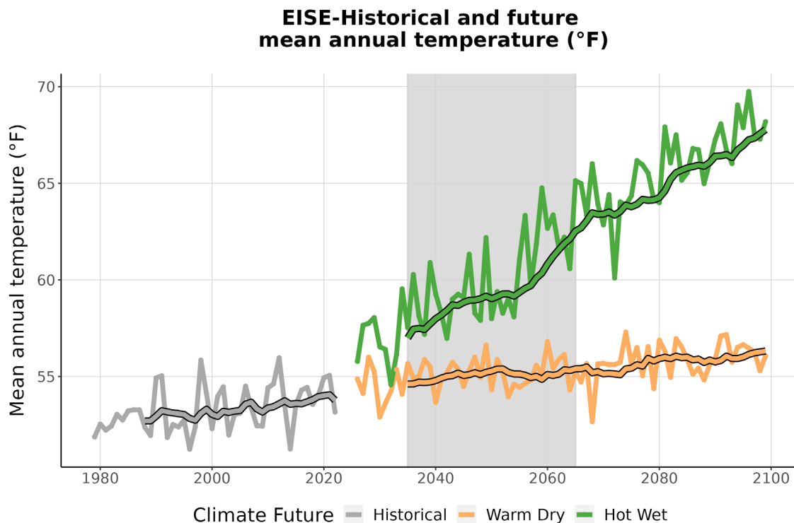
Figure 3. This graph compares observed average annual temperature at EISE (°F) (1979-2022) with projected average annual temperature for the two climate futures over the period 2023-2099. The historically observed data
