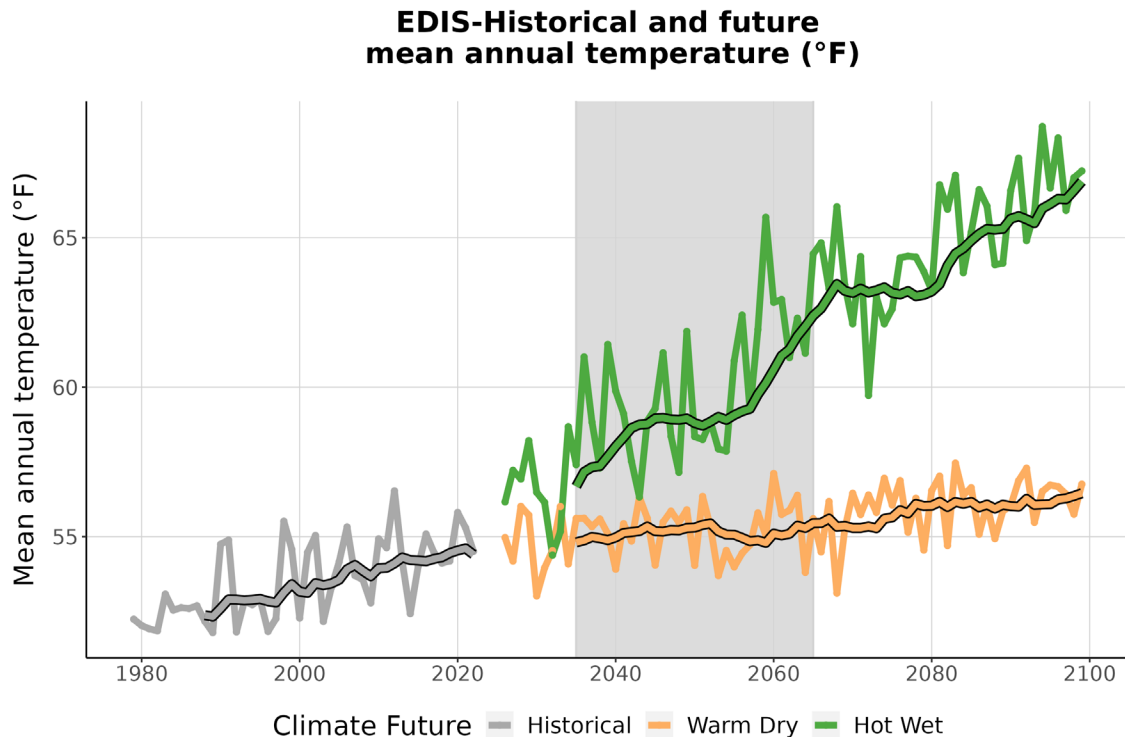
Figure 3. This graph compares observed average annual temperature at EDIS (°F) (1979-2022) with projected average annual temperature for the two climate futures over the period 2023-2099. The historically observed data
