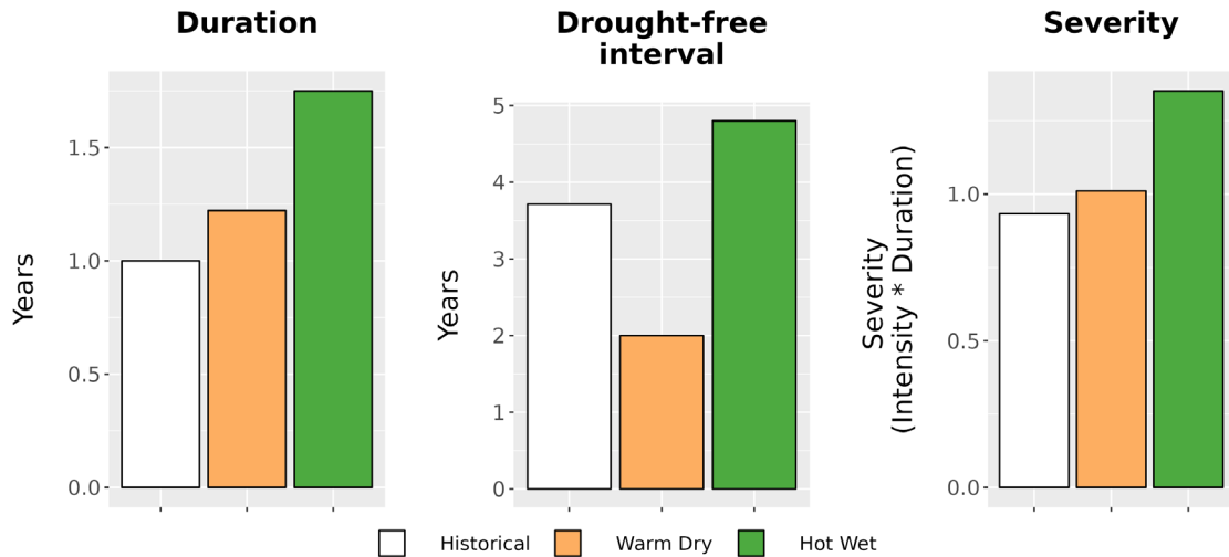
Figure 8. Drought metrics for EDIS. (Left) Average drought duration (years) historically (1979-2012) and under each climate future. (Middle) Average drought return interval (years), indicating the expected amount of time between periods of drought, historically and under each climate future. (Right) Average drought severity, a measure of drought intensity multiplied by duration, historically and under each climate future.
