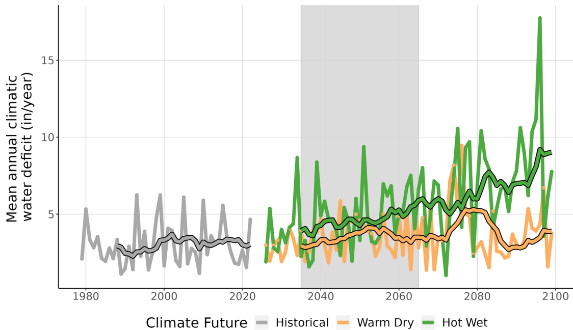
Figure 9. This line graph compares observed climatic water deficit at EDIS (inches/year) (1979-2022) with projected climatic water deficit for the two climate futures over the period 2023-2099. The historical observation data is shown in gray, the Warm Dry climate future in orange, and the Hot Wet climate future in green. The smooth line running through each projection is the 10-year running average for historical observations and future projections. Gray-shaded area represents the time period that was averaged (2035-2065) to summarize future projections for the year 2050.
