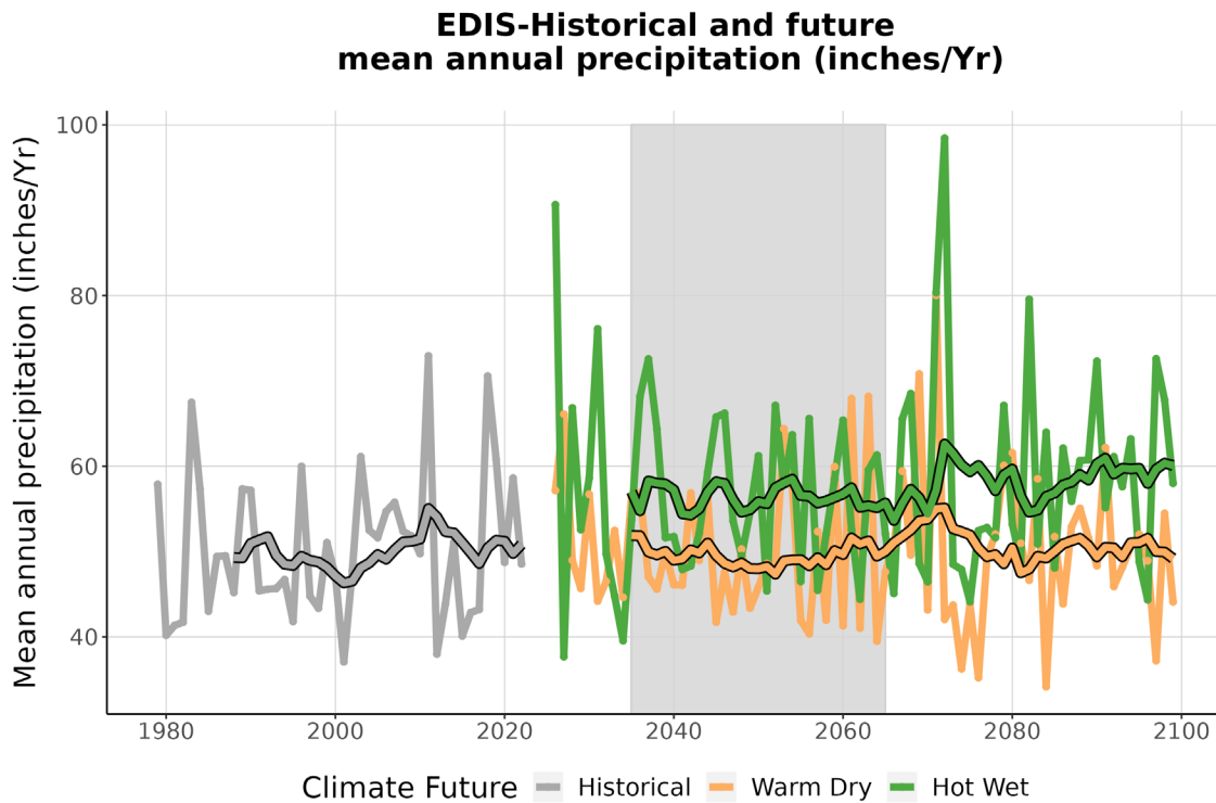
Figure 4. This graph compares observed average annual precipitation at EDIS (inches/year) (1979-2022) with projected average annual precipitation for the two climate futures over the period 2023-2099. The historically observed data is shown in gray, the Warm Dry climate future in orange, and the Hot Wet climate future in green. The smooth line running through each projection is the 10-year running average for historical observations and future projections. The gray-shaded area represents the time period that was averaged (2035-2065) to summarize future projections for the year 2050 (Appendix 1).
