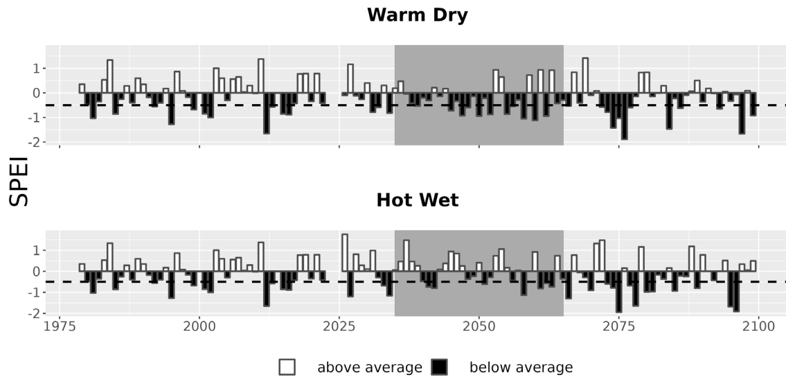
Figure 7. Drought metrics for EDIS. Drought index (SPEI; units = standard deviations from historical) timeseries for each climate future. Below-average SPEI (black bars) indicates dry conditions. The dotted line (SPEI = -0.5) indicates drought conditions.
