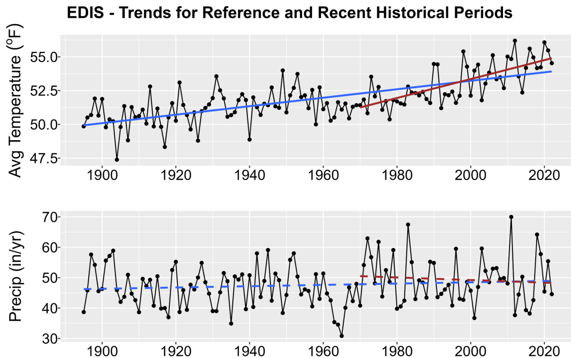
Figure 1. Historical trends in annual average temperature (upper plot) and annual total precipitation (lower plot) for EDIS from 1895-2022. Black points show yearly values while blue lines are linear regressions for the entire period record and red lines for 1970-2022 trends. Solid lines are significant trends (i.e., p < 0.05 ); dashed lines are not statistically significant.
