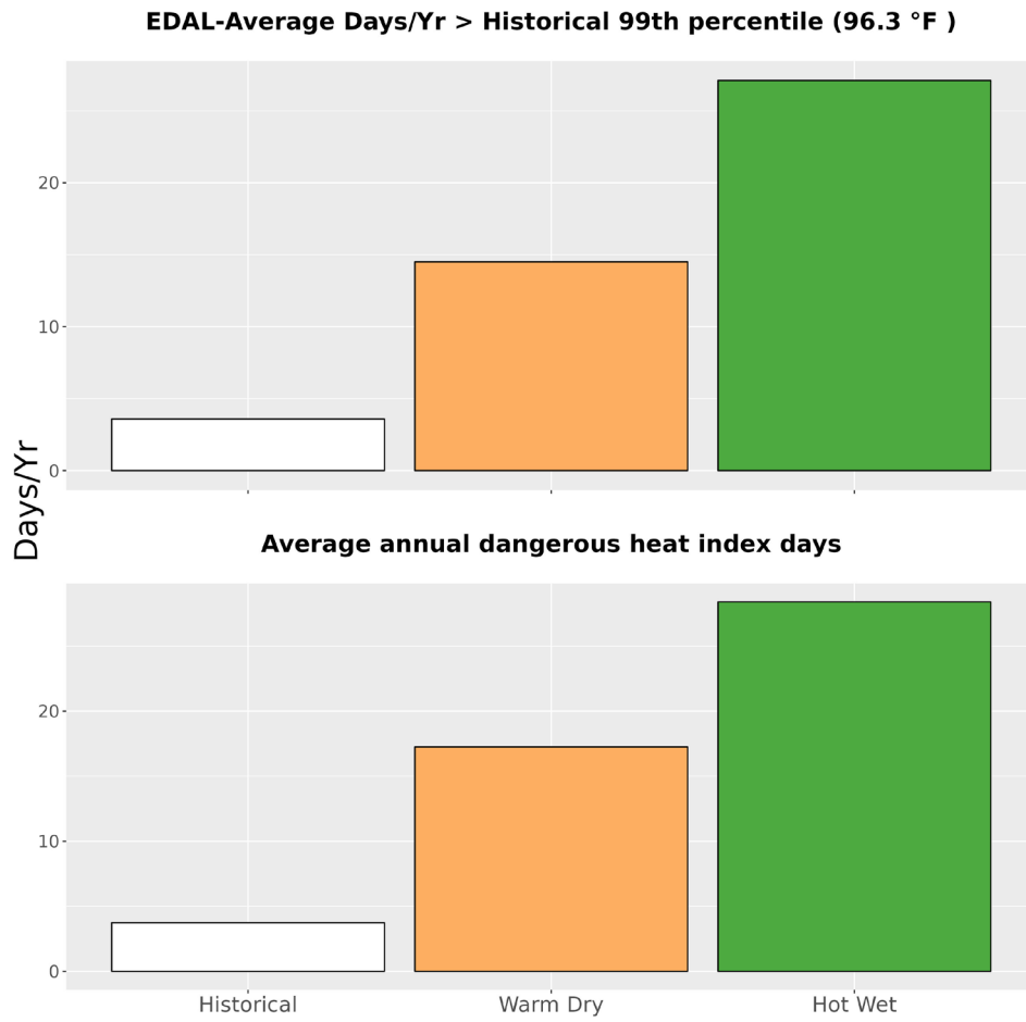
Figure 5. The upper bar graph represents the average number of days annually with temperatures greater than the historical 99th percentile (96.3 °F) historically (1979-2012) and for the two climate futures (2050). The bottom bar graph represents the average annual number of dangerous heat index days historically and for the two climate futures. Dangerous heat index days are days that exceed 105 °F.
