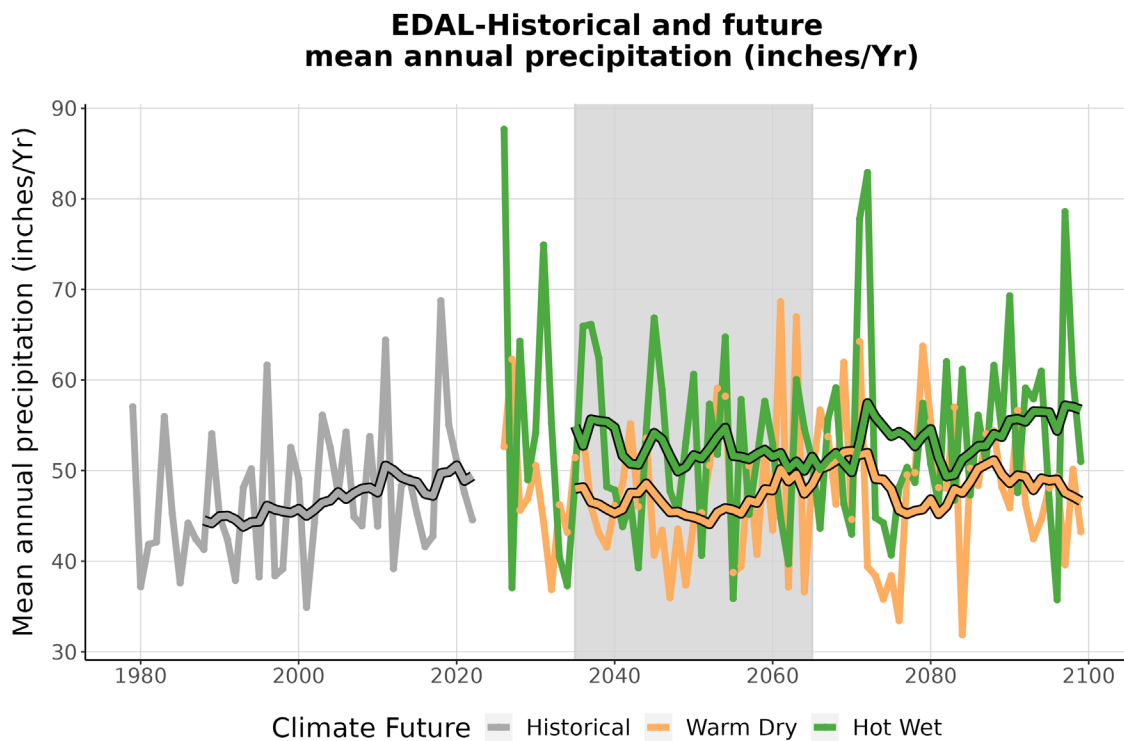
Figure 4. This graph compares observed average annual precipitation at EDAL (inches/year) (1979-2022) with projected average annual precipitation for the two climate futures over the period 2023-2099. The historically observed data is shown in gray, the Warm Dry climate future in orange, and the Hot Wet climate future in green. The smooth line running through each projection is the 10-year running average for historical observations and future projections. The gray-shaded area represents the time period that was averaged (2035-2065) to summarize future projections for the year 2050 (Appendix 1).
