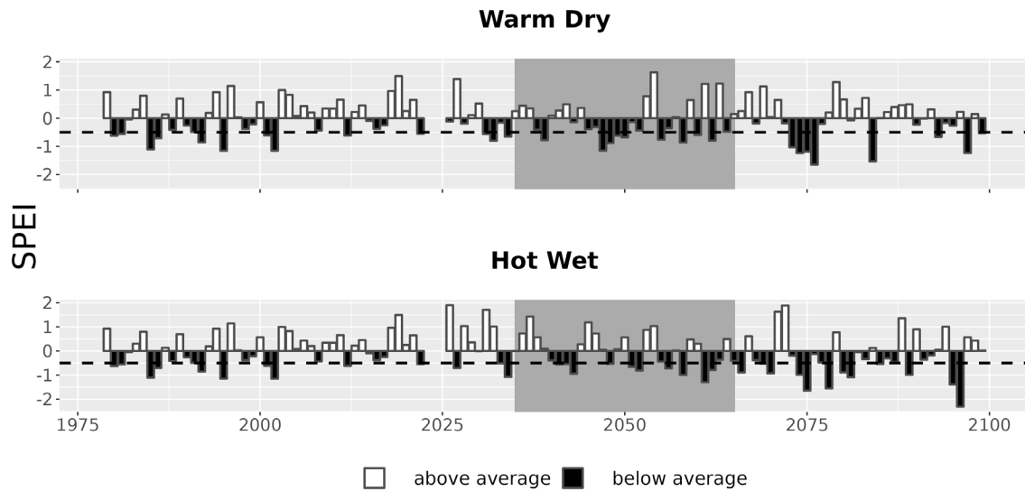
Figure 7. Drought metrics for EDAL. Drought index (SPEI; units = standard deviations from historical) timeseries for each climate future. Below-average SPEI (black bars) indicates dry conditions. The dotted line (SPEI = -0.5) indicates drought conditions.
