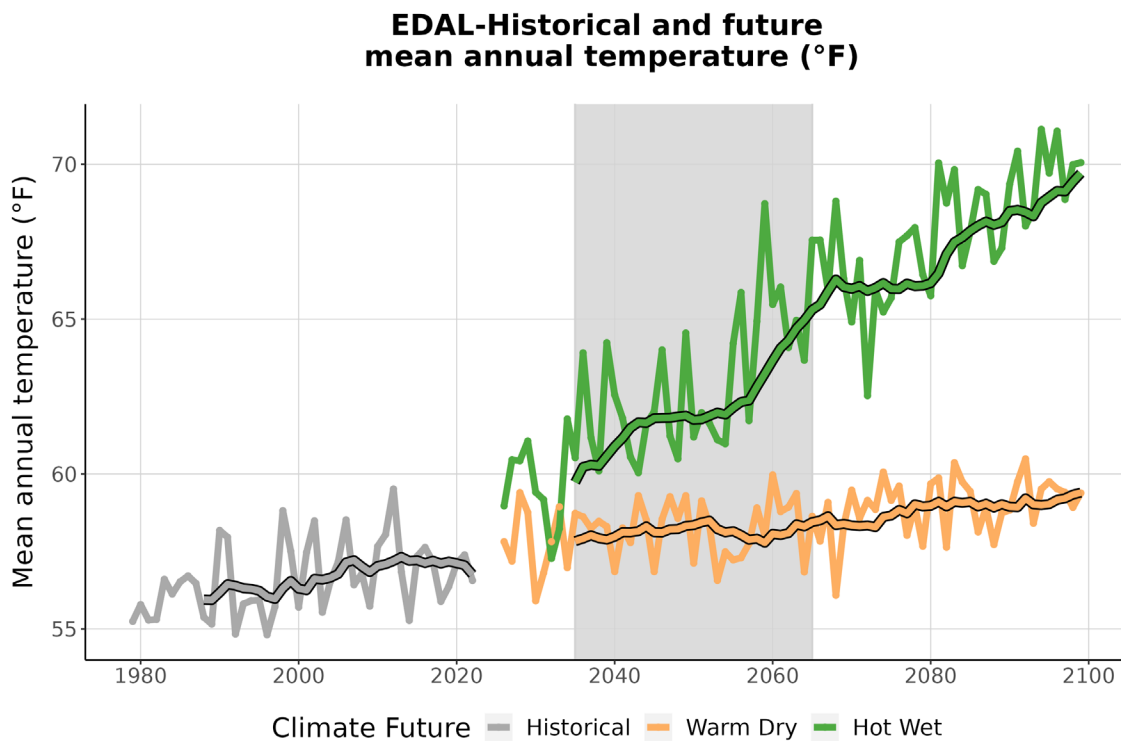
Figure 3. This graph compares observed average annual temperature at EDAL (°F) (1979-2022) with projected average annual temperature for the two climate futures over the period 2023-2099. The historically observed data is shown in gray, the Warm Dry climate future in orange, and the Hot Wet climate future in green. The smooth line
