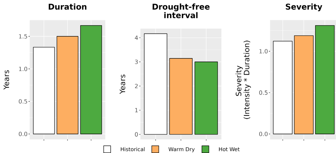
Figure 8. Drought metrics for EDAL. (Left) Average drought duration (years) historically (1979-2012) and under each climate future. (Middle) Average drought return interval (years), indicating the expected amount of time between periods of drought, historically and under each climate future. (Right) Average drought severity, a measure of drought intensity multiplied by duration, historically and under each climate future.
