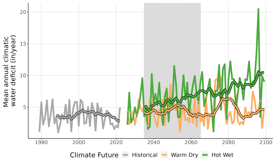
Figure 9. This line graph compares observed climatic water deficit at EDAL (inches/year) (1979-2022) with projected climatic water deficit for the two climate futures over the period 2023-2099. The historical observation data is shown in gray, the Warm Dry climate future in orange, and the Hot Wet climate future in green. The smooth line running through each projection is the 10-year running average for historical observations and future projections. Gray-shaded area represents the time period that was averaged (2035-2065) to summarize future projections for the year 2050.
