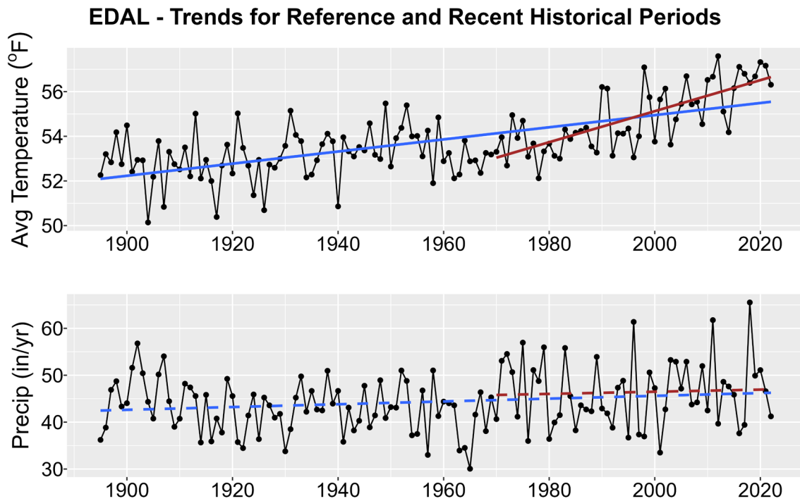
Figure 1. Historical trends in annual average temperature (upper plot) and annual total precipitation (lower plot) for EDAL from 1895-2022. Black points show yearly values while blue lines are linear regressions for the entire period record and red lines for 1970-2022 trends. Solid lines are significant trends (i.e., p < 0.05 ); dashed lines are not statistically significant.
