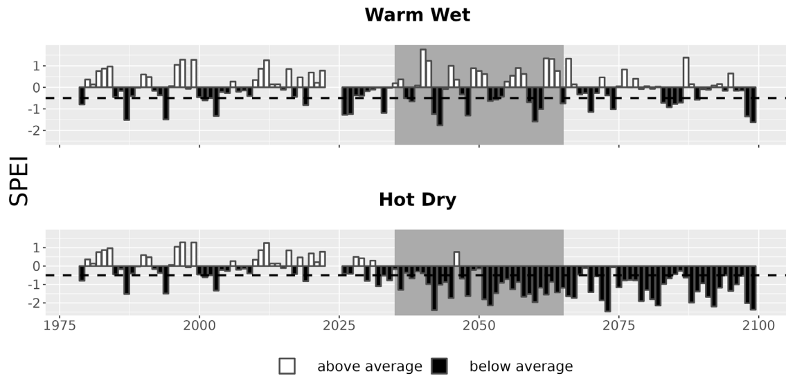
Figure 7. Drought metrics for EBLA. Drought index (SPEI; units = standard deviations from historical) timeseries for each climate future. Below-average SPEI (black bars) indicates dry conditions. The dotted line (SPEI = -0.5) indicates drought conditions.
