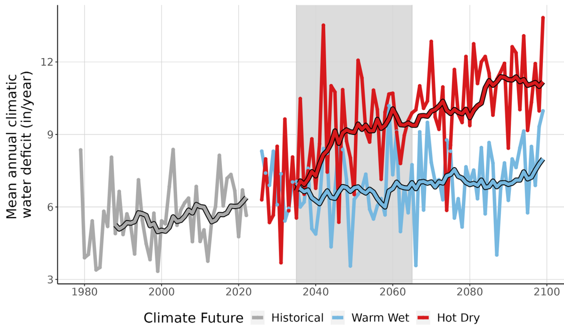
Figure 9. This line graph compares observed climatic water deficit at EBLA (inches/year) (1979-2022) with projected climatic water deficit for the two climate futures over the period 2023-2099. The historical observation data is shown in gray, the Warm Wet climate future in blue, and the Hot Dry climate future in red. The smooth line running through each projection is the 10-year running average for historical observations and future projections. Gray-shaded area represents the time period that was averaged (2035-2065) to summarize future projections for the year 2050.
