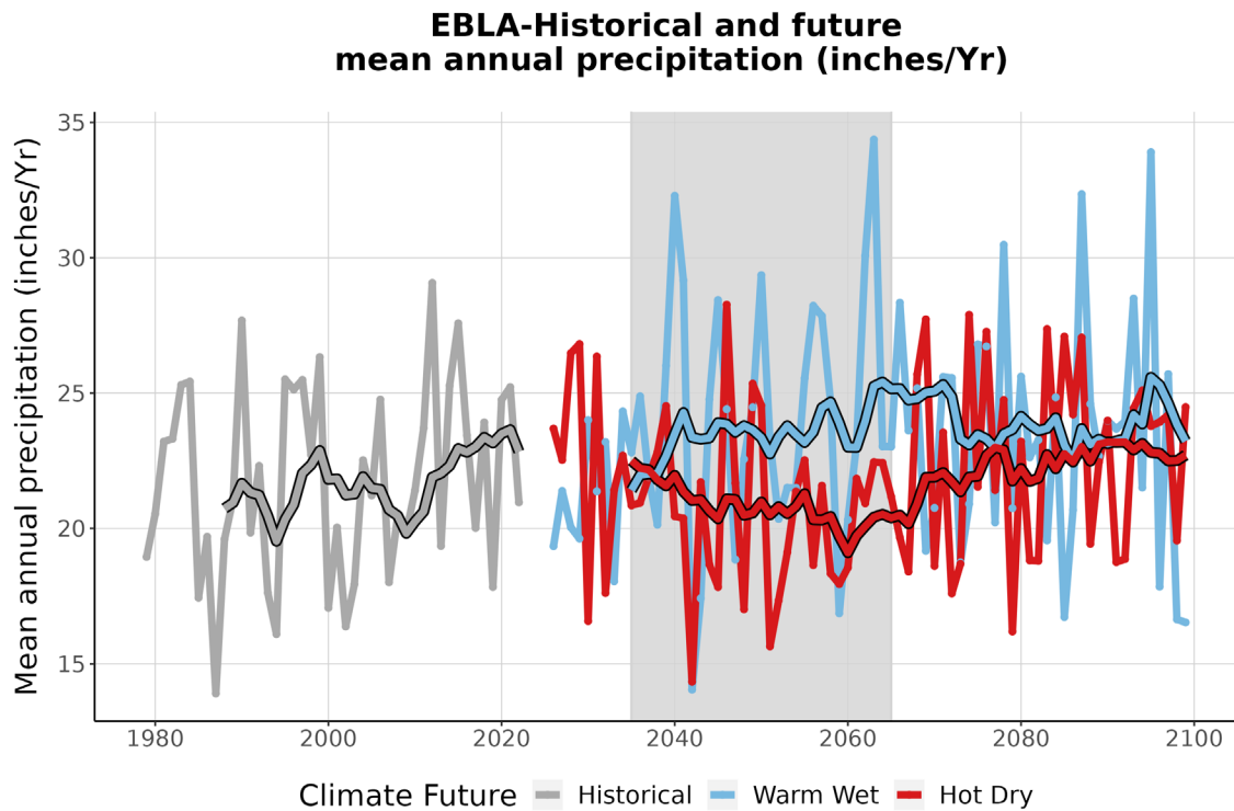
Figure 4. This graph compares observed average annual precipitation at EBLA (inches/year) (1979-2022) with projected average annual precipitation for the two climate futures over the period 2023-2099. The historically observed data is shown in gray, the Warm Wet climate future in blue, and the Hot Dry climate future in red. The smooth line running through each projection is the 10-year running average for historical observations and future projections. The gray-shaded area represents the time period that was averaged (2035-2065) to summarize future projections for the year 2050 (Appendix 1).
