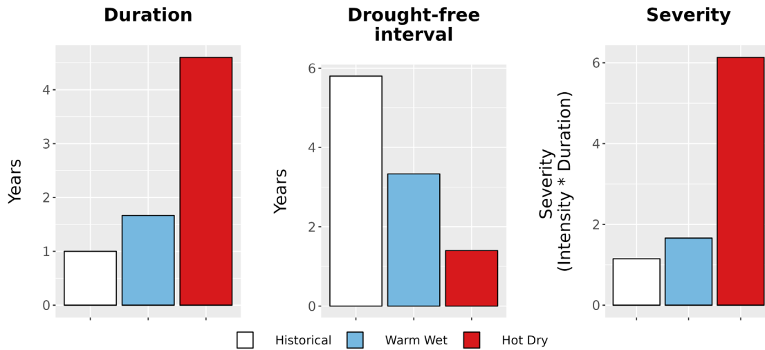
Figure 8. Drought metrics for EBLA. (Left) Average drought duration (years) historically (1979-2012) and under each climate future. (Middle) Average drought return interval (years), indicating the expected amount of time between periods of drought, historically and under each climate future. (Right) Average drought severity, a measure of drought intensity multiplied by duration, historically and under each climate future.
