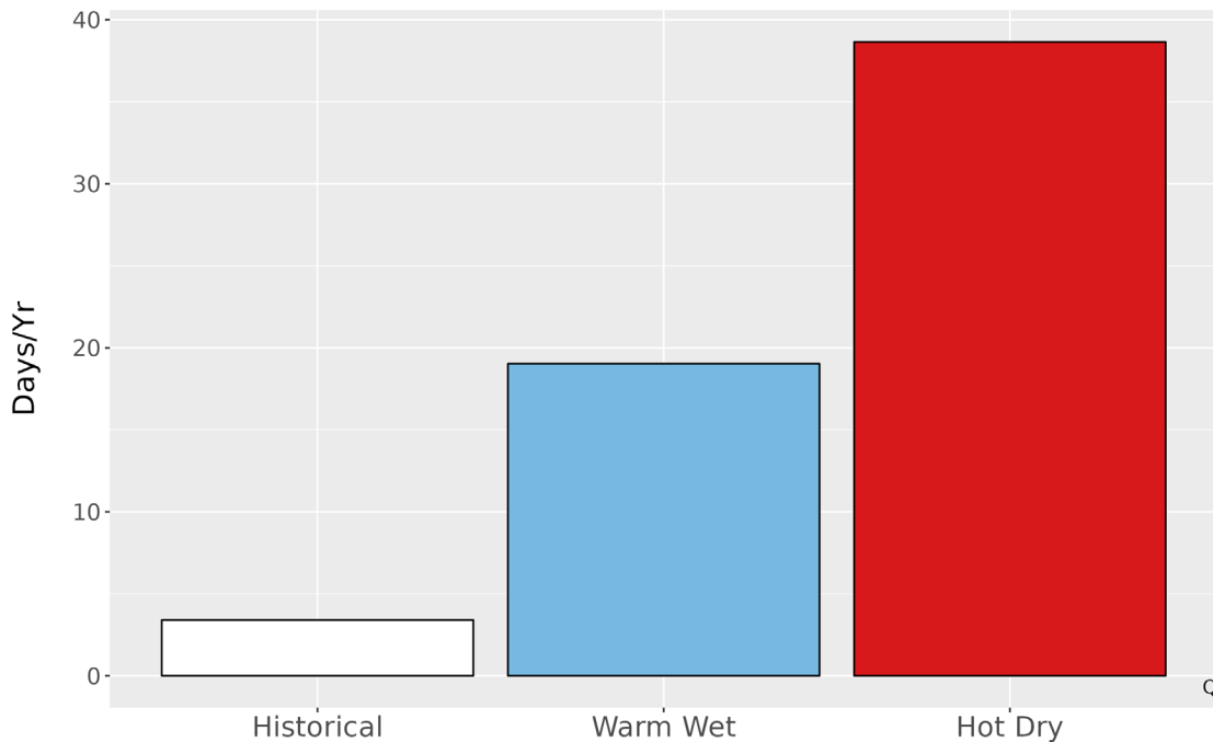
Figure 5. Metrics of extreme temperature at EBLA. The bar graph represents the average number of days annually with temperatures greater than the historical 99th percentile (78.7 °F) historically (1979-2012) and for the two climate futures (2050).
