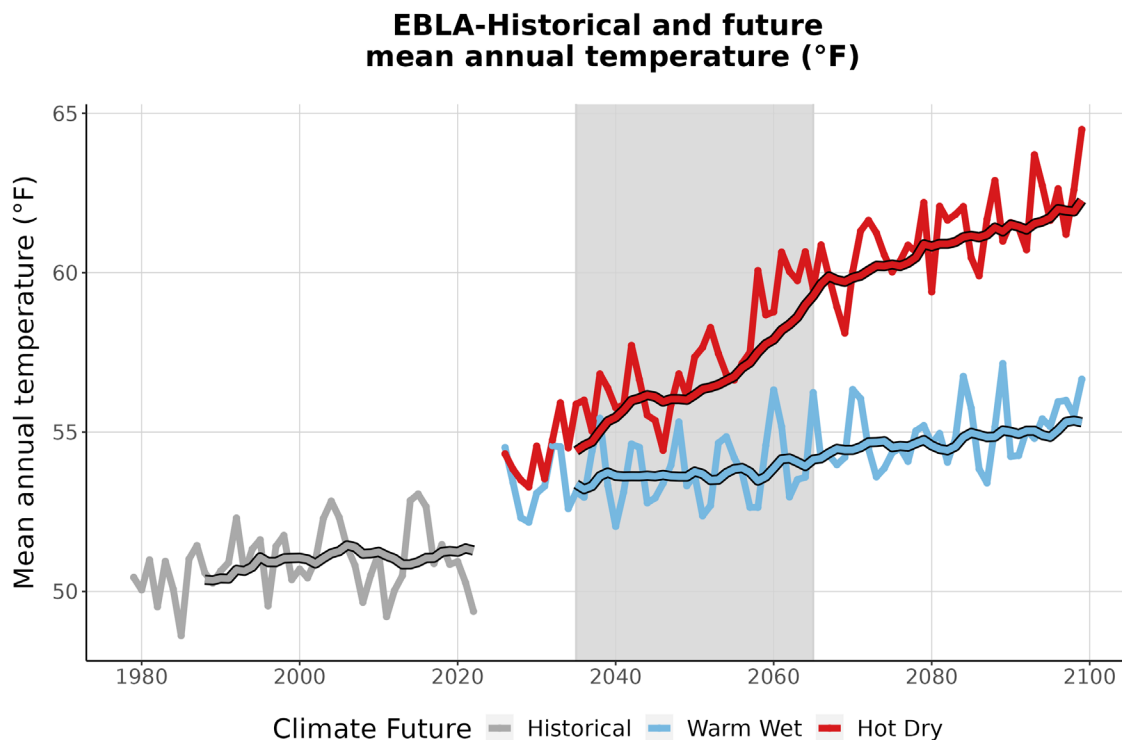
Figure 3. This graph compares observed average annual temperature at EBLA (°F) (1979-2022) with projected average annual temperature for the two climate futures over the period 2023-2099. The historically observed data
