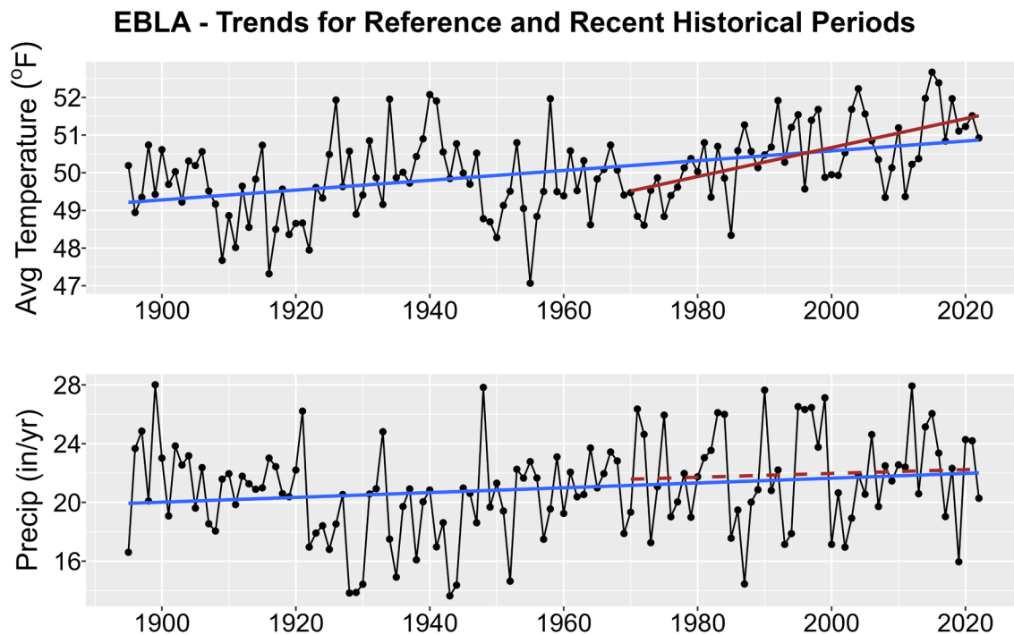
Figure 1. Historical trends in annual average temperature (upper plot) and annual total precipitation (lower plot) for EBLA from 1895-2022. Black points show yearly values while blue lines are linear regressions for the entire period record and red lines for 1970-2022 trends. Solid lines are significant trends (i.e., p < 0.05 ); dashed lines are not statistically significant.
