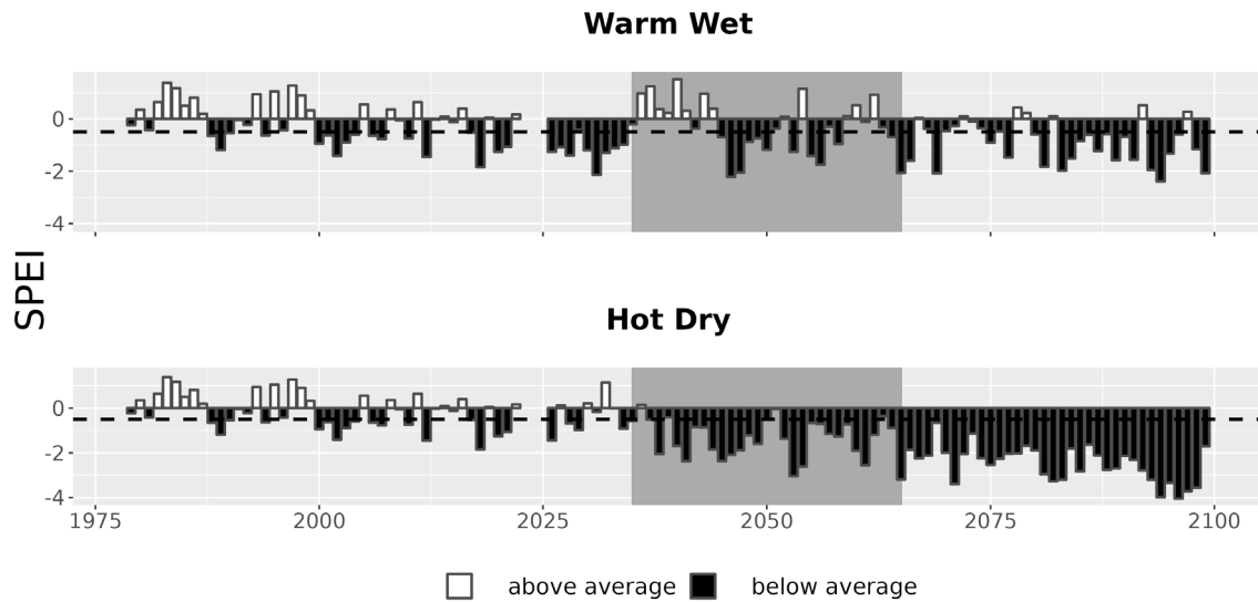
Figure 7. Drought metrics for DINO. Drought index (SPEI; units = standard deviations from historical) timeseries for each climate future. Below-average SPEI (black bars) indicates dry conditions. The dotted line (SPEI = -0.5) indicates drought conditions.
