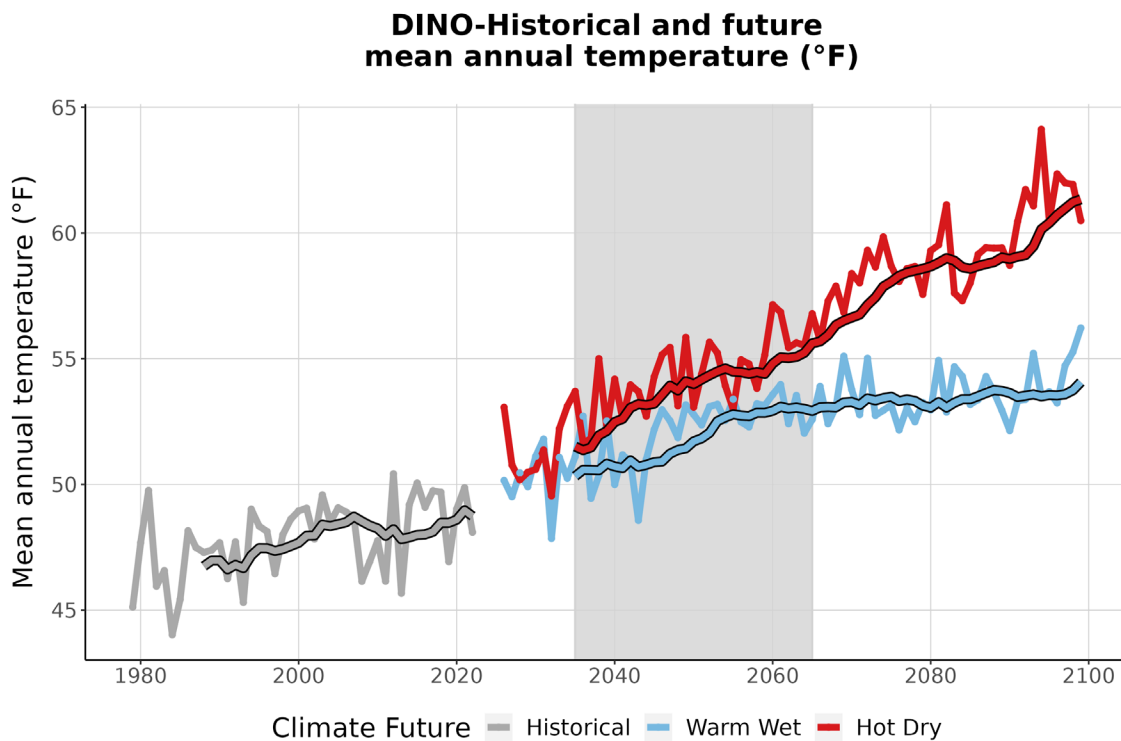
Figure 3. This graph compares observed average annual temperature at DINO (°F) (1979-2022) with projected average annual temperature for the two climate futures over the period 2023-2099. The historically observed data is shown in gray, the Warm Wet climate future in blue, and the Hot Dry climate future in red. The smooth line
