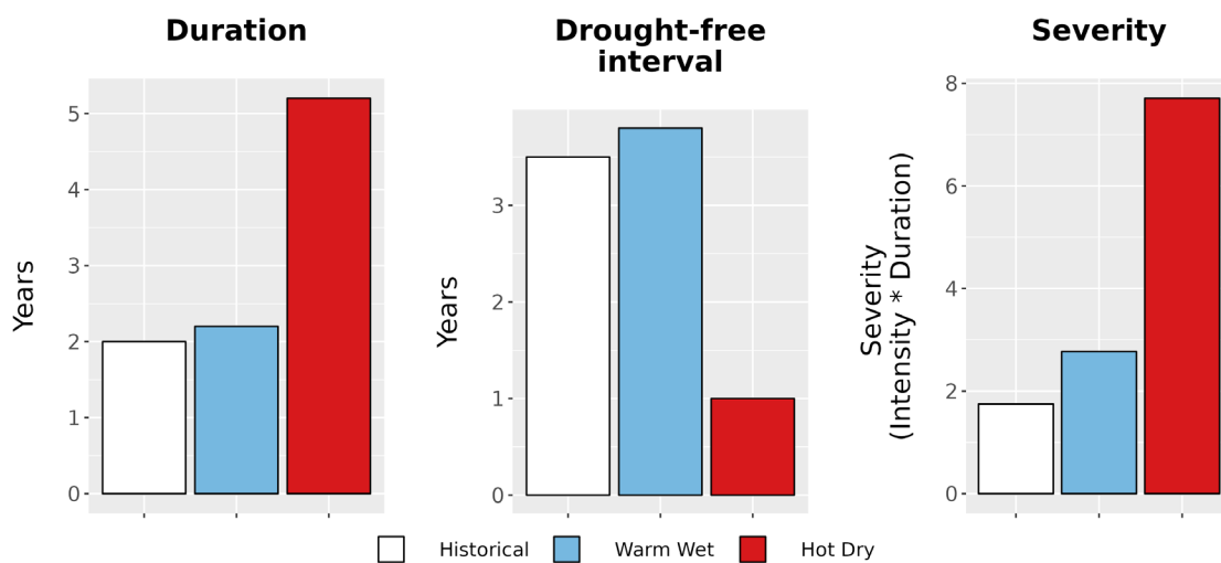
Figure 8. Drought metrics for DINO. (Left) Average drought duration (years) historically (1979-2012) and under each climate future. (Middle) Average drought return interval (years), indicating the expected amount of time between periods of drought, historically and under each climate future. (Right) Average drought severity, a measure of drought intensity multiplied by duration, historically and under each climate future.
