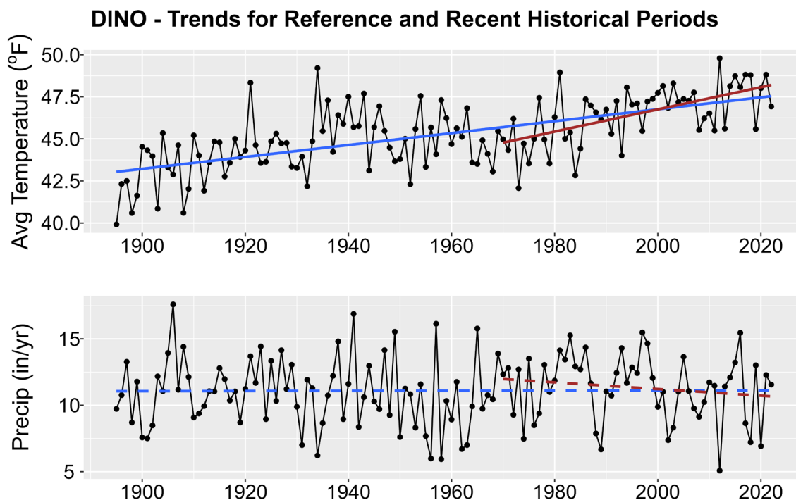
Figure 1. Historical trends in annual average temperature (upper plot) and annual total precipitation (lower plot) for DINO from 1895-2022. Black points show yearly values while blue lines are linear regressions for the entire period record and red lines for 1970-2022 trends. Solid lines are significant trends (i.e., p < 0.05 ); dashed lines are not statistically significant.
