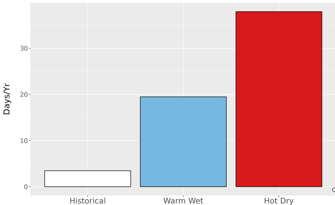
Figure 5. Metrics of extreme temperature at DINO. The bar graph represents the average number of days annually with temperatures greater than the historical 99th percentile (94.4 °F) historically (1979-2012) and for the two climate futures (2050).
