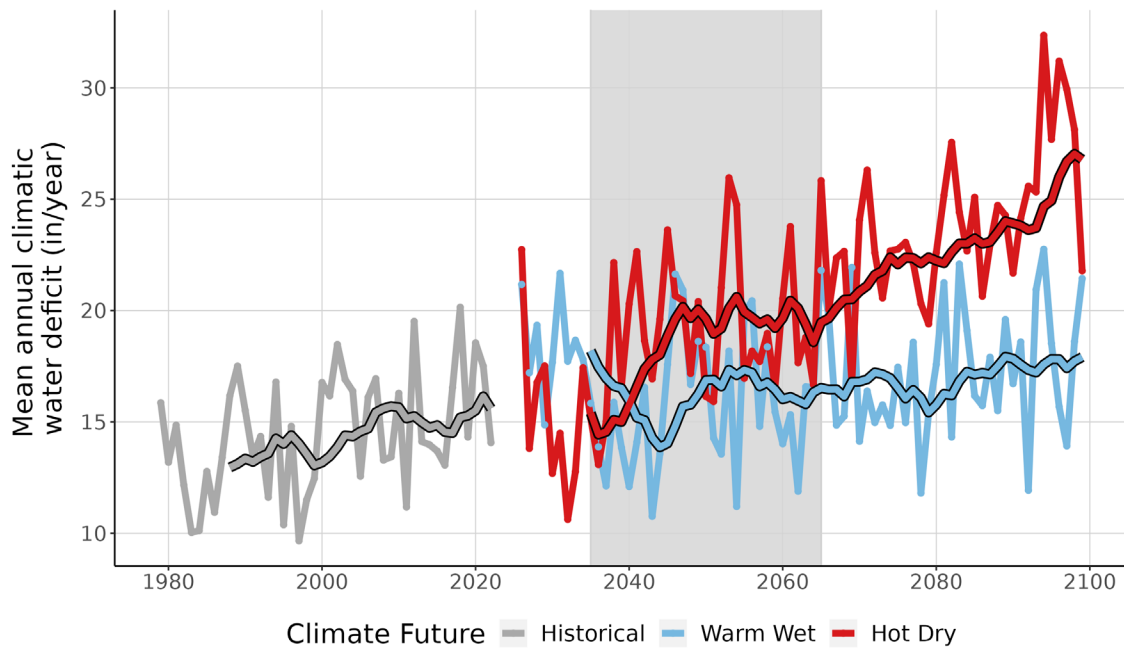
Figure 9. This line graph compares observed climatic water deficit at DINO (inches/year) (1979-2022) with projected climatic water deficit for the two climate futures over the period 2023-2099. The historical observation data is shown in gray, the Warm Wet climate future in blue, and the Hot Dry climate future in red. The smooth line running through each projection is the 10-year running average for historical observations and future projections. Gray-shaded area represents the time period that was averaged (2035-2065) to summarize future projections for the year 2050.
