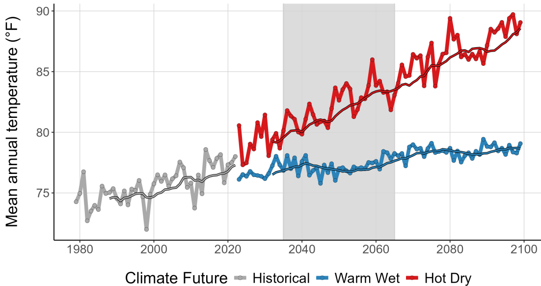
Figure 3. This graph compares observed average annual temperature at DEVA (°F) (1979-2022) with projected average annual temperature for the two climate futures over the period 2023-2099. The historically observed data is shown in gray, the Warm Wet climate future in blue, and the Hot Dry climate future in red. The smooth line running through each projection is the 10-year running average for historical observations and future projections. Gray-shaded area represents the time period that was averaged (2035-2065) to summarize future projections for the year 2050 (Appendix 1).
