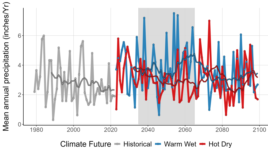
Figure 4. This graph compares observed average annual precipitation at DEVA (inches/year) (1979-2022) with projected average annual precipitation for the two climate futures over the period 2023-2099. The historically observed data is shown in gray, the Warm Wet climate future in blue, and the Hot Dry climate future in red. The smooth line running through each projection is the 10-year running average for historical observations and future projections. The gray-shaded area represents the time period that was averaged (2035-2065) to summarize future projections for the year 2050 (Appendix 1).
