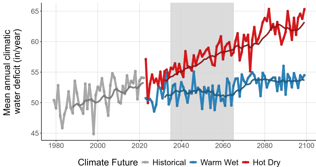
Figure 9. This line graph compares observed climatic water deficit at DEVA (inches/year) (1979-2022) with projected climatic water deficit for the two climate futures over the period 2023-2099. The historical observation data is shown in gray, the Warm Wet climate future in blue, and the Hot Dry climate future in red. The smooth line running through each projection is the 10-year running average for historical observations and future projections. Gray-shaded area represents the time period that was averaged (2035-2065) to summarize future projections for the year 2050.
