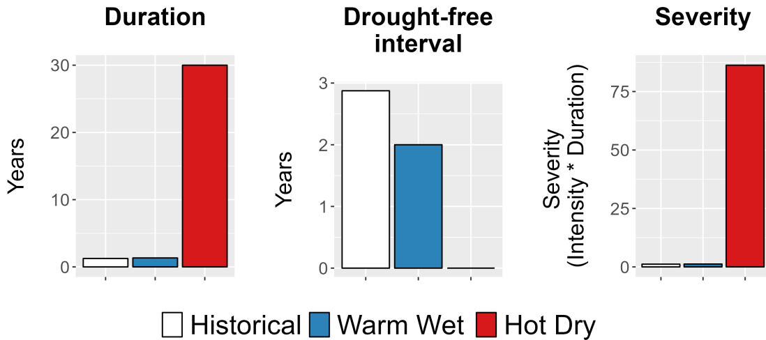
Figure 8. Drought metrics for DEVA. (Left) Average drought duration (years) historically (1979-2012) and under each climate future. (Middle) Average drought return interval (years), indicating the expected amount of time between periods of drought, historically and under each climate future. (Right) Average drought severity, a measure of drought intensity multiplied by duration, historically and under each climate future.
