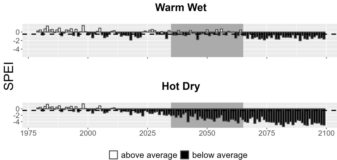
Figure 7. Drought metrics for DEVA. Drought index (SPEI; units = standard deviations from historical) timeseries for each climate future. Below-average SPEI (black bars) indicates dry conditions. The dotted line (SPEI = -0.5) indicates drought conditions.
