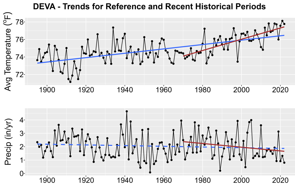
Figure 1. Historical trends in annual average temperature (upper plot) and annual total precipitation (lower plot) for DEVA from 1895-2022. Black points show yearly values while blue lines are linear regressions for the entire period record and red lines for 1970-2022 trends. Solid lines are significant trends (i.e., p < 0.05 ); dashed lines are not statistically significant.
