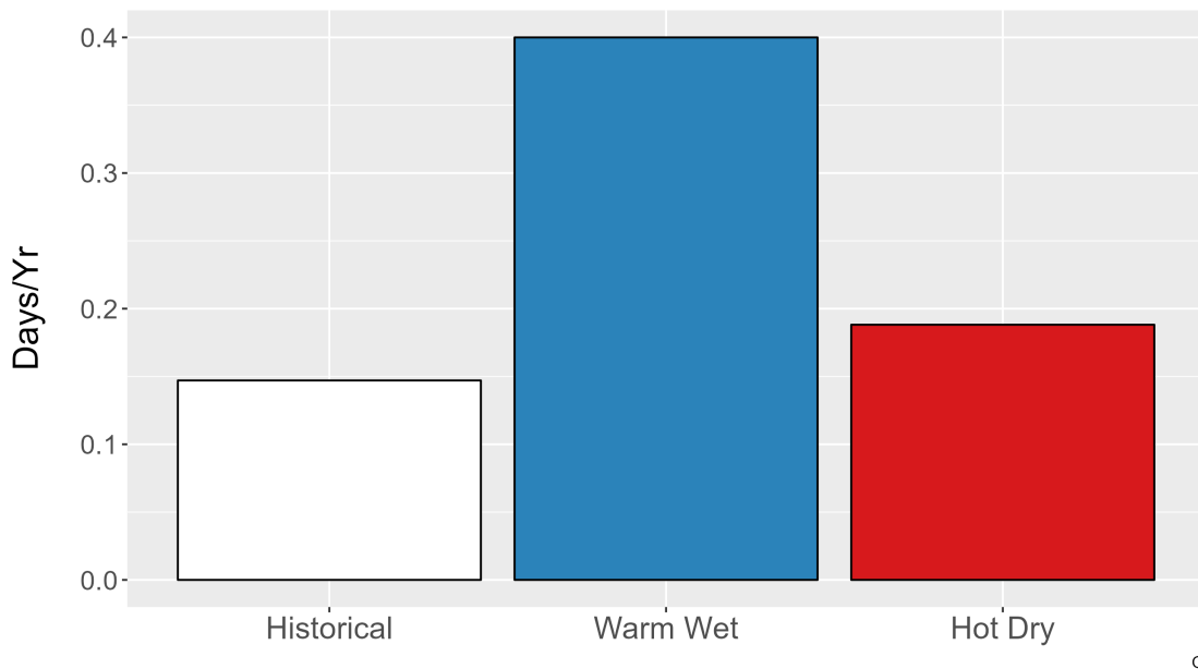
Figure 6. Average number of days annually with precipitation exceeding the 99th percentile (0.8 in.) of precipitation from the historical period 1979-2012 and for each climate future.
