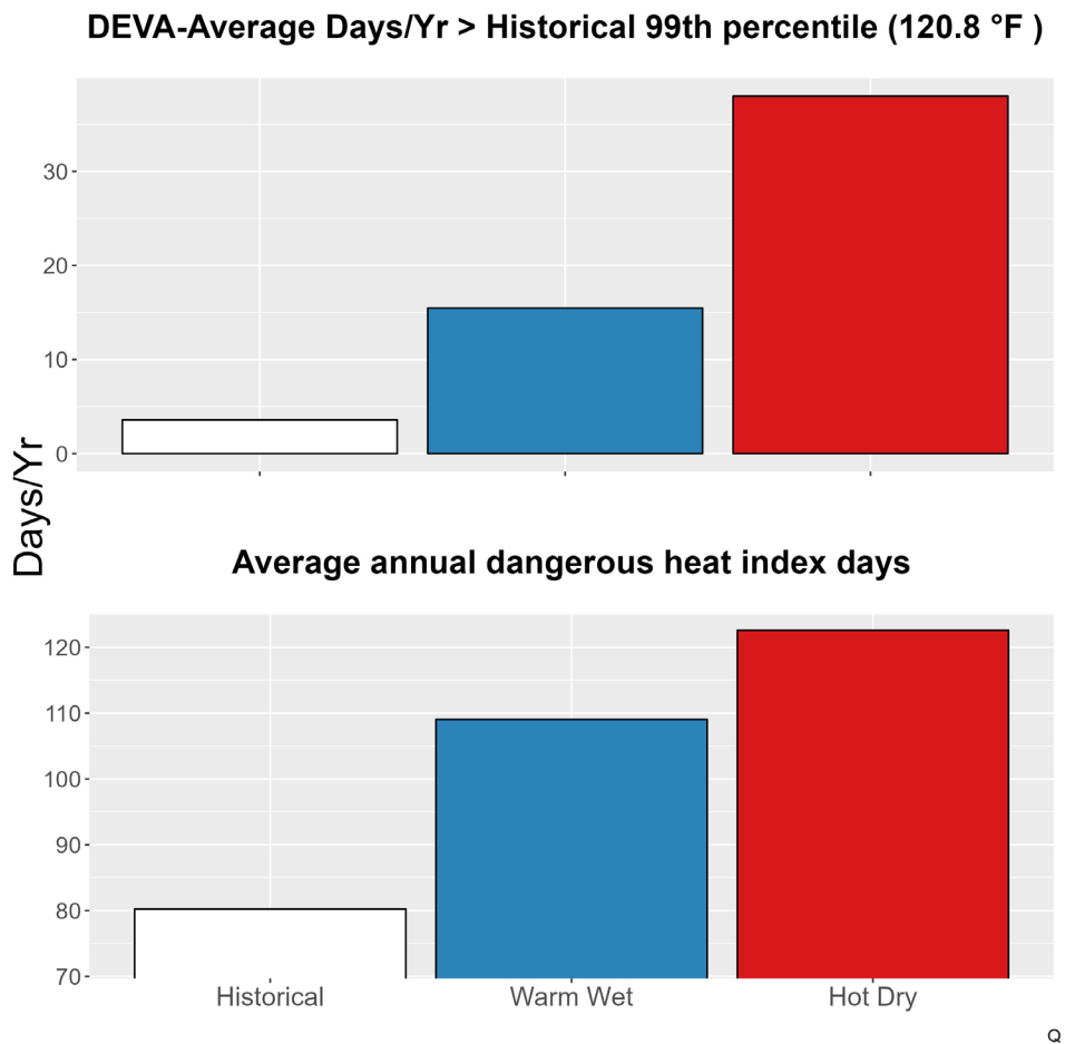
Figure 5. The upper bar graph represents the average number of days annually with temperatures greater than the historical 99th percentile (120.8 °F) historically (1979-2012) and for the two climate futures (2050). The bottom bar graph represents the average annual number of dangerous heat index days historically and for the two climate futures. Dangerous heat index days are days that exceed 105 °F.
