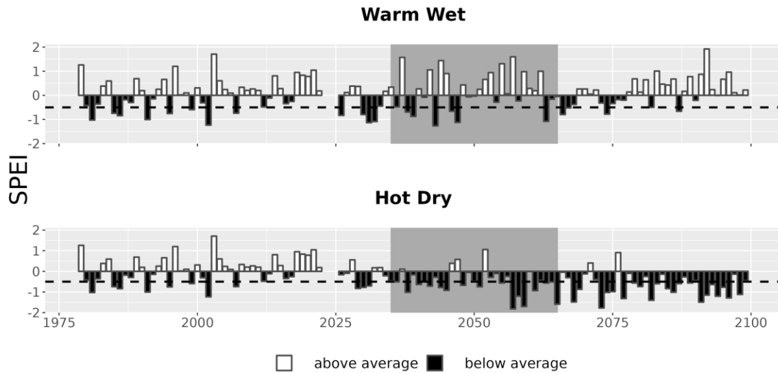
Figure 7. Drought metrics for DDEM. Drought index (SPEI; units = standard deviations from historical) timeseries for each climate future. Below-average SPEI (black bars) indicates dry conditions. The dotted line (SPEI = -0.5) indicates drought conditions.
