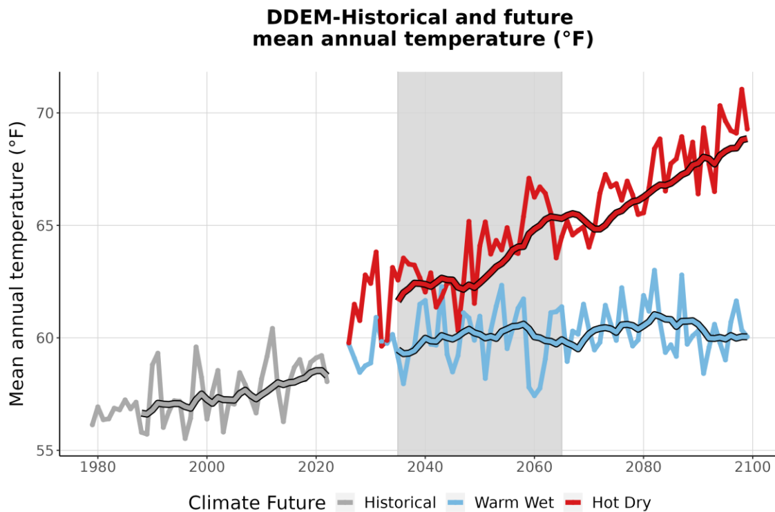
Figure 3. This graph compares observed average annual temperature at DDEM (°F) (1979-2022) with projected average annual temperature for the two climate futures over the period 2023-2099. The historically observed data is shown in gray, the Warm Wet climate future in blue, and the Hot Dry climate future in red. The smooth line
