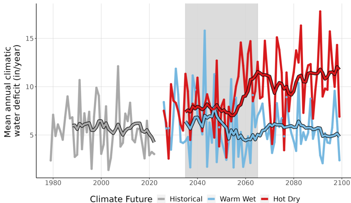
Figure 9. This line graph compares observed climatic water deficit at DDEM (inches/year) (1979-2022) with projected climatic water deficit for the two climate futures over the period 2023-2099. The historical observation data is shown in gray, the Warm Wet climate future in blue, and the Hot Dry climate future in red. The smooth line running through each projection is the 10-year running average for historical observations and future projections. Gray-shaded area represents the time period that was averaged (2035-2065) to summarize future projections for the year 2050.
