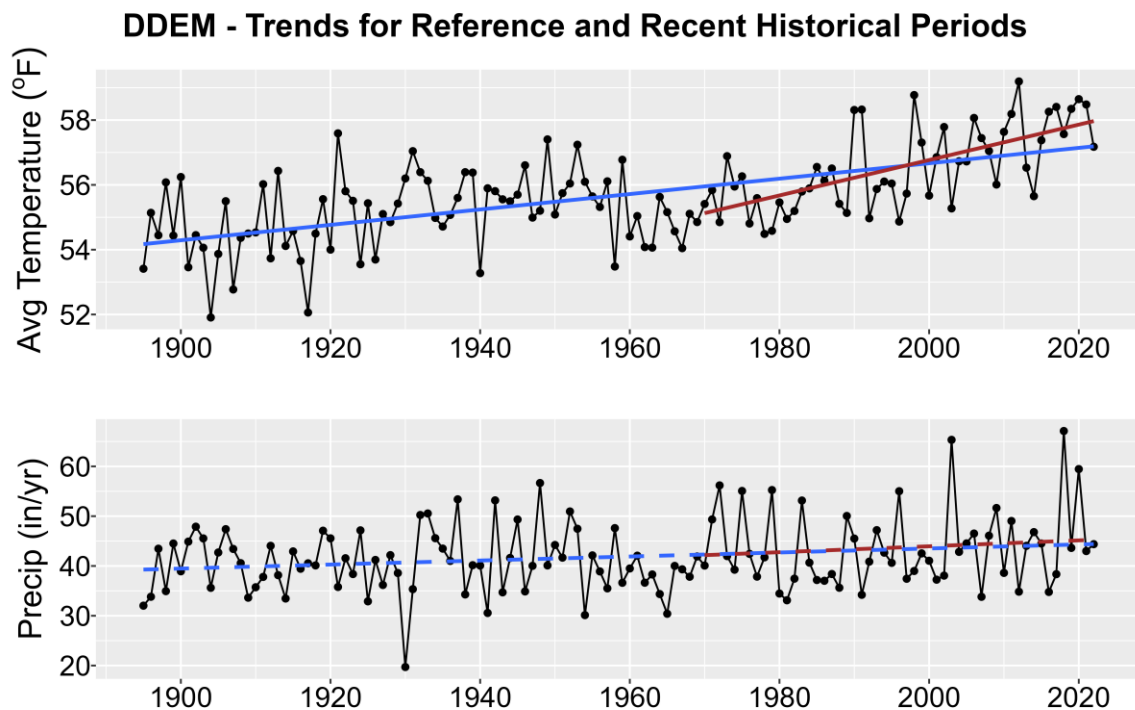
Figure 1. Historical trends in annual average temperature (upper plot) and annual total precipitation (lower plot) for DDEM from 1895-2022. Black points show yearly values while blue lines are linear regressions for the entire period record and red lines for 1970-2022 trends. Solid lines are significant trends (i.e., p < 0.05 ); dashed lines are not statistically significant.
