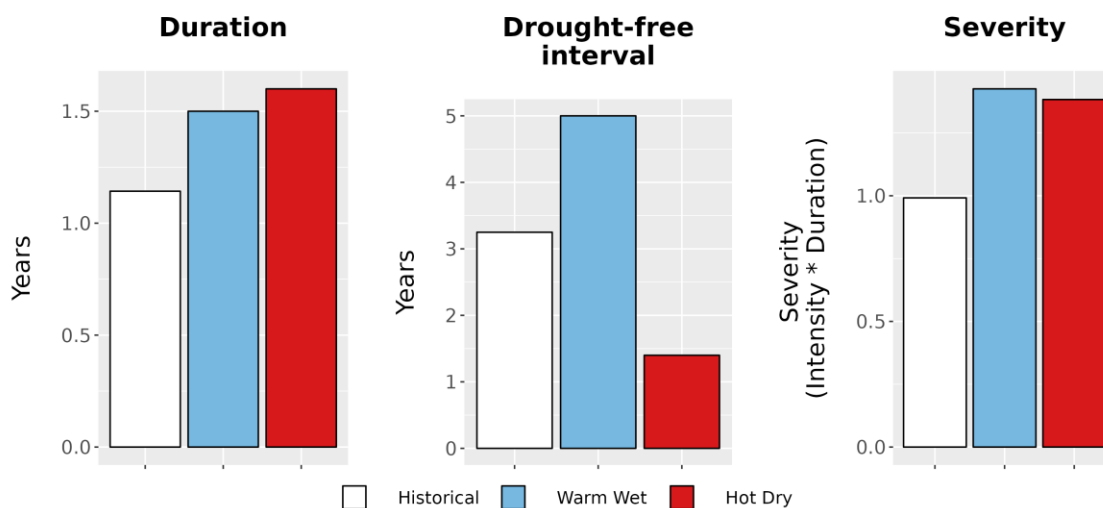
Figure 8. Drought metrics for DDEM. (Left) Average drought duration (years) historically (1979-2012) and under each climate future. (Middle) Average drought return interval (years), indicating the expected amount of time between periods of drought, historically and under each climate future. (Right) Average drought severity, a measure of drought intensity multiplied by duration, historically and under each climate future.
