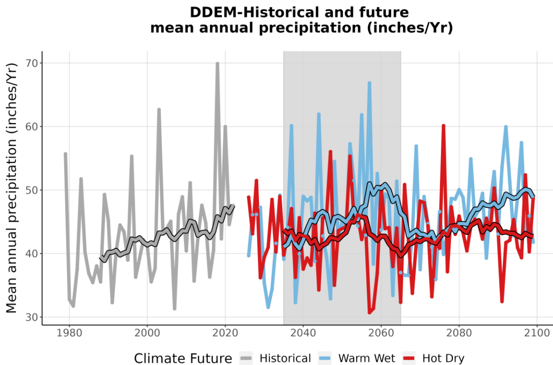
Figure 4. This graph compares observed average annual precipitation at DDEM (inches/year) (1979-2022) with projected average annual precipitation for the two climate futures over the period 2023-2099. The historically observed data is shown in gray, the Warm Wet climate future in blue, and the Hot Dry climate future in red. The smooth line running through each projection is the 10-year running average for historical observations and future projections. The gray-shaded area represents the time period that was averaged (2035-2065) to summarize future projections for the year 2050 (Appendix 1).
