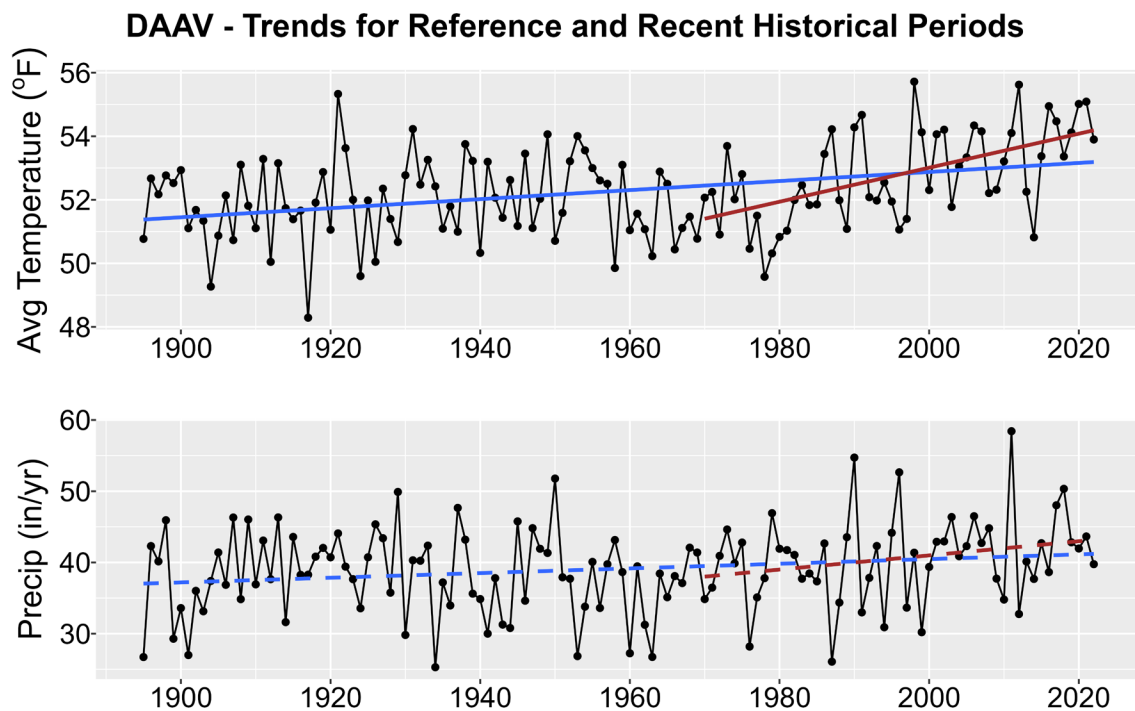
Figure 1. Historical trends in annual average temperature (upper plot) and annual total precipitation (lower plot) for DAAV from 1895-2022. Black points show yearly values while blue lines are linear regressions for the entire period record and red lines for 1970-2022 trends. Solid lines are significant trends (i.e., p < 0.05 ); dashed lines are not statistically significant.
