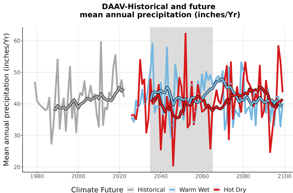
Figure 4. This graph compares observed average annual precipitation at DAAV (inches/year) (1979-2022) with projected average annual precipitation for the two climate futures over the period 2023-2099. The historically observed data is shown in gray, the Warm Wet climate future in blue, and the Hot Dry climate future in red. The smooth line running through each projection is the 10-year running average for historical observations and future projections. The gray-shaded area represents the time period that was averaged (2035-2065) to summarize future projections for the year 2050 (Appendix 1).
