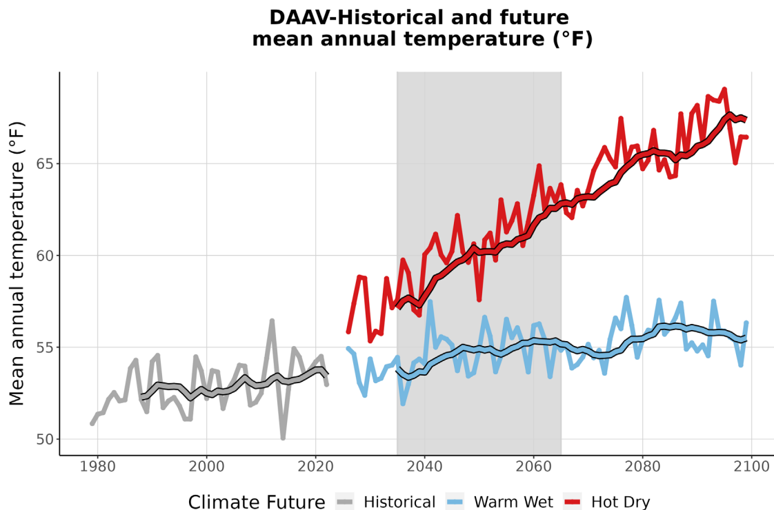
Figure 3. This graph compares observed average annual temperature at DAAV (°F) (1979-2022) with projected average annual temperature for the two climate futures over the period 2023-2099. The historically observed data
