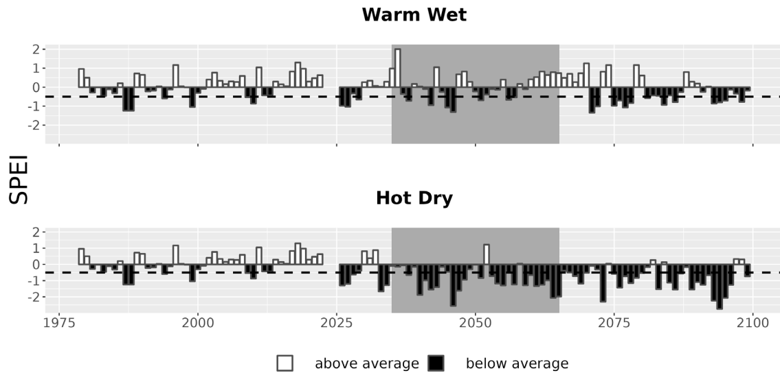
Figure 7. Drought metrics for DAAV. Drought index (SPEI; units = standard deviations from historical) timeseries for each climate future. Below-average SPEI (black bars) indicates dry conditions. The dotted line (SPEI = -0.5) indicates drought conditions.
