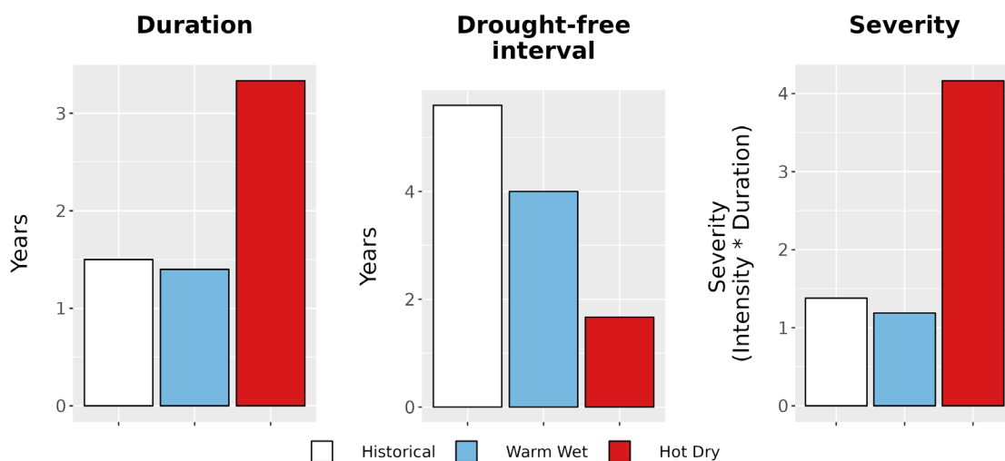
Figure 8. Drought metrics for DAAV. (Left) Average drought duration (years) historically (1979-2012) and under each climate future. (Middle) Average drought return interval (years), indicating the expected amount of time between periods of drought, historically and under each climate future. (Right) Average drought severity, a measure of drought intensity multiplied by duration, historically and under each climate future.
