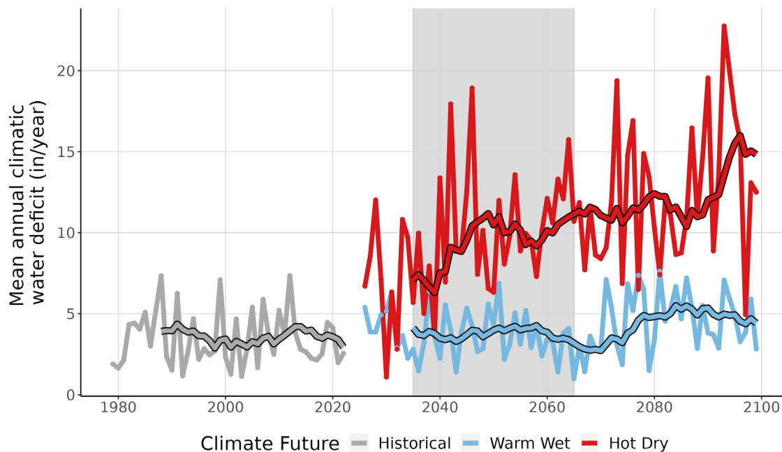
Figure 9. This line graph compares observed climatic water deficit at DAAV (inches/year) (1979-2022) with projected climatic water deficit for the two climate futures over the period 2023-2099. The historical observation data is shown in gray, the Warm Wet climate future in blue, and the Hot Dry climate future in red. The smooth line running through each projection is the 10-year running average for historical observations and future projections. Gray-shaded area represents the time period that was averaged (2035-2065) to summarize future projections for the year 2050.
