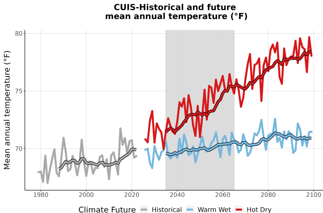
Figure 3. This graph compares observed average annual temperature at CUIS (°F) (1979-2022) with projected average annual temperature for the two climate futures over the period 2023-2099. The historically observed data
