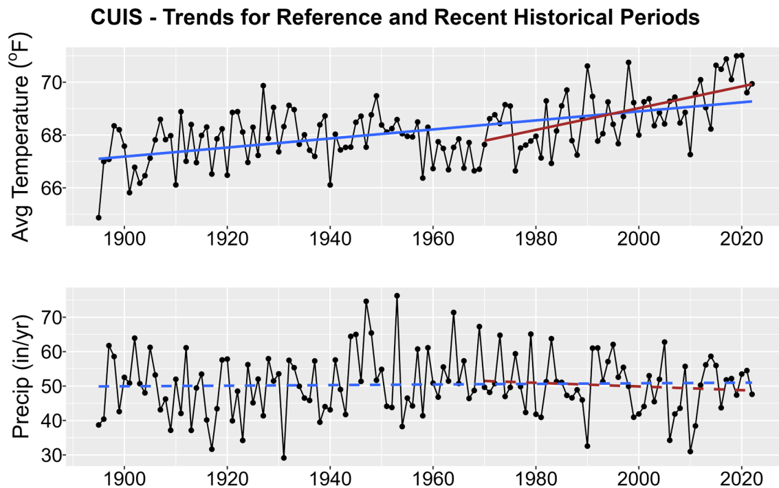
Figure 1. Historical trends in annual average temperature (upper plot) and annual total precipitation (lower plot) for CUIS from 1895-2022. Black points show yearly values while blue lines are linear regressions for the entire period record and red lines for 1970-2022 trends. Solid lines are significant trends (i.e., p < 0.05 ); dashed lines are not statistically significant.
