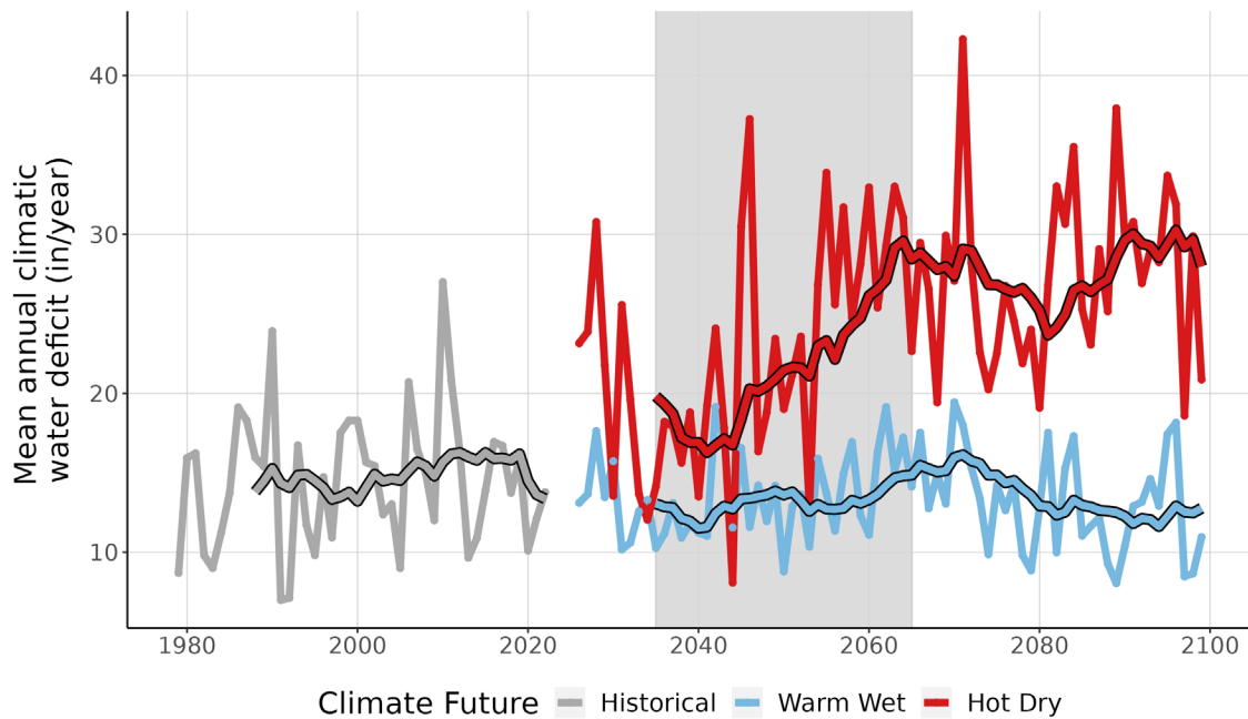
Figure 9. This line graph compares observed climatic water deficit at CUIS (inches/year) (1979-2022) with projected climatic water deficit for the two climate futures over the period 2023-2099. The historical observation data is shown in gray, the Warm Wet climate future in blue, and the Hot Dry climate future in red. The smooth line running through each projection is the 10-year running average for historical observations and future projections. Gray-shaded area represents the time period that was averaged (2035-2065) to summarize future projections for the year 2050.
