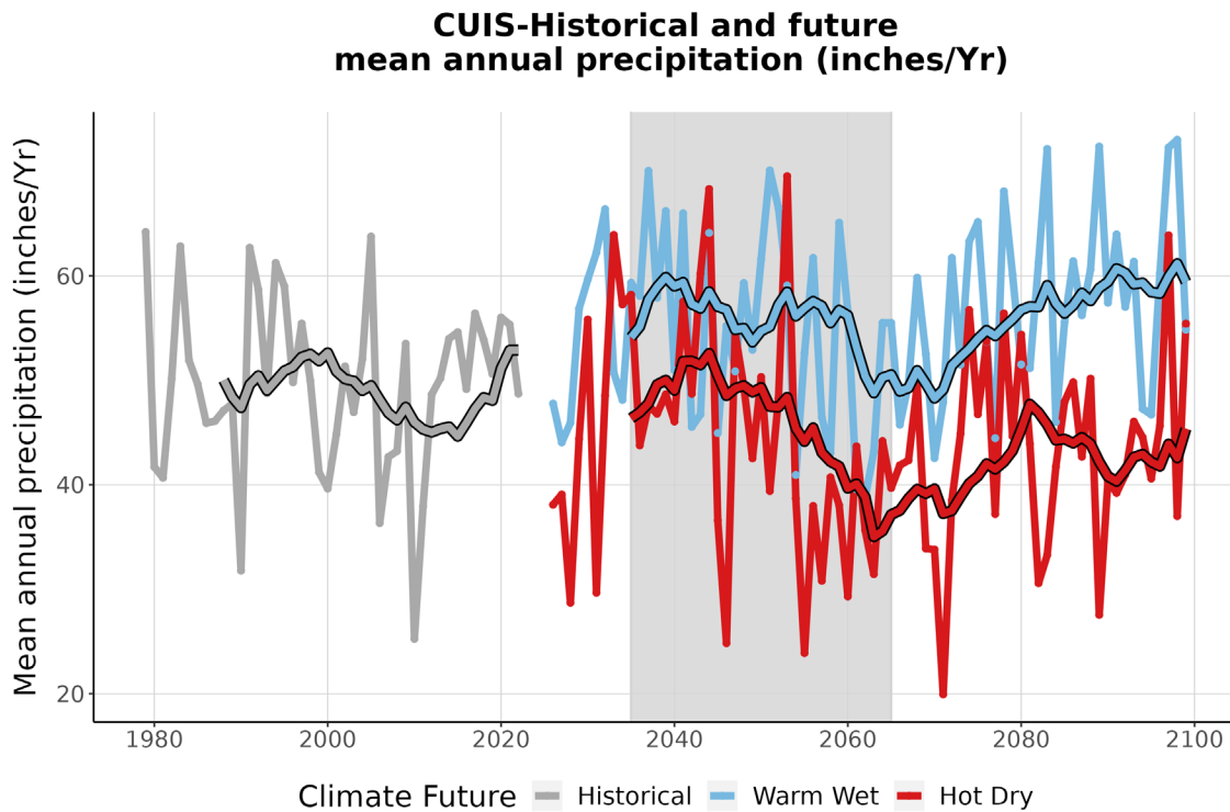
Figure 4. This graph compares observed average annual precipitation at CUIS (inches/year) (1979-2022) with projected average annual precipitation for the two climate futures over the period 2023-2099. The historically observed data is shown in gray, the Warm Wet climate future in blue, and the Hot Dry climate future in red. The smooth line running through each projection is the 10-year running average for historical observations and future projections. The gray-shaded area represents the time period that was averaged (2035-2065) to summarize future projections for the year 2050 (Appendix 1).
