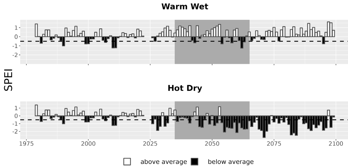
Figure 7. Drought metrics for CUIS. Drought index (SPEI; units = standard deviations from historical) timeseries for each climate future. Below-average SPEI (black bars) indicates dry conditions. The dotted line (SPEI = -0.5) indicates drought conditions.
