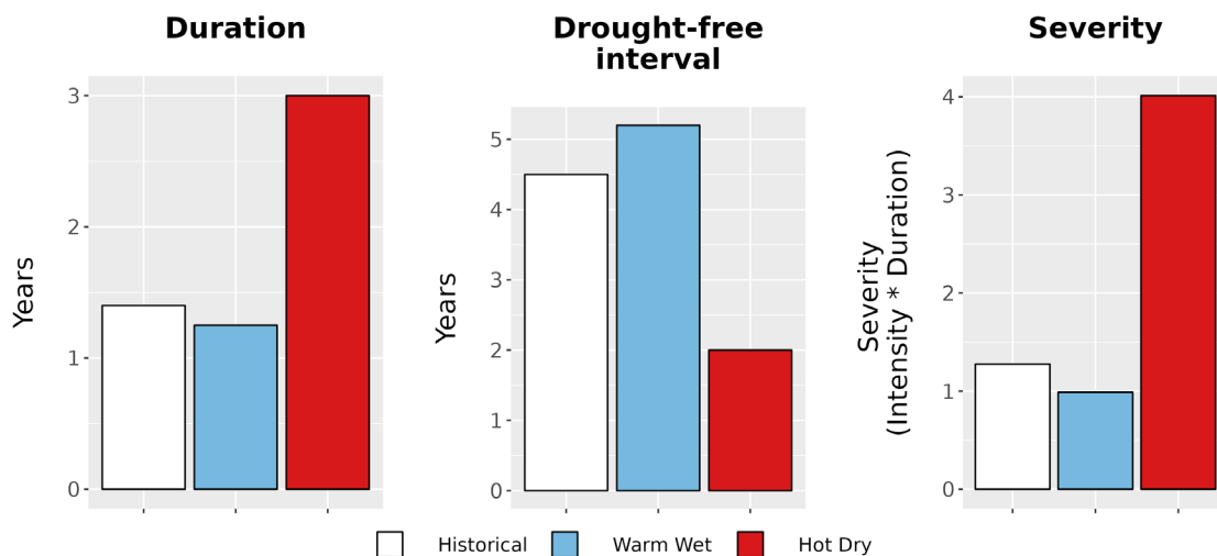
Figure 8. Drought metrics for CUIS. (Left) Average drought duration (years) historically (1979-2012) and under each climate future. (Middle) Average drought return interval (years), indicating the expected amount of time between periods of drought, historically and under each climate future. (Right) Average drought severity, a measure of drought intensity multiplied by duration, historically and under each climate future.
