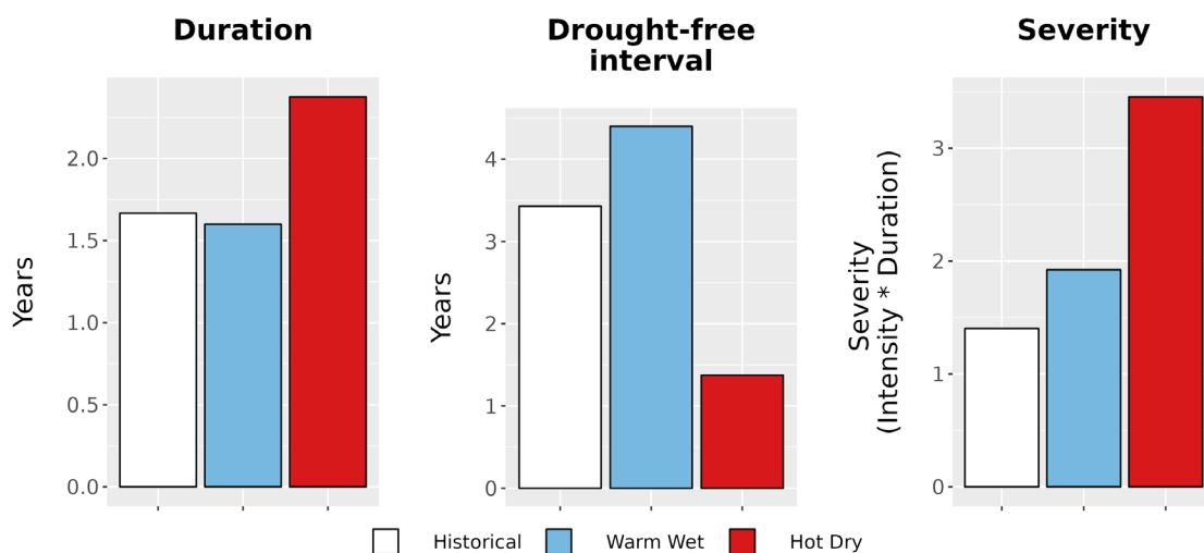
Figure 8. Drought metrics for CUGA. (Left) Average drought duration (years) historically (1979-2012) and under each climate future. (Middle) Average drought return interval (years), indicating the expected amount of time between periods of drought, historically and under each climate future. (Right) Average drought severity, a measure of drought intensity multiplied by duration, historically and under each climate future.
