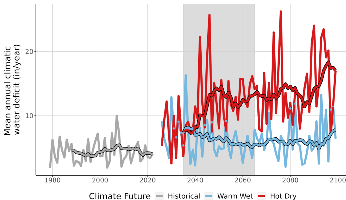
Figure 9. This line graph compares observed climatic water deficit at CUGA (inches/year) (1979-2022) with projected climatic water deficit for the two climate futures over the period 2023-2099. The historical observation data is shown in gray, the Warm Wet climate future in blue, and the Hot Dry climate future in red. The smooth line running through each projection is the 10-year running average for historical observations and future projections. Gray-shaded area represents the time period that was averaged (2035-2065) to summarize future projections for the year 2050.
