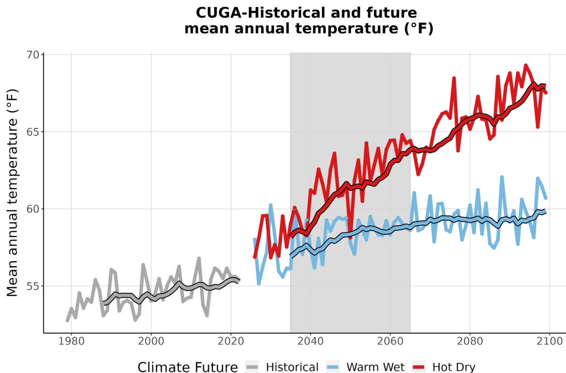
Figure 3. This graph compares observed average annual temperature at CUGA (°F) (1979-2022) with projected average annual temperature for the two climate futures over the period 2023-2099. The historically observed data
