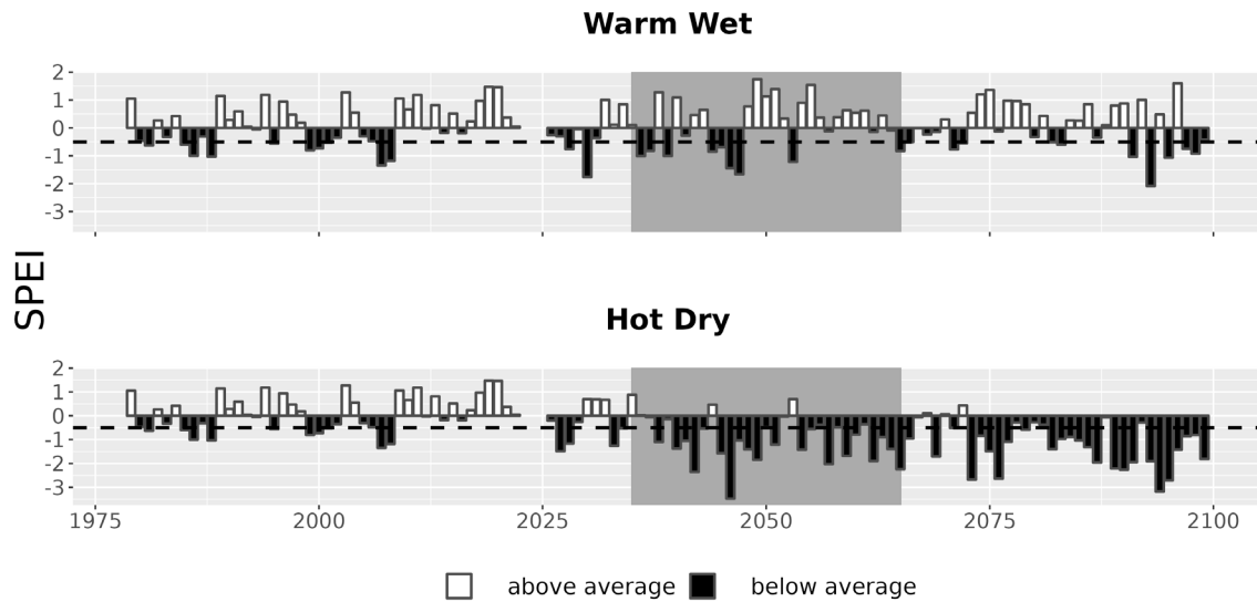
Figure 7. Drought metrics for CUGA. Drought index (SPEI; units = standard deviations from historical) timeseries for each climate future. Below-average SPEI (black bars) indicates dry conditions. The dotted line (SPEI = -0.5) indicates drought conditions.
