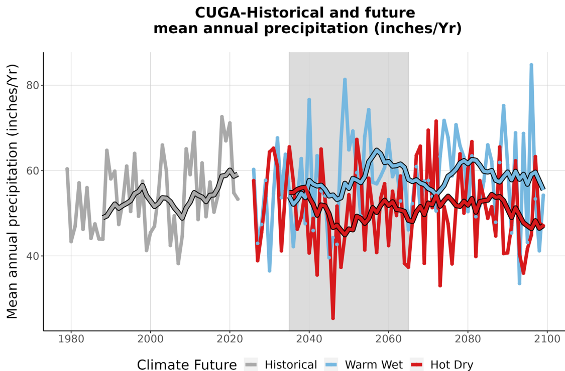
Figure 4. This graph compares observed average annual precipitation at CUGA (inches/year) (1979-2022) with projected average annual precipitation for the two climate futures over the period 2023-2099. The historically observed data is shown in gray, the Warm Wet climate future in blue, and the Hot Dry climate future in red. The smooth line running through each projection is the 10-year running average for historical observations and future projections. The gray-shaded area represents the time period that was averaged (2035-2065) to summarize future projections for the year 2050 (Appendix 1).
