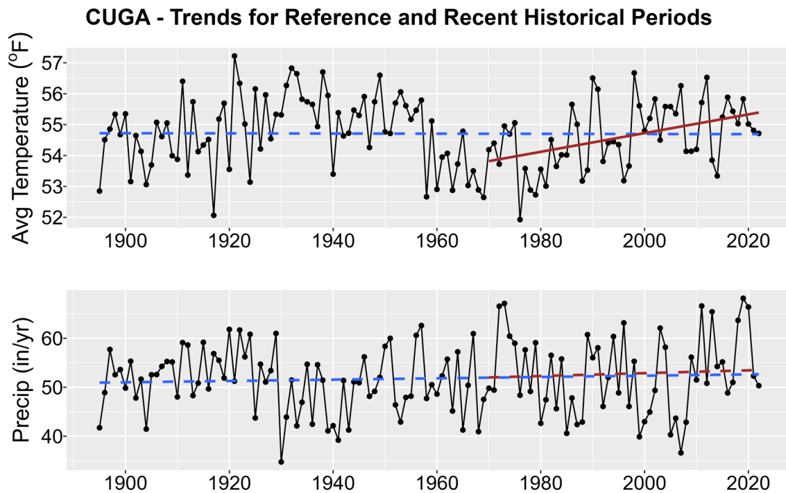
Figure 1. Historical trends in annual average temperature (upper plot) and annual total precipitation (lower plot) for CUGA from 1895-2022. Black points show yearly values while blue lines are linear regressions for the entire period record and red lines for 1970-2022 trends. Solid lines are significant trends (i.e., p < 0.05 ); dashed lines are not statistically significant.
