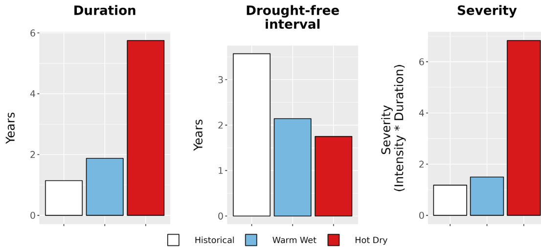
Figure 8. Drought metrics for CRMO. (Left) Average drought duration (years) historically (1979-2012) and under each climate future. (Middle) Average drought return interval (years), indicating the expected amount of time between periods of drought, historically and under each climate future. (Right) Average drought severity, a measure of drought intensity multiplied by duration, historically and under each climate future.
