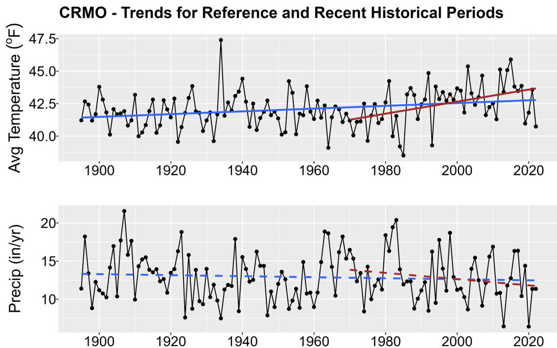
Figure 1. Historical trends in annual average temperature (upper plot) and annual total precipitation (lower plot) for CRMO from 1895-2022. Black points show yearly values while blue lines are linear regressions for the entire period record and red lines for 1970-2022 trends. Solid lines are significant trends (i.e., p < 0.05 ); dashed lines are not statistically significant.
