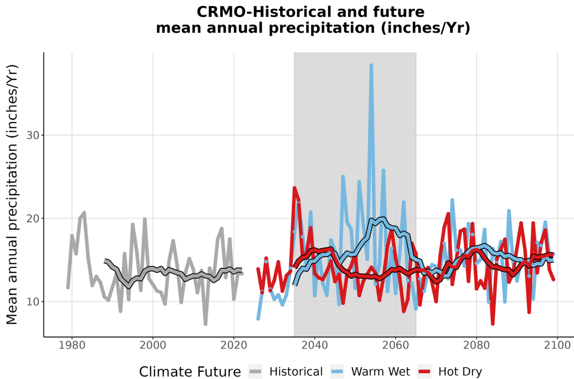
Figure 4. This graph compares observed average annual precipitation at CRMO (inches/year) (1979-2022) with projected average annual precipitation for the two climate futures over the period 2023-2099. The historically observed data is shown in gray, the Warm Wet climate future in blue, and the Hot Dry climate future in red. The smooth line running through each projection is the 10-year running average for historical observations and future projections. The gray-shaded area represents the time period that was averaged (2035-2065) to summarize future projections for the year 2050 (Appendix 1).
