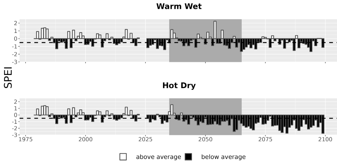
Figure 7. Drought metrics for CRMO. Drought index (SPEI; units = standard deviations from historical) timeseries for each climate future. Below-average SPEI (black bars) indicates dry conditions. The dotted line (SPEI = -0.5) indicates drought conditions.
