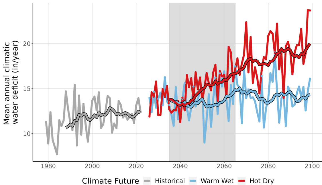
Figure 9. This line graph compares observed climatic water deficit at CRMO (inches/year) (1979-2022) with projected climatic water deficit for the two climate futures over the period 2023-2099. The historical observation data is shown in gray, the Warm Wet climate future in blue, and the Hot Dry climate future in red. The smooth line running through each projection is the 10-year running average for historical observations and future projections. Gray-shaded area represents the time period that was averaged (2035-2065) to summarize future projections for the year 2050.
