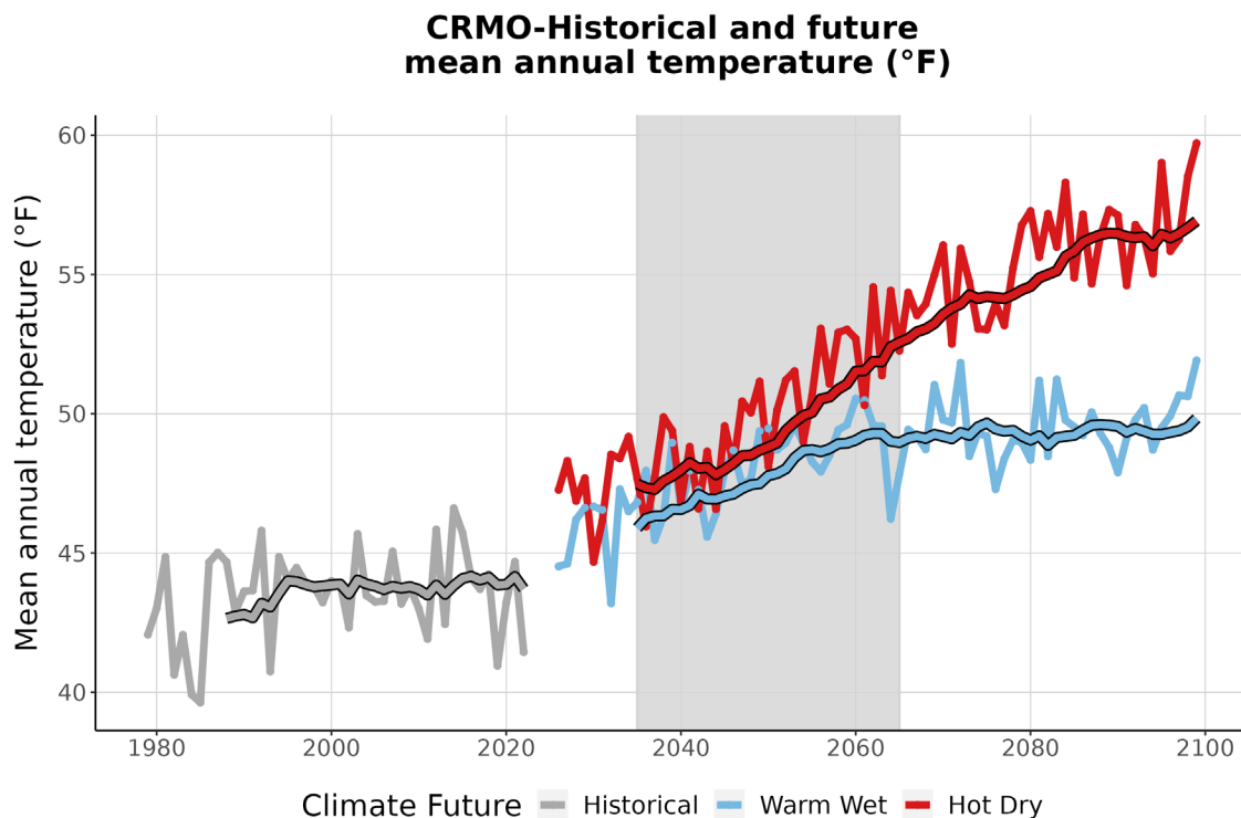
Figure 3. This graph compares observed average annual temperature at CRMO (°F) (1979-2022) with projected average annual temperature for the two climate futures over the period 2023-2099. The historically observed data
