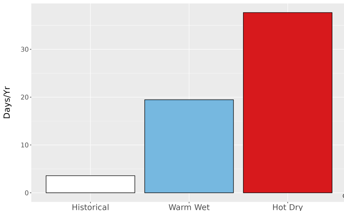
Figure 5. Metrics of extreme temperature at CRMO. The bar graph represents the average number of days annually with temperatures greater than the historical 99th percentile (93.5 °F) historically (1979-2012) and for the two climate futures (2050).
