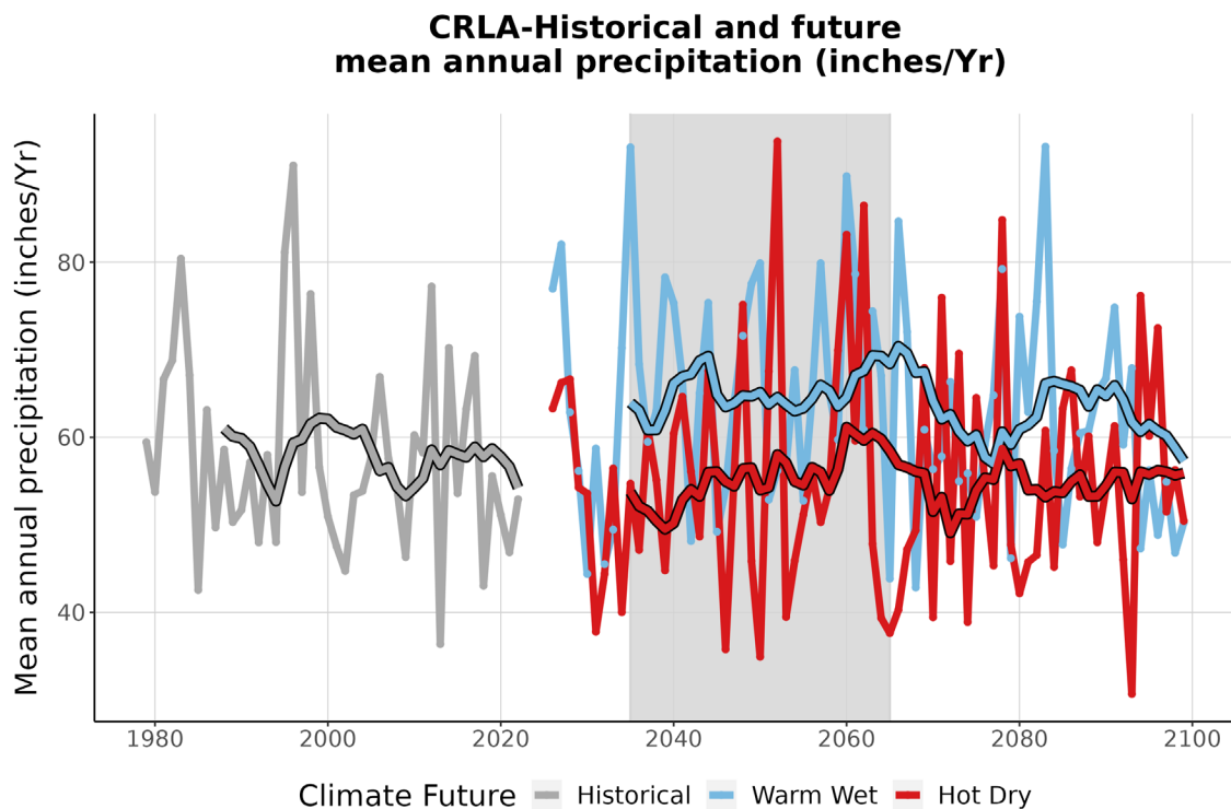
Figure 4. This graph compares observed average annual precipitation at CRLA (inches/year) (1979-2022) with projected average annual precipitation for the two climate futures over the period 2023-2099. The historically observed data is shown in gray, the Warm Wet climate future in blue, and the Hot Dry climate future in red. The smooth line running through each projection is the 10-year running average for historical observations and future projections. The gray-shaded area represents the time period that was averaged (2035-2065) to summarize future projections for the year 2050 (Appendix 1).
