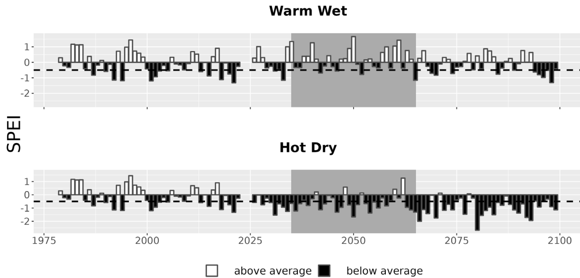
Figure 7. Drought metrics for CRLA. Drought index (SPEI; units = standard deviations from historical) timeseries for each climate future. Below-average SPEI (black bars) indicates dry conditions. The dotted line (SPEI = -0.5) indicates drought conditions.
