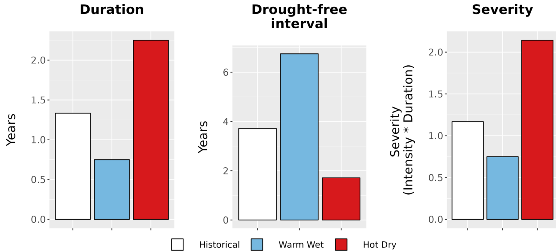
Figure 8. Drought metrics for CRLA. (Left) Average drought duration (years) historically (1979-2012) and under each climate future. (Middle) Average drought return interval (years), indicating the expected amount of time between periods of drought, historically and under each climate future. (Right) Average drought severity, a measure of drought intensity multiplied by duration, historically and under each climate future.
