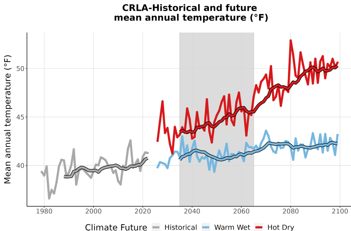
Figure 3. This graph compares observed average annual temperature at CRLA (°F) (1979-2022) with projected average annual temperature for the two climate futures over the period 2023-2099. The historically observed data
