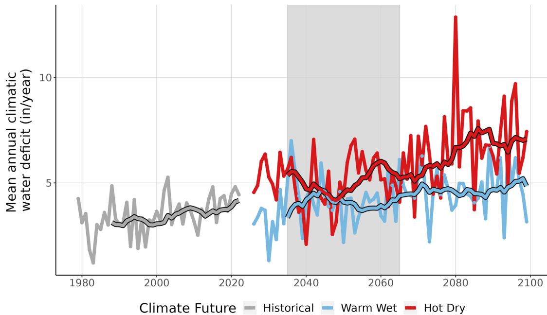
Figure 9. This line graph compares observed climatic water deficit at CRLA (inches/year) (1979-2022) with projected climatic water deficit for the two climate futures over the period 2023-2099. The historical observation data is shown in gray, the Warm Wet climate future in blue, and the Hot Dry climate future in red. The smooth line running through each projection is the 10-year running average for historical observations and future projections. Gray-shaded area represents the time period that was averaged (2035-2065) to summarize future projections for the year 2050.
