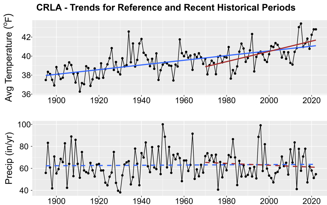
Figure 1. Historical trends in annual average temperature (upper plot) and annual total precipitation (lower plot) for CRLA from 1895-2022. Black points show yearly values while blue lines are linear regressions for the entire period record and red lines for 1970-2022 trends. Solid lines are significant trends (i.e., p < 0.05 ); dashed lines are not statistically significant.
