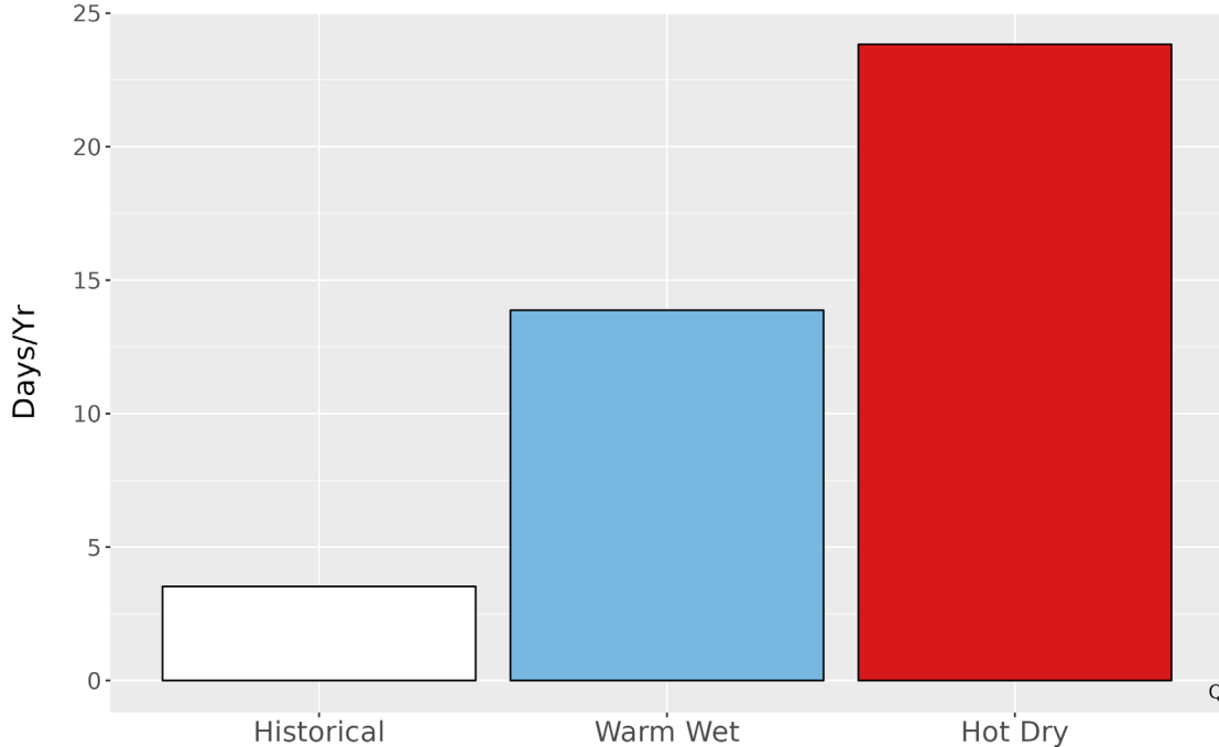
Figure 5. Metrics of extreme temperature at CRLA. The bar graph represents the average number of days annually with temperatures greater than the historical 99th percentile (81.6 °F) historically (1979-2012) and for the two climate futures (2050).
