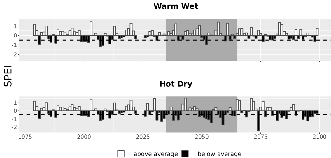
Figure 7. Drought metrics for COWP. Drought index (SPEI; units = standard deviations from historical) timeseries for each climate future. Below-average SPEI (black bars) indicates dry conditions. The dotted line (SPEI = -0.5) indicates drought conditions.
