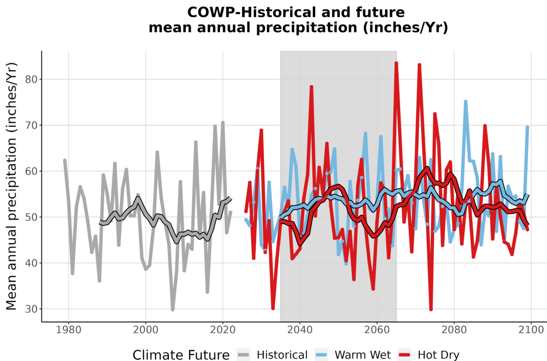
Figure 4. This graph compares observed average annual precipitation at COWP (inches/year) (1979-2022) with projected average annual precipitation for the two climate futures over the period 2023-2099. The historically observed data is shown in gray, the Warm Wet climate future in blue, and the Hot Dry climate future in red. The smooth line running through each projection is the 10-year running average for historical observations and future projections. The gray-shaded area represents the time period that was averaged (2035-2065) to summarize future projections for the year 2050 (Appendix 1).
