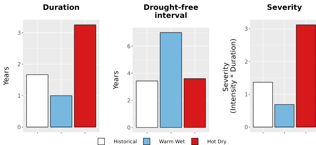
Figure 8. Drought metrics for COWP. (Left) Average drought duration (years) historically (1979-2012) and under each climate future. (Middle) Average drought return interval (years), indicating the expected amount of time between periods of drought, historically and under each climate future. (Right) Average drought severity, a measure of drought intensity multiplied by duration, historically and under each climate future.
