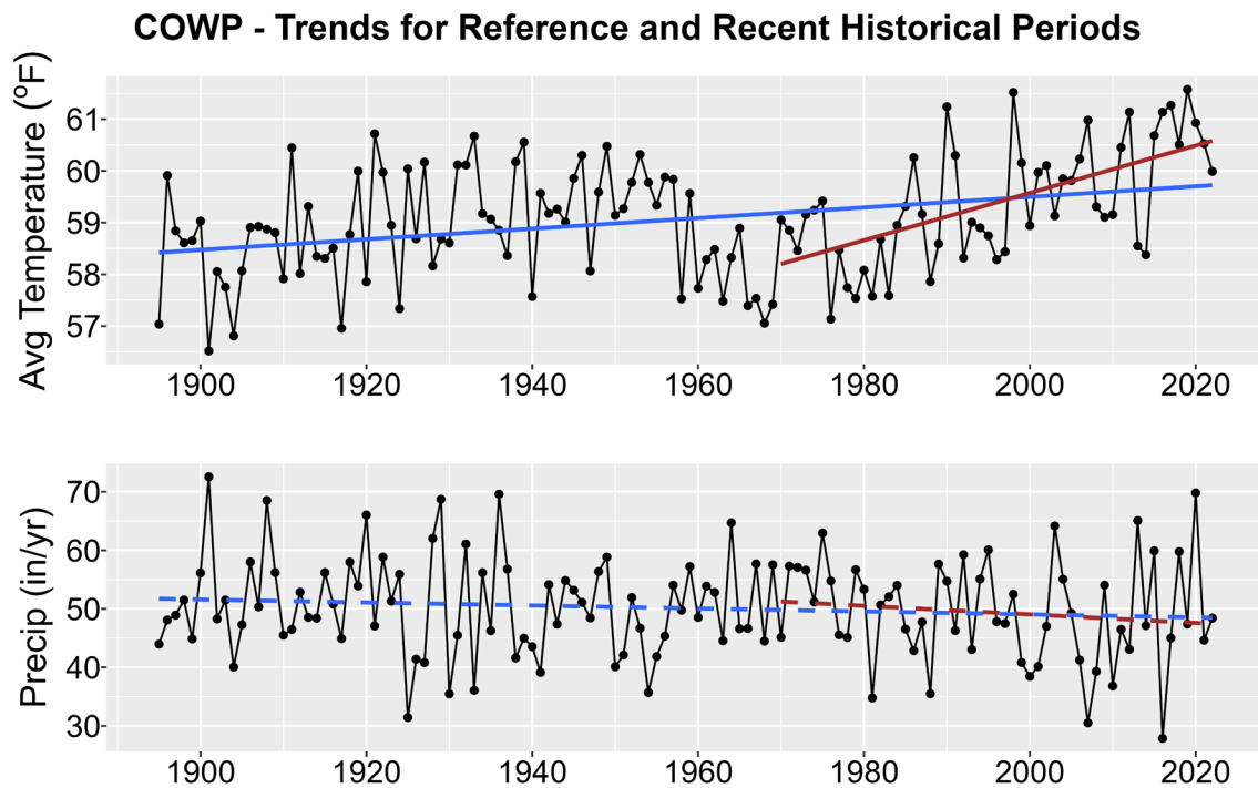
Figure 1. Historical trends in annual average temperature (upper plot) and annual total precipitation (lower plot) for COWP from 1895-2022. Black points show yearly values while blue lines are linear regressions for the entire period record and red lines for 1970-2022 trends. Solid lines are significant trends (i.e., p < 0.05 ); dashed lines are not statistically significant.
