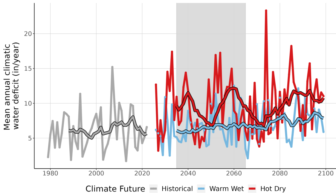
Figure 9. This line graph compares observed climatic water deficit at COWP (inches/year) (1979-2022) with projected climatic water deficit for the two climate futures over the period 2023-2099. The historical observation data is shown in gray, the Warm Wet climate future in blue, and the Hot Dry climate future in red. The smooth line running through each projection is the 10-year running average for historical observations and future projections. Gray-shaded area represents the time period that was averaged (2035-2065) to summarize future projections for the year 2050.
