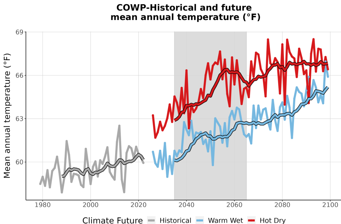
Figure 3. This graph compares observed average annual temperature at COWP (°F) (1979-2022) with projected average annual temperature for the two climate futures over the period 2023-2099. The historically observed data
