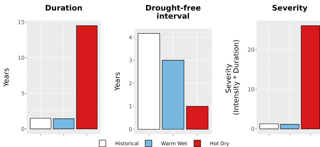
Figure 8. Drought metrics for CORO. (Left) Average drought duration (years) historically (1979-2012) and under each climate future. (Middle) Average drought return interval (years), indicating the expected amount of time between periods of drought, historically and under each climate future. (Right) Average drought severity, a measure of drought intensity multiplied by duration, historically and under each climate future.
