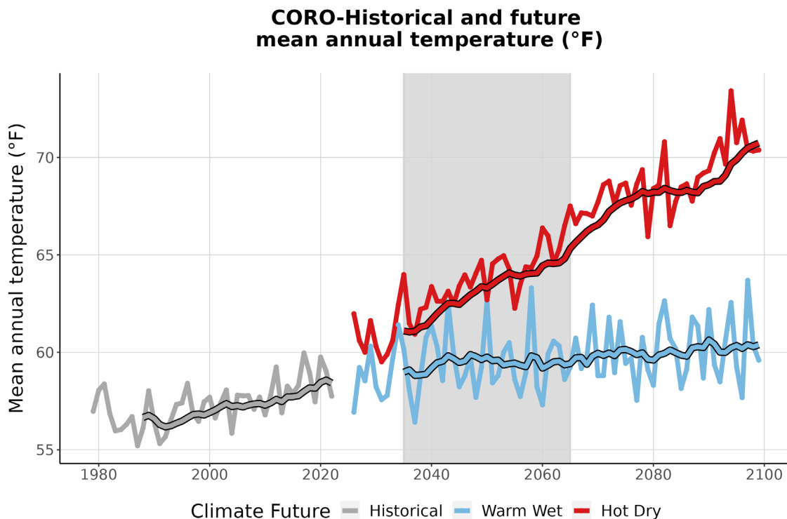
Figure 3. This graph compares observed average annual temperature at CORO (°F) (1979-2022) with projected average annual temperature for the two climate futures over the period 2023-2099. The historically observed data
