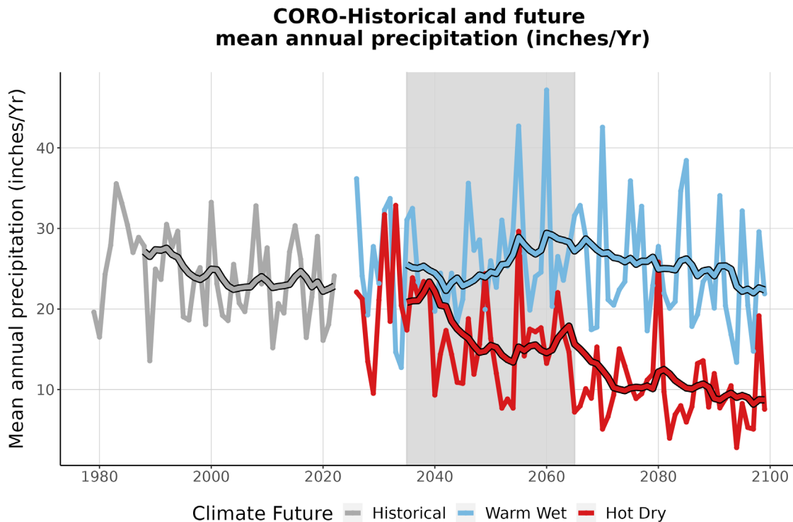
Figure 4. This graph compares observed average annual precipitation at CORO (inches/year) (1979-2022) with projected average annual precipitation for the two climate futures over the period 2023-2099. The historically observed data is shown in gray, the Warm Wet climate future in blue, and the Hot Dry climate future in red. The smooth line running through each projection is the 10-year running average for historical observations and future projections. The gray-shaded area represents the time period that was averaged (2035-2065) to summarize future projections for the year 2050 (Appendix 1).
