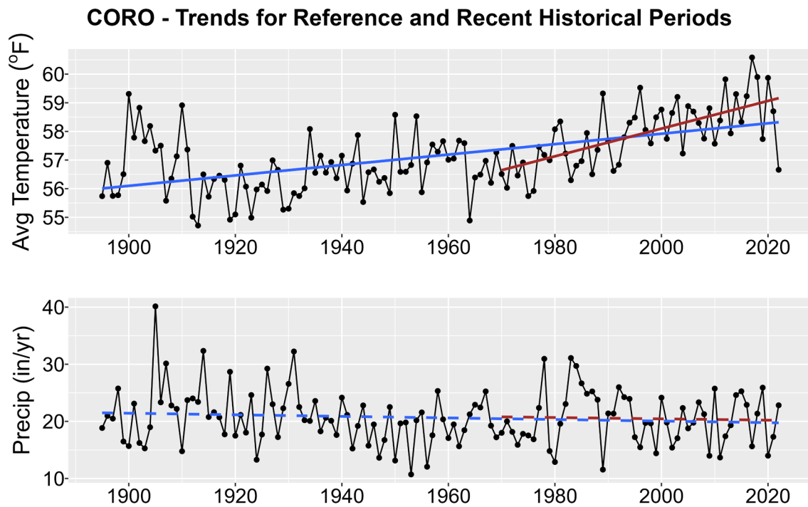
Figure 1. Historical trends in annual average temperature (upper plot) and annual total precipitation (lower plot) for CORO from 1895-2022. Black points show yearly values while blue lines are linear regressions for the entire period record and red lines for 1970-2022 trends. Solid lines are significant trends (i.e., p < 0.05 ); dashed lines are not statistically significant.
