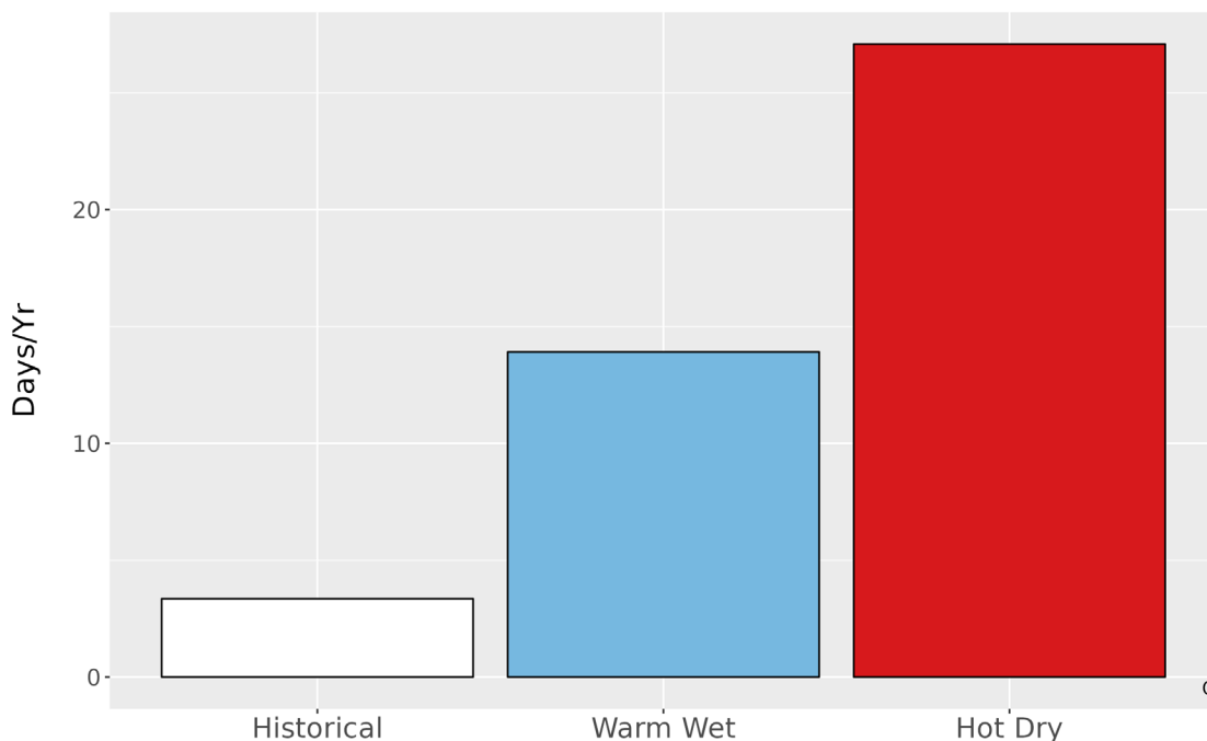
Figure 5. Metrics of extreme temperature at CORO. The bar graph represents the average number of days annually with temperatures greater than the historical 99th percentile (94.2 °F) historically (1979-2012) and for the two climate futures (2050).
