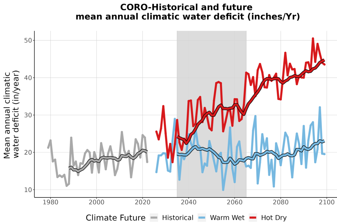
Figure 9. This line graph compares observed climatic water deficit at CORO (inches/year) (1979-2022) with projected climatic water deficit for the two climate futures over the period 2023-2099. The historical observation data is shown in gray, the Warm Wet climate future in blue, and the Hot Dry climate future in red. The smooth line running through each projection is the 10-year running average for historical observations and future projections. Gray-shaded area represents the time period that was averaged (2035-2065) to summarize future projections for the year 2050.
