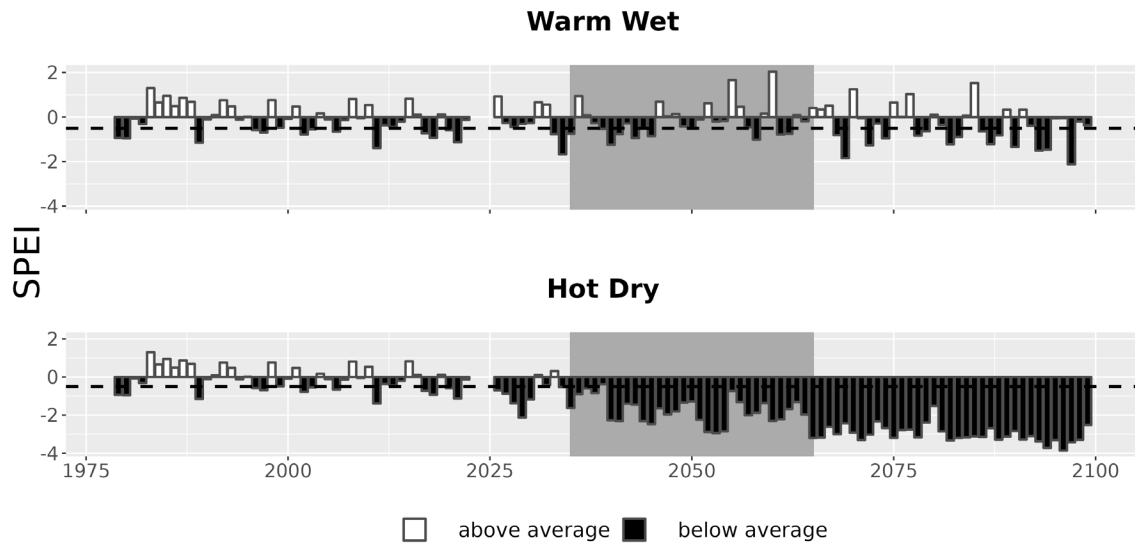
Figure 7. Drought metrics for CORO. Drought index (SPEI; units = standard deviations from historical) timeseries for each climate future. Below-average SPEI (black bars) indicates dry conditions. The dotted line (SPEI = -0.5) indicates drought conditions.
