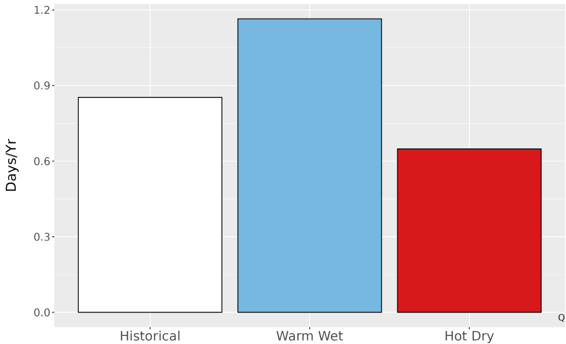
Figure 6. Average number of days annually with precipitation exceeding the 99th percentile (1.4 in.) of precipitation from the historical period 1979-2012 and for each climate future.
