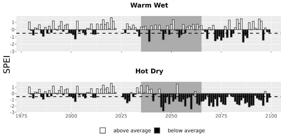
Figure 7. Drought metrics for CONG. Drought index (SPEI; units = standard deviations from historical) timeseries for each climate future. Below-average SPEI (black bars) indicates dry conditions. The dotted line (SPEI = -0.5) indicates drought conditions.
