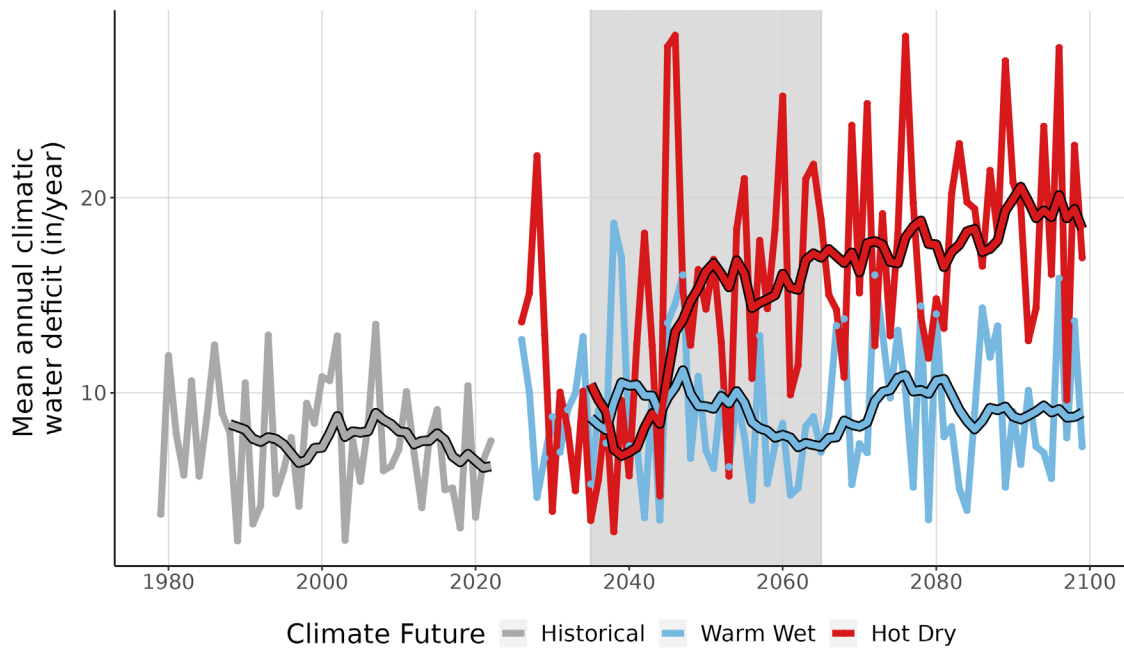
Figure 9. This line graph compares observed climatic water deficit at CONG (inches/year) (1979-2022) with projected climatic water deficit for the two climate futures over the period 2023-2099. The historical observation data is shown in gray, the Warm Wet climate future in blue, and the Hot Dry climate future in red. The smooth line running through each projection is the 10-year running average for historical observations and future projections. Gray-shaded area represents the time period that was averaged (2035-2065) to summarize future projections for the year 2050.
