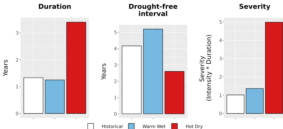
Figure 8. Drought metrics for CONG. (Left) Average drought duration (years) historically (1979-2012) and under each climate future. (Middle) Average drought return interval (years), indicating the expected amount of time between periods of drought, historically and under each climate future. (Right) Average drought severity, a measure of drought intensity multiplied by duration, historically and under each climate future.
