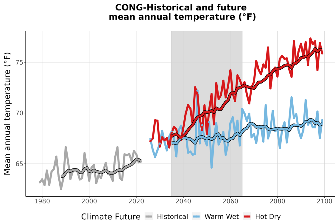
Figure 3. This graph compares observed average annual temperature at CONG (°F) (1979-2022) with projected average annual temperature for the two climate futures over the period 2023-2099. The historically observed data
