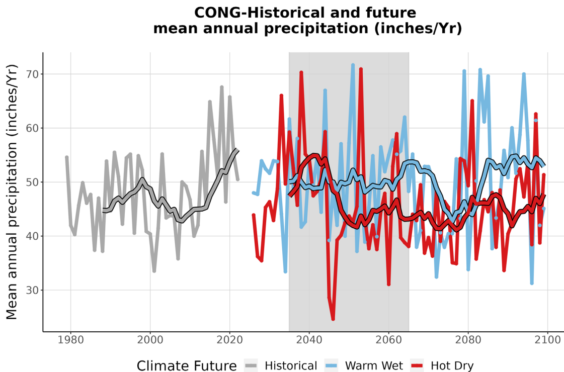
Figure 4. This graph compares observed average annual precipitation at CONG (inches/year) (1979-2022) with projected average annual precipitation for the two climate futures over the period 2023-2099. The historically observed data is shown in gray, the Warm Wet climate future in blue, and the Hot Dry climate future in red. The smooth line running through each projection is the 10-year running average for historical observations and future projections. The gray-shaded area represents the time period that was averaged (2035-2065) to summarize future projections for the year 2050 (Appendix 1).
