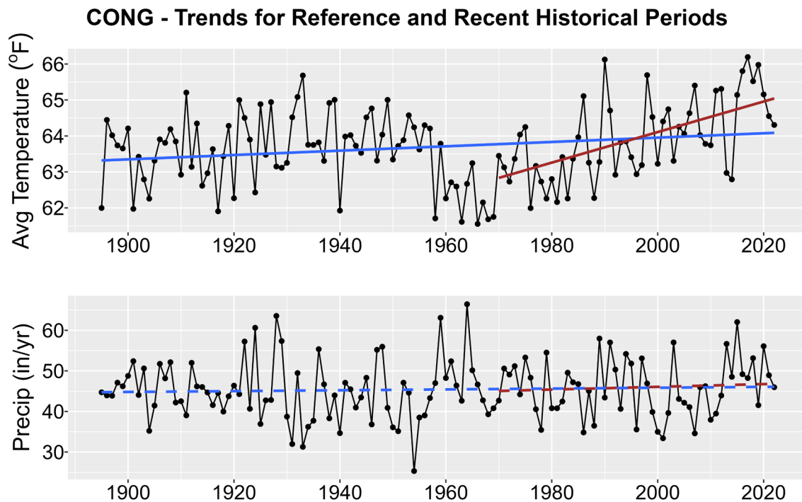
Figure 1. Historical trends in annual average temperature (upper plot) and annual total precipitation (lower plot) for CONG from 1895-2022. Black points show yearly values while blue lines are linear regressions for the entire period record and red lines for 1970-2022 trends. Solid lines are significant trends (i.e., p < 0.05 ); dashed lines are not statistically significant.
