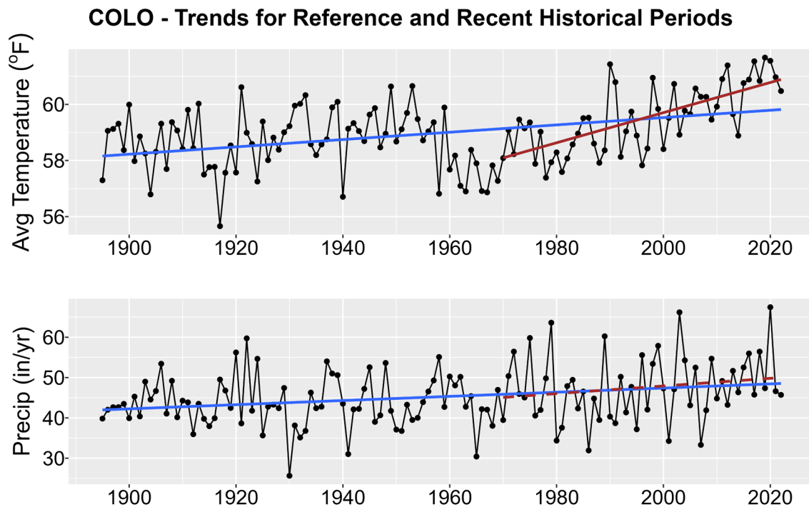
Figure 1. Historical trends in annual average temperature (upper plot) and annual total precipitation (lower plot) for COLO from 1895-2022. Black points show yearly values while blue lines are linear regressions for the entire period record and red lines for 1970-2022 trends. Solid lines are significant trends (i.e., p < 0.05 ); dashed lines are not statistically significant.
