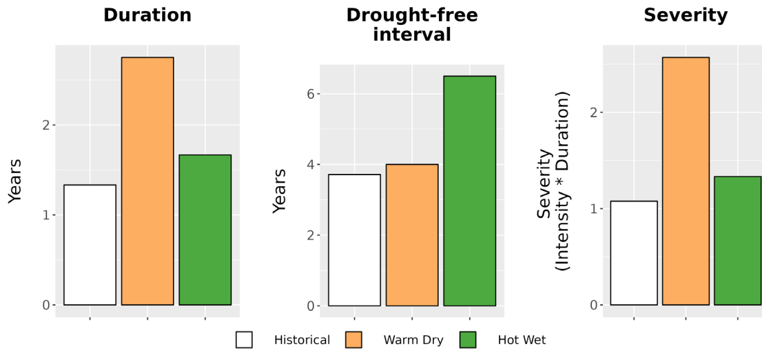
Figure 8. Drought metrics for COLO. (Left) Average drought duration (years) historically (1979-2012) and under each climate future. (Middle) Average drought return interval (years), indicating the expected amount of time between periods of drought, historically and under each climate future. (Right) Average drought severity, a measure of drought intensity multiplied by duration, historically and under each climate future.
