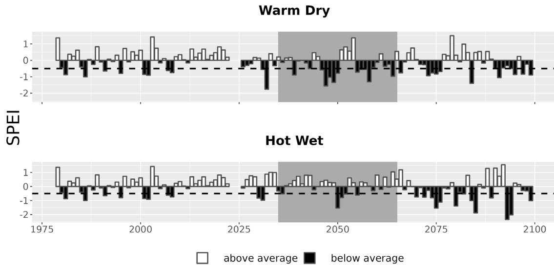
Figure 7. Drought metrics for COLO. Drought index (SPEI; units = standard deviations from historical) timeseries for each climate future. Below-average SPEI (black bars) indicates dry conditions. The dotted line (SPEI = -0.5) indicates drought conditions.
