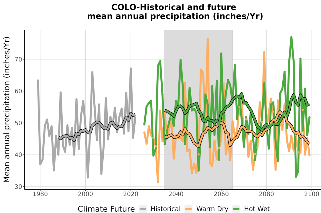
Figure 4. This graph compares observed average annual precipitation at COLO (inches/year) (1979-2022) with projected average annual precipitation for the two climate futures over the period 2023-2099. The historically observed data is shown in gray, the Warm Dry climate future in orange, and the Hot Wet climate future in green. The smooth line running through each projection is the 10-year running average for historical observations and future projections. The gray-shaded area represents the time period that was averaged (2035-2065) to summarize future projections for the year 2050 (Appendix 1).
