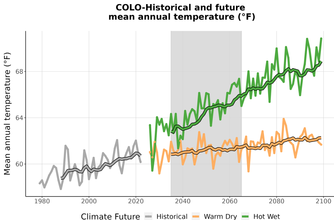
Figure 3. This graph compares observed average annual temperature at COLO (°F) (1979-2022) with projected average annual temperature for the two climate futures over the period 2023-2099. The historically observed data
