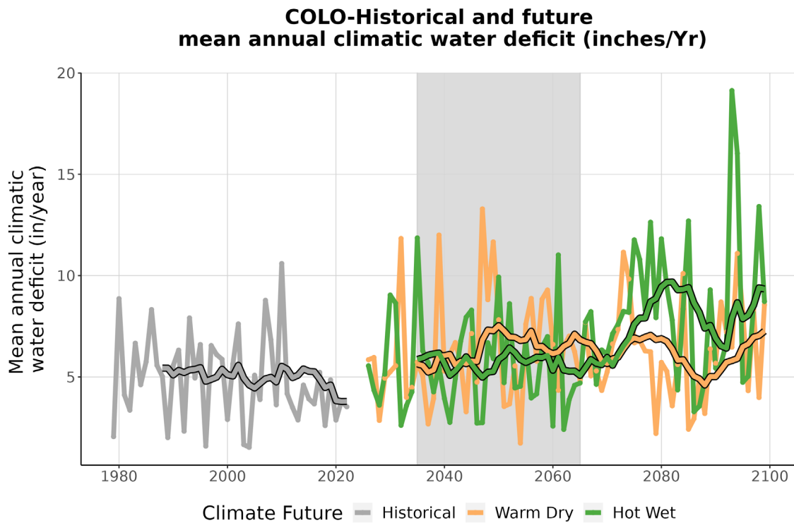
Figure 9. This line graph compares observed climatic water deficit at COLO (inches/year) (1979-2022) with projected climatic water deficit for the two climate futures over the period 2023-2099. The historical observation data is shown in gray, the Warm Dry climate future in orange, and the Hot Wet climate future in green. The smooth line running through each projection is the 10-year running average for historical observations and future projections. Gray-shaded area represents the time period that was averaged (2035-2065) to summarize future projections for the year 2050.
