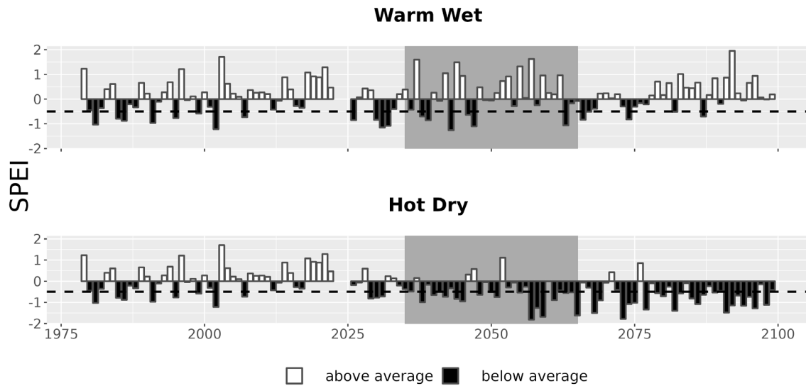
Figure 7. Drought metrics for COGA. Drought index (SPEI; units = standard deviations from historical) timeseries for each climate future. Below-average SPEI (black bars) indicates dry conditions. The dotted line (SPEI = -0.5) indicates drought conditions.
