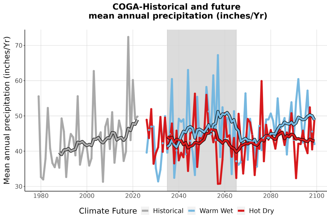
Figure 4. This graph compares observed average annual precipitation at COGA (inches/year) (1979-2022) with projected average annual precipitation for the two climate futures over the period 2023-2099. The historically observed data is shown in gray, the Warm Wet climate future in blue, and the Hot Dry climate future in red. The smooth line running through each projection is the 10-year running average for historical observations and future projections. The gray-shaded area represents the time period that was averaged (2035-2065) to summarize future projections for the year 2050 (Appendix 1).
