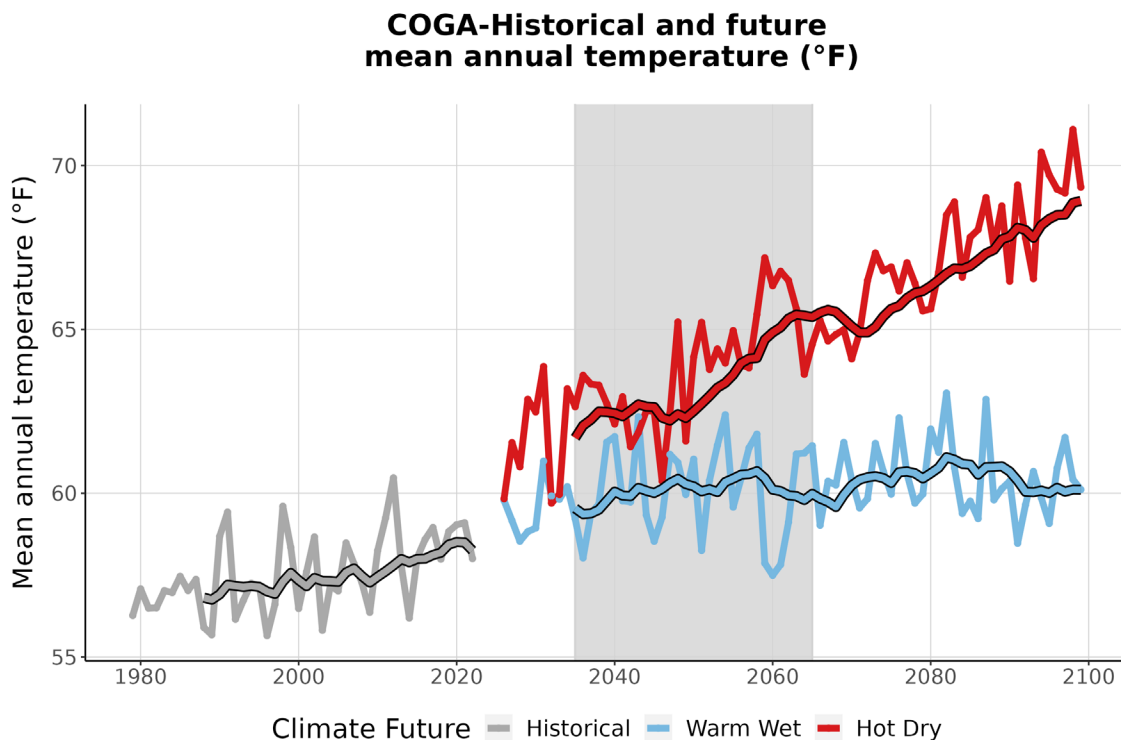
Figure 3. This graph compares observed average annual temperature at COGA (°F) (1979-2022) with projected average annual temperature for the two climate futures over the period 2023-2099. The historically observed data
