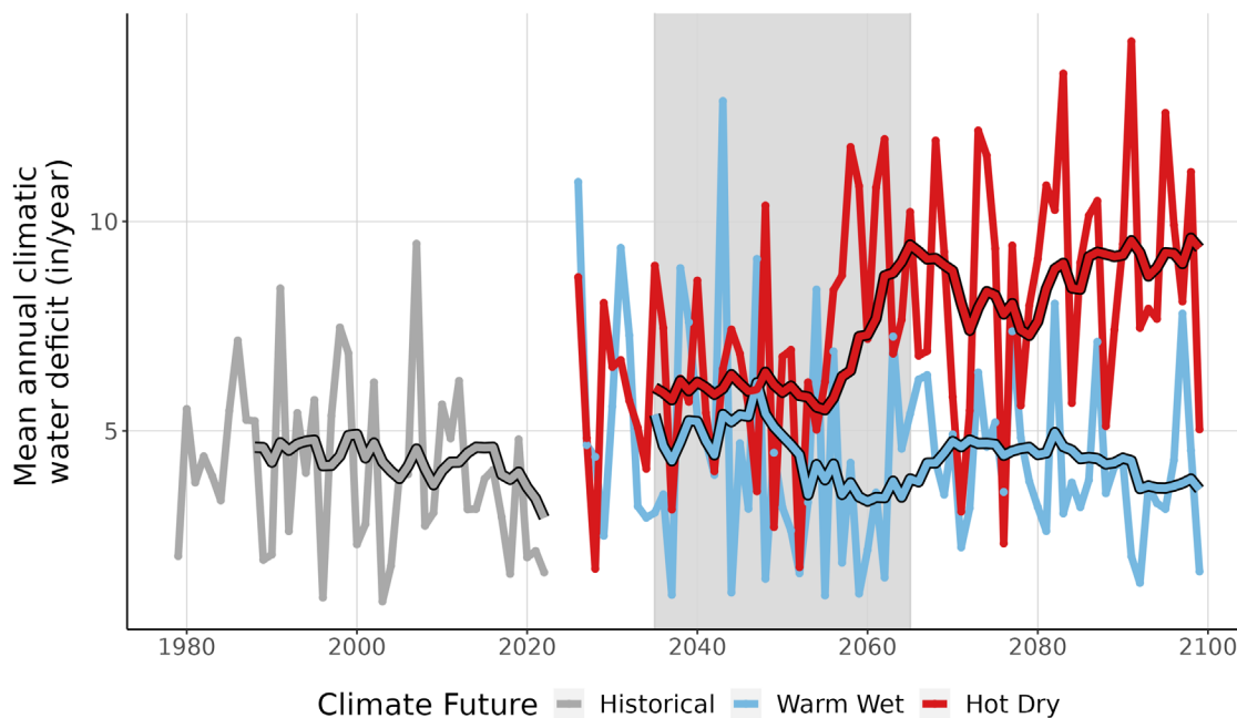
Figure 9. This line graph compares observed climatic water deficit at COGA (inches/year) (1979-2022) with projected climatic water deficit for the two climate futures over the period 2023-2099. The historical observation data is shown in gray, the Warm Wet climate future in blue, and the Hot Dry climate future in red. The smooth line running through each projection is the 10-year running average for historical observations and future projections. Gray-shaded area represents the time period that was averaged (2035-2065) to summarize future projections for the year 2050.
