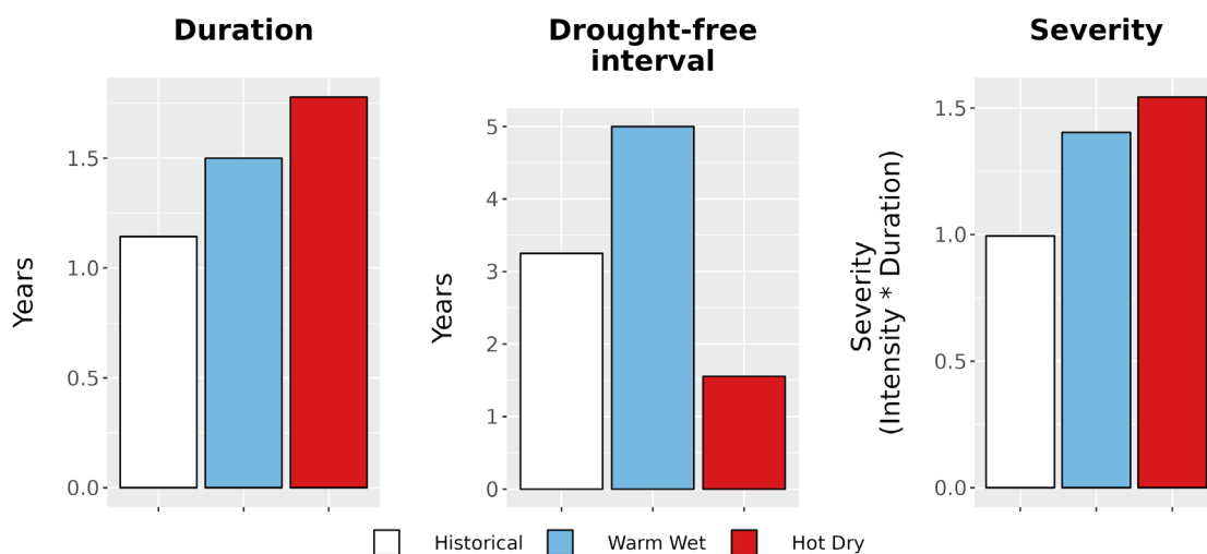
Figure 8. Drought metrics for COGA. (Left) Average drought duration (years) historically (1979-2012) and under each climate future. (Middle) Average drought return interval (years), indicating the expected amount of time between periods of drought, historically and under each climate future. (Right) Average drought severity, a measure of drought intensity multiplied by duration, historically and under each climate future.
