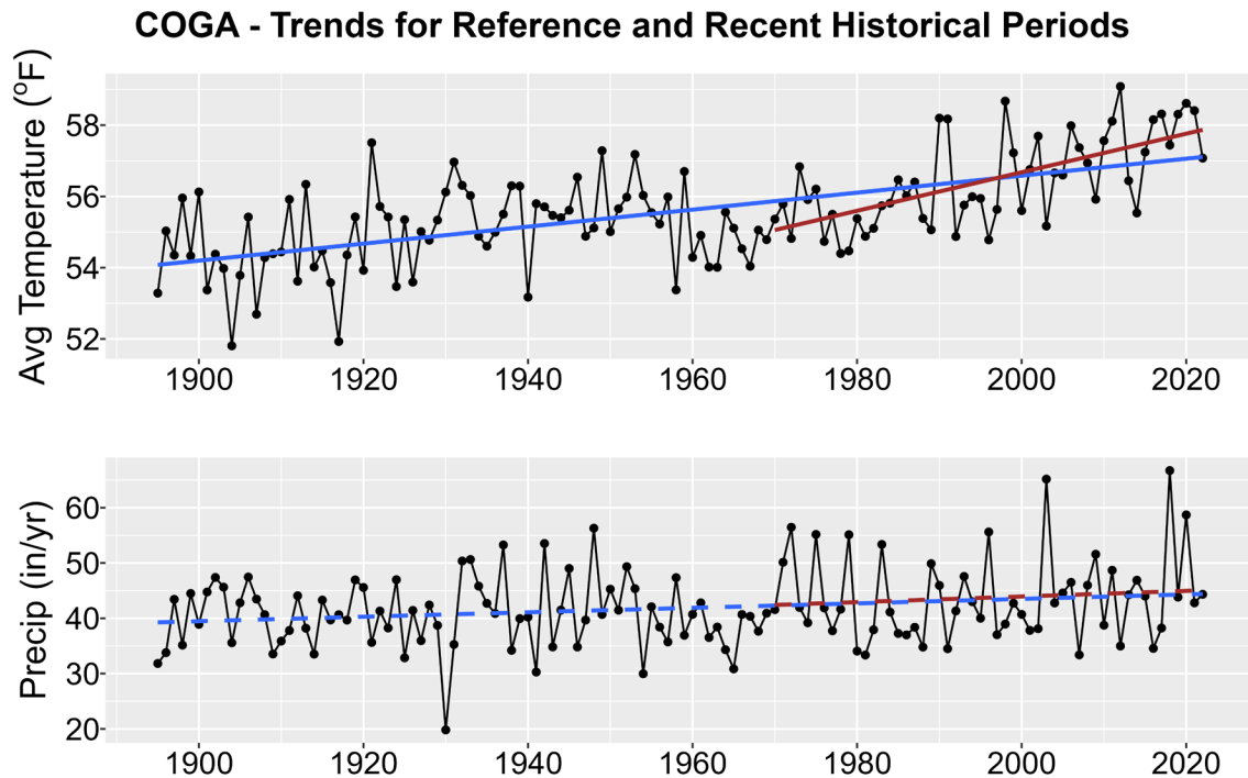
Figure 1. Historical trends in annual average temperature (upper plot) and annual total precipitation (lower plot) for COGA from 1895-2022. Black points show yearly values while blue lines are linear regressions for the entire period record and red lines for 1970-2022 trends. Solid lines are significant trends (i.e., p < 0.05 ); dashed lines are not statistically significant.
