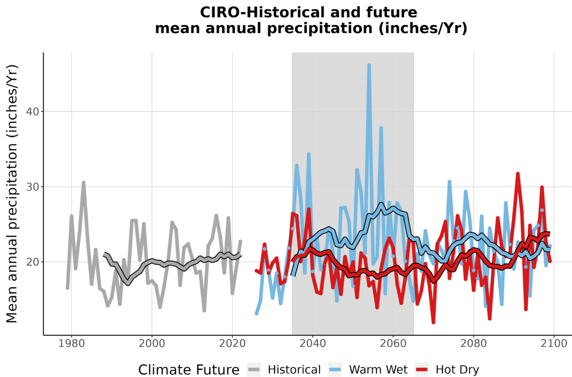
Figure 4. This graph compares observed average annual precipitation at CIRO (inches/year) (1979-2022) with projected average annual precipitation for the two climate futures over the period 2023-2099. The historically observed data is shown in gray, the Warm Wet climate future in blue, and the Hot Dry climate future in red. The smooth line running through each projection is the 10-year running average for historical observations and future projections. The gray-shaded area represents the time period that was averaged (2035-2065) to summarize future projections for the year 2050 (Appendix 1).
