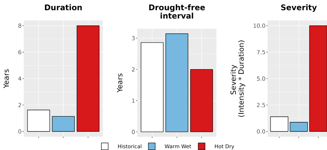
Figure 8. Drought metrics for CIRO. (Left) Average drought duration (years) historically (1979-2012) and under each climate future. (Middle) Average drought return interval (years), indicating the expected amount of time between periods of drought, historically and under each climate future. (Right) Average drought severity, a measure of drought intensity multiplied by duration, historically and under each climate future.
