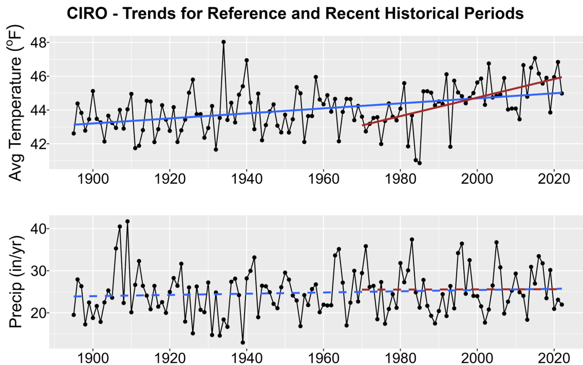
Figure 1. Historical trends in annual average temperature (upper plot) and annual total precipitation (lower plot) for CIRO from 1895-2022. Black points show yearly values while blue lines are linear regressions for the entire period record and red lines for 1970-2022 trends. Solid lines are significant trends (i.e., p < 0.05 ); dashed lines are not statistically significant.
