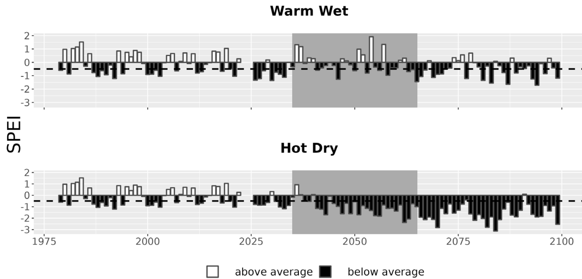
Figure 7. Drought metrics for CIRO. Drought index (SPEI; units = standard deviations from historical) timeseries for each climate future. Below-average SPEI (black bars) indicates dry conditions. The dotted line (SPEI = -0.5) indicates drought conditions.
