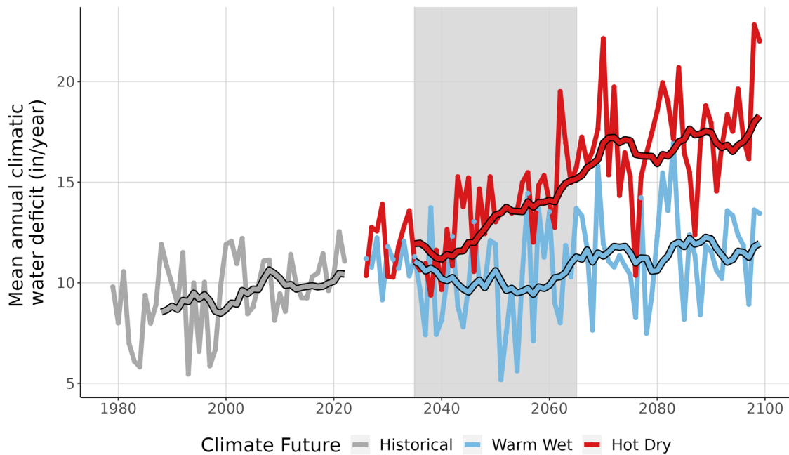
Figure 9. This line graph compares observed climatic water deficit at CIRO (inches/year) (1979-2022) with projected climatic water deficit for the two climate futures over the period 2023-2099. The historical observation data is shown in gray, the Warm Wet climate future in blue, and the Hot Dry climate future in red. The smooth line running through each projection is the 10-year running average for historical observations and future projections. Gray-shaded area represents the time period that was averaged (2035-2065) to summarize future projections for the year 2050.
