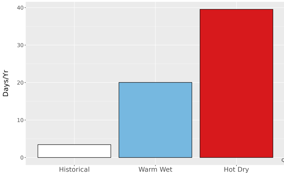
Figure 5. Metrics of extreme temperature at CIRO. The bar graph represents the average number of days annually with temperatures greater than the historical 99th percentile (88.8 °F) historically (1979-2012) and for the two climate futures (2050).
