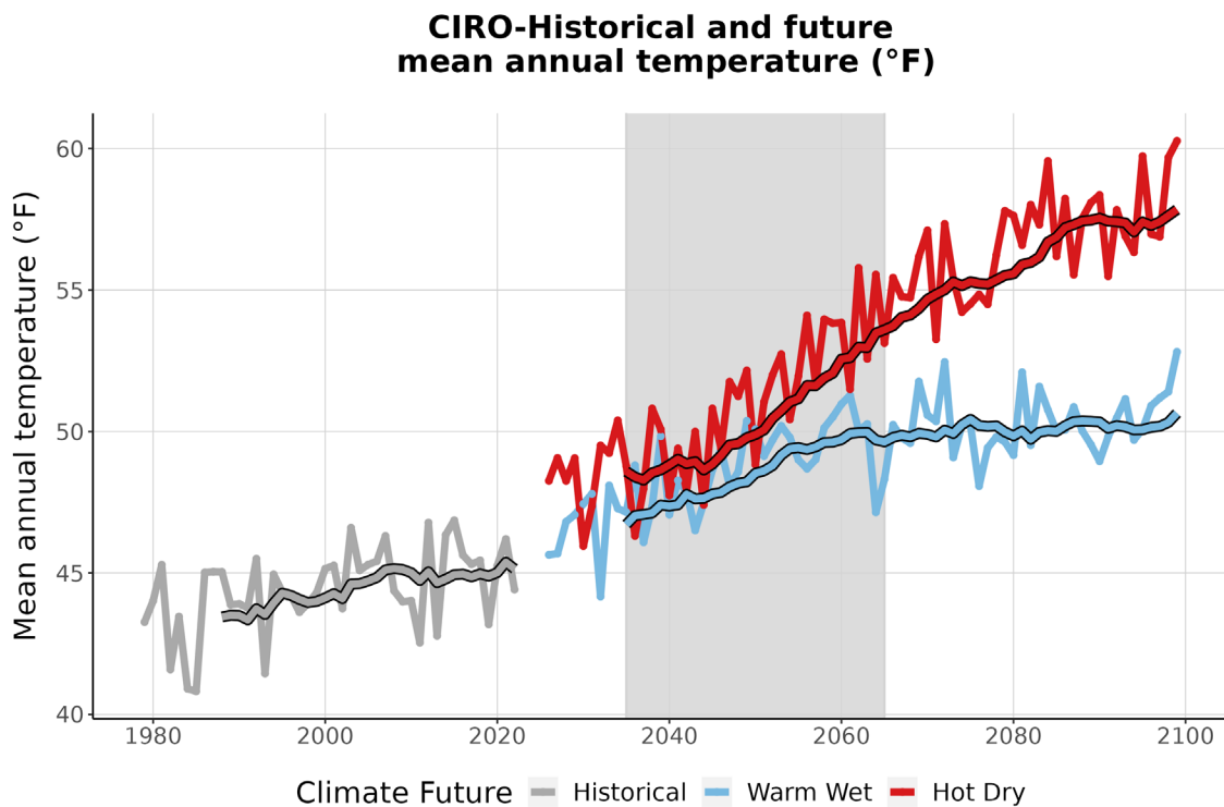
Figure 3. This graph compares observed average annual temperature at CIRO (°F) (1979-2022) with projected average annual temperature for the two climate futures over the period 2023-2099. The historically observed data is shown in gray, the Warm Wet climate future in blue, and the Hot Dry climate future in red. The smooth line
