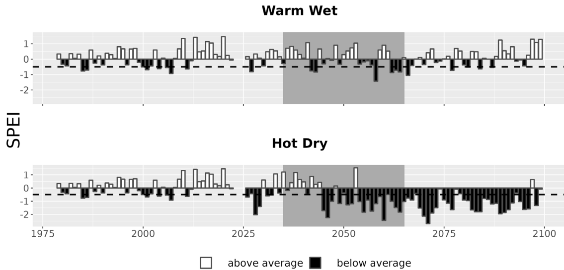
Figure 7. Drought metrics for CHPI. Drought index (SPEI; units = standard deviations from historical) timeseries for each climate future. Below-average SPEI (black bars) indicates dry conditions. The dotted line (SPEI = -0.5) indicates drought conditions.
