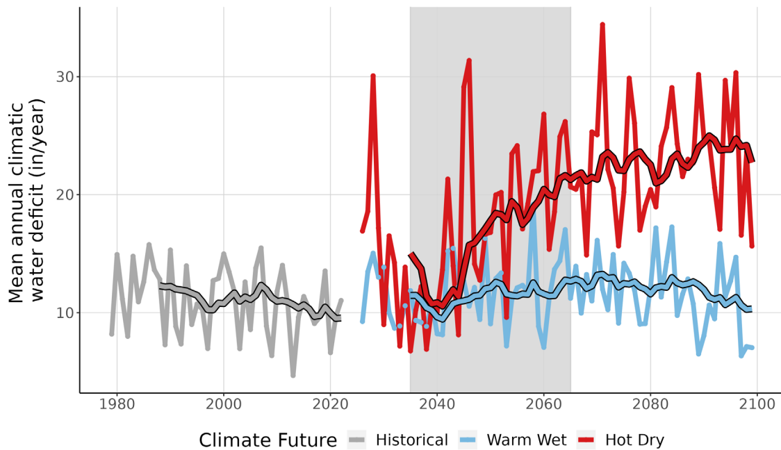
Figure 9. This line graph compares observed climatic water deficit at CHPI (inches/year) (1979-2022) with projected climatic water deficit for the two climate futures over the period 2023-2099. The historical observation data is shown in gray, the Warm Wet climate future in blue, and the Hot Dry climate future in red. The smooth line running through each projection is the 10-year running average for historical observations and future projections. Gray-shaded area represents the time period that was averaged (2035-2065) to summarize future projections for the year 2050.
