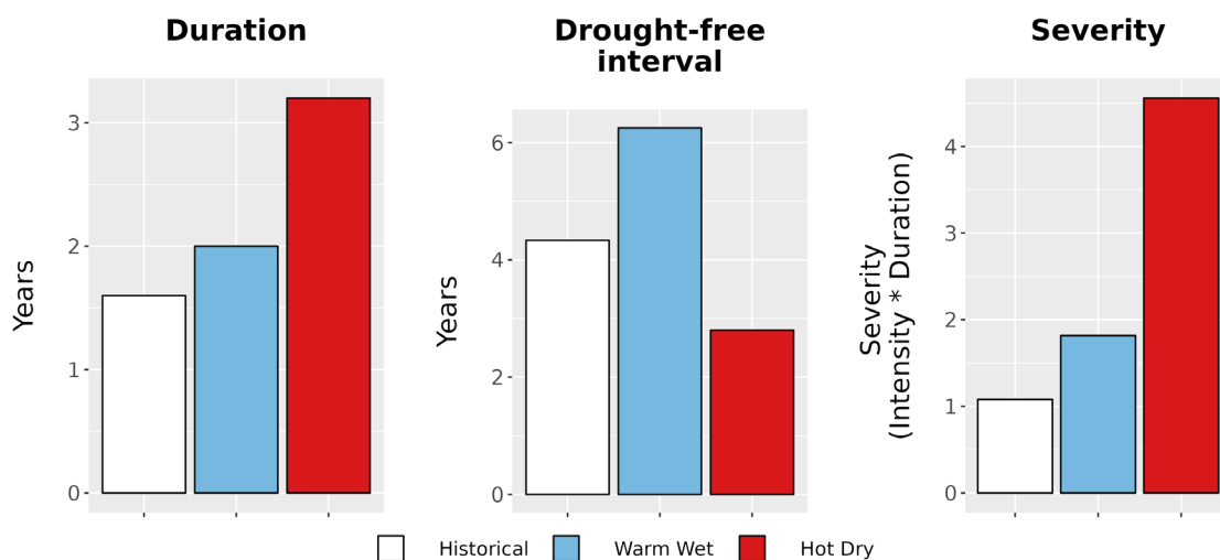
Figure 8. Drought metrics for CHPI. (Left) Average drought duration (years) historically (1979-2012) and under each climate future. (Middle) Average drought return interval (years), indicating the expected amount of time between periods of drought, historically and under each climate future. (Right) Average drought severity, a measure of drought intensity multiplied by duration, historically and under each climate future.
