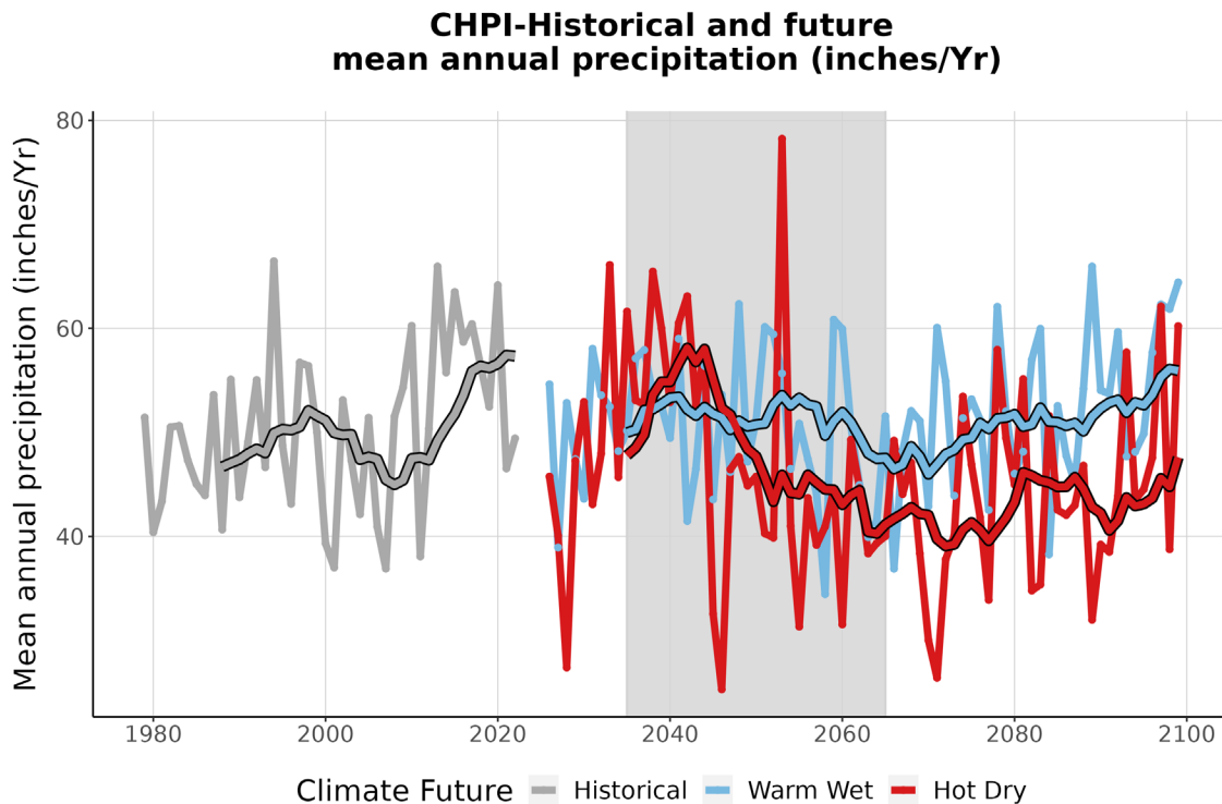
Figure 4. This graph compares observed average annual precipitation at CHPI (inches/year) (1979-2022) with projected average annual precipitation for the two climate futures over the period 2023-2099. The historically observed data is shown in gray, the Warm Wet climate future in blue, and the Hot Dry climate future in red. The smooth line running through each projection is the 10-year running average for historical observations and future projections. The gray-shaded area represents the time period that was averaged (2035-2065) to summarize future projections for the year 2050 (Appendix 1).
