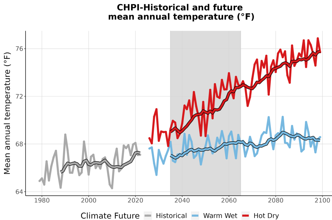
Figure 3. This graph compares observed average annual temperature at CHPI (°F) (1979-2022) with projected average annual temperature for the two climate futures over the period 2023-2099. The historically observed data
