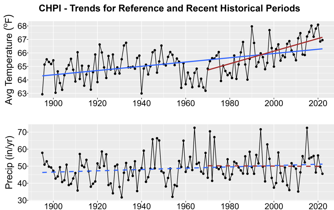
Figure 1. Historical trends in annual average temperature (upper plot) and annual total precipitation (lower plot) for CHPI from 1895-2022. Black points show yearly values while blue lines are linear regressions for the entire period record and red lines for 1970-2022 trends. Solid lines are significant trends (i.e., p < 0.05 ); dashed lines are not statistically significant.
