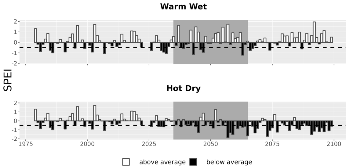
Figure 7. Drought metrics for CHOH. Drought index (SPEI; units = standard deviations from historical) timeseries for each climate future. Below-average SPEI (black bars) indicates dry conditions. The dotted line (SPEI = -0.5) indicates drought conditions.
