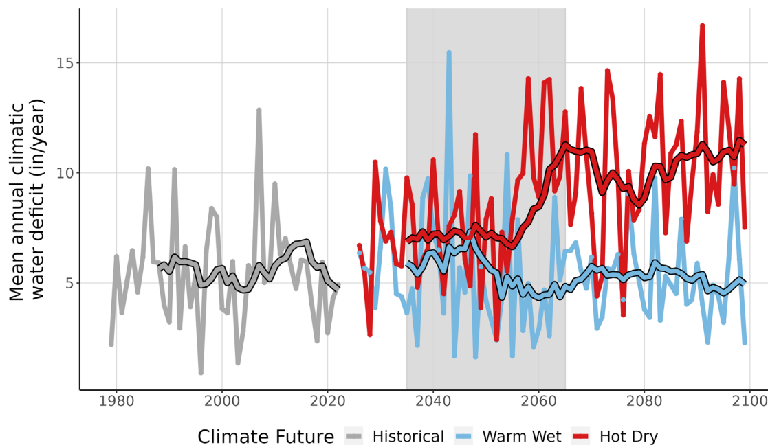
Figure 9. This line graph compares observed climatic water deficit at CCHOH (inches/year) (1979-2022) with projected climatic water deficit for the two climate futures over the period 2023-2099. The historical observation data is shown in gray, the Warm Wet climate future in blue, and the Hot Dry climate future in red. The smooth line running through each projection is the 10-year running average for historical observations and future projections. Gray-shaded area represents the time period that was averaged (2035-2065) to summarize future projections for the year 2050.
