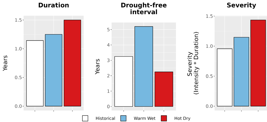
Figure 8. Drought metrics for CHO. (Left) Average drought duration (years) historically (1979-2012) and under each climate future. (Middle) Average drought return interval (years), indicating the expected amount of time between periods of drought, historically and under each climate future. (Right) Average drought severity, a measure of drought intensity multiplied by duration, historically and under each climate future.
