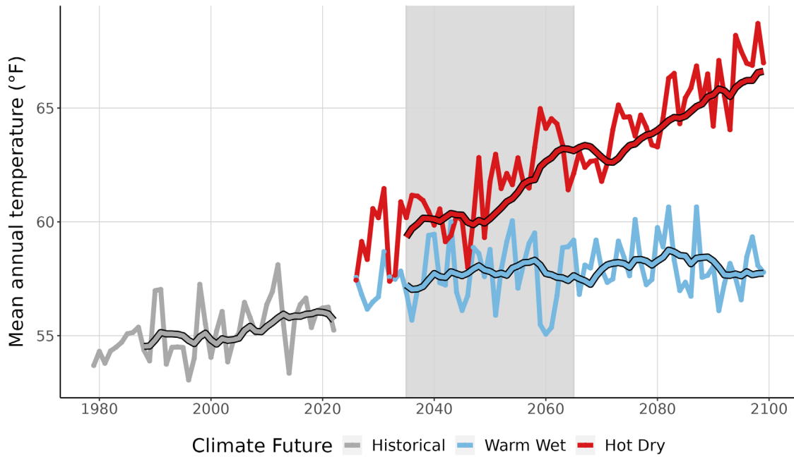
Figure 3. This graph compares observed average annual temperature at CHOH (°F) (1979-2022) with projected average annual temperature for the two climate futures over the period 2023-2099. The historically observed data is shown in gray, the Warm Wet climate future in blue, and the Hot Dry climate future in red. The smooth line running through each projection is the 10-year running average for historical observations and future projections. Gray-shaded area represents the time period that was averaged (2035-2065) to summarize future projections for the year 2050 (Appendix 1).
