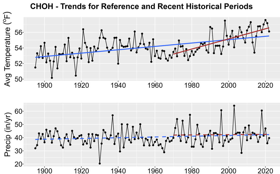
Figure 1. Historical trends in annual average temperature (upper plot) and annual total precipitation (lower plot) for CHOH from 1895-2022. Black points show yearly values while blue lines are linear regressions for the entire
