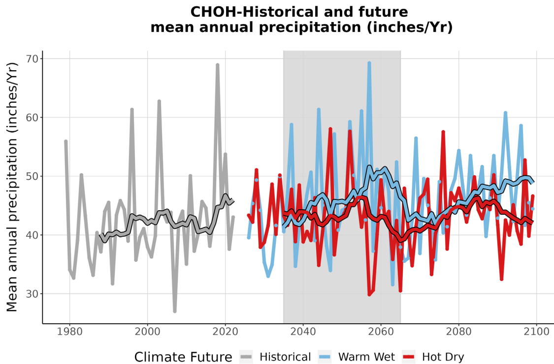
Figure 4. This graph compares observed average annual precipitation at CHOH (inches/year) (1979-2022) with projected average annual precipitation for the two climate futures over the period 2023-2099. The historically observed data is shown in gray, the Warm Wet climate future in blue, and the Hot Dry climate future in red. The smooth line running through each projection is the 10-year running average for historical observations and future projections. The gray-shaded area represents the time period that was averaged (2035-2065) to summarize future projections for the year 2050 (Appendix 1).
