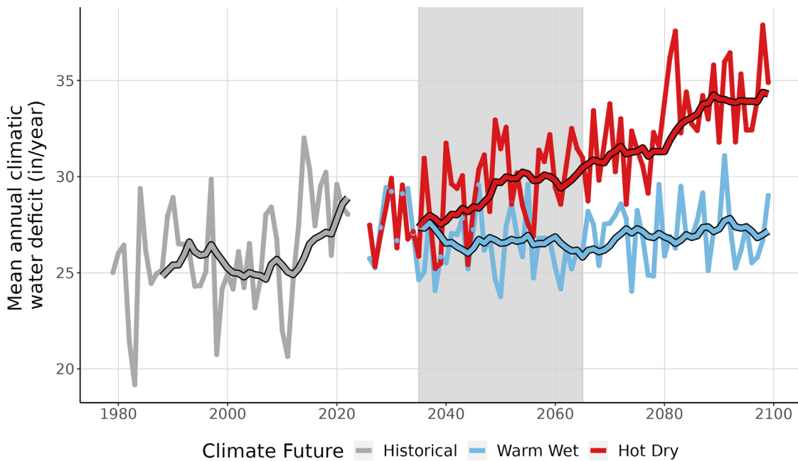
Figure 9. This line graph compares observed climatic water deficit at CHIS (inches/year) (1979-2022) with projected climatic water deficit for the two climate futures over the period 2023-2099. The historical observation data is shown in gray, the Warm Wet climate future in blue, and the Hot Dry climate future in red. The smooth line running through each projection is the 10-year running average for historical observations and future projections. Gray-shaded area represents the time period that was averaged (2035-2065) to summarize future projections for the year 2050.
