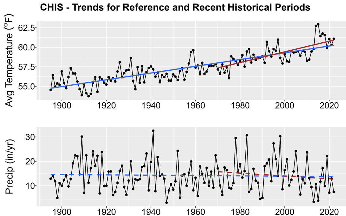
Figure 1. Historical trends in annual average temperature (upper plot) and annual total precipitation (lower plot) for CHIS from 1895-2022. Black points show yearly values while blue lines are linear regressions for the entire period record and red lines for 1970-2022 trends. Solid lines are significant trends (i.e., p < 0.05 ); dashed lines are not statistically significant.
