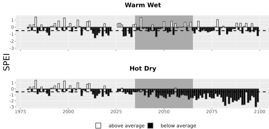
Figure 7. Drought metrics for CHIS. Drought index (SPEI; units = standard deviations from historical) timeseries for each climate future. Below-average SPEI (black bars) indicates dry conditions. The dotted line (SPEI = -0.5) indicates drought conditions.
