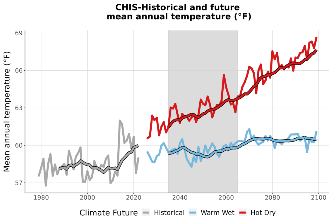
Figure 3. This graph compares observed average annual temperature at CHIS (°F) (1979-2022) with projected average annual temperature for the two climate futures over the period 2023-2099. The historically observed data
