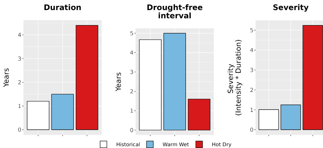
Figure 8. Drought metrics for CHIS. (Left) Average drought duration (years) historically (1979-2012) and under each climate future. (Middle) Average drought return interval (years), indicating the expected amount of time between periods of drought, historically and under each climate future. (Right) Average drought severity, a measure of drought intensity multiplied by duration, historically and under each climate future.
