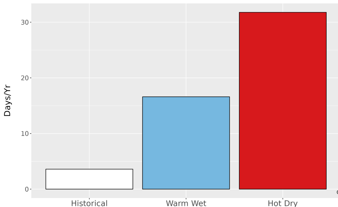
Figure 5. Metrics of extreme temperature at CHIS. The bar graph represents the average number of days annually with temperatures greater than the historical 99th percentile (80.5 °F) historically (1979-2012) and for the two climate futures (2050).
