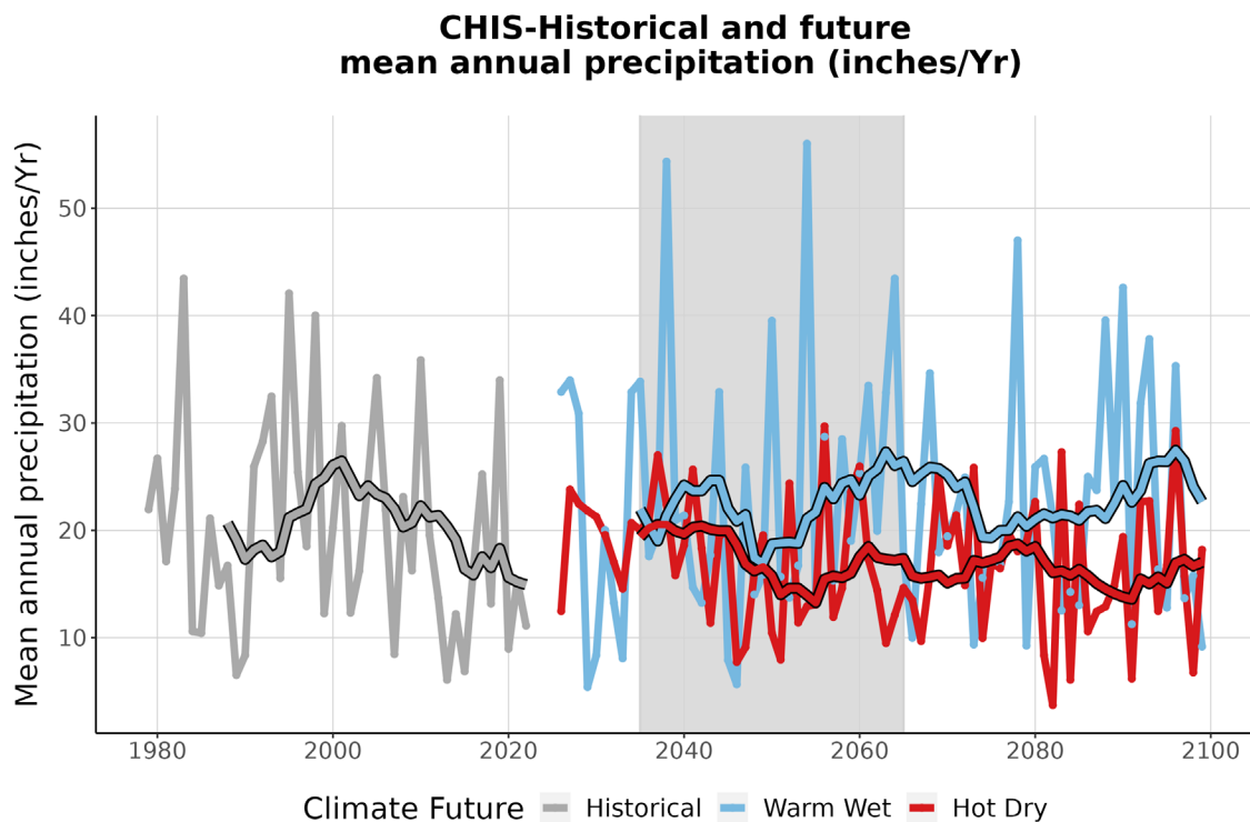
Figure 4. This graph compares observed average annual precipitation at CHIS (inches/year) (1979-2022) with projected average annual precipitation for the two climate futures over the period 2023-2099. The historically observed data is shown in gray, the Warm Wet climate future in blue, and the Hot Dry climate future in red. The smooth line running through each projection is the 10-year running average for historical observations and future projections. The gray-shaded area represents the time period that was averaged (2035-2065) to summarize future projections for the year 2050 (Appendix 1).
