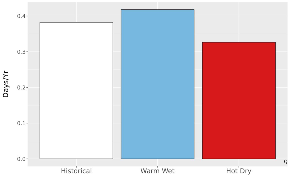
Figure 6. Average number of days annually with precipitation exceeding the 99th percentile (3.4 in.) of precipitation from the historical period 1979-2012 and for each climate future.
