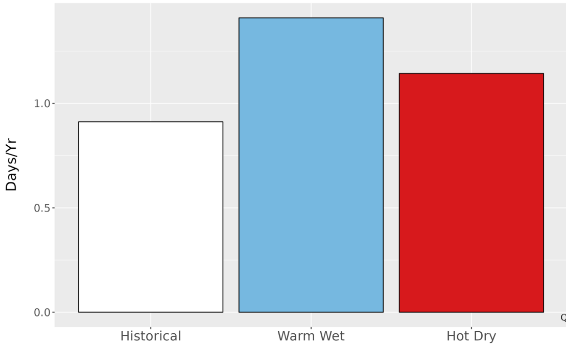
Figure 6. Average number of days annually with precipitation exceeding the 99th percentile (2.4 in.) of precipitation from the historical period 1979-2012 and for each climate future.
