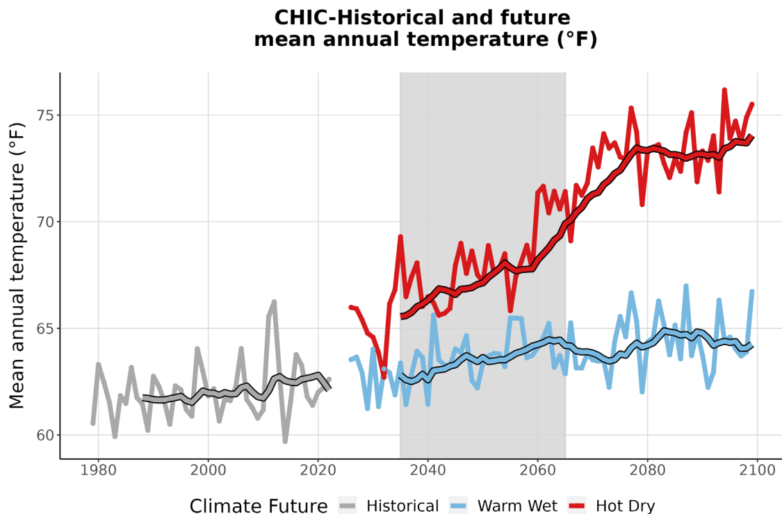
Figure 3. This graph compares observed average annual temperature at CHIC (°F) (1979-2022) with projected average annual temperature for the two climate futures over the period 2023-2099. The historically observed data
