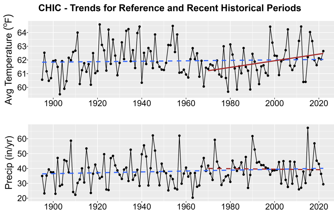
Figure 1. Historical trends in annual average temperature (upper plot) and annual total precipitation (lower plot) for CHIC from 1895-2022. Black points show yearly values while blue lines are linear regressions for the entire period record and red lines for 1970-2022 trends. Solid lines are significant trends (i.e., p < 0.05 ); dashed lines are not statistically significant.
