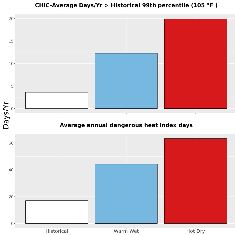
Figure 5. The upper bar graph represents the average number of days annually with temperatures greater than the historical 99th percentile (105 °F) historically (1979-2012) and for the two climate futures (2050). The bottom bar graph represents the average annual number of dangerous heat index days historically and for the two climate futures. Dangerous heat index days are days that exceed 105 °F.
