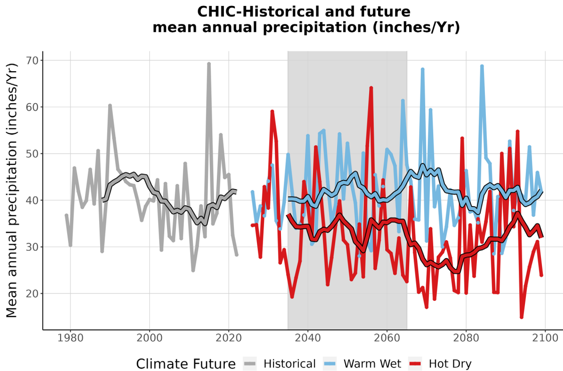
Figure 4. This graph compares observed average annual precipitation at CHIC (inches/year) (1979-2022) with projected average annual precipitation for the two climate futures over the period 2023-2099. The historically observed data is shown in gray, the Warm Wet climate future in blue, and the Hot Dry climate future in red. The smooth line running through each projection is the 10-year running average for historical observations and future projections. The gray-shaded area represents the time period that was averaged (2035-2065) to summarize future projections for the year 2050 (Appendix 1).
