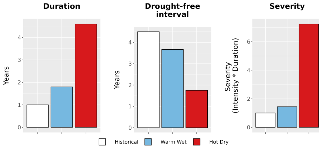
Figure 8. Drought metrics for CHIC. (Left) Average drought duration (years) historically (1979-2012) and under each climate future. (Middle) Average drought return interval (years), indicating the expected amount of time between periods of drought, historically and under each climate future. (Right) Average drought severity, a measure of drought intensity multiplied by duration, historically and under each climate future.
