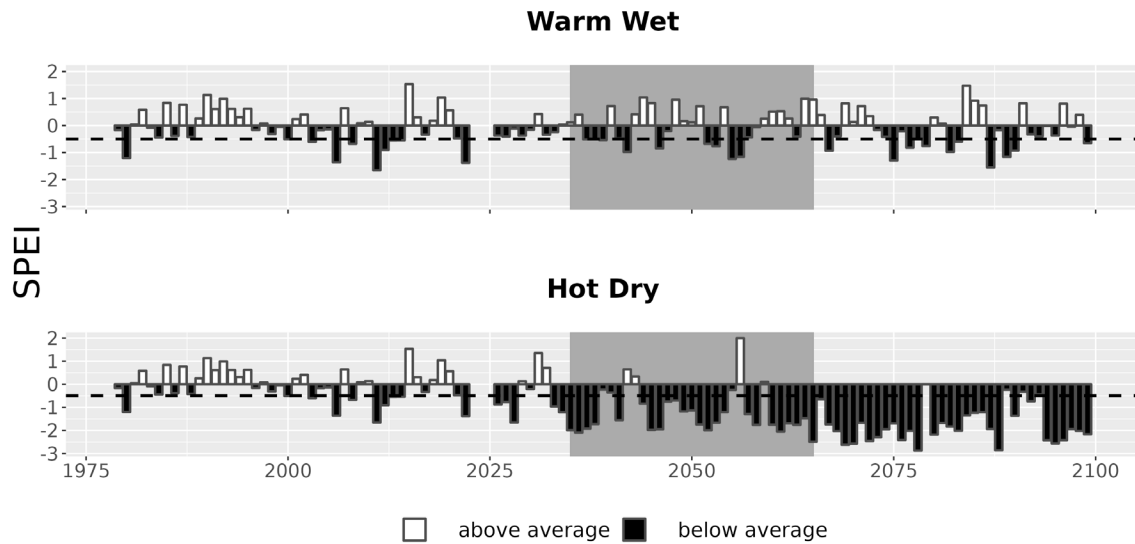
Figure 7. Drought metrics for CHIC. Drought index (SPEI; units = standard deviations from historical) timeseries for each climate future. Below-average SPEI (black bars) indicates dry conditions. The dotted line (SPEI = -0.5) indicates drought conditions.
