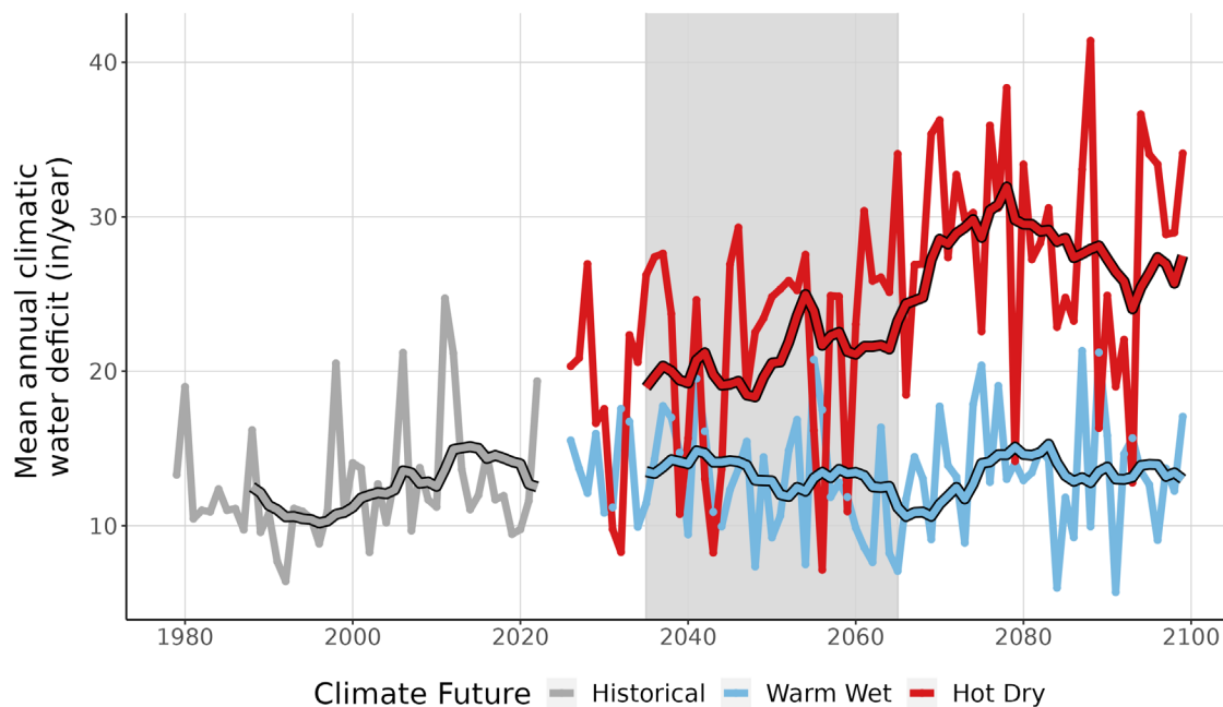
Figure 9. This line graph compares observed climatic water deficit at CHIC (inches/year) (1979-2022) with projected climatic water deficit for the two climate futures over the period 2023-2099. The historical observation data is shown in gray, the Warm Wet climate future in blue, and the Hot Dry climate future in red. The smooth line running through each projection is the 10-year running average for historical observations and future projections. Gray-shaded area represents the time period that was averaged (2035-2065) to summarize future projections for the year 2050.
