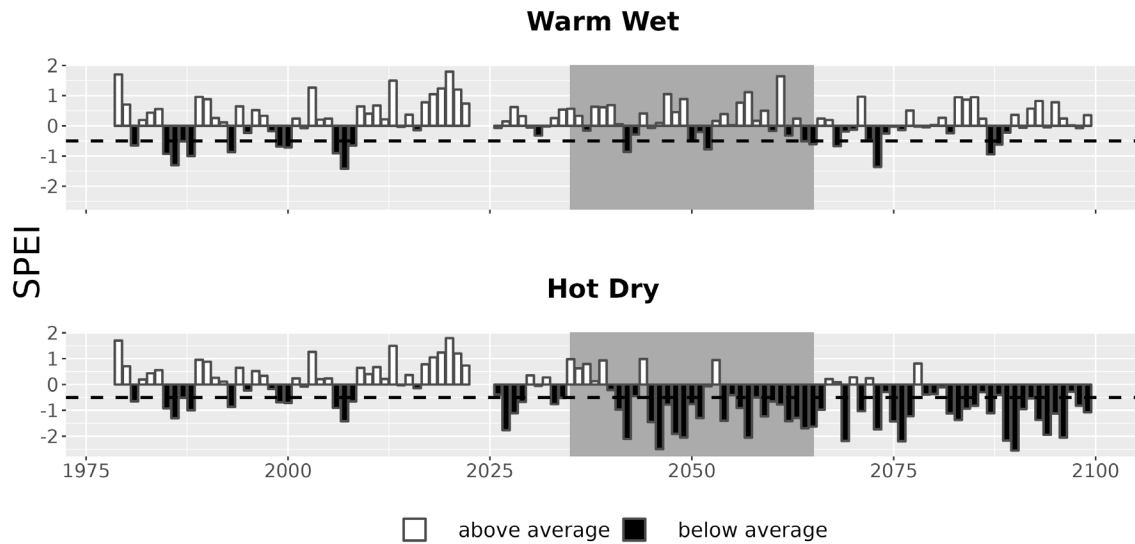
Figure 7. Drought metrics for CHCH. Drought index (SPEI; units = standard deviations from historical) timeseries for each climate future. Below-average SPEI (black bars) indicates dry conditions. The dotted line (SPEI = -0.5) indicates drought conditions.
