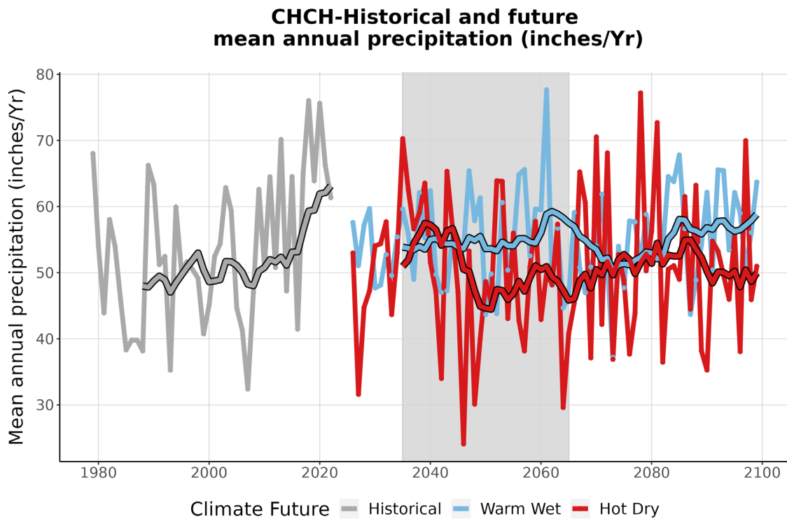
Figure 4. This graph compares observed average annual precipitation at CHCH (inches/year) (1979-2022) with projected average annual precipitation for the two climate futures over the period 2023-2099. The historically observed data is shown in gray, the Warm Wet climate future in blue, and the Hot Dry climate future in red. The smooth line running through each projection is the 10-year running average for historical observations and future projections. The gray-shaded area represents the time period that was averaged (2035-2065) to summarize future projections for the year 2050 (Appendix 1).
