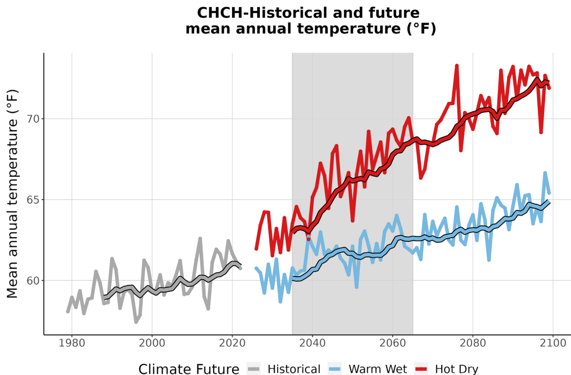
Figure 3. This graph compares observed average annual temperature at CHCH (°F) (1979-2022) with projected average annual temperature for the two climate futures over the period 2023-2099. The historically observed data
