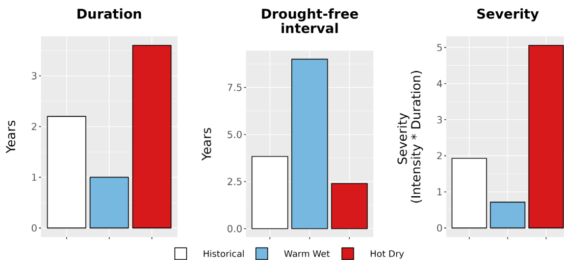
Figure 8. Drought metrics for CHCH. (Left) Average drought duration (years) historically (1979-2012) and under each climate future. (Middle) Average drought return interval (years), indicating the expected amount of time between periods of drought, historically and under each climate future. (Right) Average drought severity, a measure of drought intensity multiplied by duration, historically and under each climate future.
