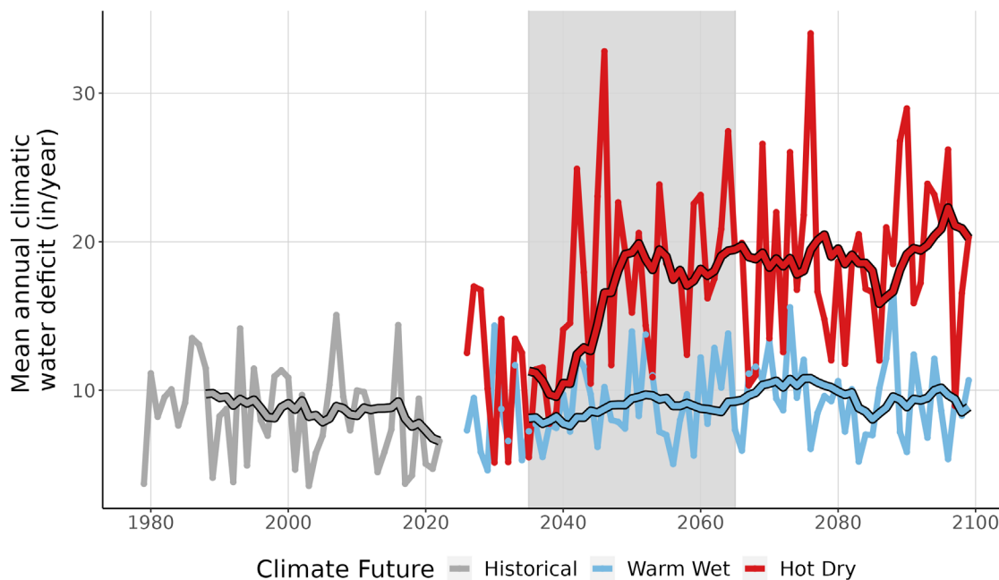
Figure 9. This line graph compares observed climatic water deficit at CHCH (inches/year) (1979-2022) with projected climatic water deficit for the two climate futures over the period 2023-2099. The historical observation data is shown in gray, the Warm Wet climate future in blue, and the Hot Dry climate future in red. The smooth line running through each projection is the 10-year running average for historical observations and future projections. Gray-shaded area represents the time period that was averaged (2035-2065) to summarize future projections for the year 2050.
