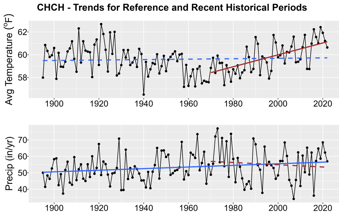
Figure 1. Historical trends in annual average temperature (upper plot) and annual total precipitation (lower plot) for CHCH from 1895-2022. Black points show yearly values while blue lines are linear regressions for the entire period record and red lines for 1970-2022 trends. Solid lines are significant trends (i.e., p < 0.05 ); dashed lines are not statistically significant.
